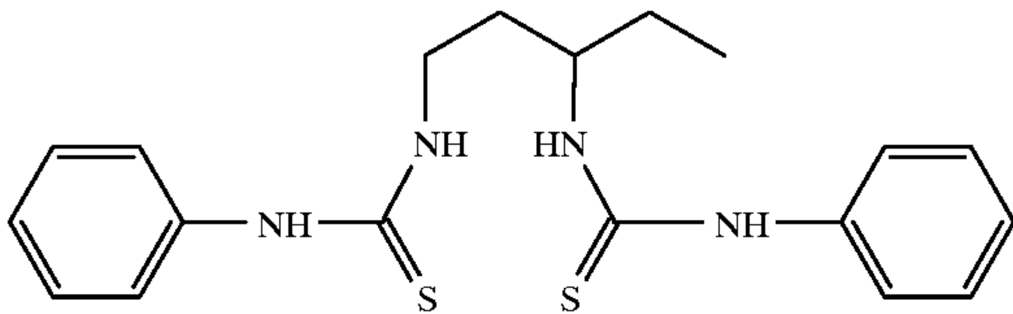
Et-DTU-Ph
