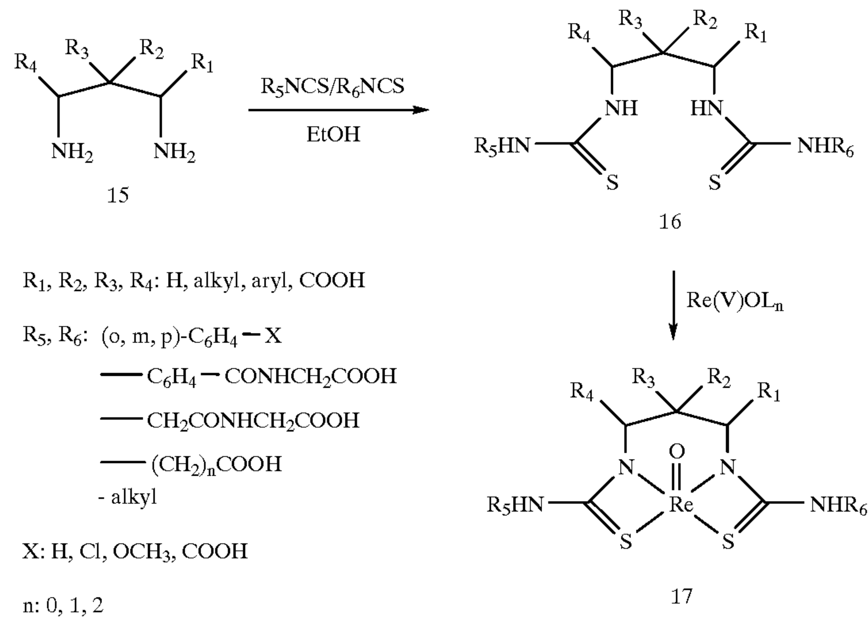
Scheme 4
