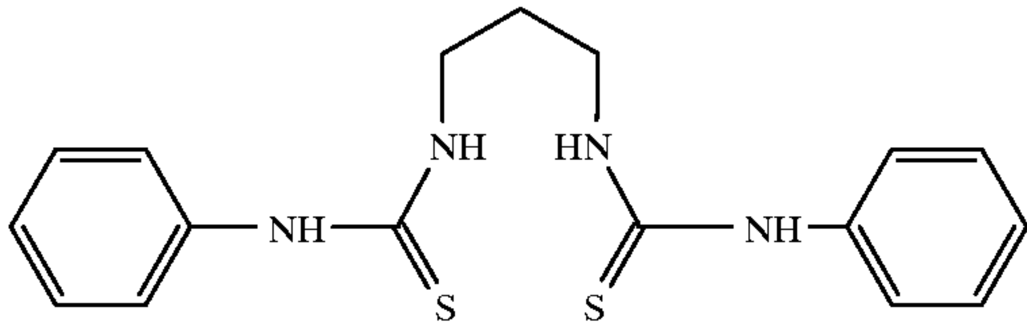
DTU-Ph
