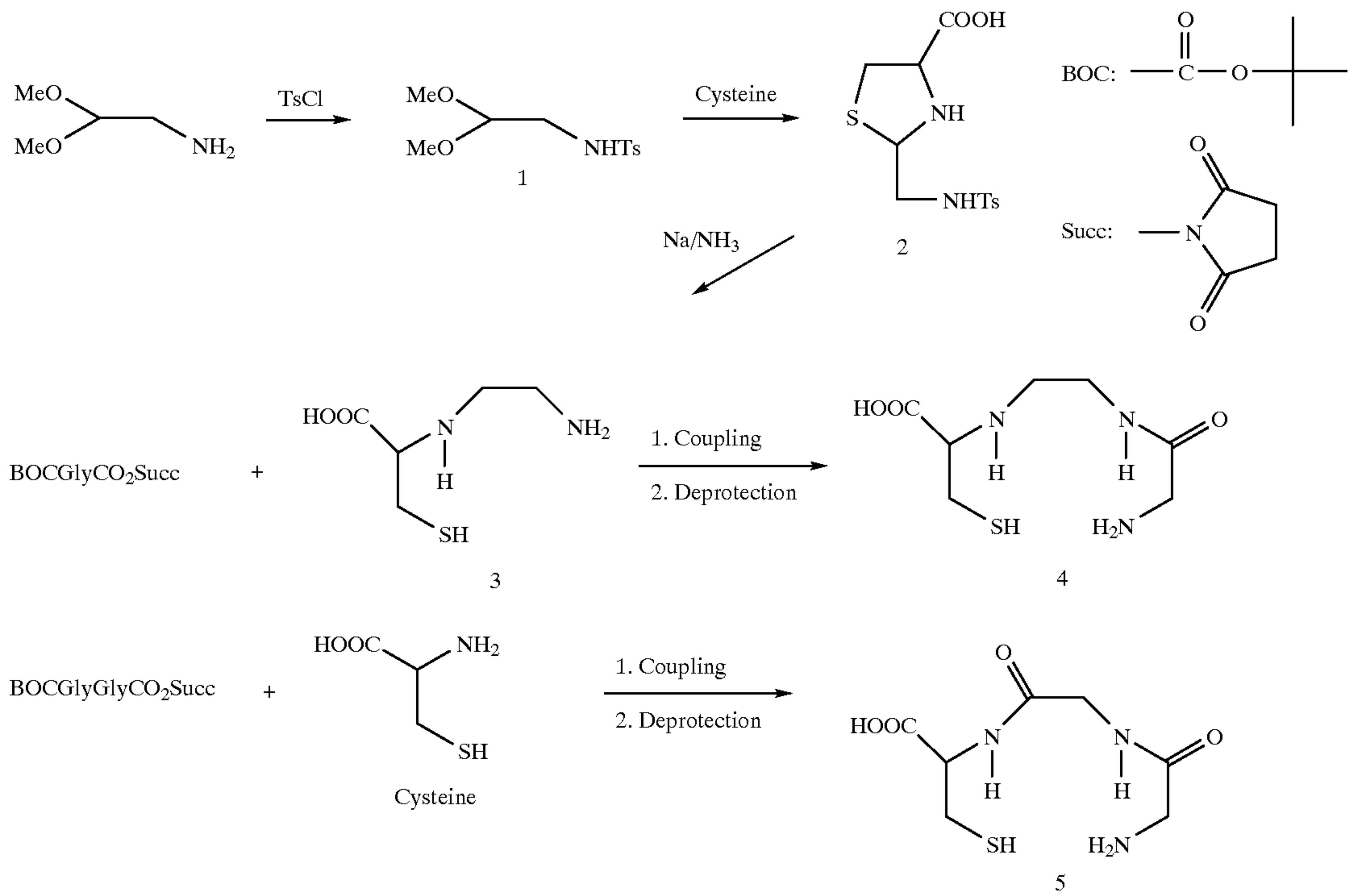
Scheme 1
