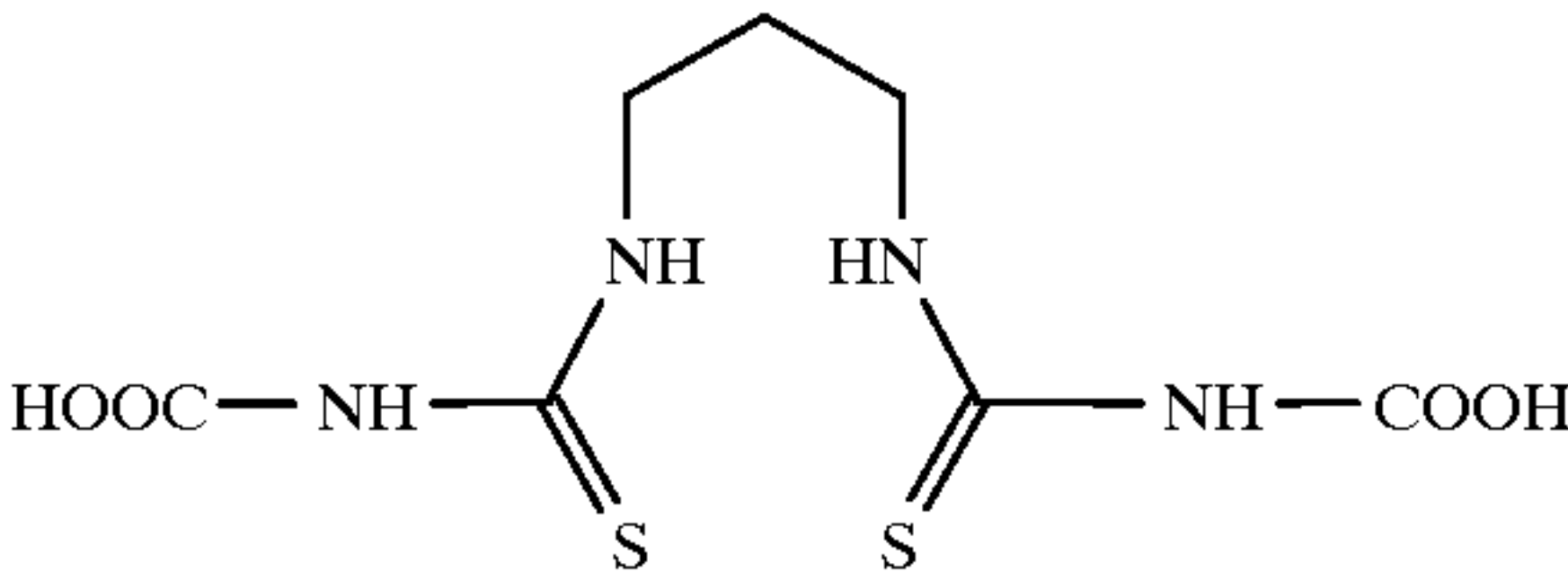
DTU-COOH
