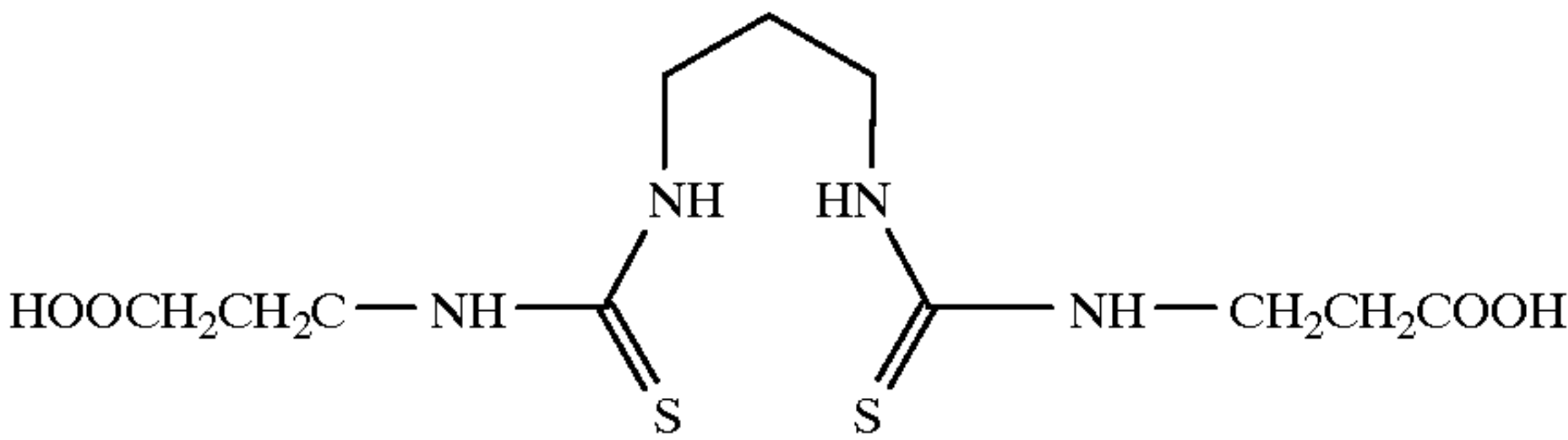
DTU-EtCOOH
