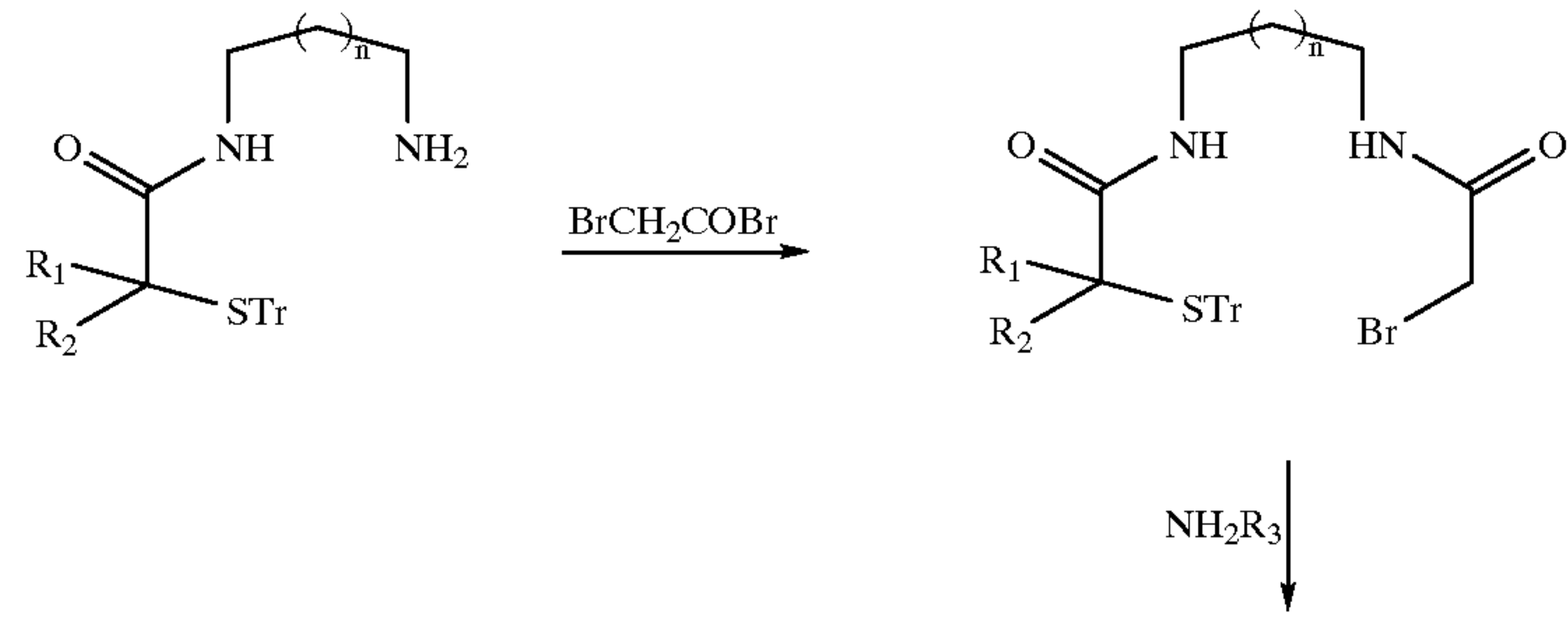
Scheme 5
