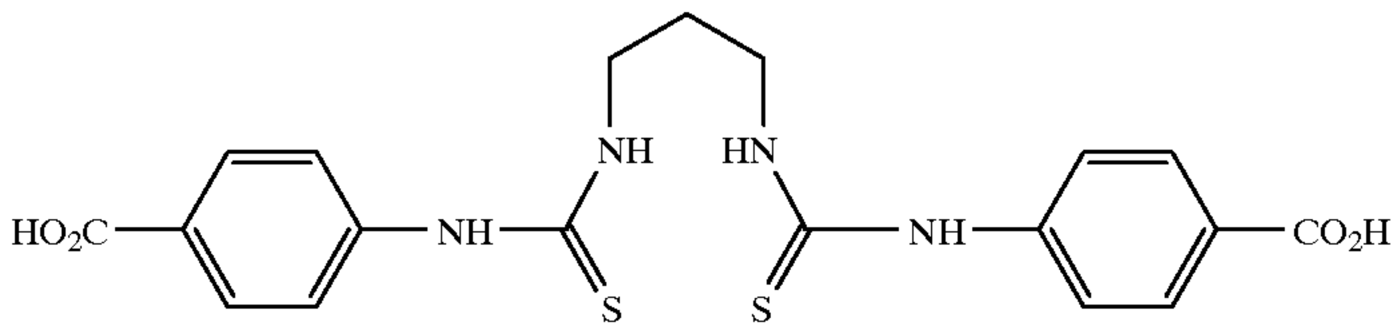
DTU-PhCOOH
