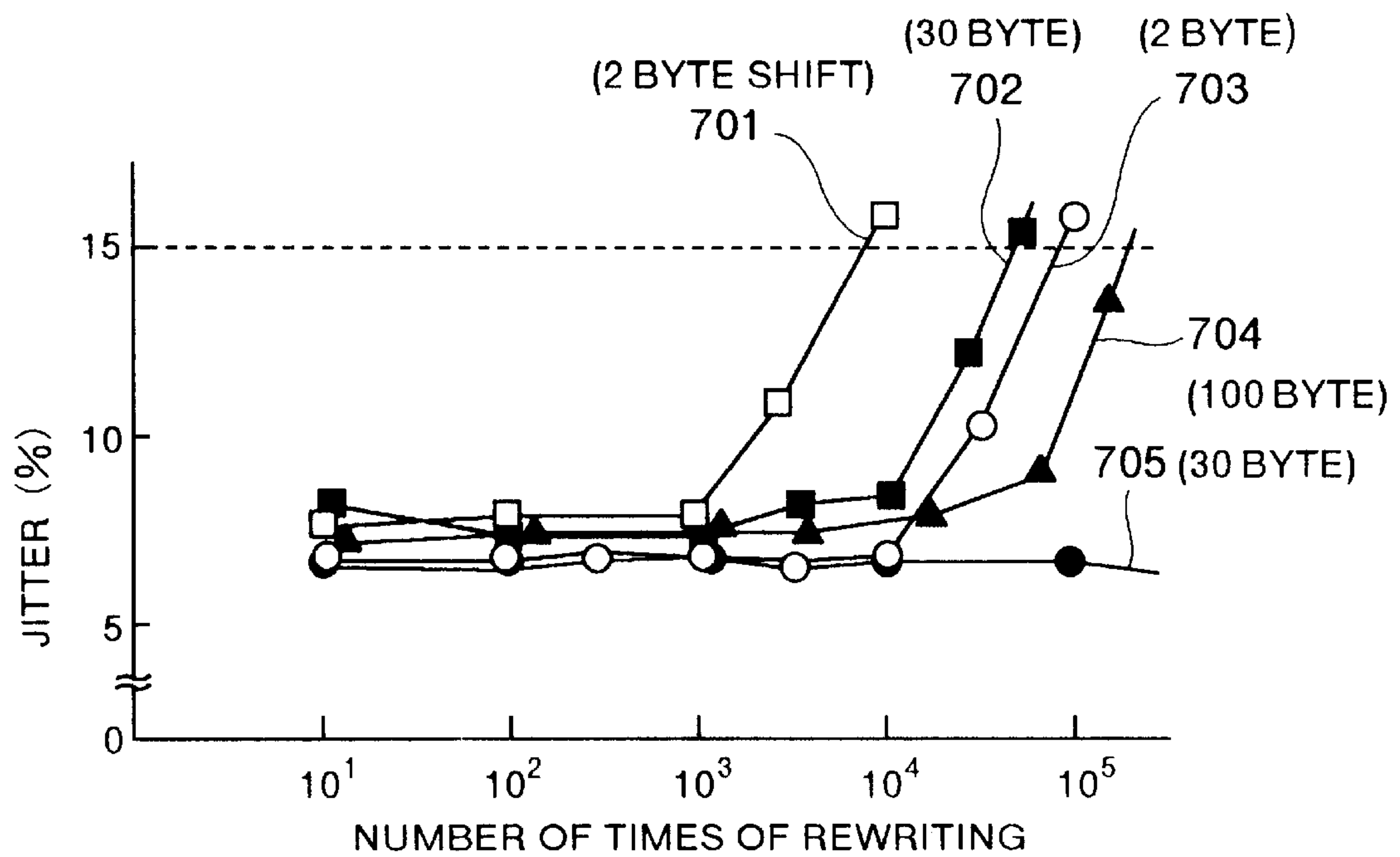
FIG.7 PRIOR ART
