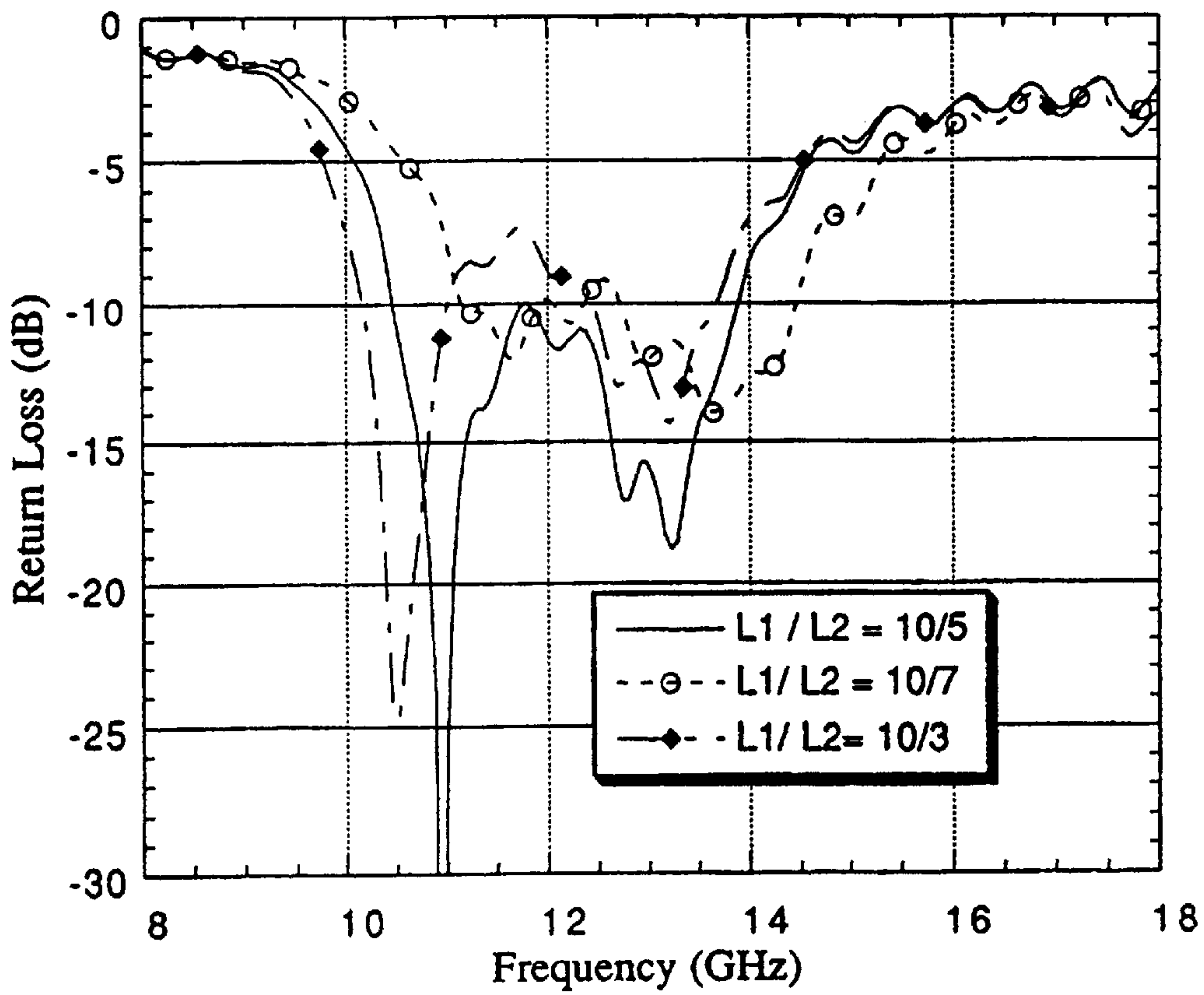
Figure 3 Return Loss of Rectangular Ring Dielectric Resonator Antennas
