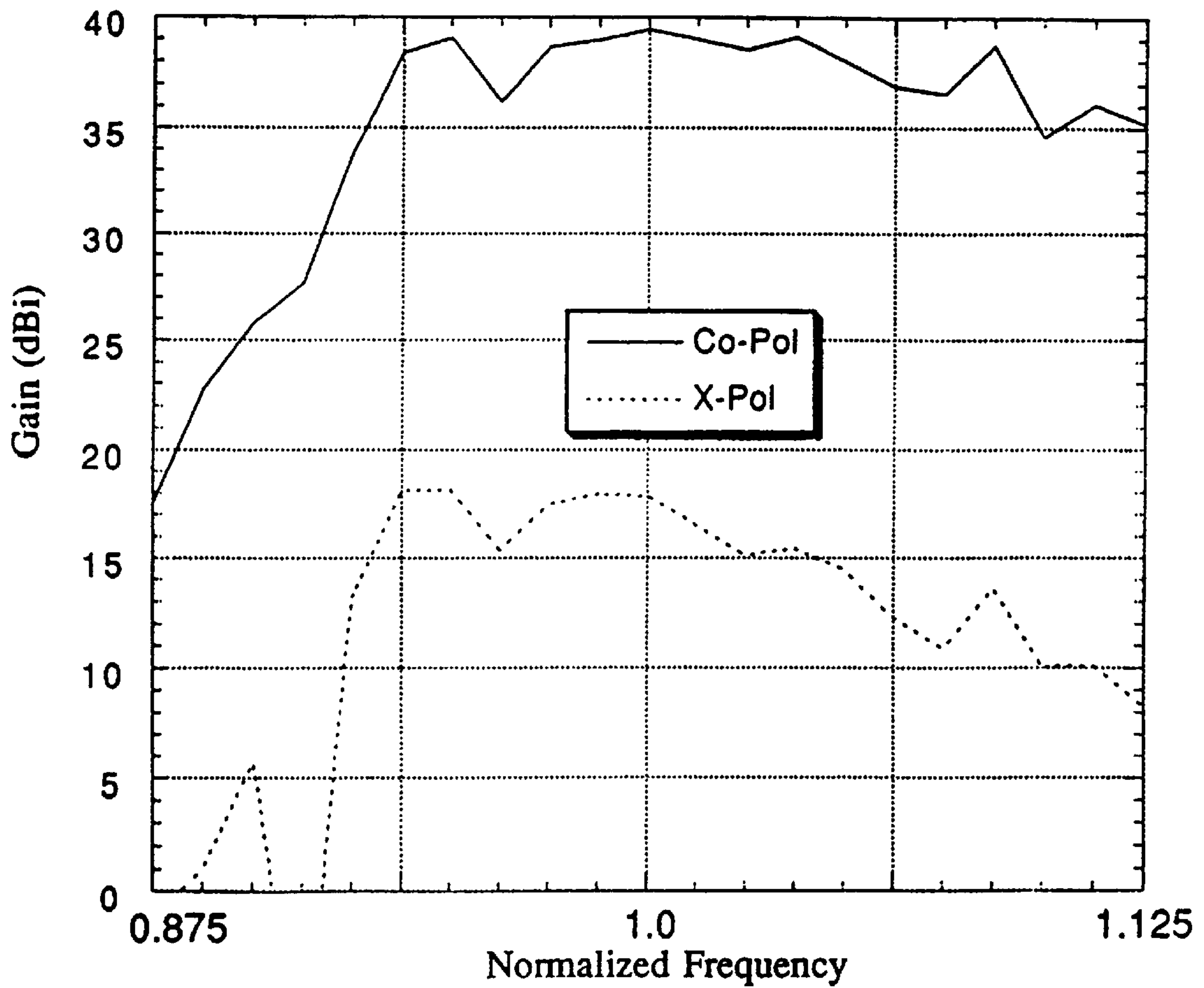
Figure 10 Active gain vs. normalized frequency of 320 DRA antenna
