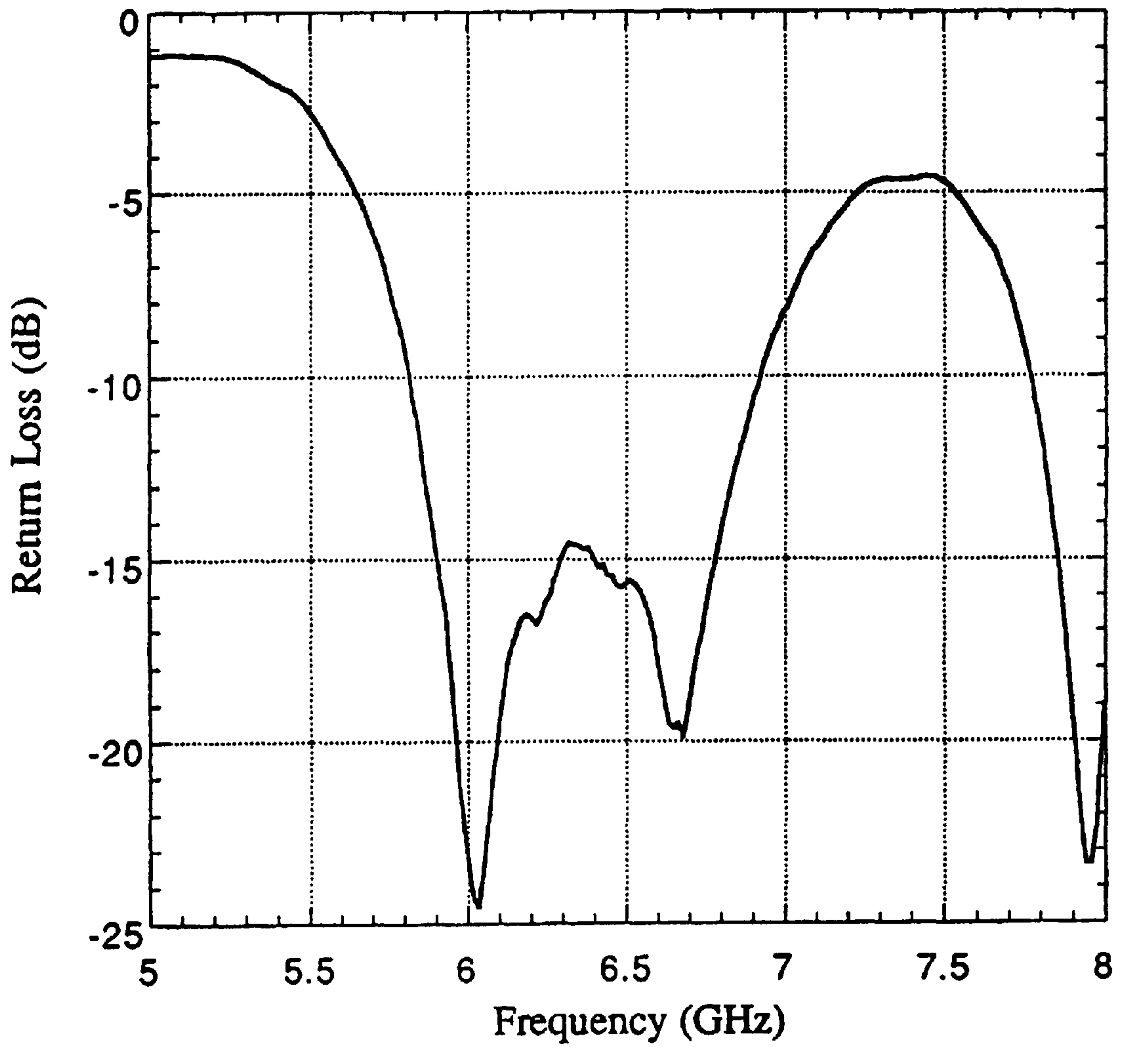
Figure 5 Measured return loss of MSDRA
