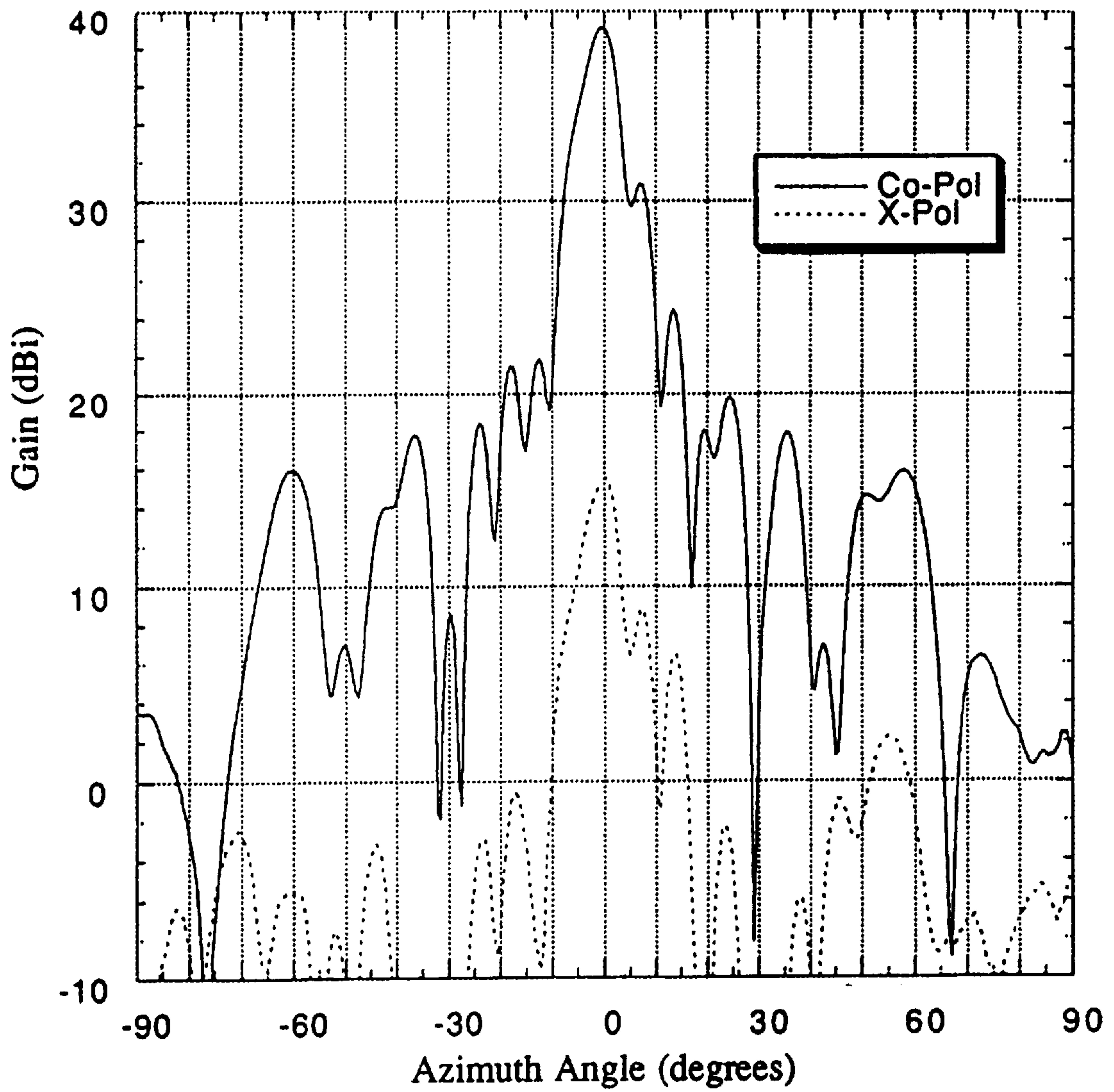
Figure 9 Measured azimuth pattern of the 320 DRA active array
