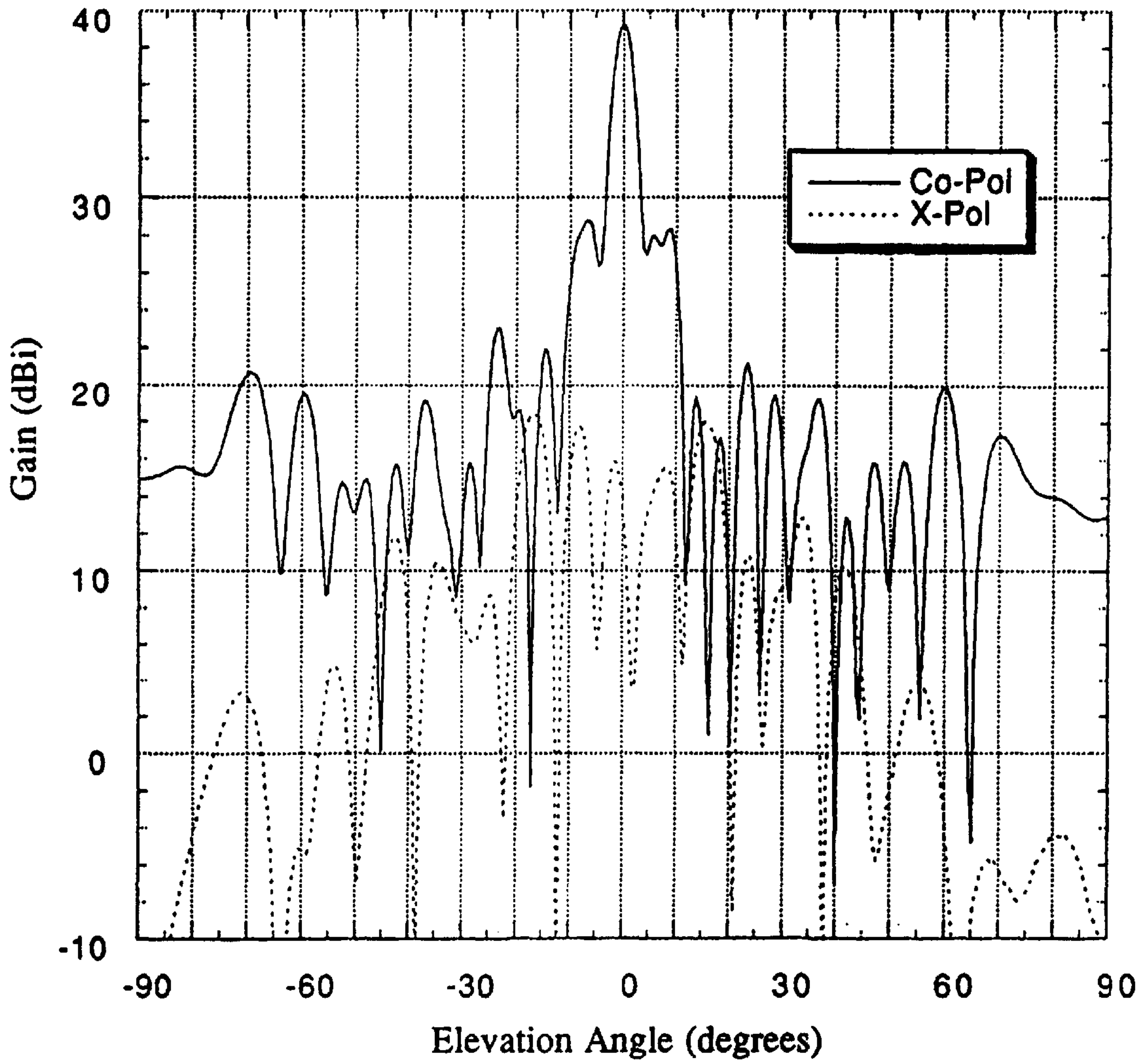
Figure 8 Measured elevation pattern of the 320 DRA active array
