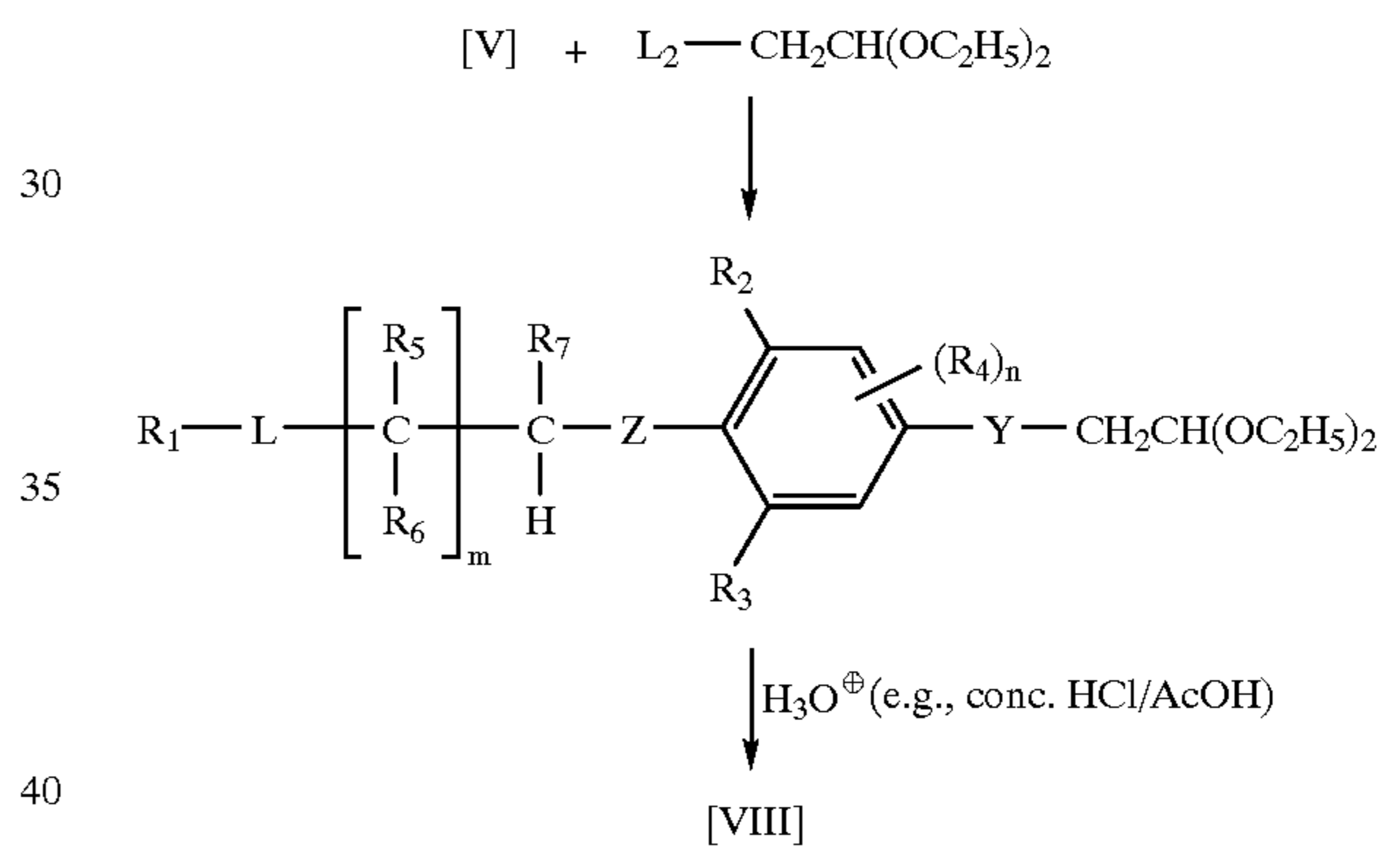
SCHEME 6
