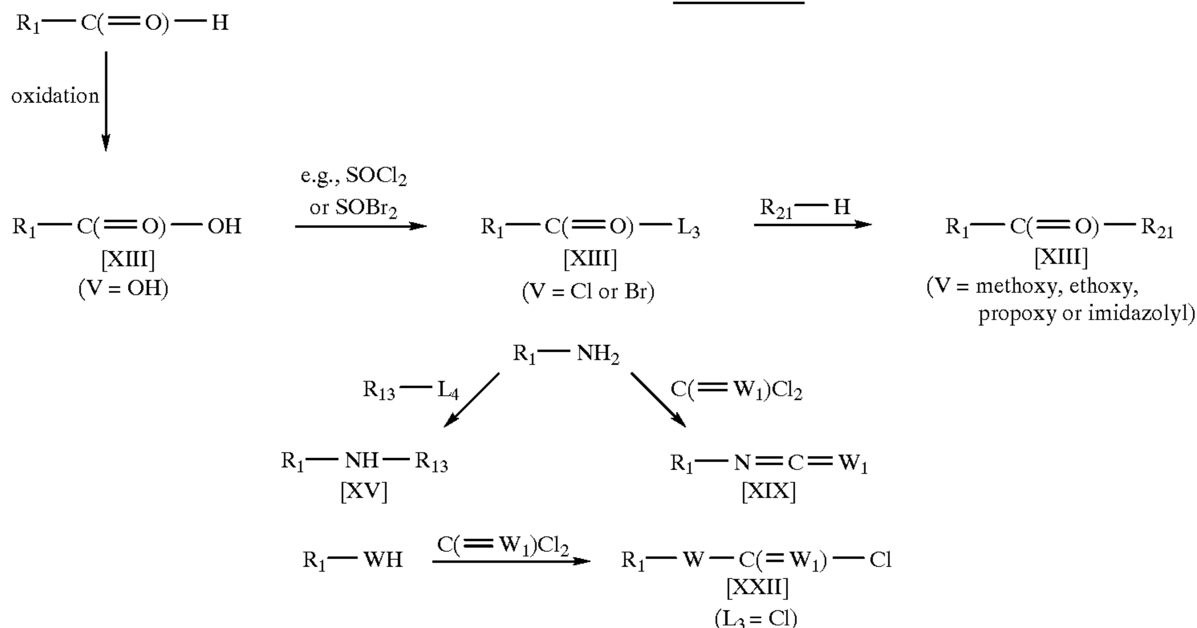
SCHEME 11
