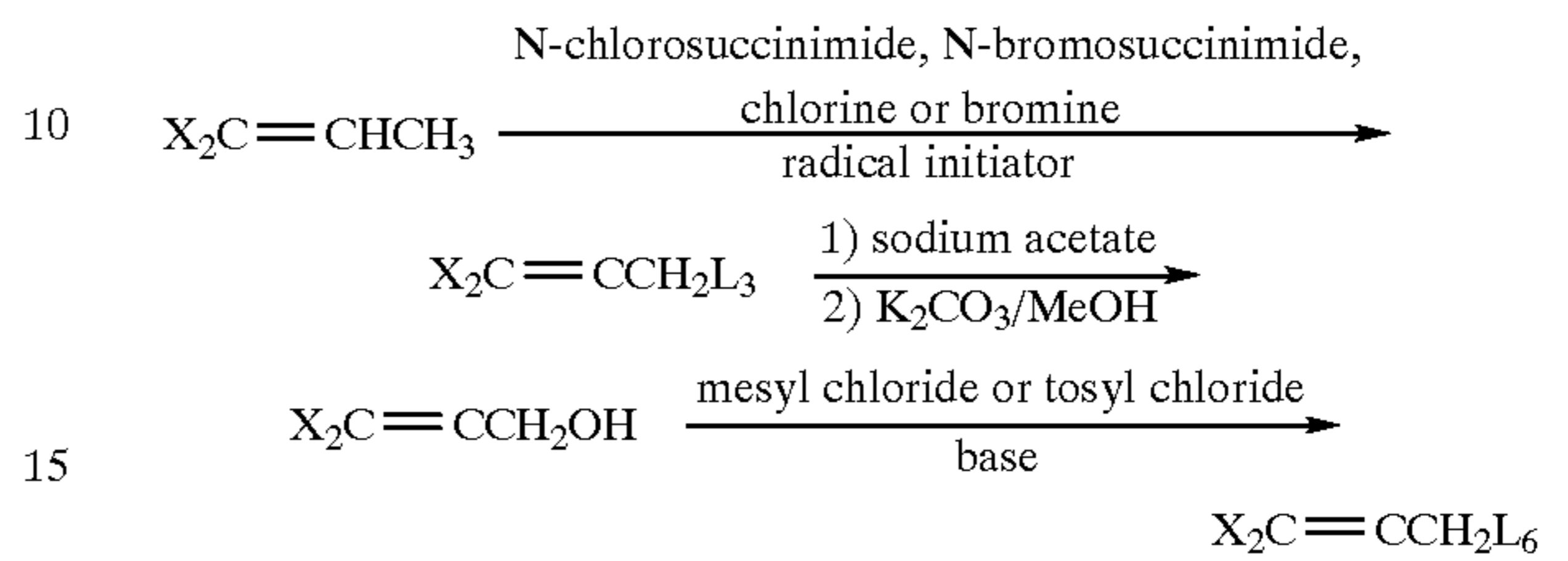
SCHEME 5
