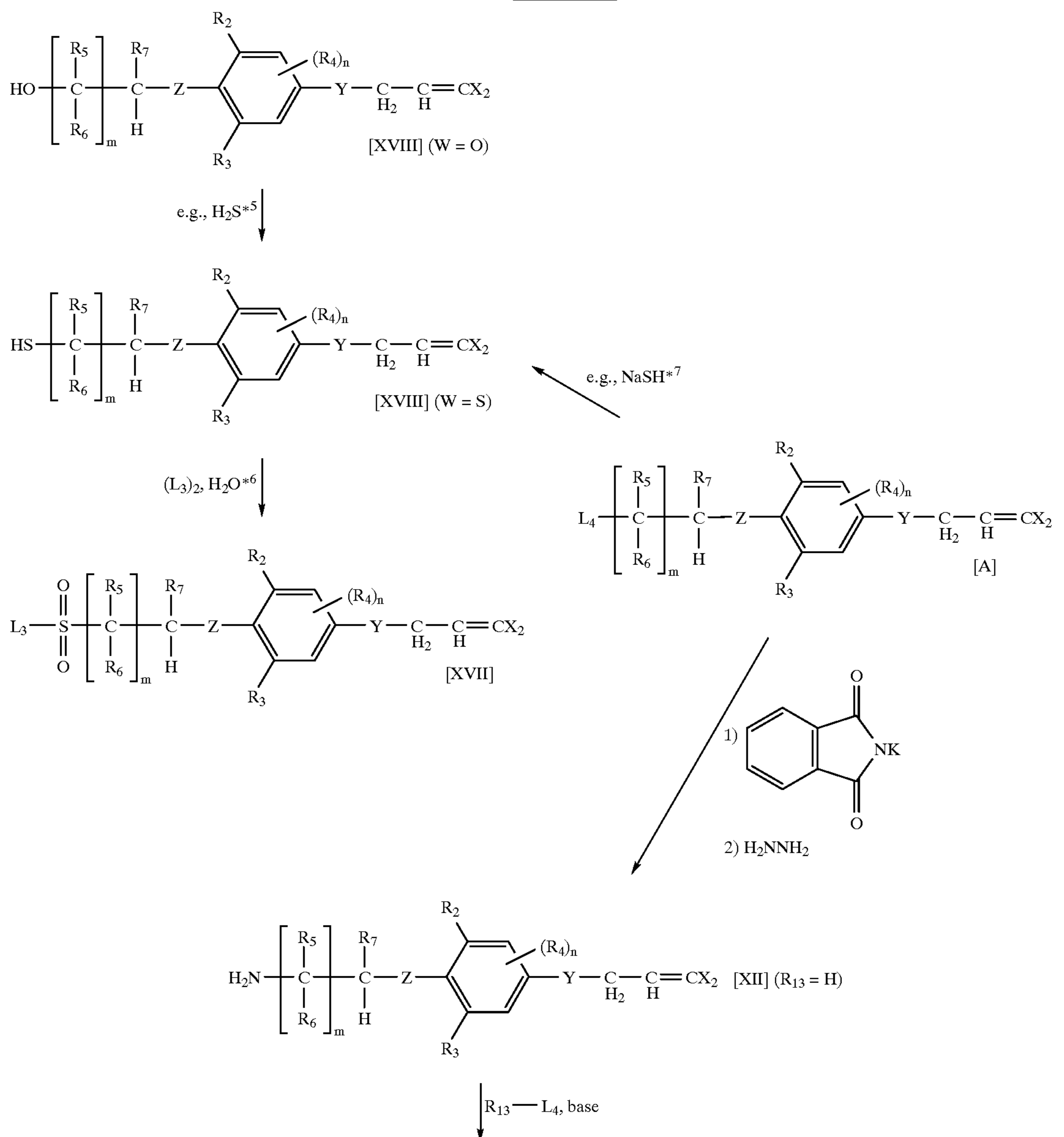
SCHEME 9.1
