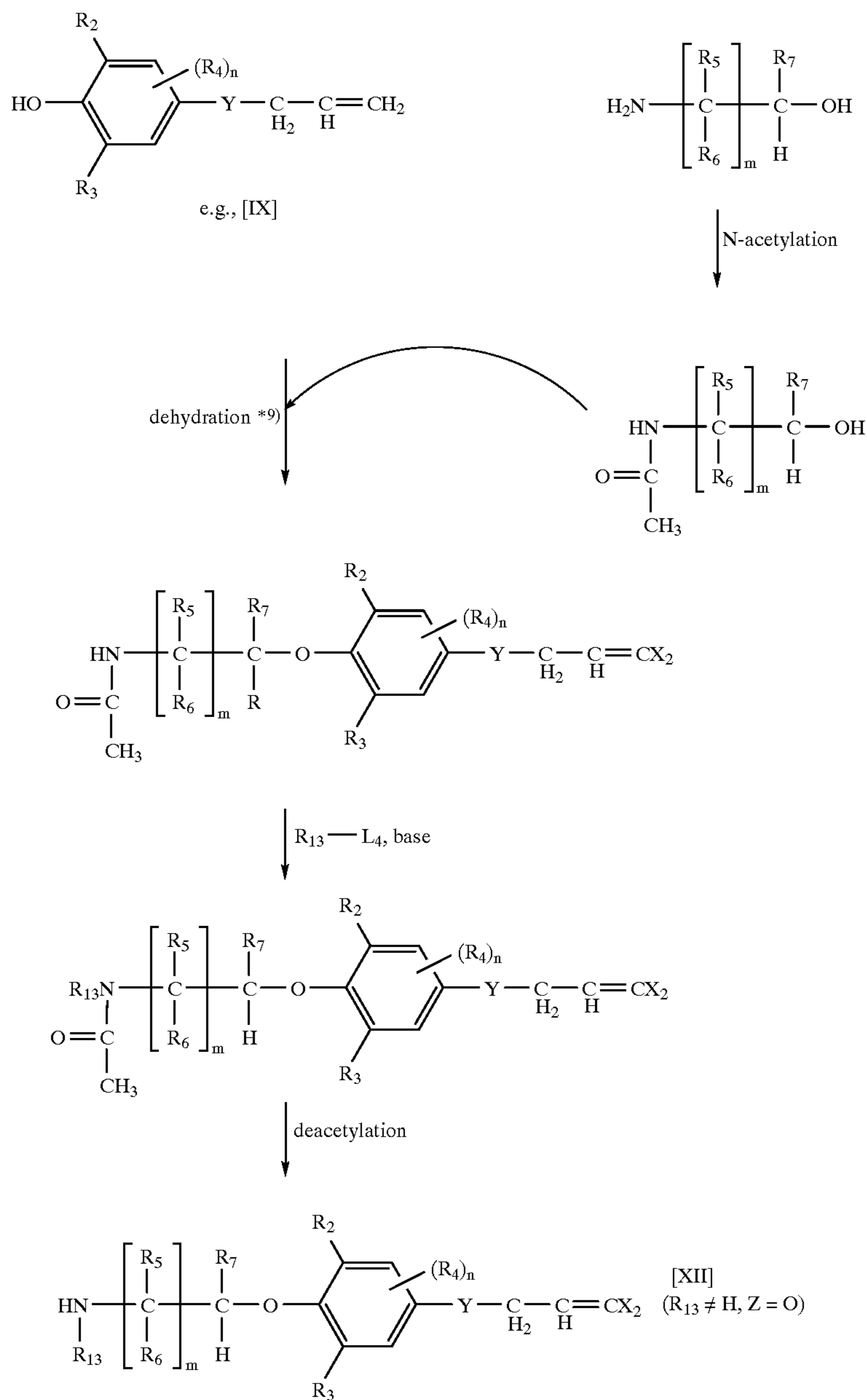
SCHEME 10
