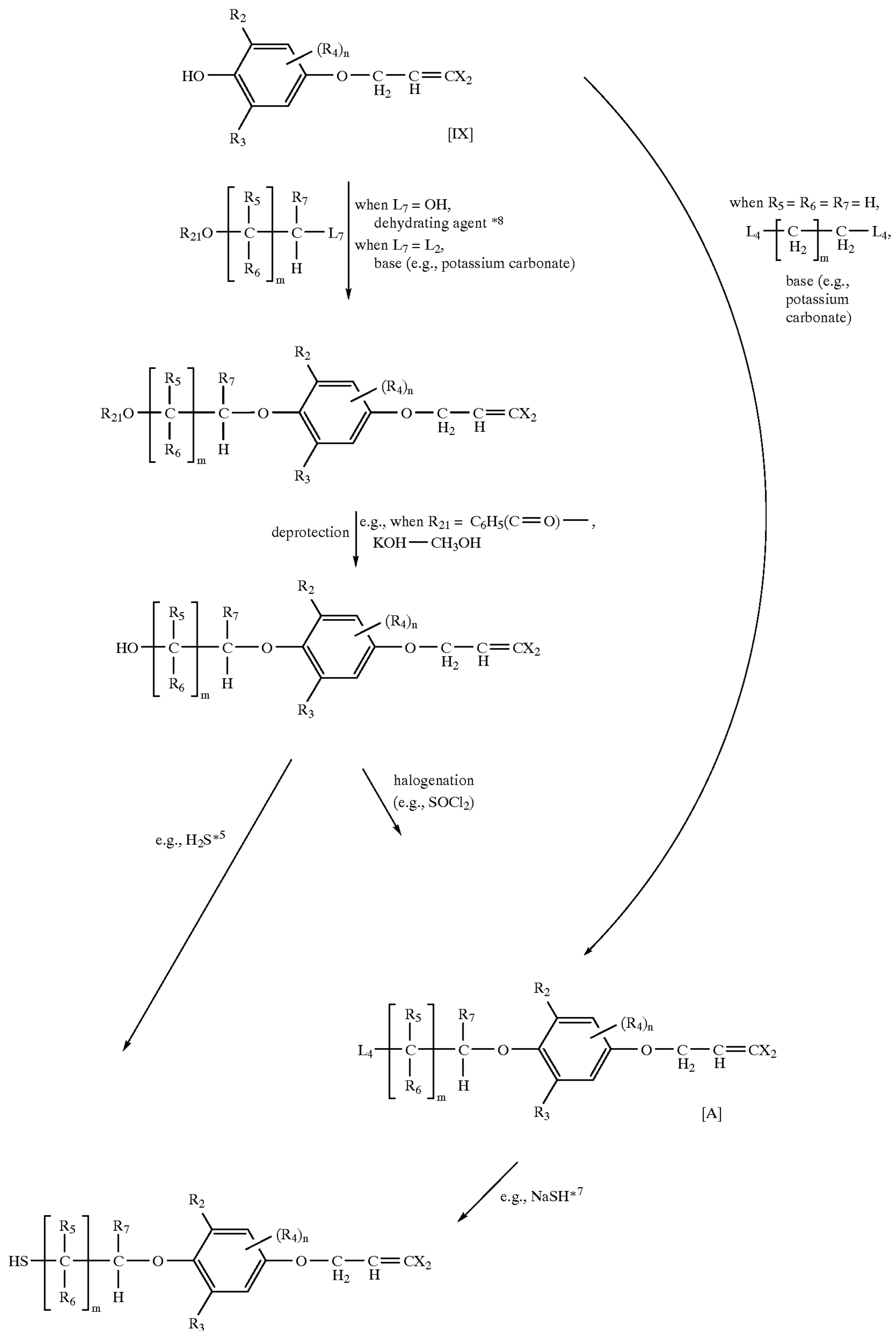
SCHEME 8.2
