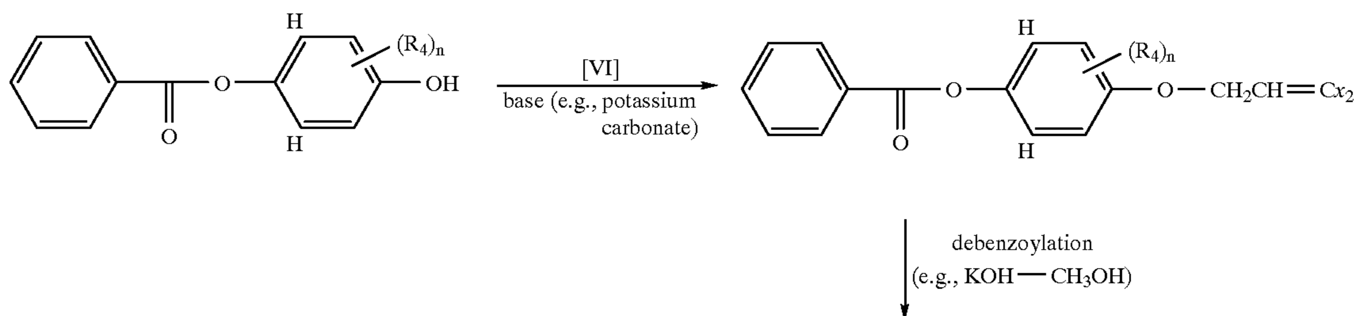
SCHEME 7
