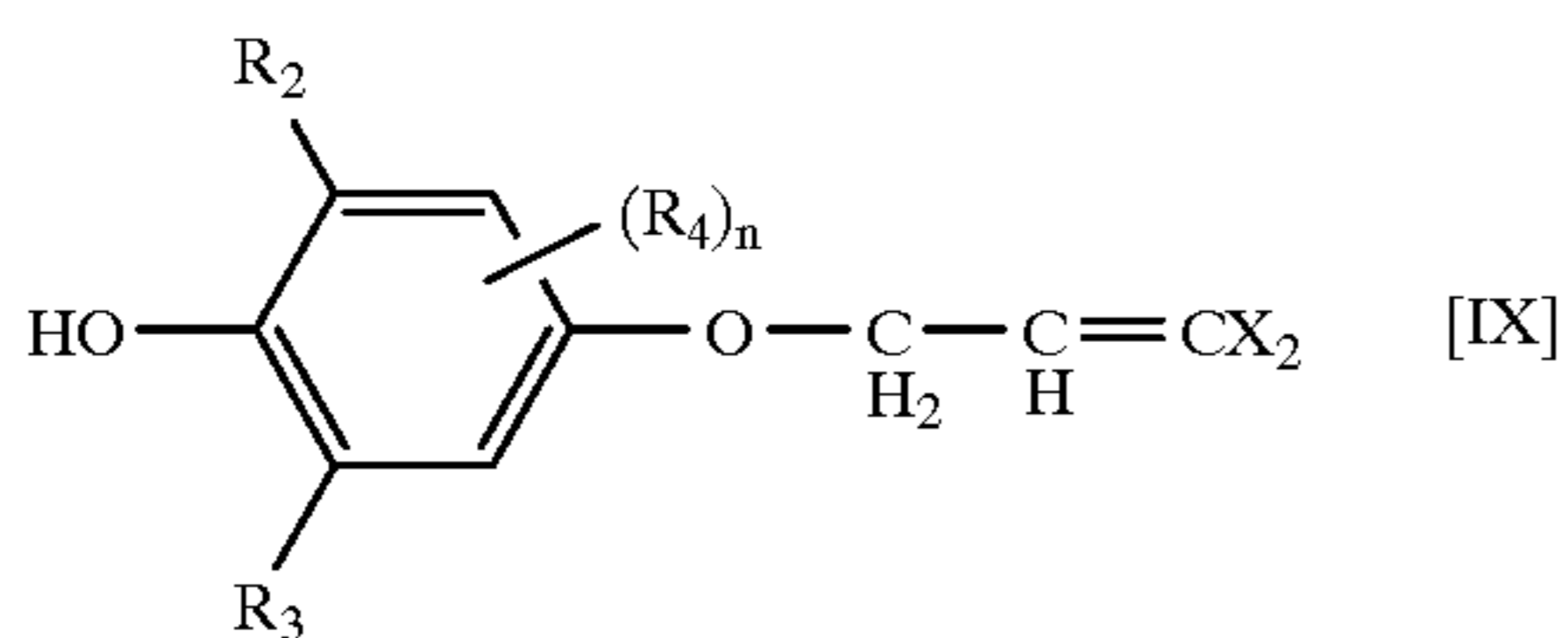
SCHEME 8.1
