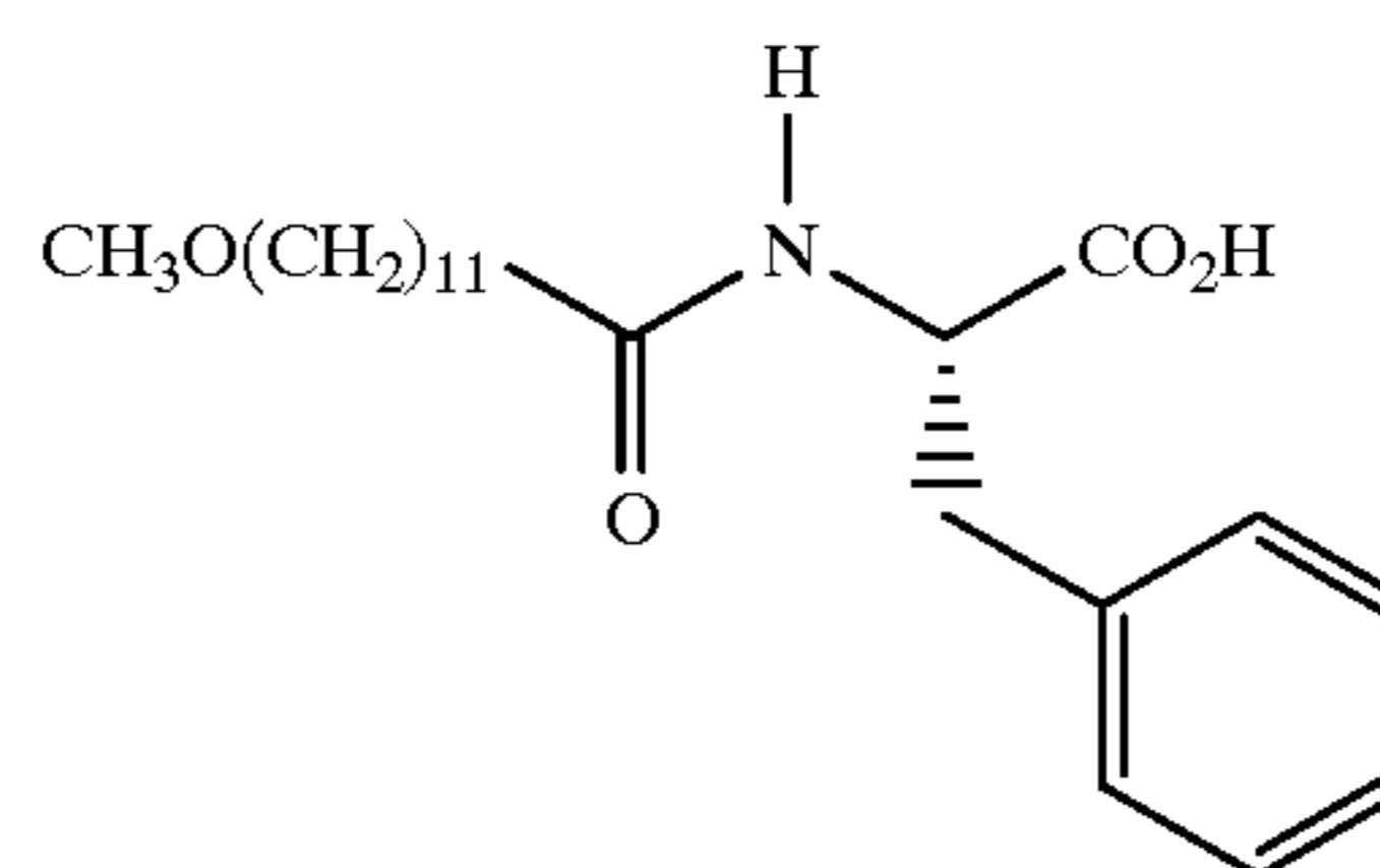
N-(12-Methoxy-1-oxododecyl)-L-phenylalanine
