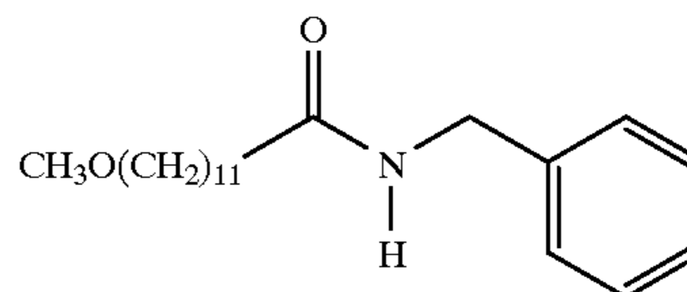
12-Methoxy-N-(phenylmethyl)dodecanamide
