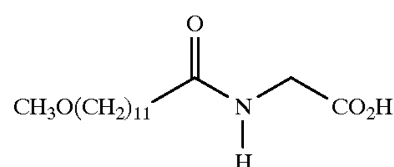
N-(12-Methoxy-1-oxododecyl)glycine
