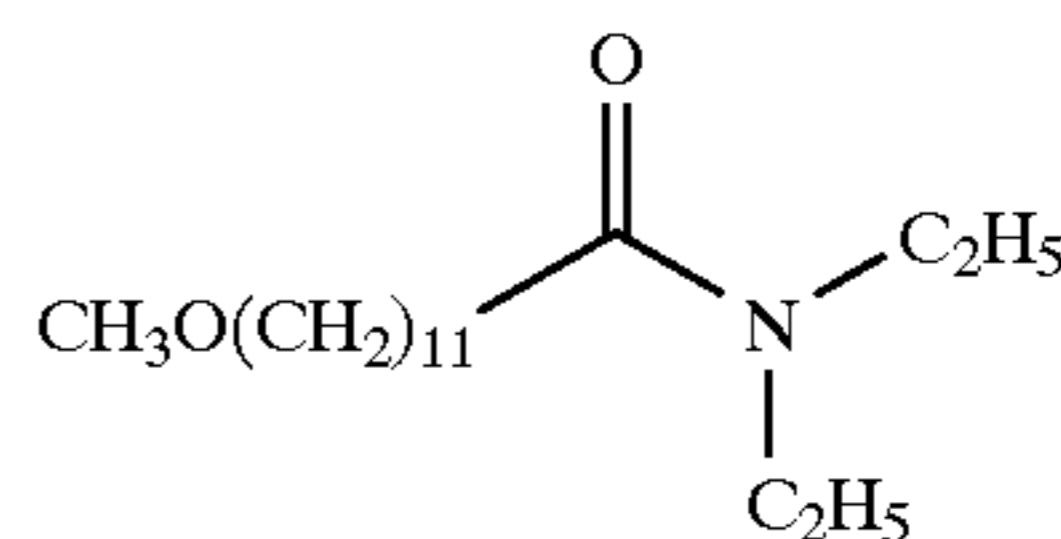
N,N-Diethyl-12-methoxydodecanamide
