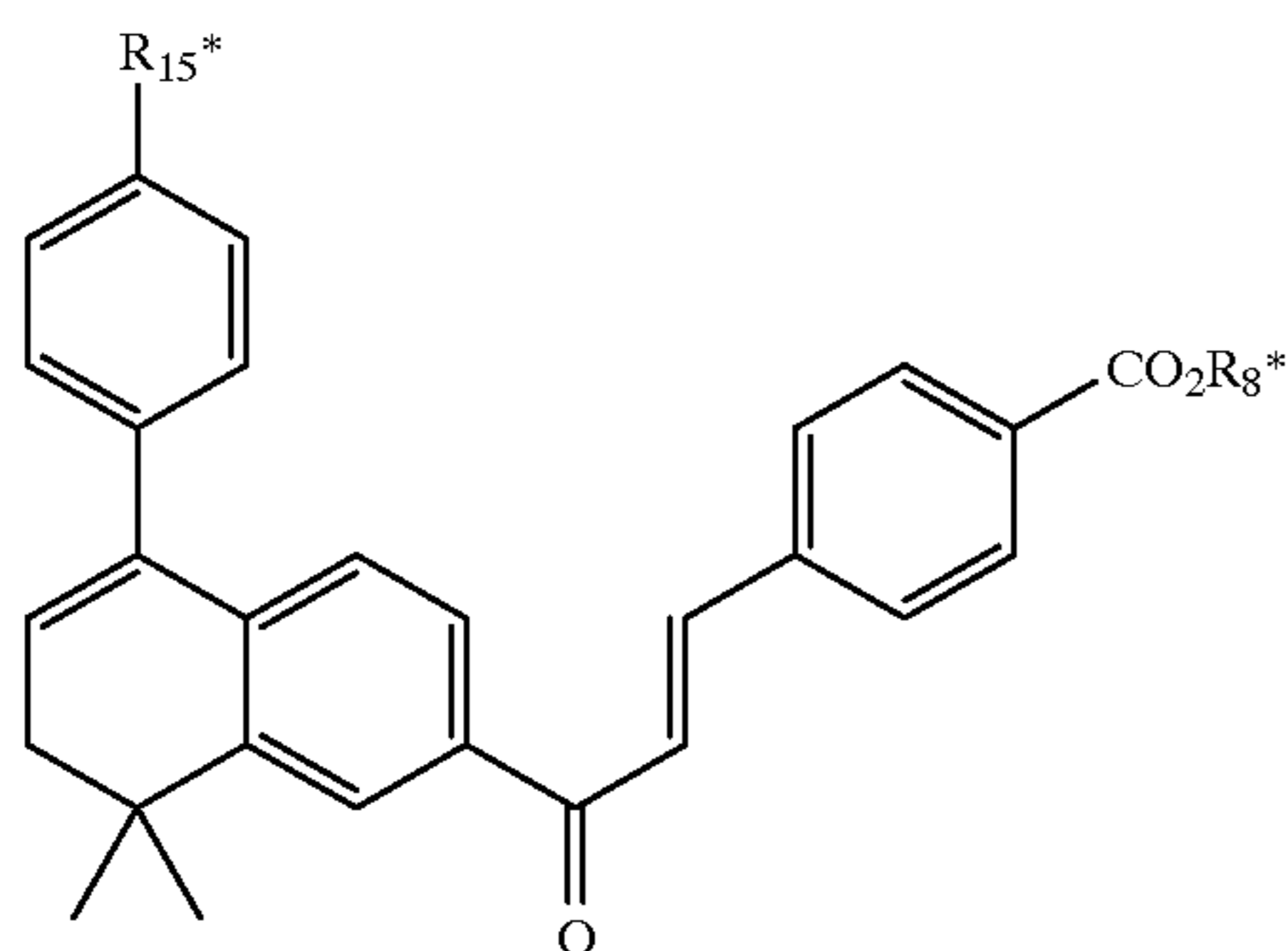
Formula 102
