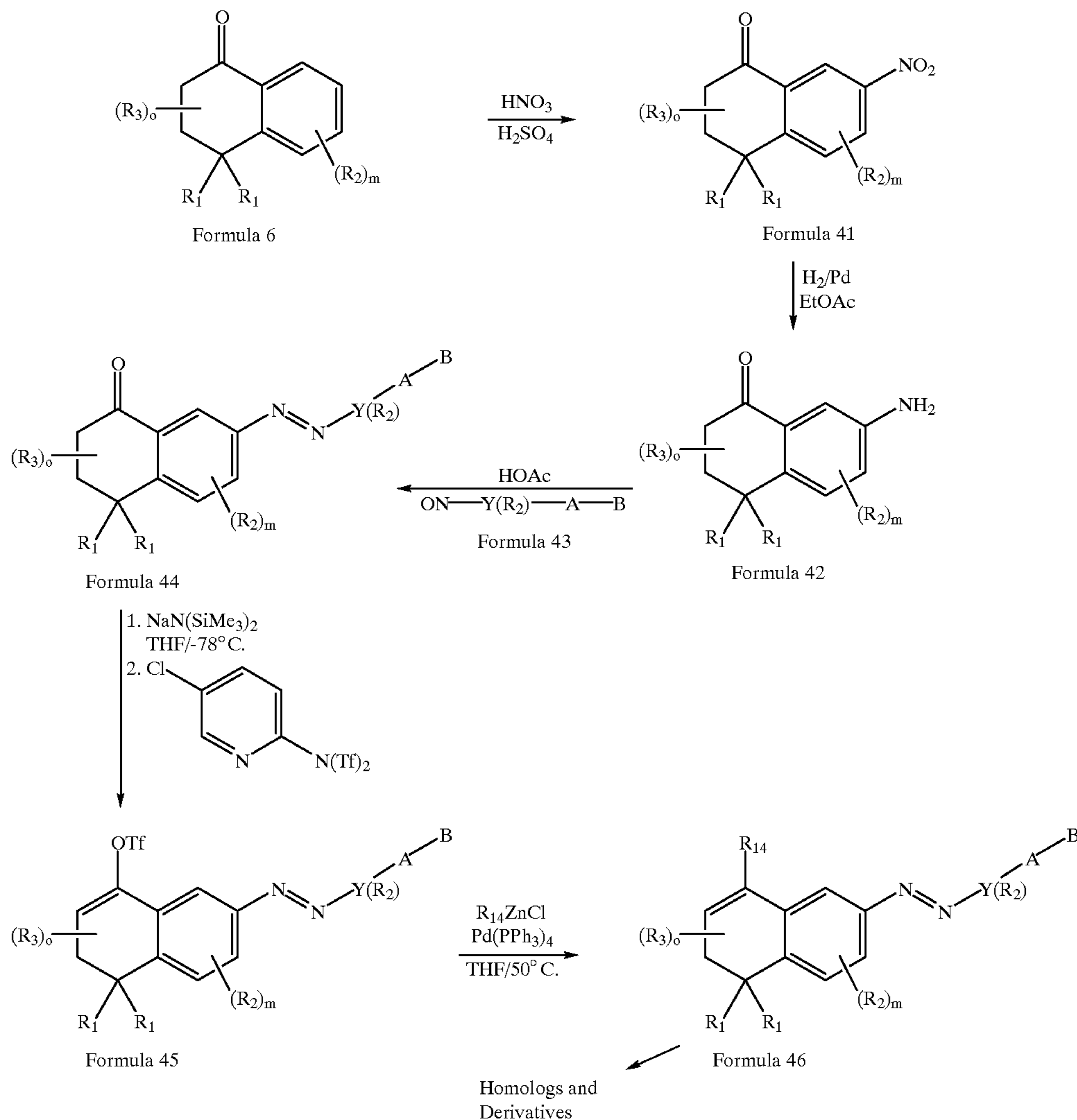
Reaction Scheme 5
