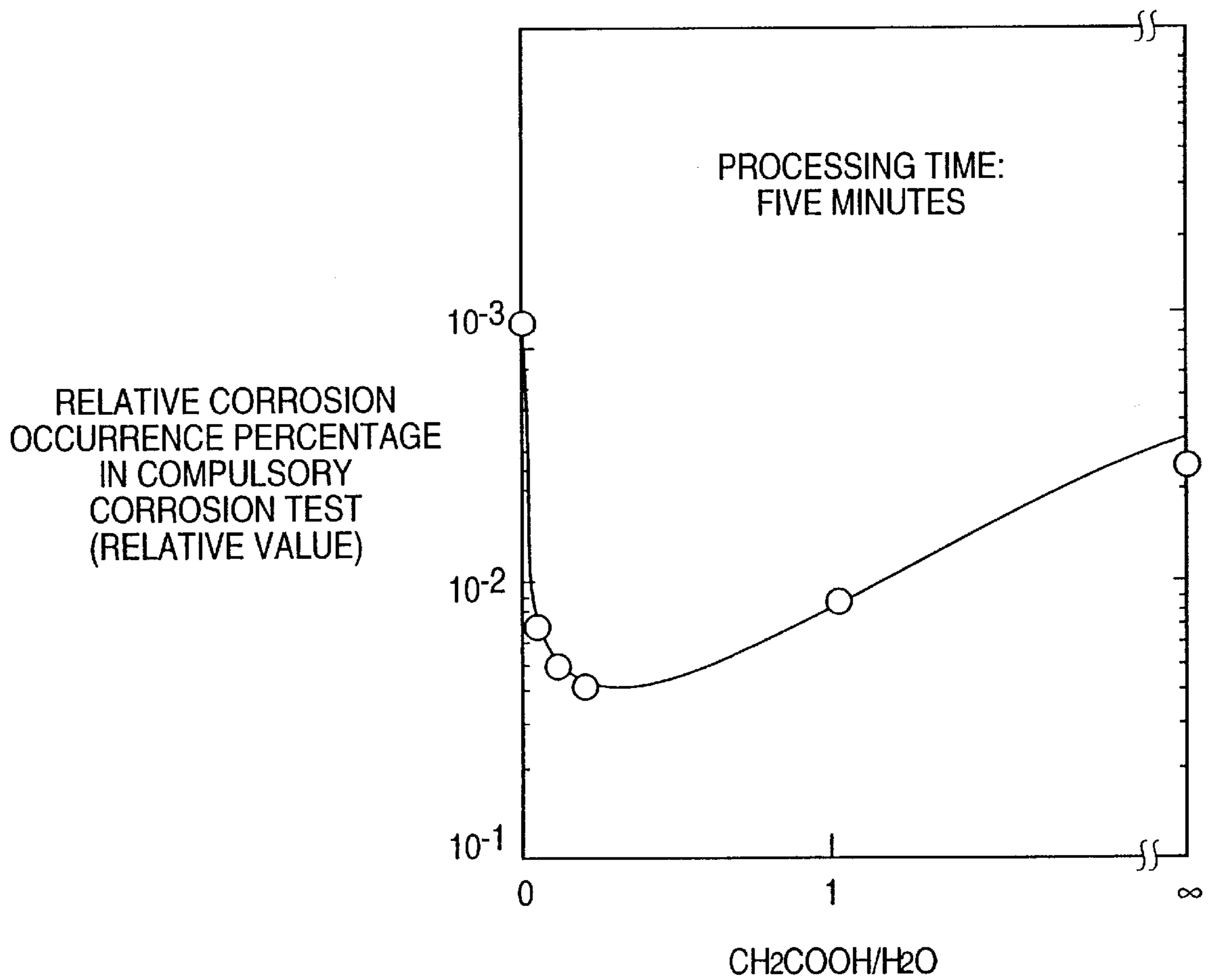
ACETIC ACID CONCENTRATION AND CORROSION OCCURRENCE PERCENTAGE IN ACETIC ACID WASHING
