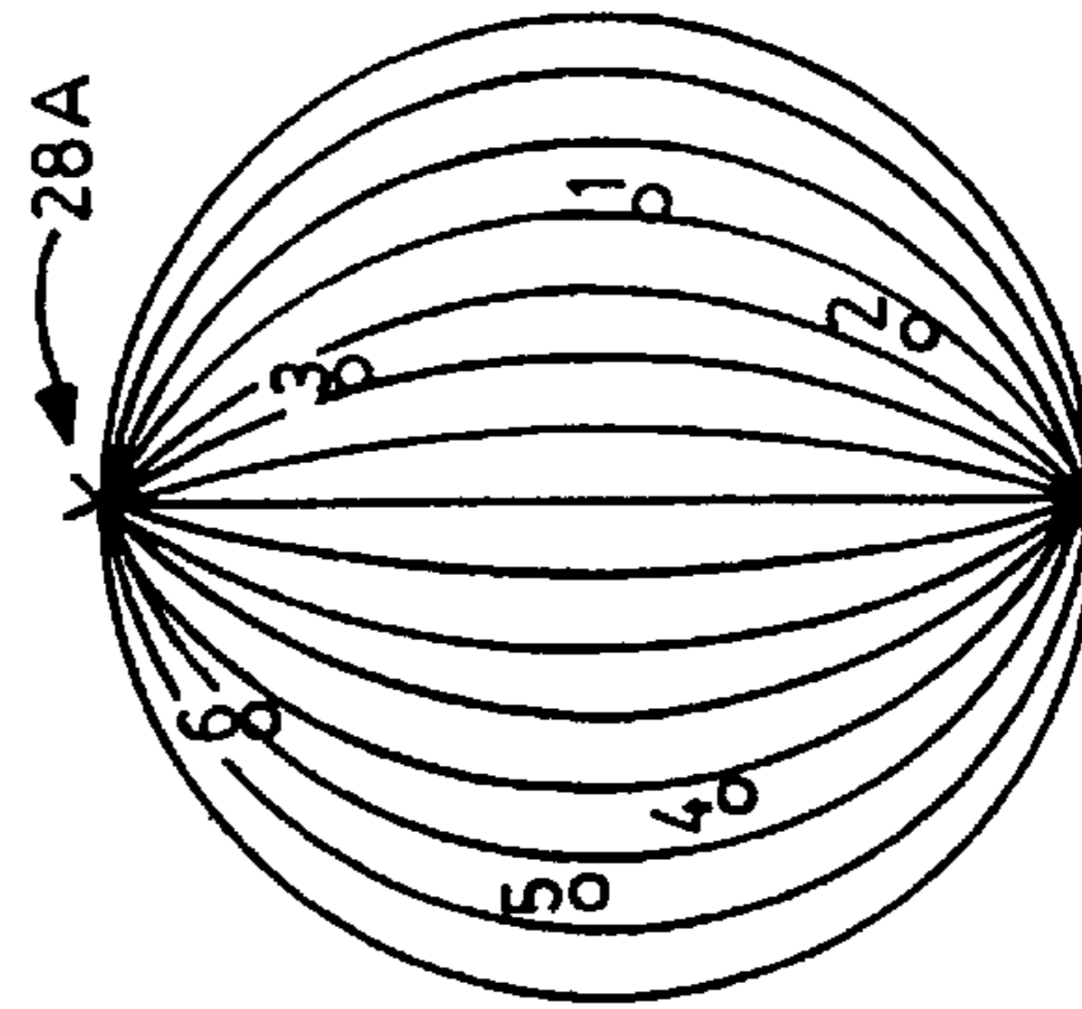
3. DETERMINE LONGITUDINAL CO-ORDINATES FOR SPATIAL POINTS 28 WITH RESPECT TO MATCHED POINT 28A
