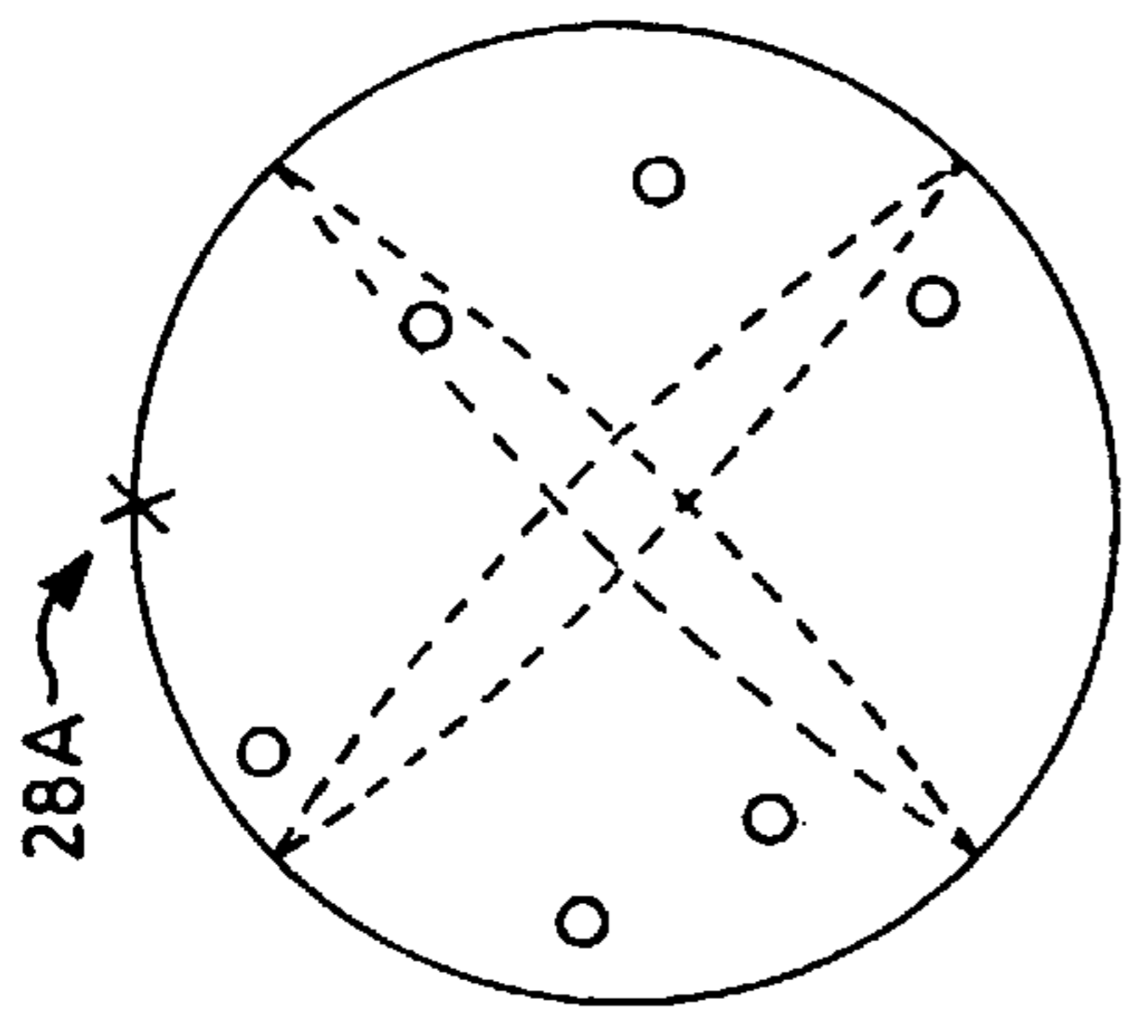
2. ROTATE SPHERE SO THAT POINT 28A IS LOCATED AT THE "NORTH POLE"
