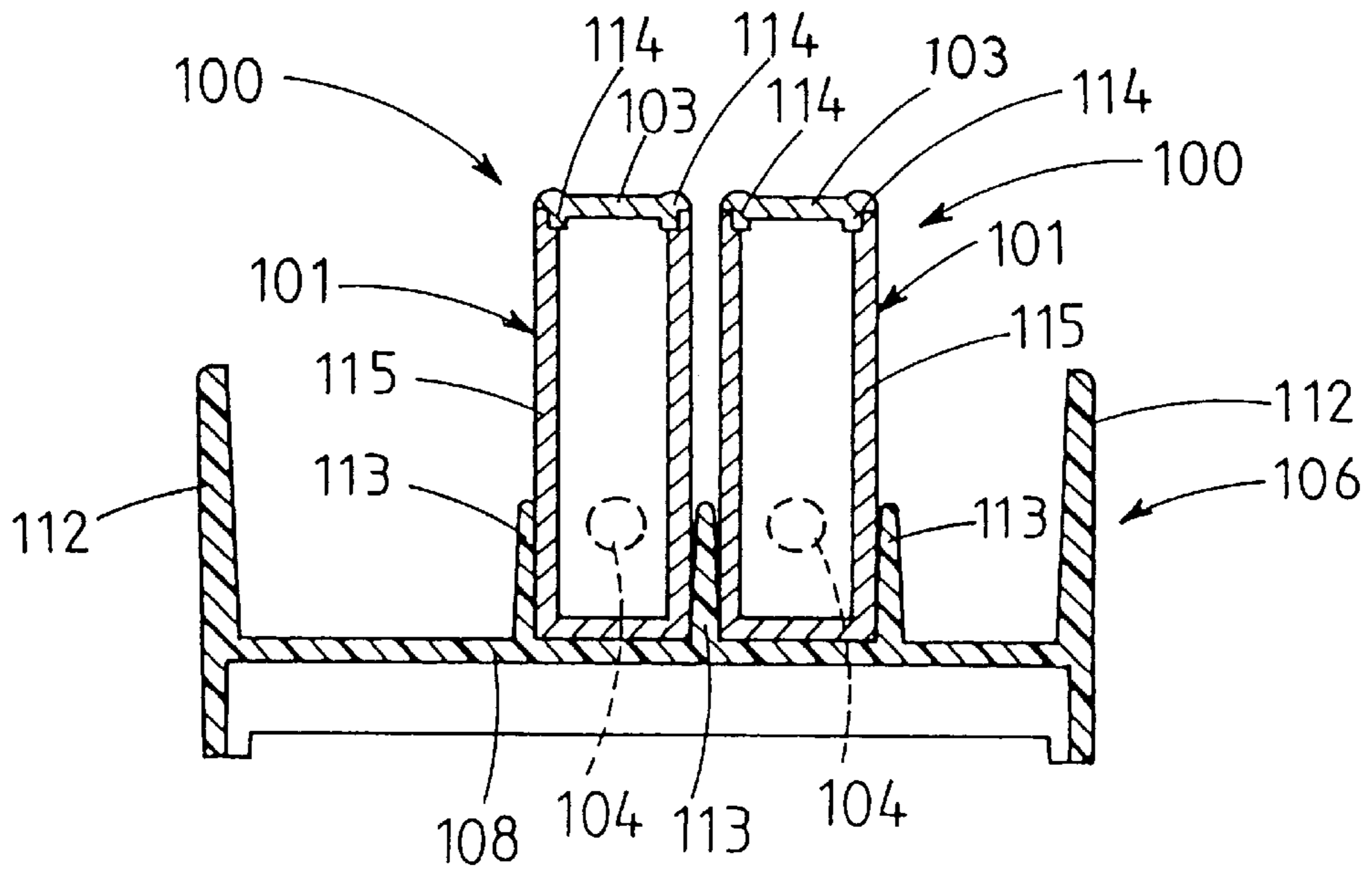
Fig.14 PRIOR ART
