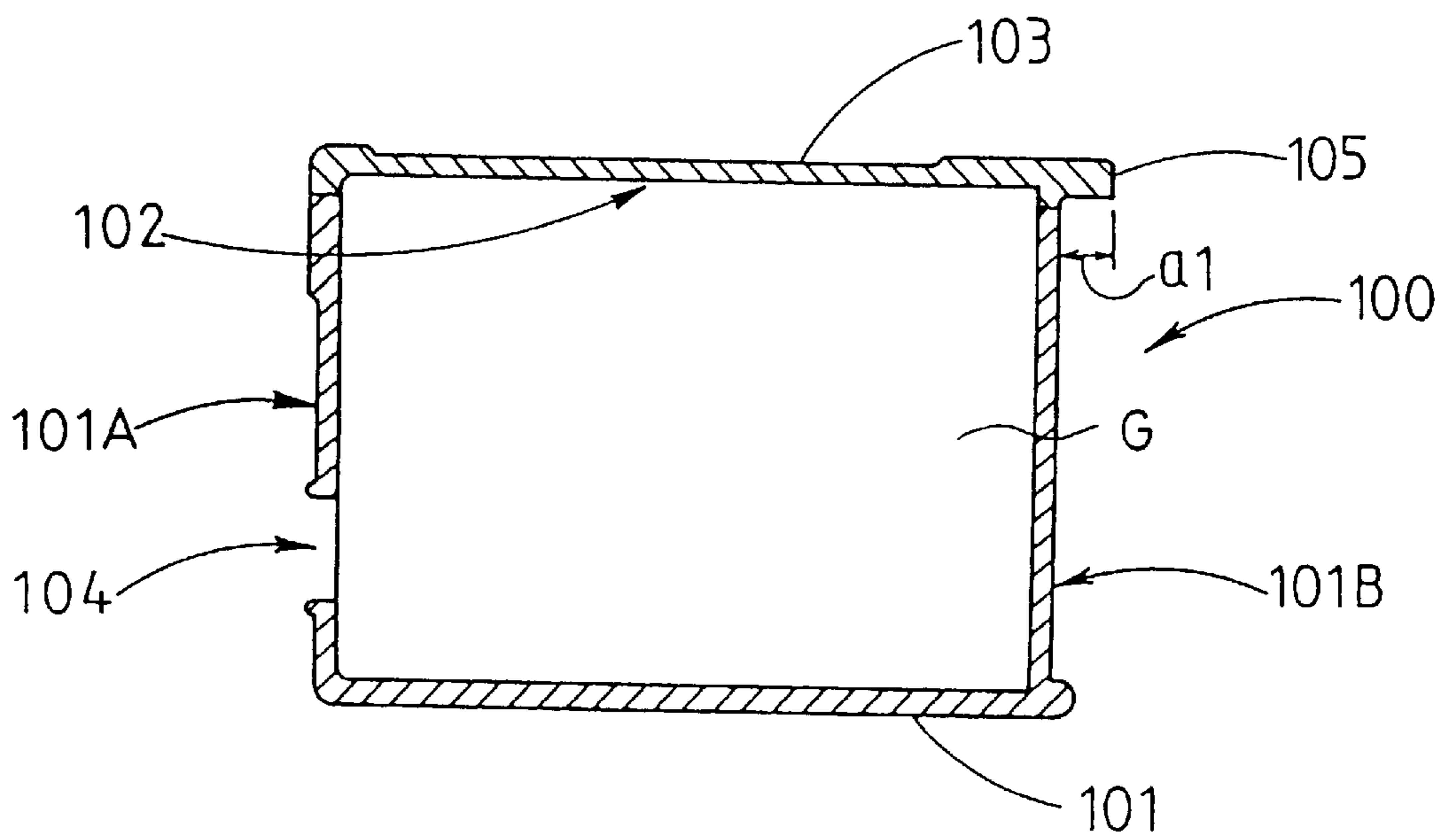
Fig.12 PRIOR ART
