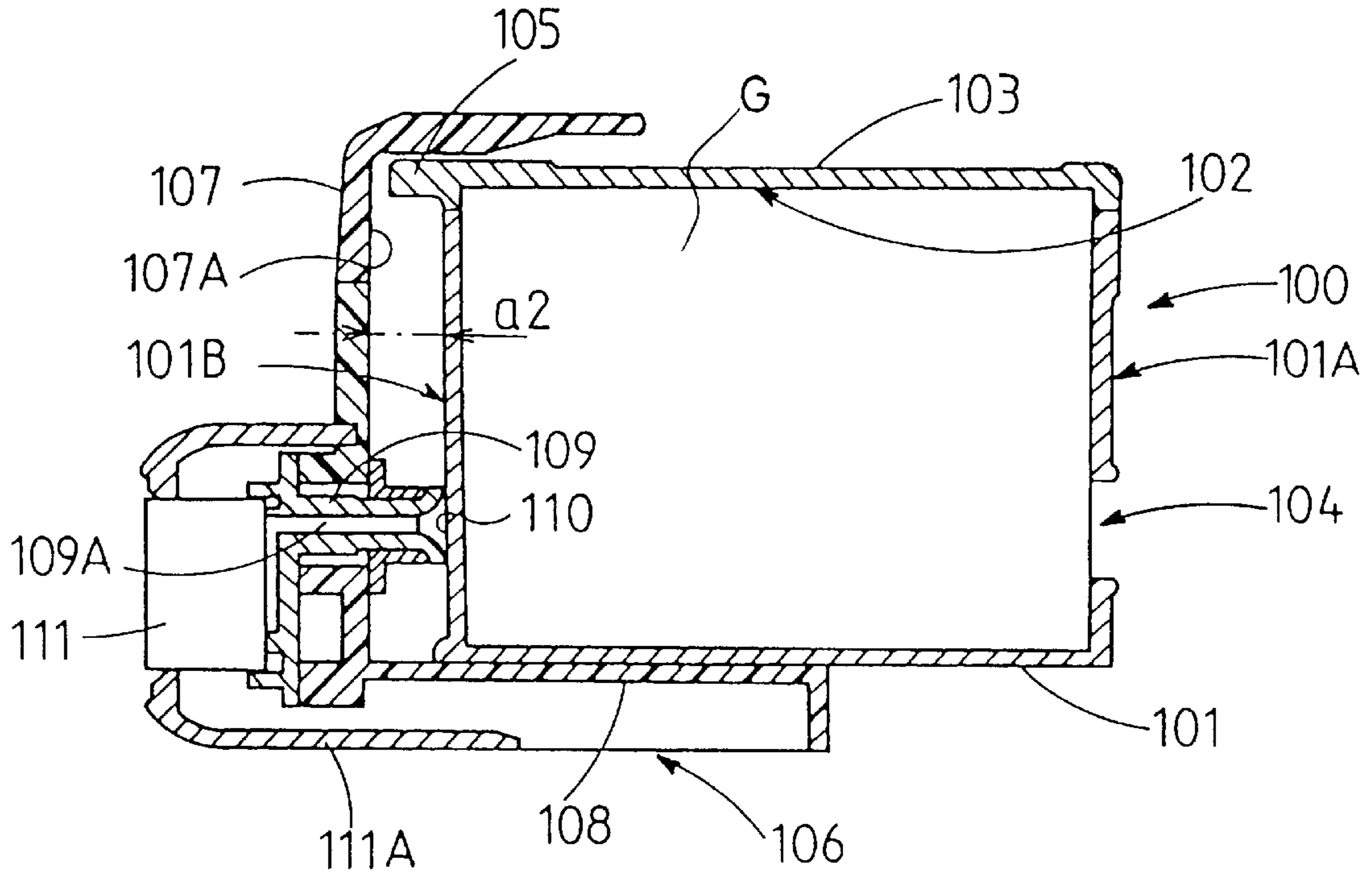
Fig.13 PRIOR ART
