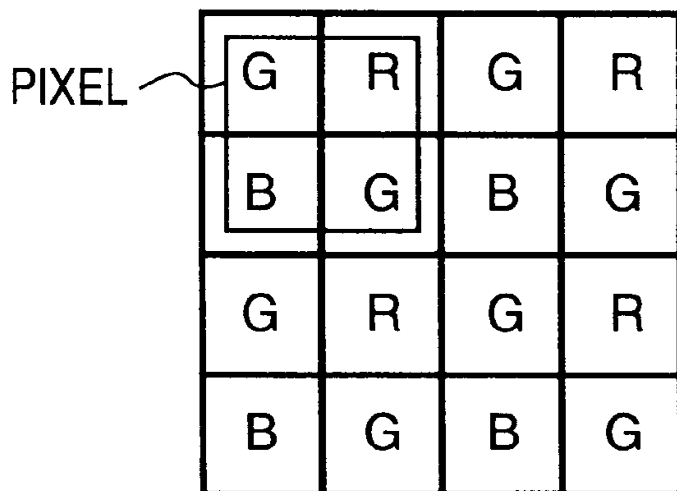
CHECKERBOARD LAYOUT
