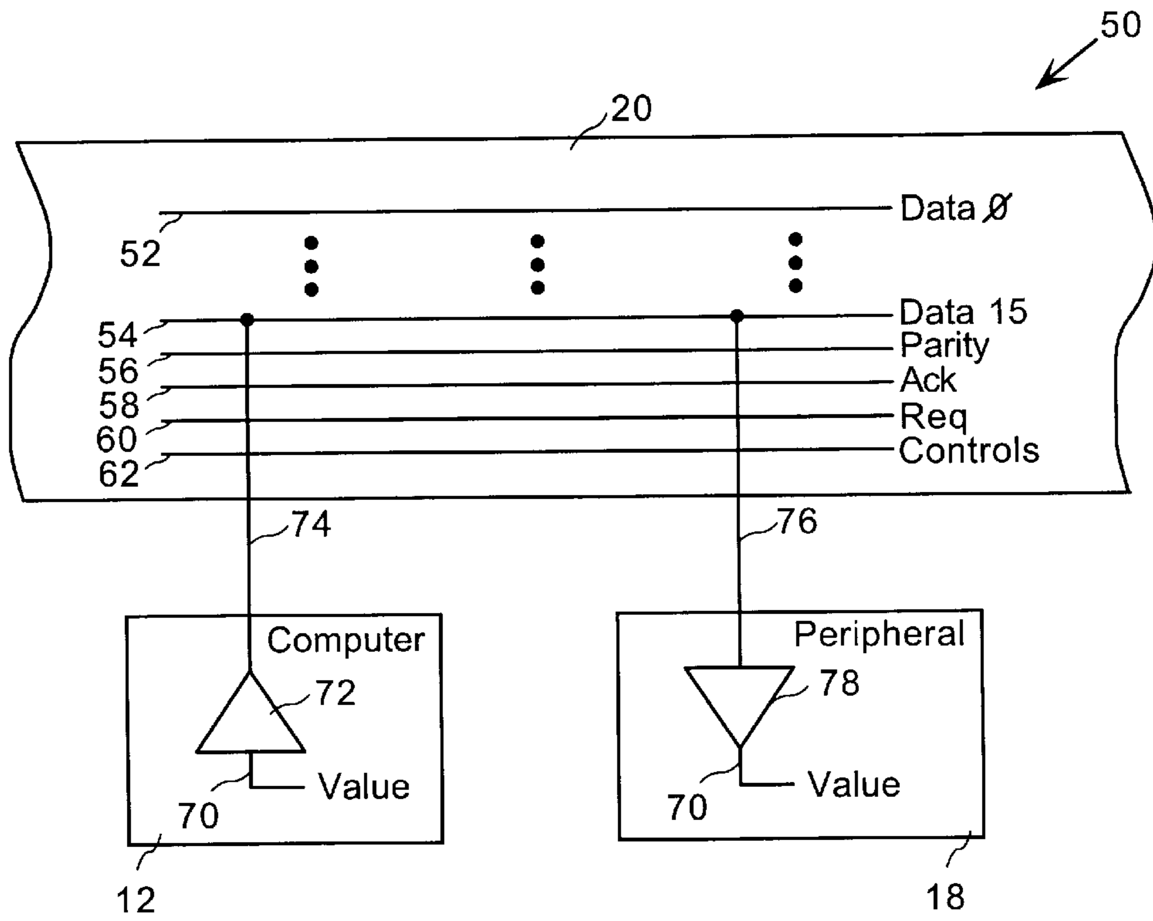
FIG. 2 (prior art)
