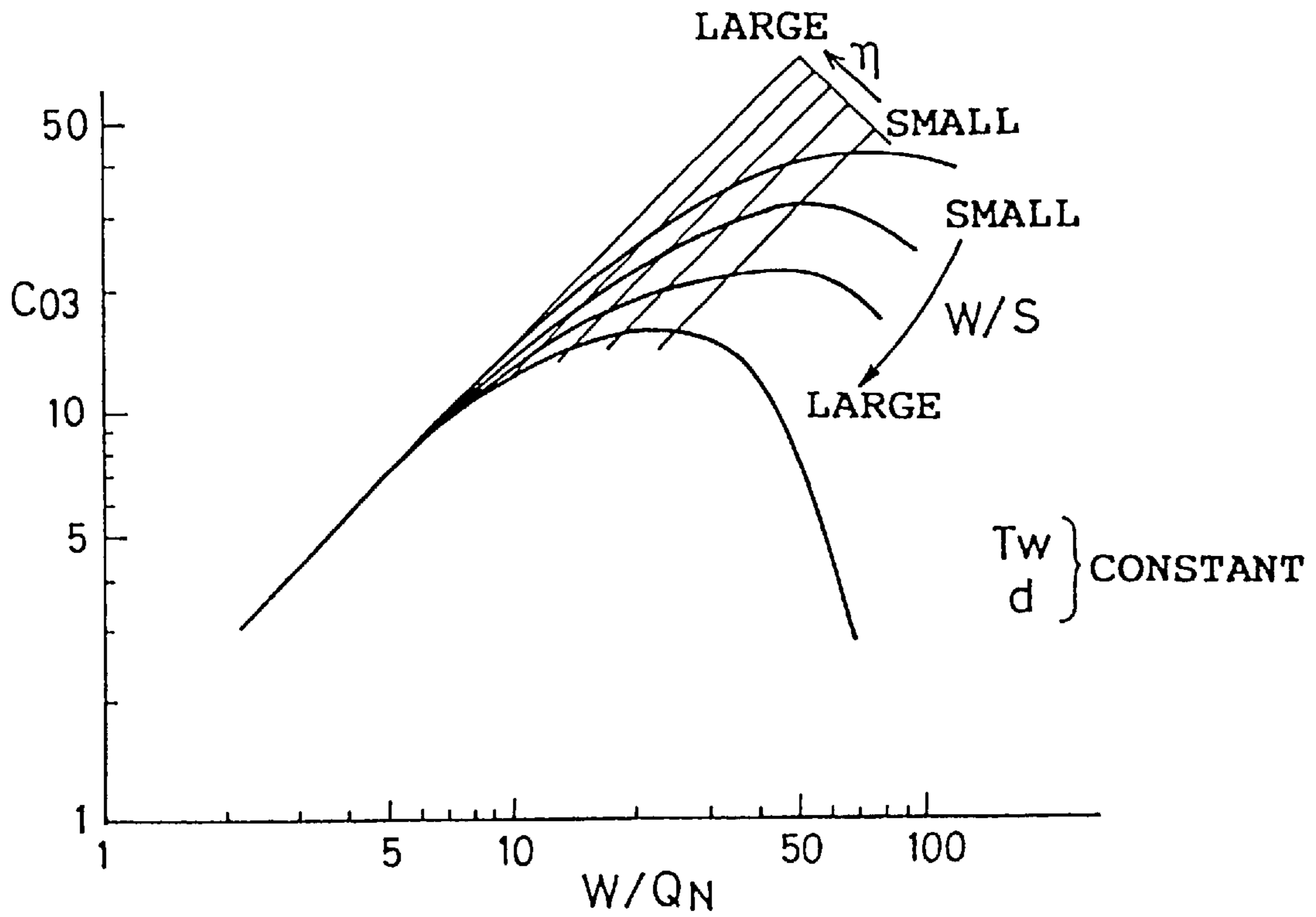
FIG. 4 (PRIOR ART)
