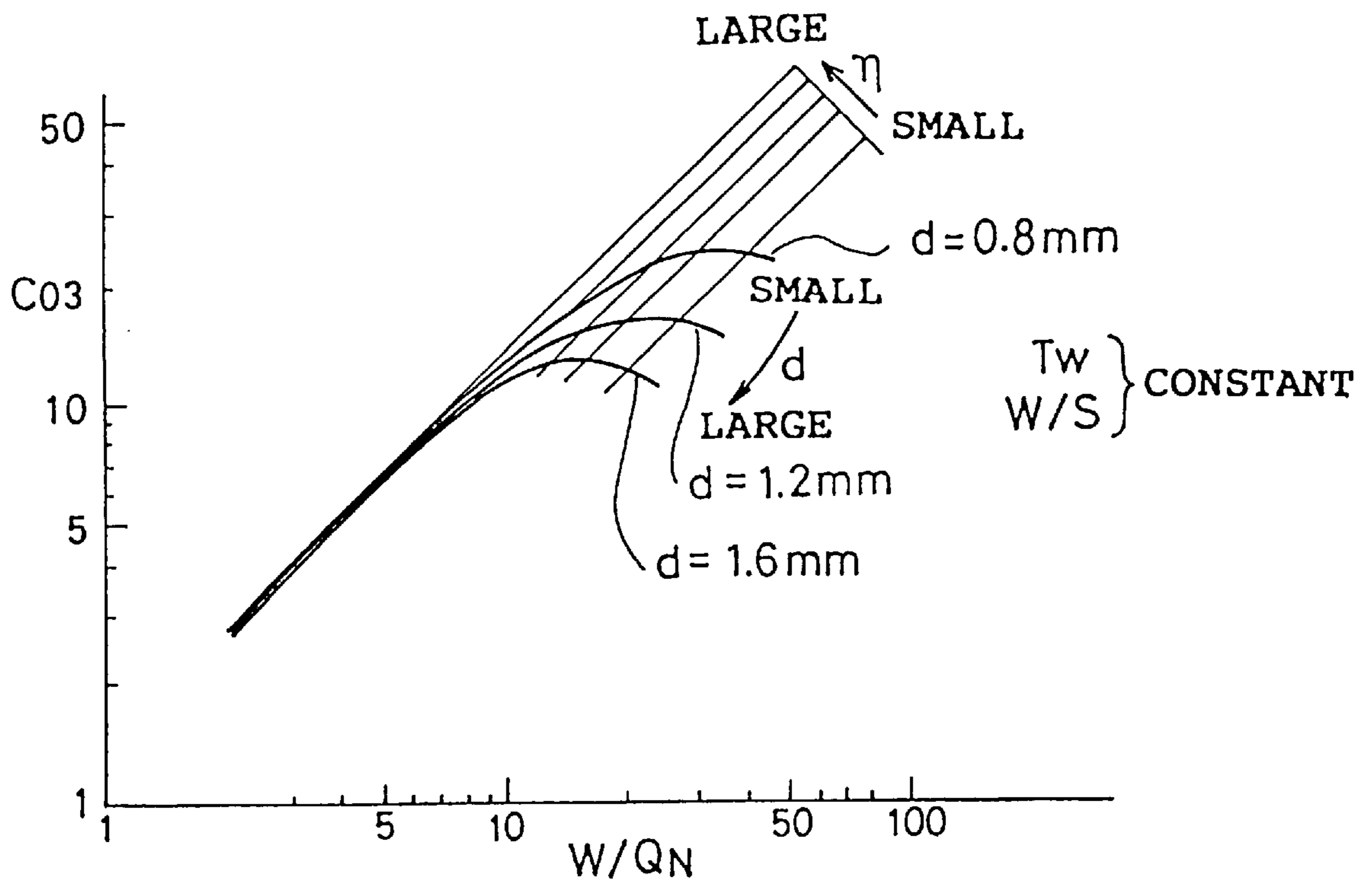
FIG. 5 (PRIOR ART)
