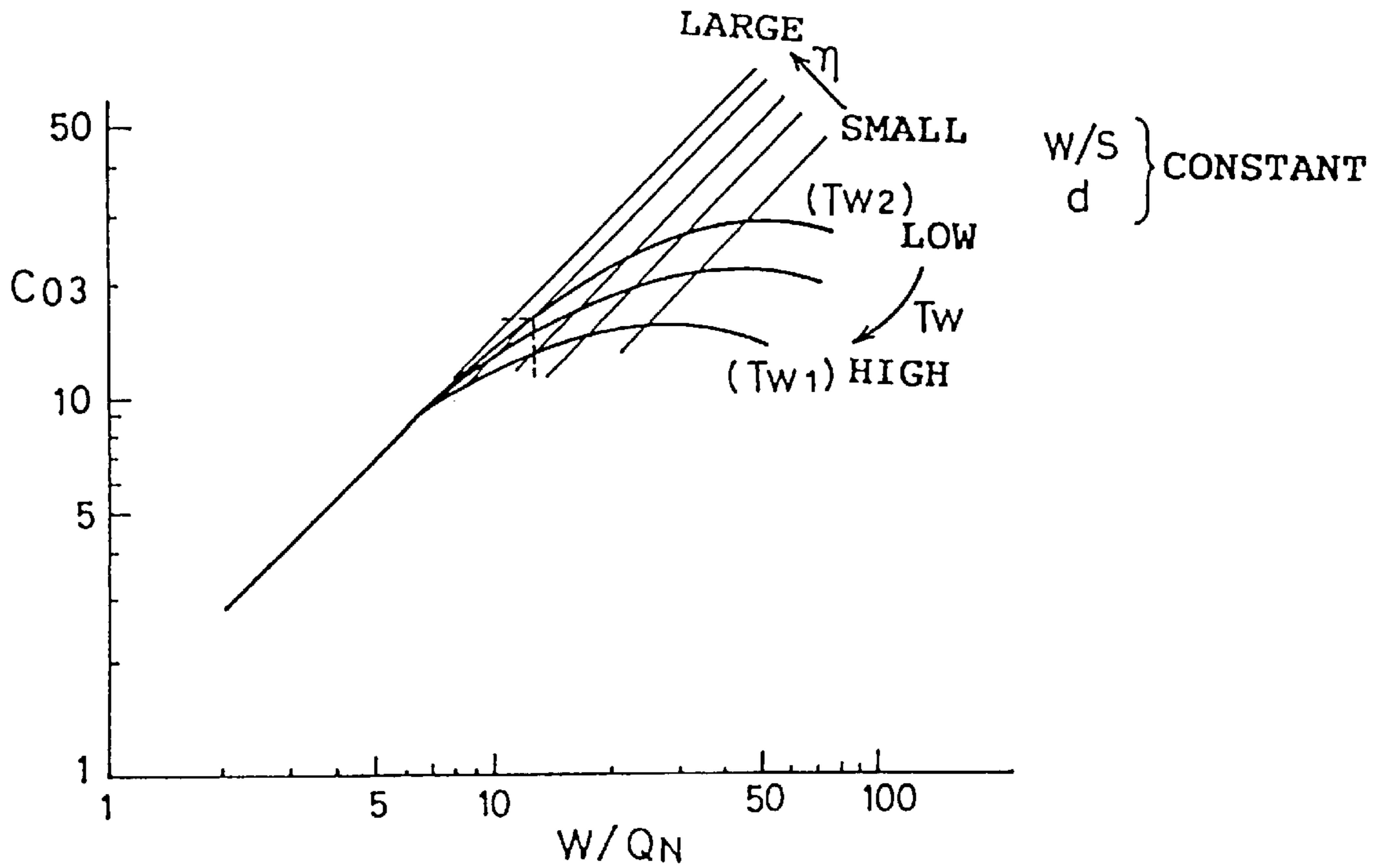
FIG. 3 (PRIOR ART)
