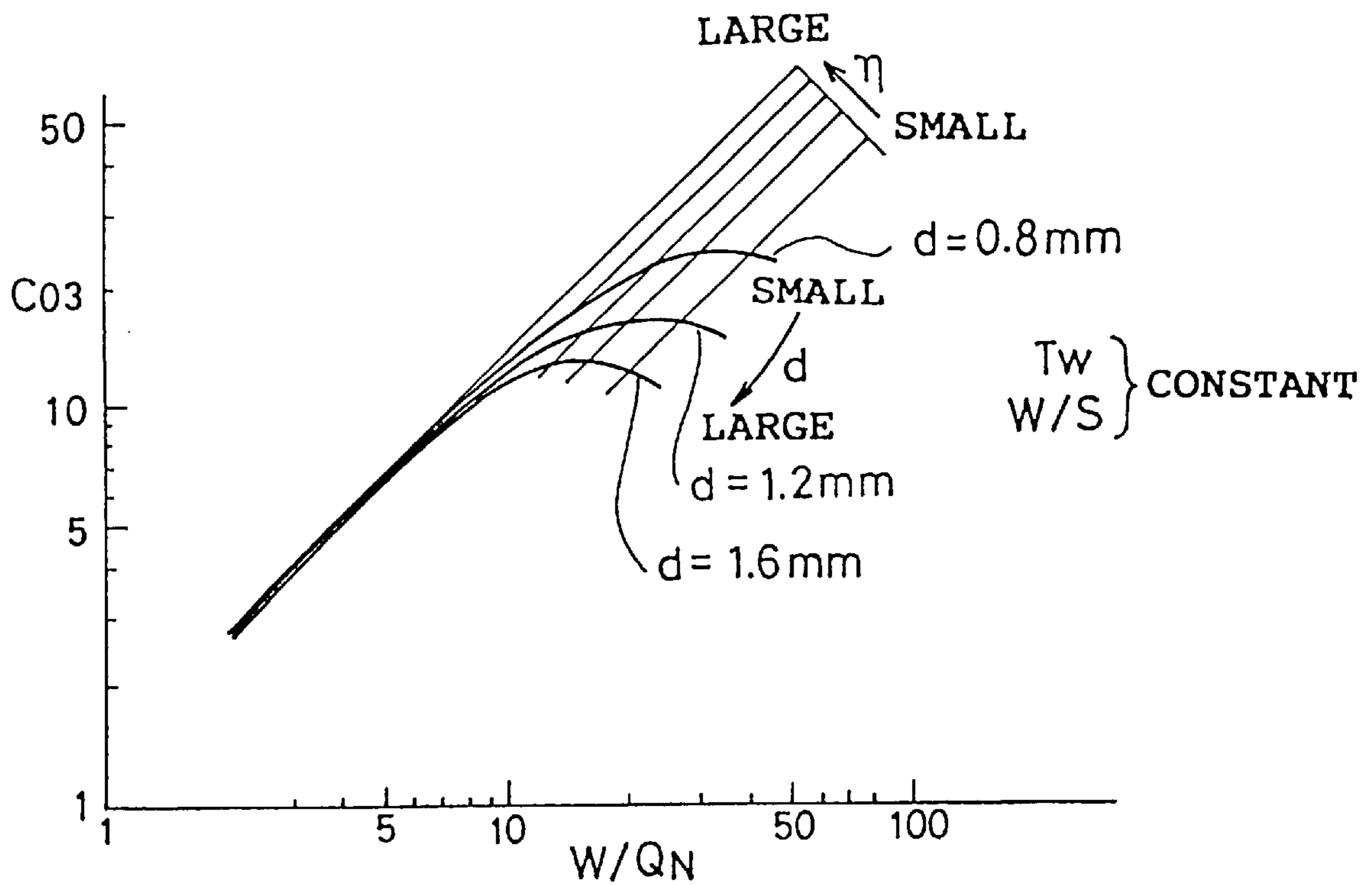
FIG. 5 (PRIOR ART)
