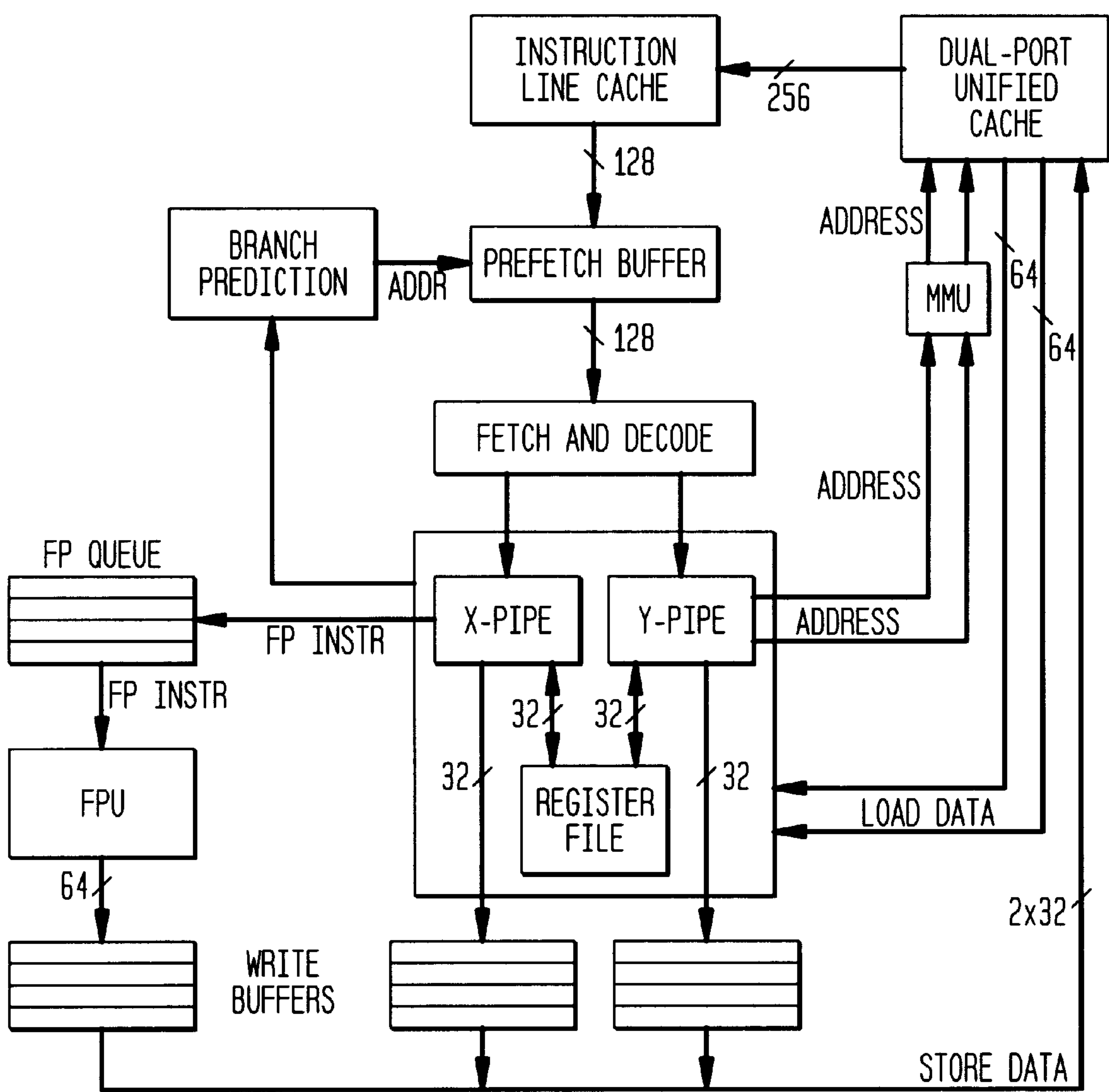
FIG. 2 (PRIOR ART)
