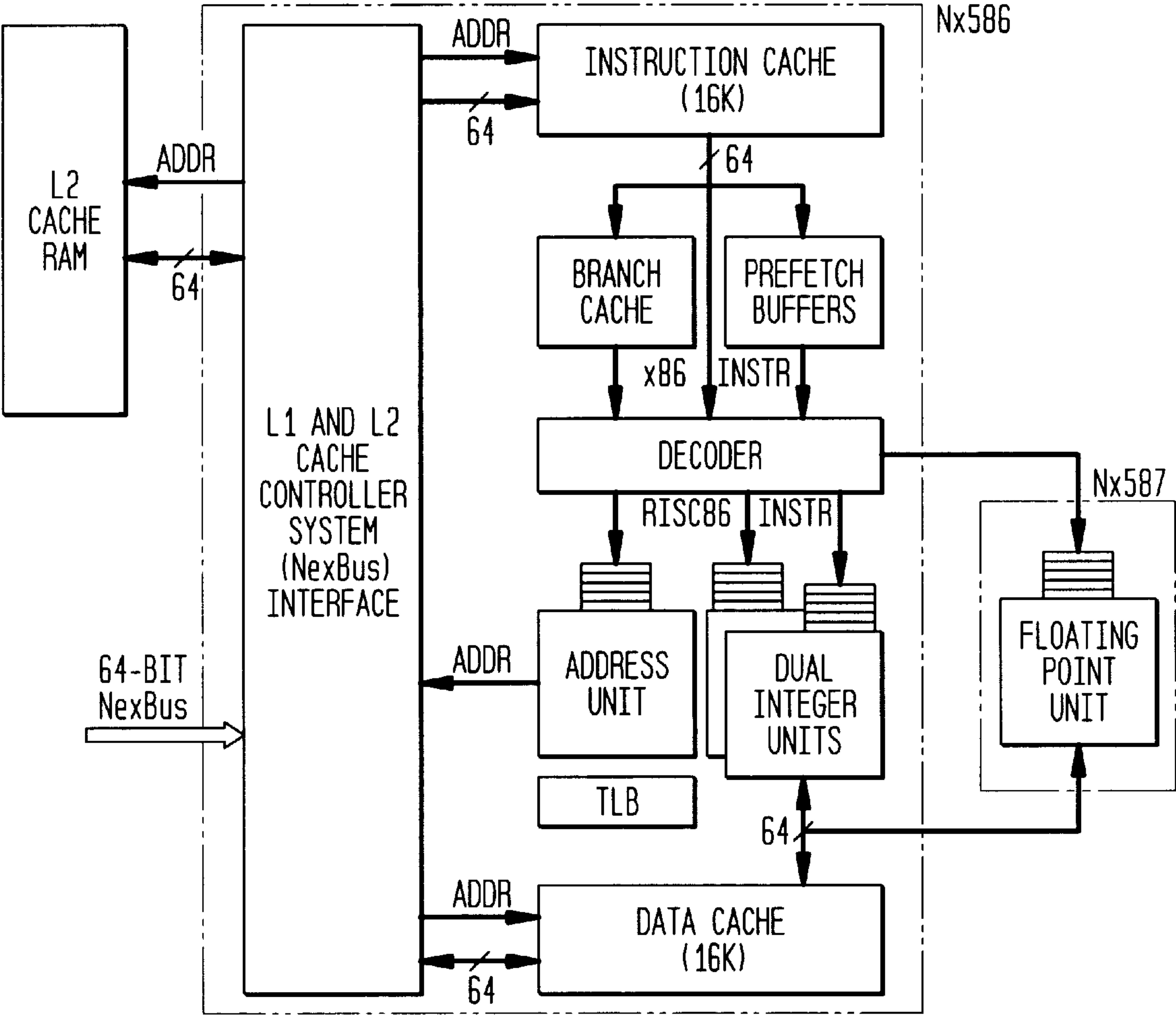
FIG. 3 (PRIOR ART)
