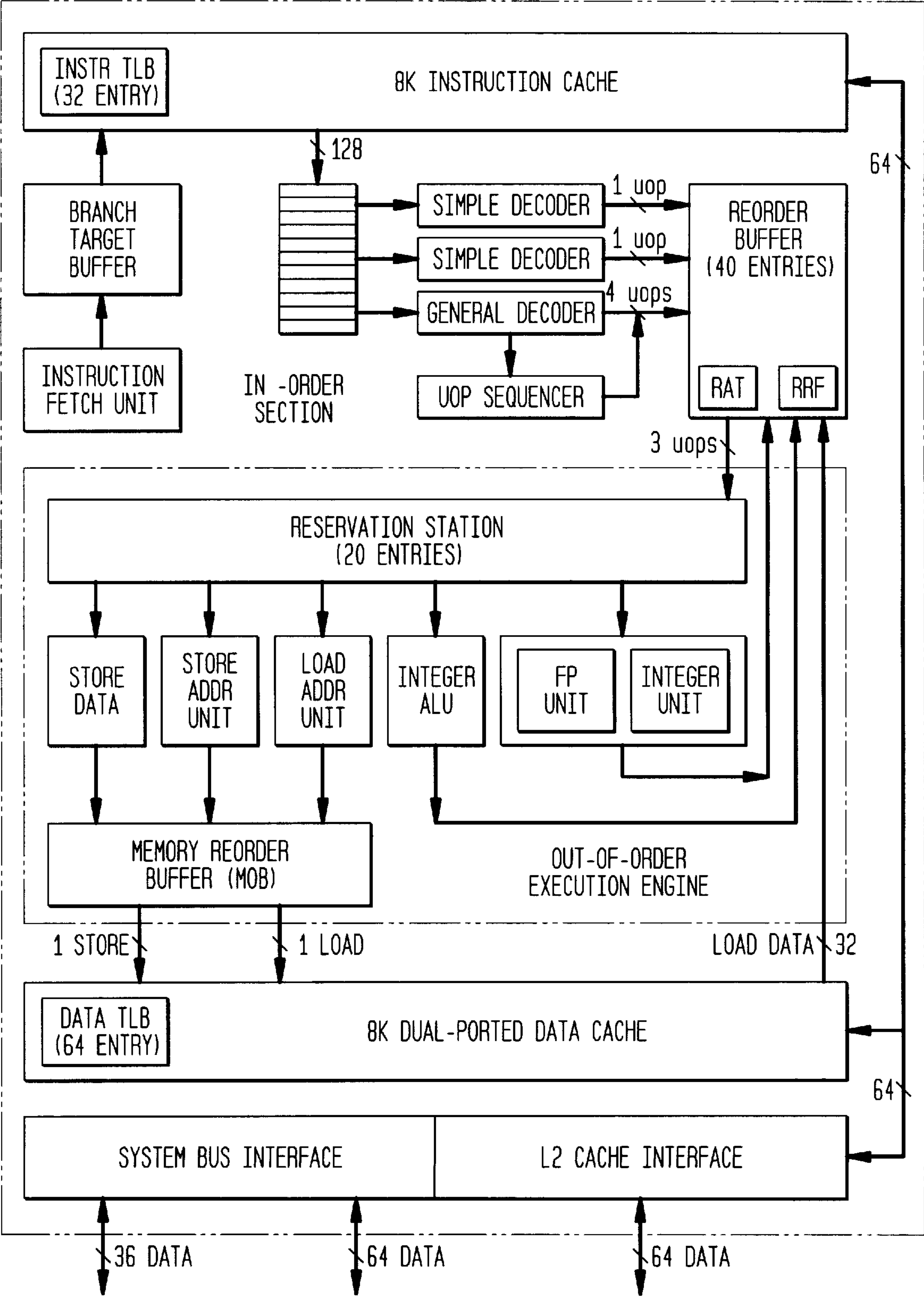
FIG. 6 (PRIOR ART)
