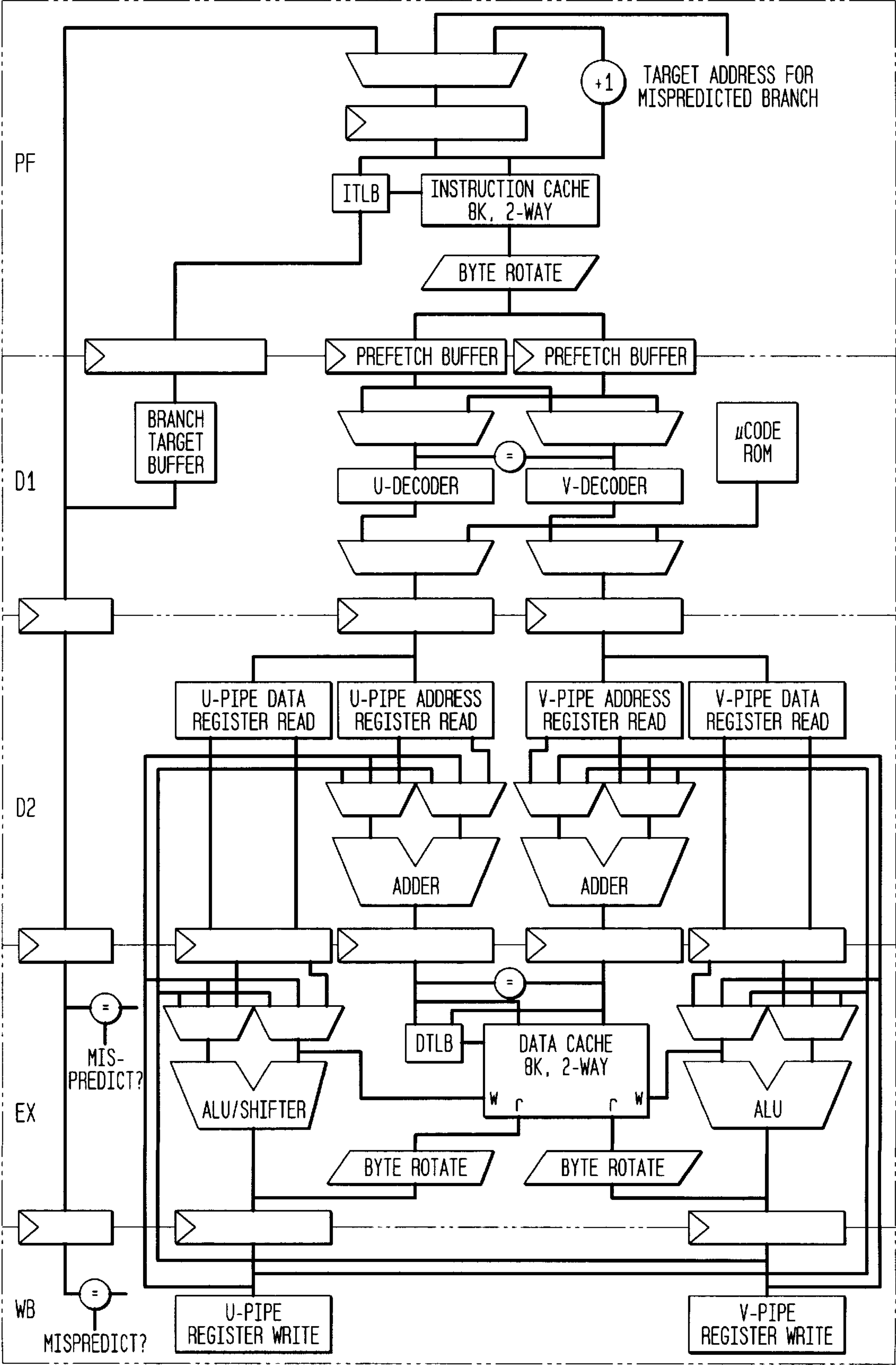
FIG. 1 (PRIOR ART)
