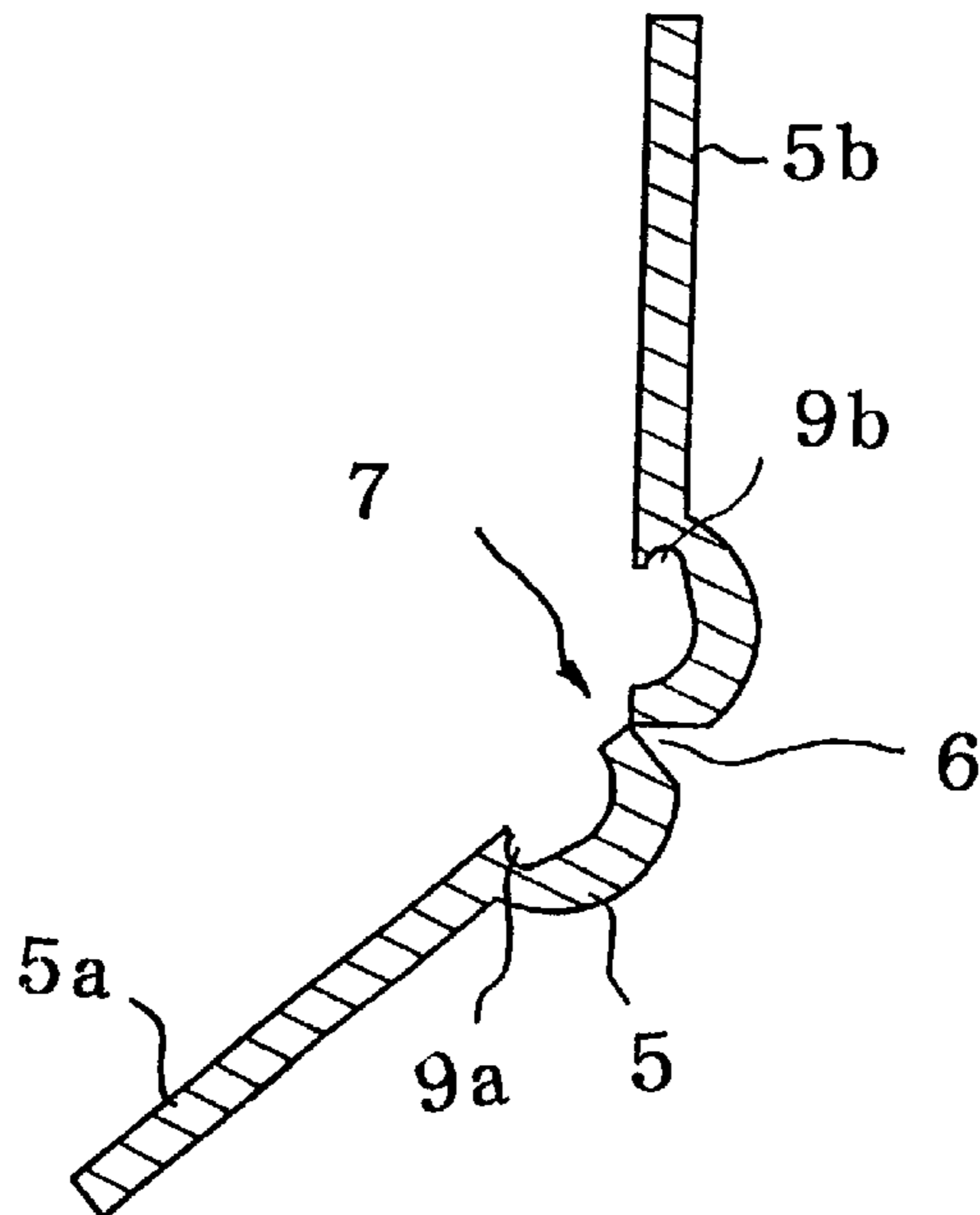
FIG. 27 Prior Art
