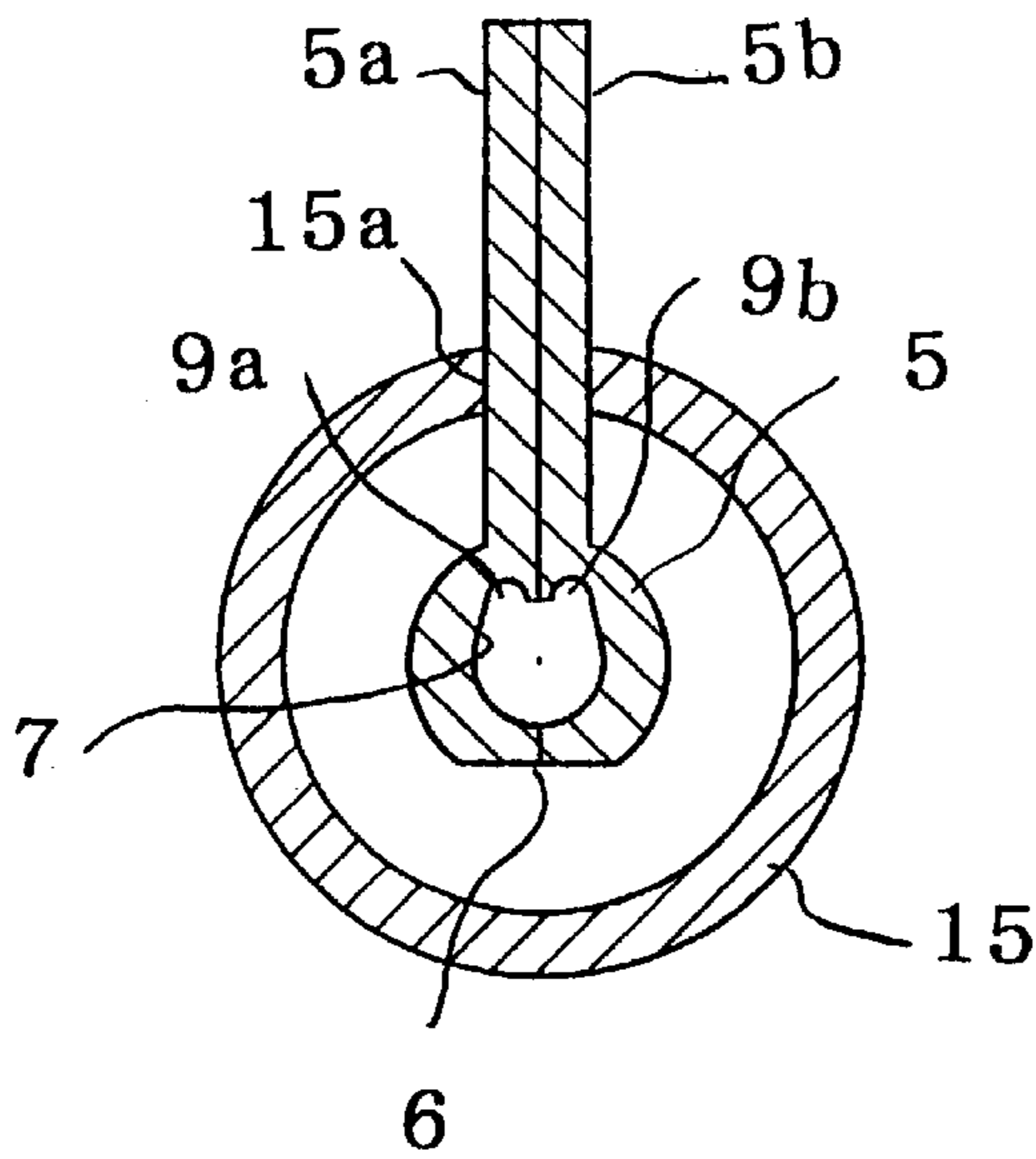
FIG. 29 Prior Art
