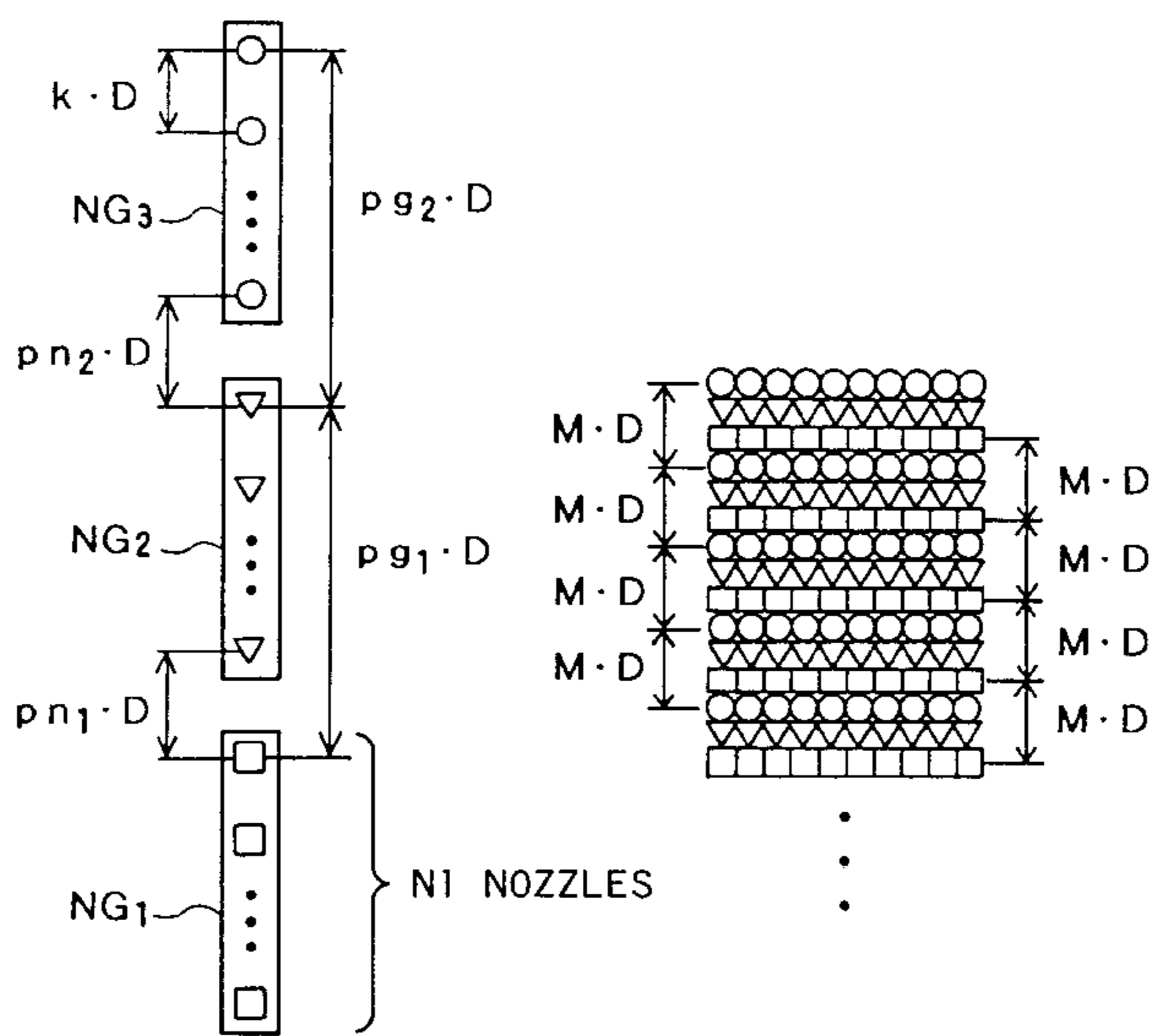
FIRST PRINTING SCHEME USING MULTIPLE NOZZLE GROUPS (EACH NOZZLE GROUP RECORDS DIFFERENT RASTER LINES FROM THE OTHERS)
