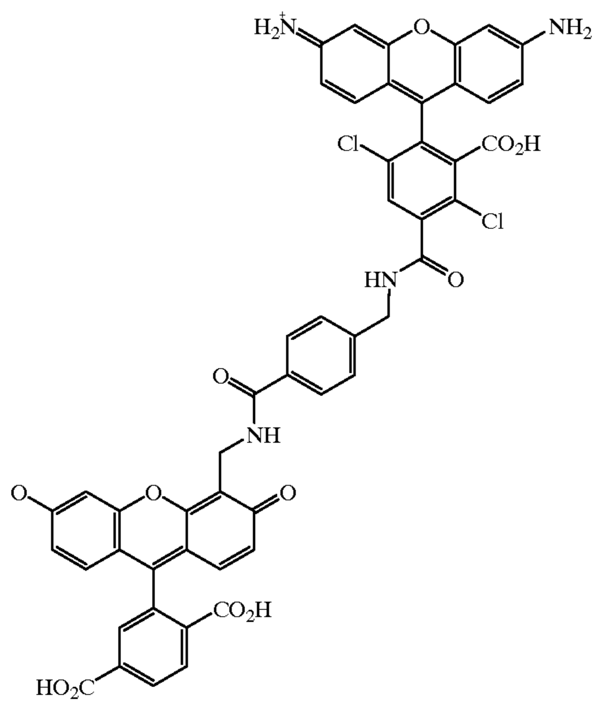
6-CFB-DR110-2
