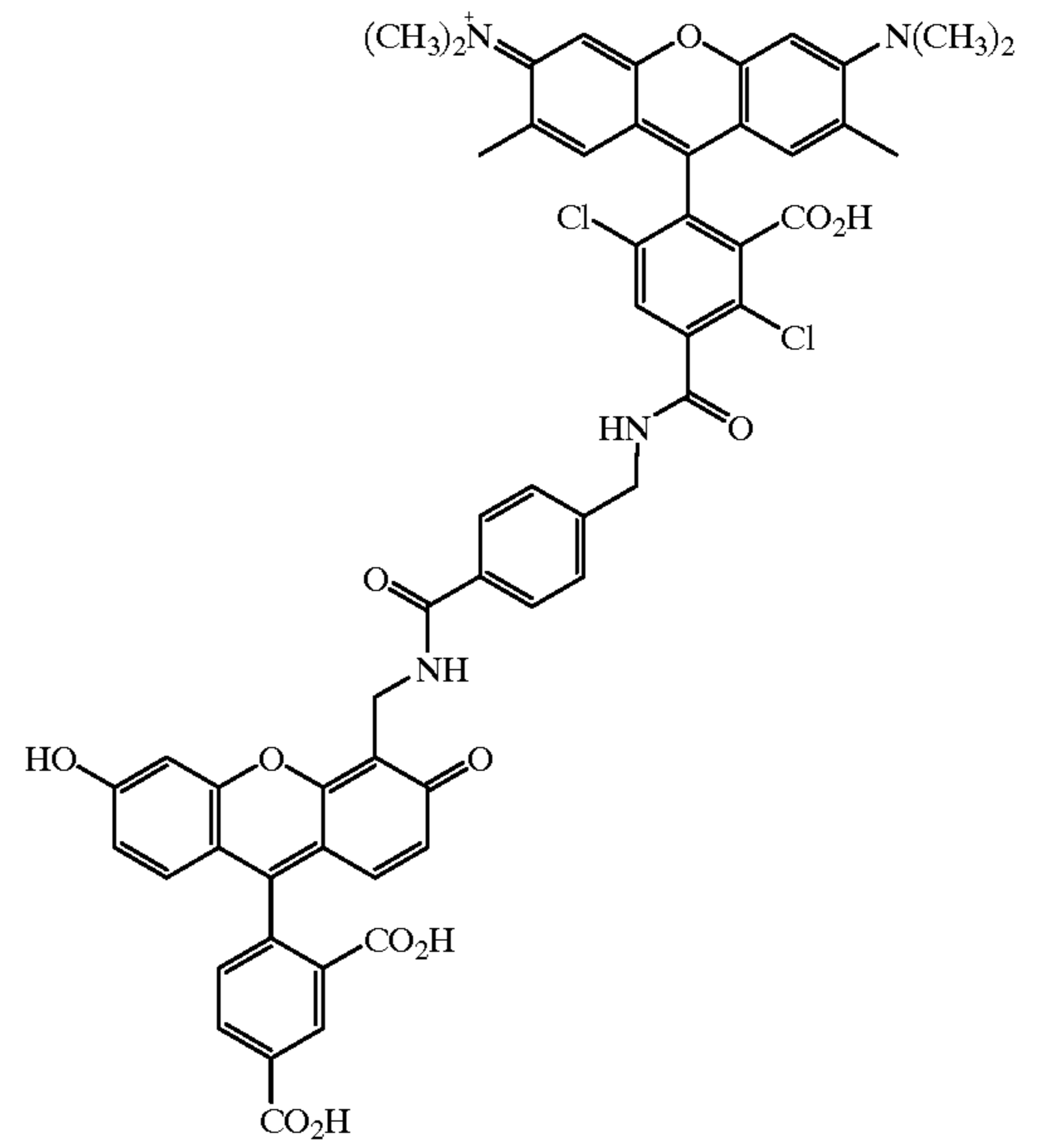
5-CFB-DTMR-2
