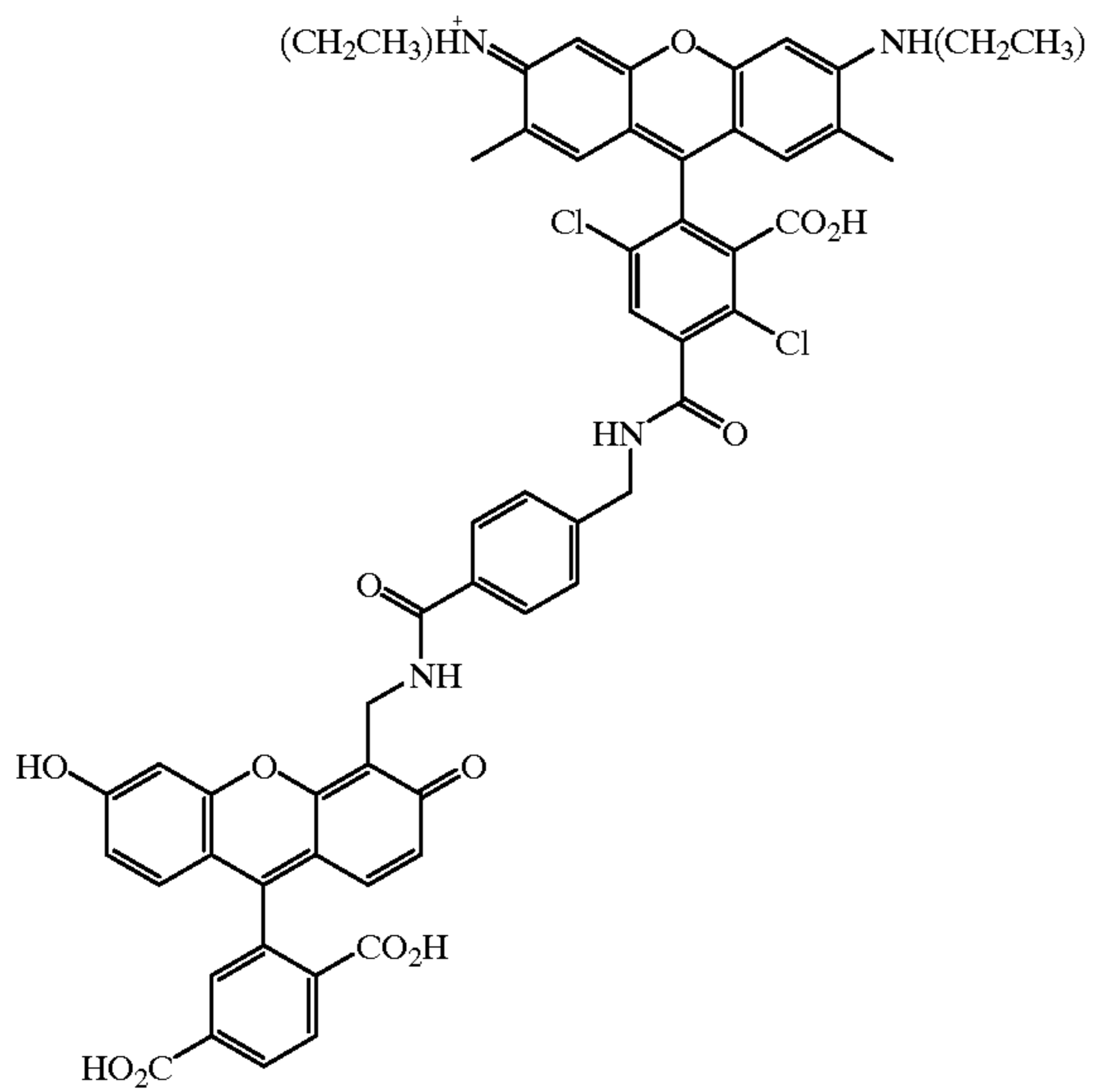
6-CFB-DR6G-2
