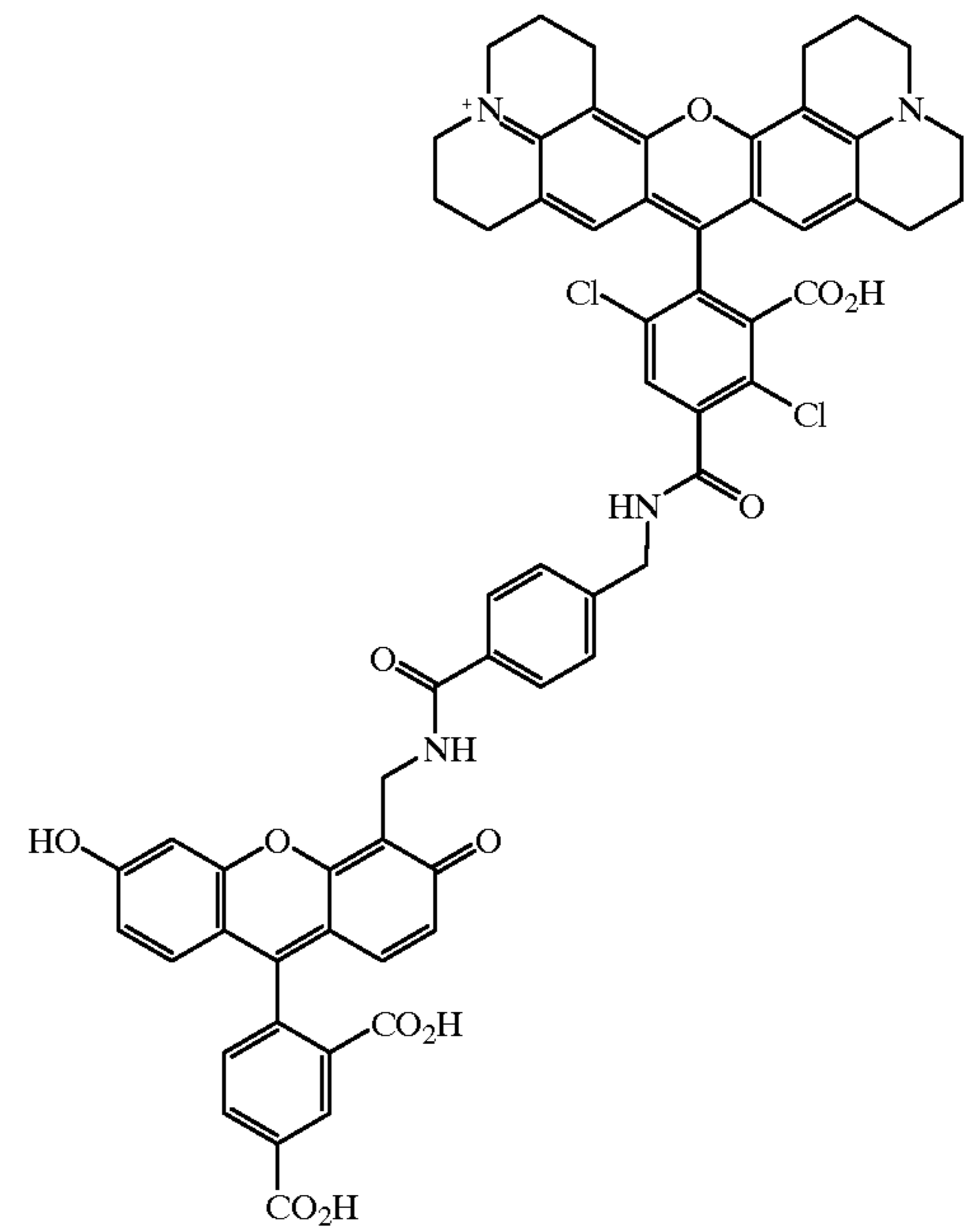
5-CFB-DROX-2
