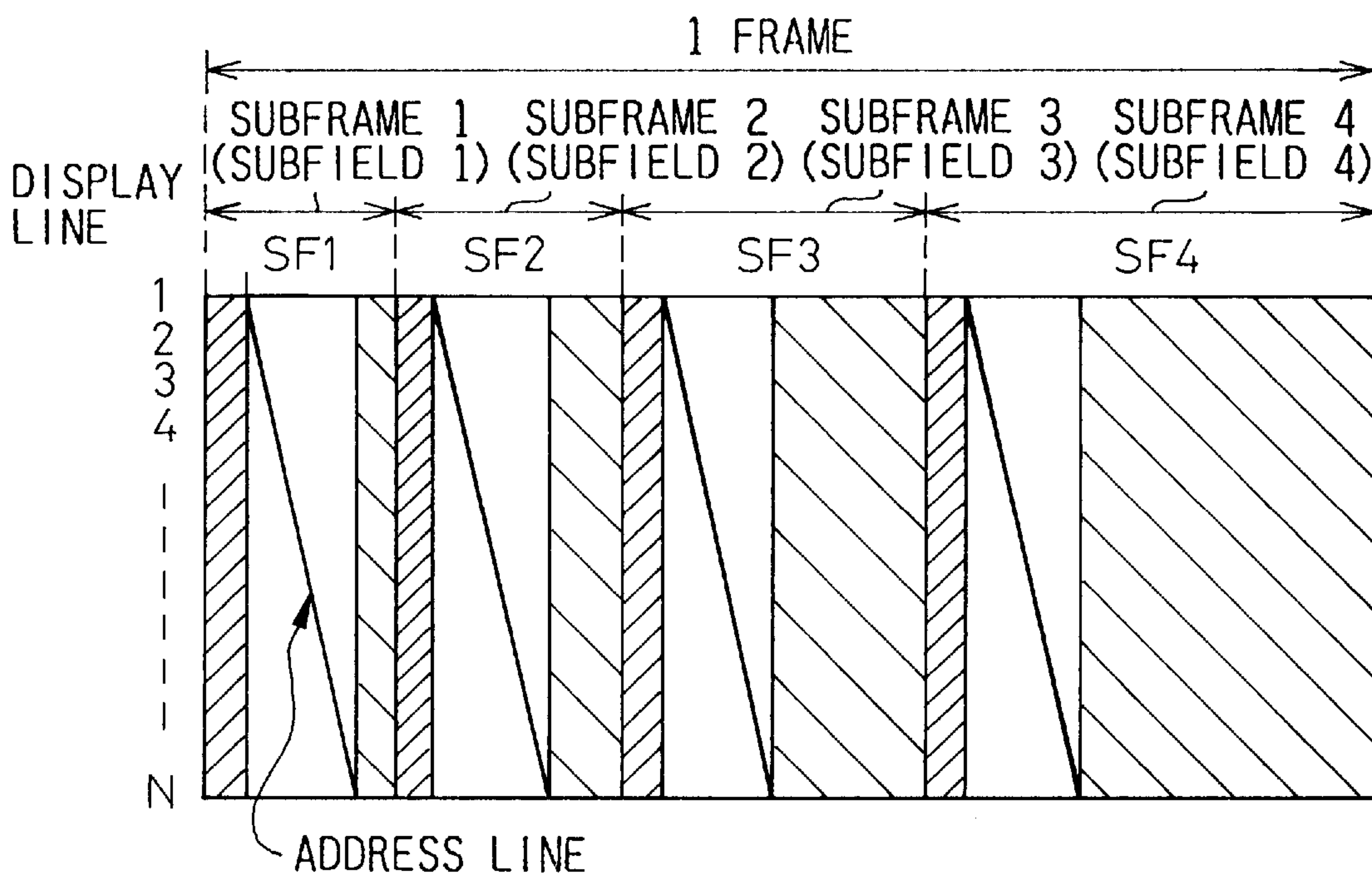
Fig.6 (PRIOR ART)
