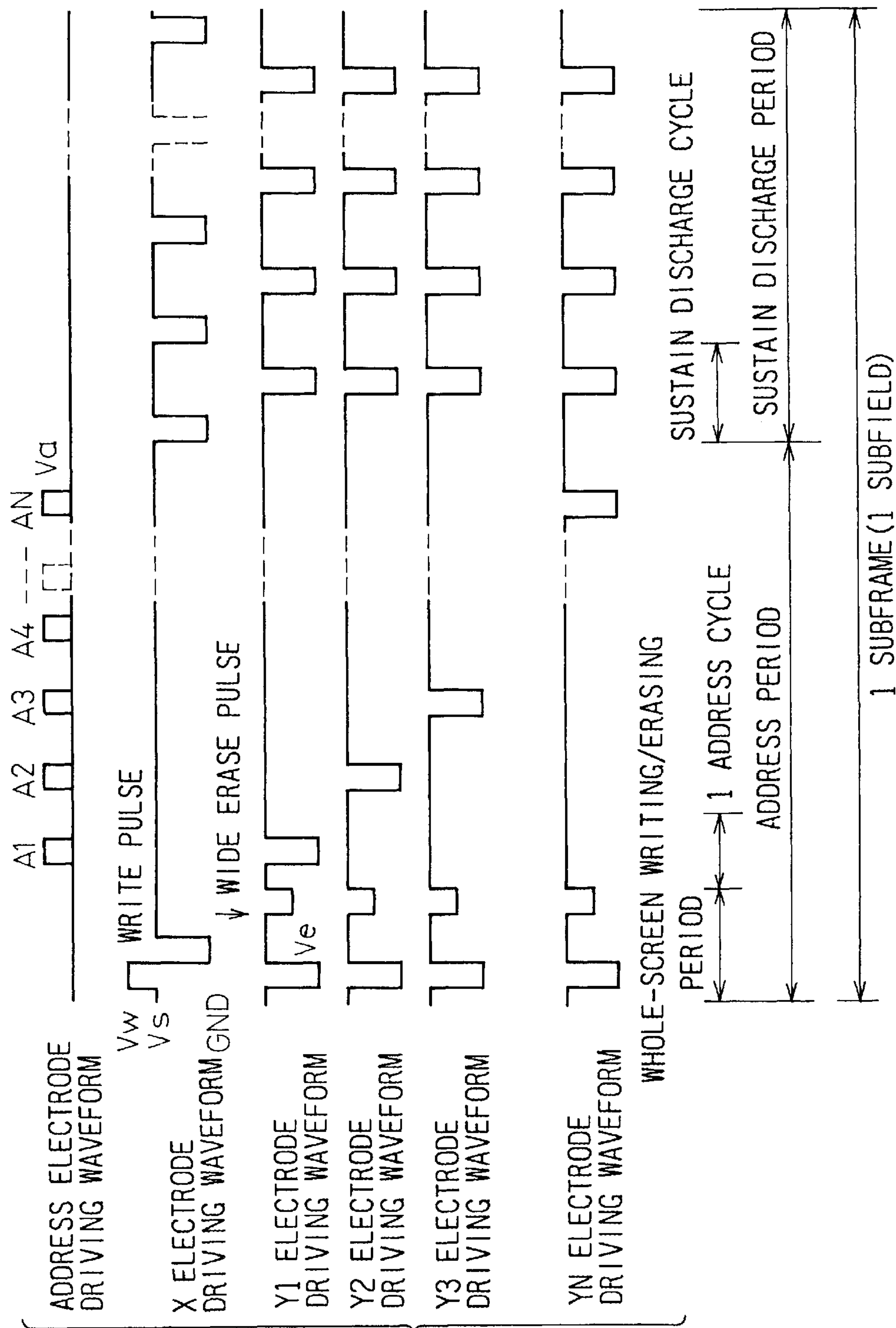
Fig.4 (PRIOR ART)
