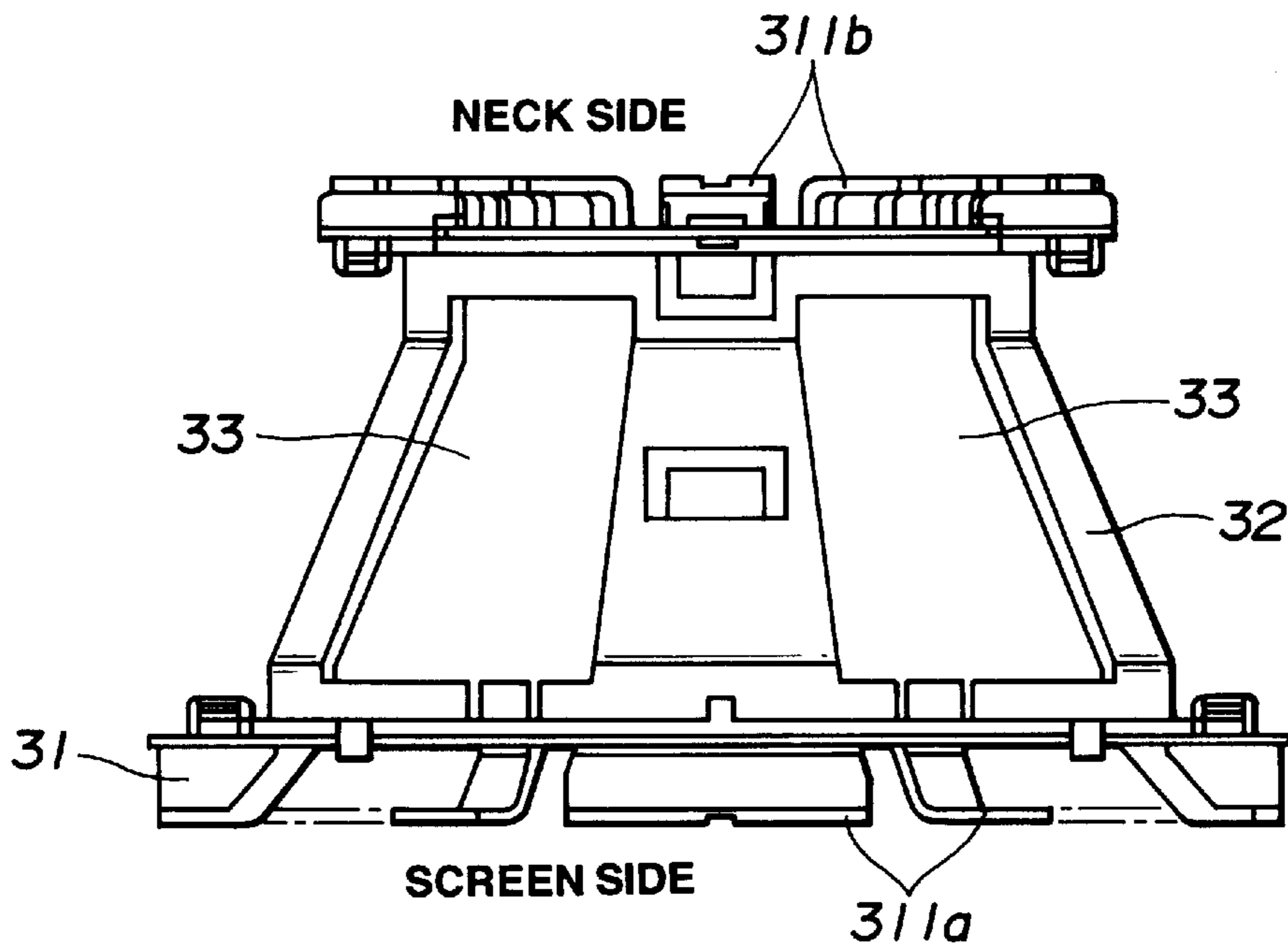
FIG.14 (RELATED ART)
