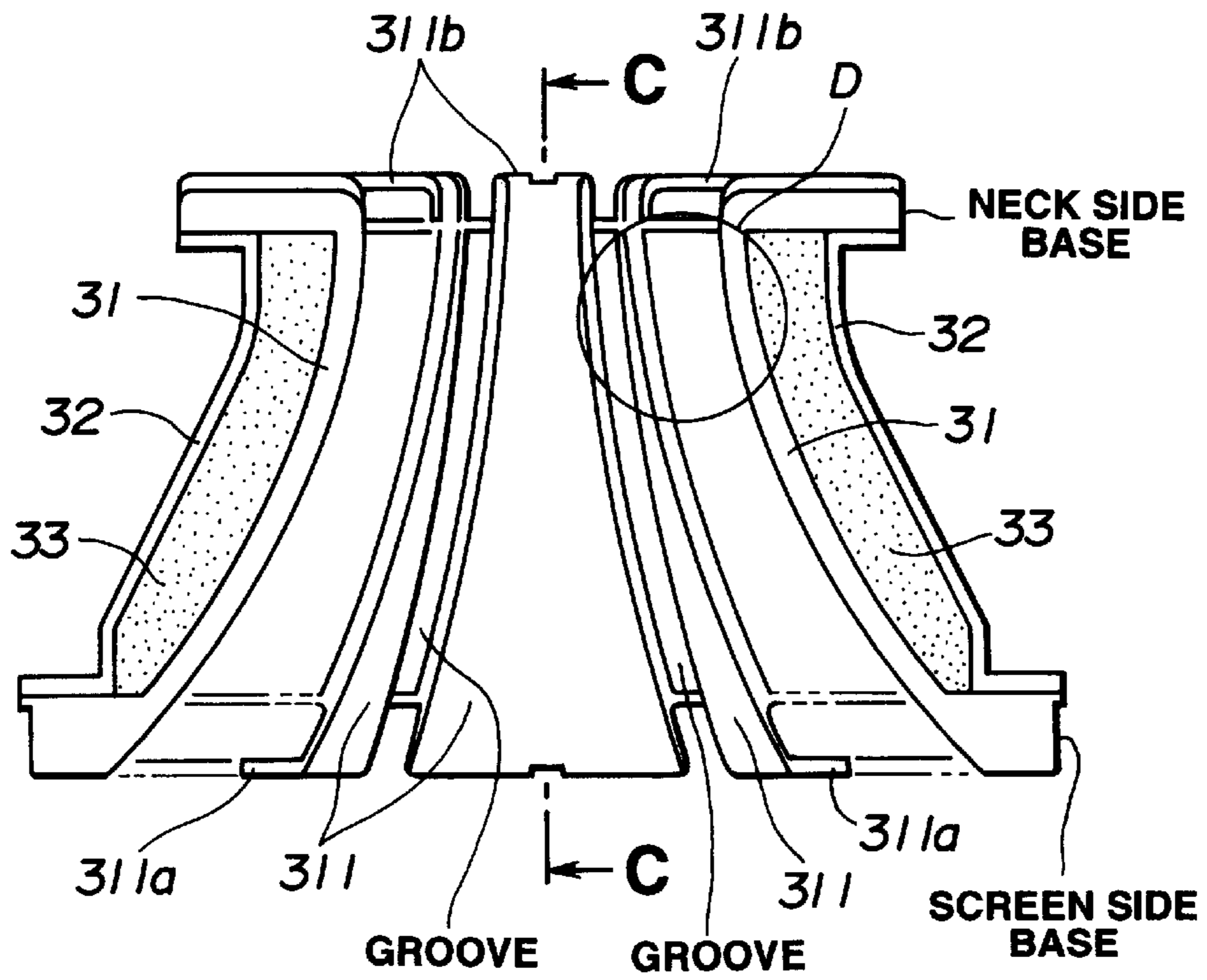
FIG.16 (RELATED ART)
