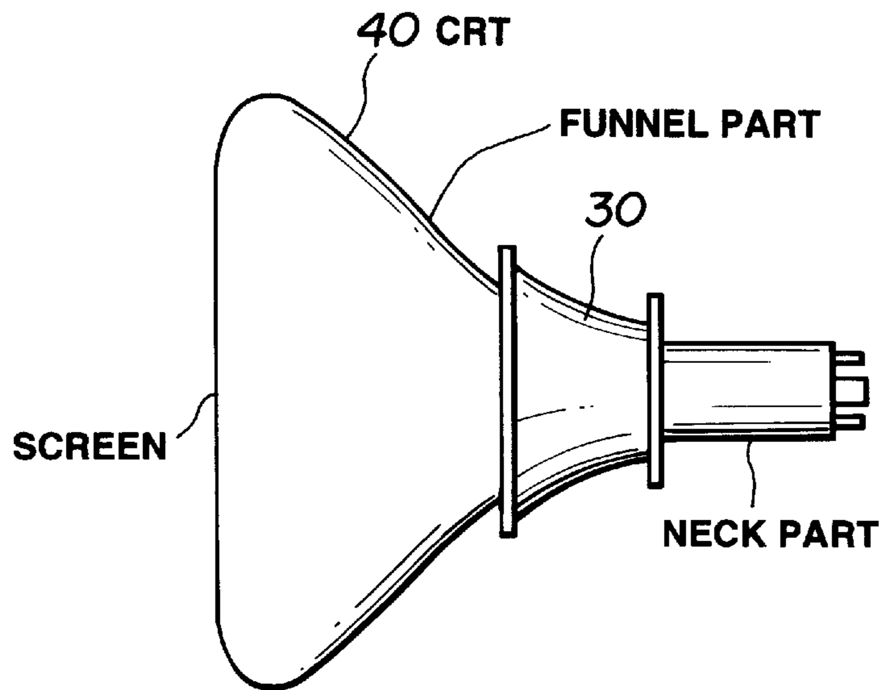
FIG.13 (RELATED ART)
