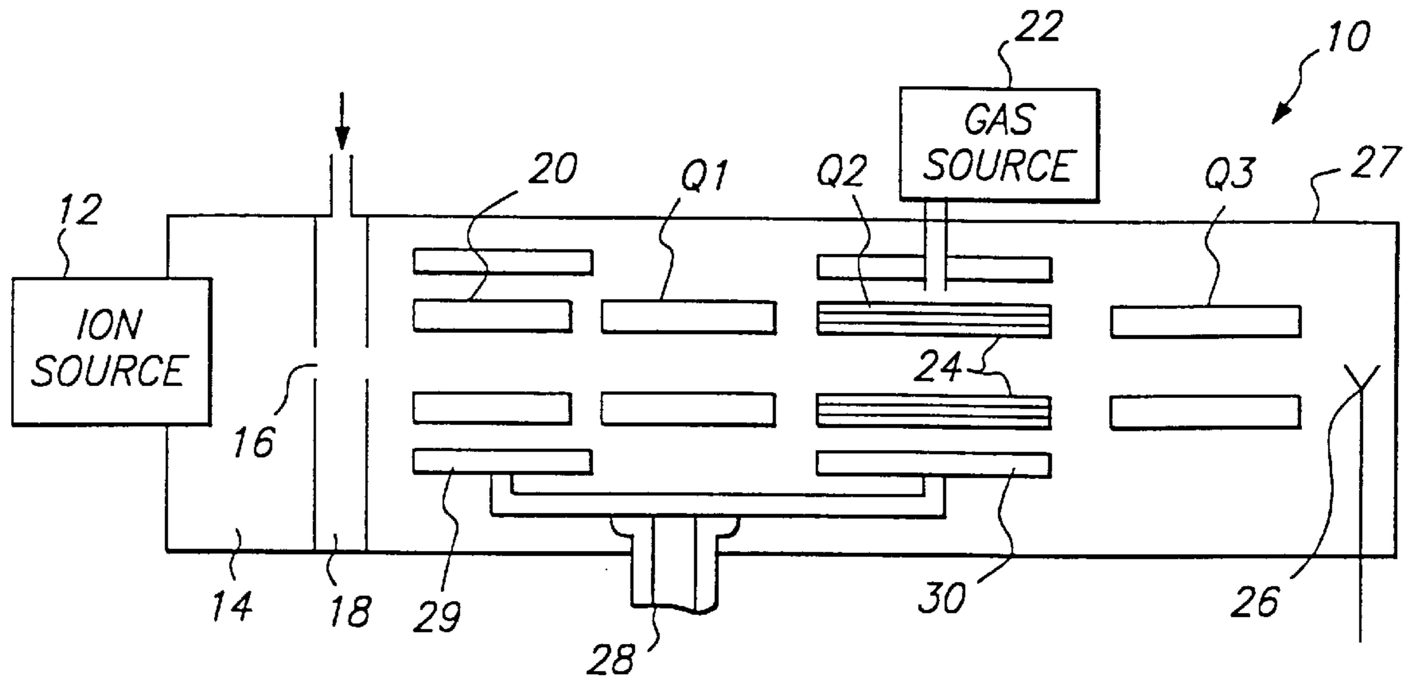
FIG. 1 (PRIOR ART)
