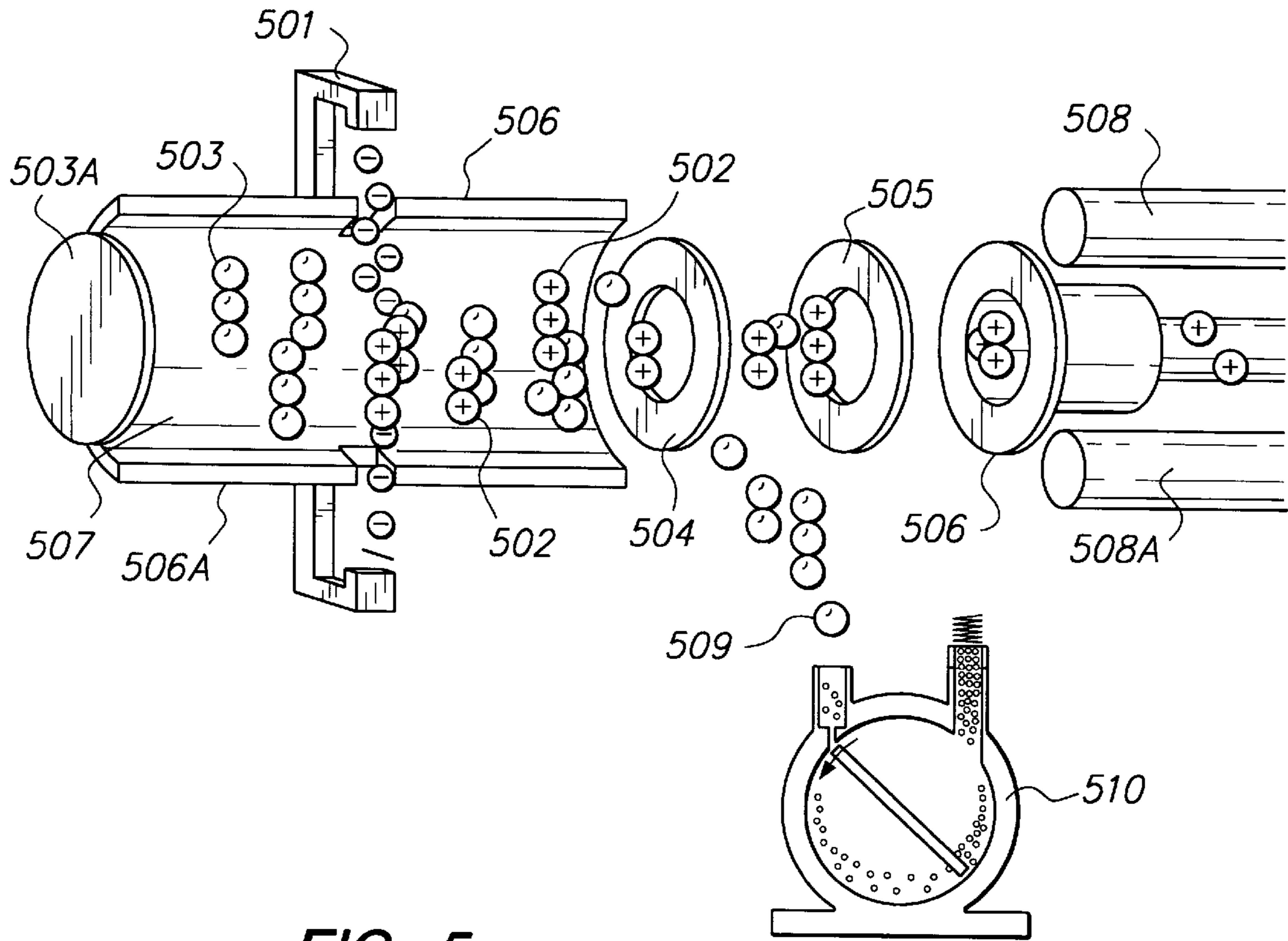
FIG. 5 (PRIOR ART)
