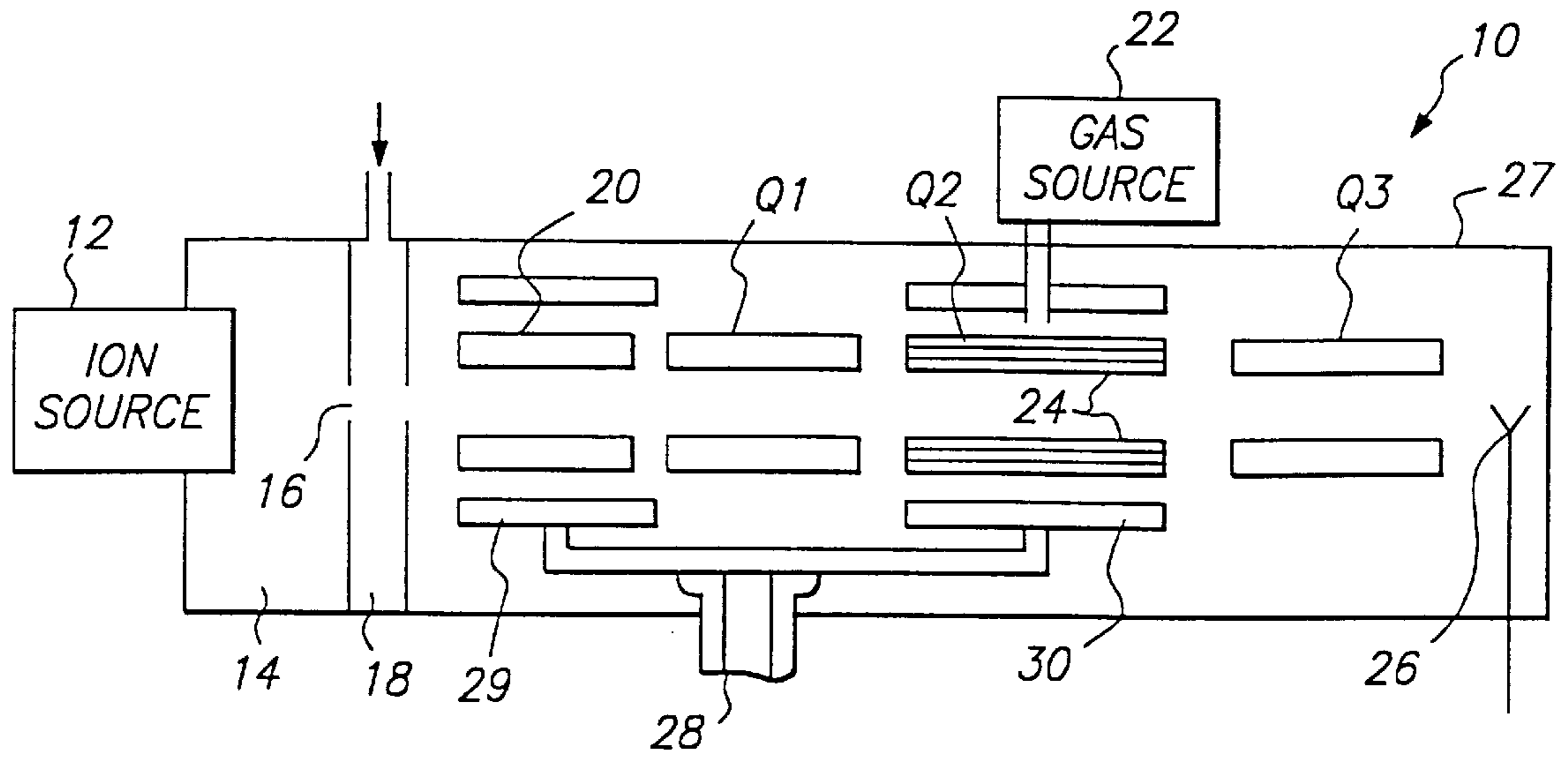
FIG. 1 (PRIOR ART)
