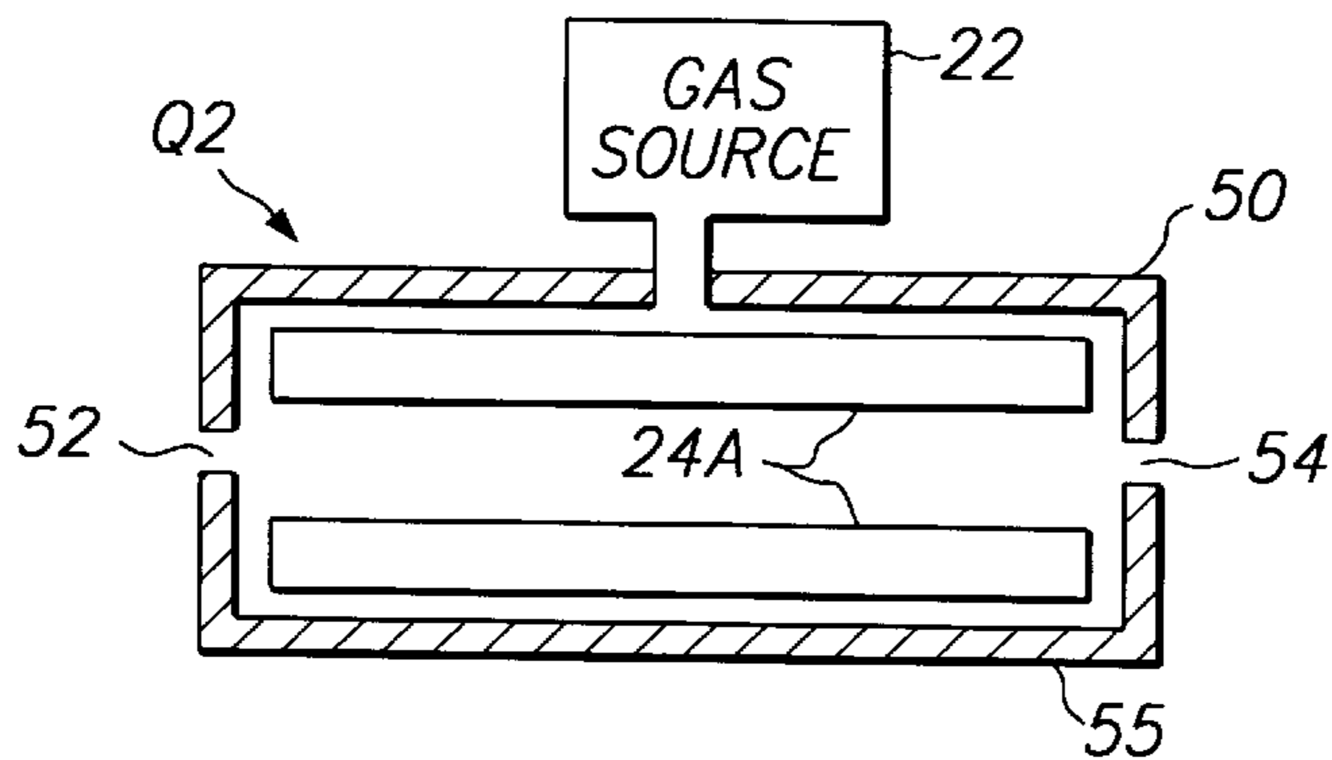
FIG. 6 (PRIOR ART)
