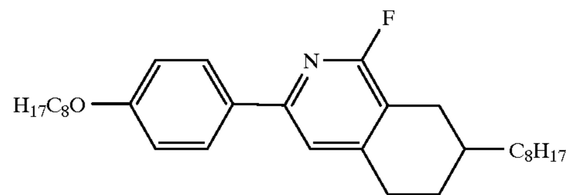
1-Fluoro-3-[4-(octyloxy)phenyl]-7-octyl-5,6,7,8-tetrahydroisoquinoline
