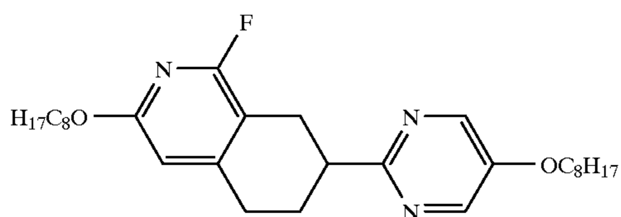
7-[5-(Octyloxy)pyrimidin-2-yl]-1-fluoro-3-octyloxy-5,6,7,8-tetrahydroisoquinoline
