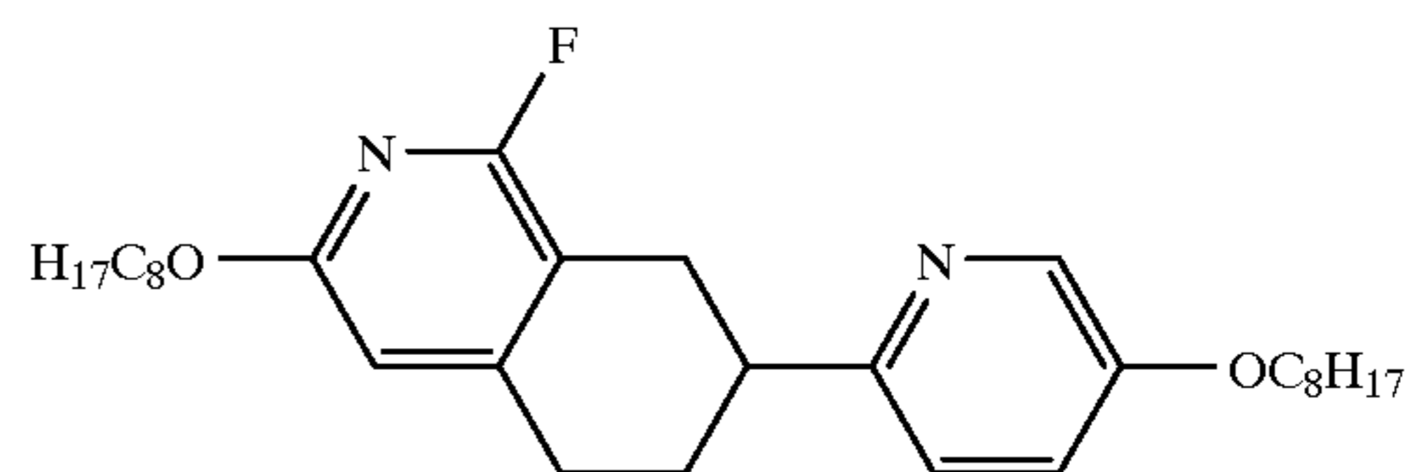
7-[5-(Octyloxy)pyridin-2-yl]-1-fluoro-3-octyloxy-5,6,7,8-tetrahydroisoquinoline
