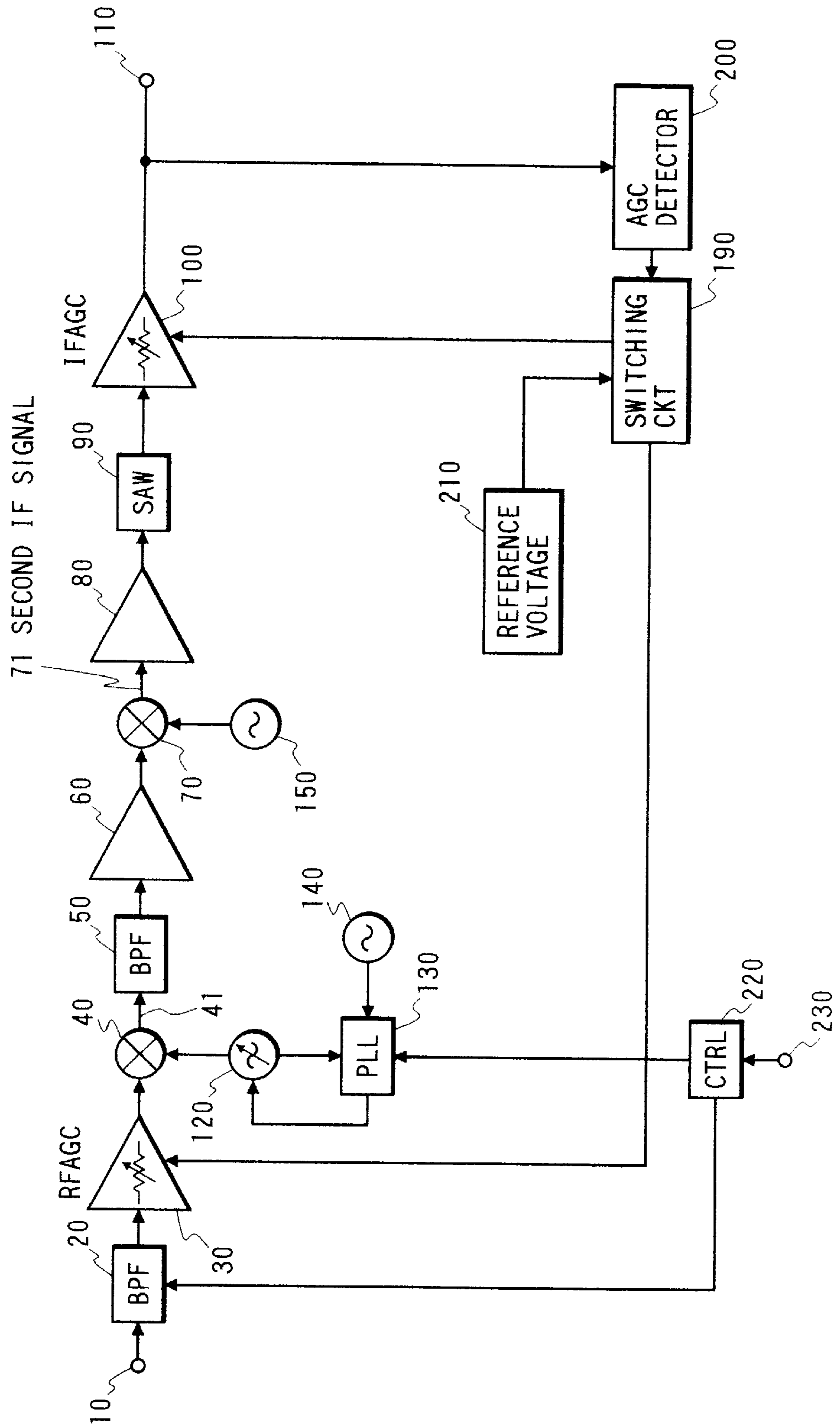
FIG. 4 PRIOR ART
