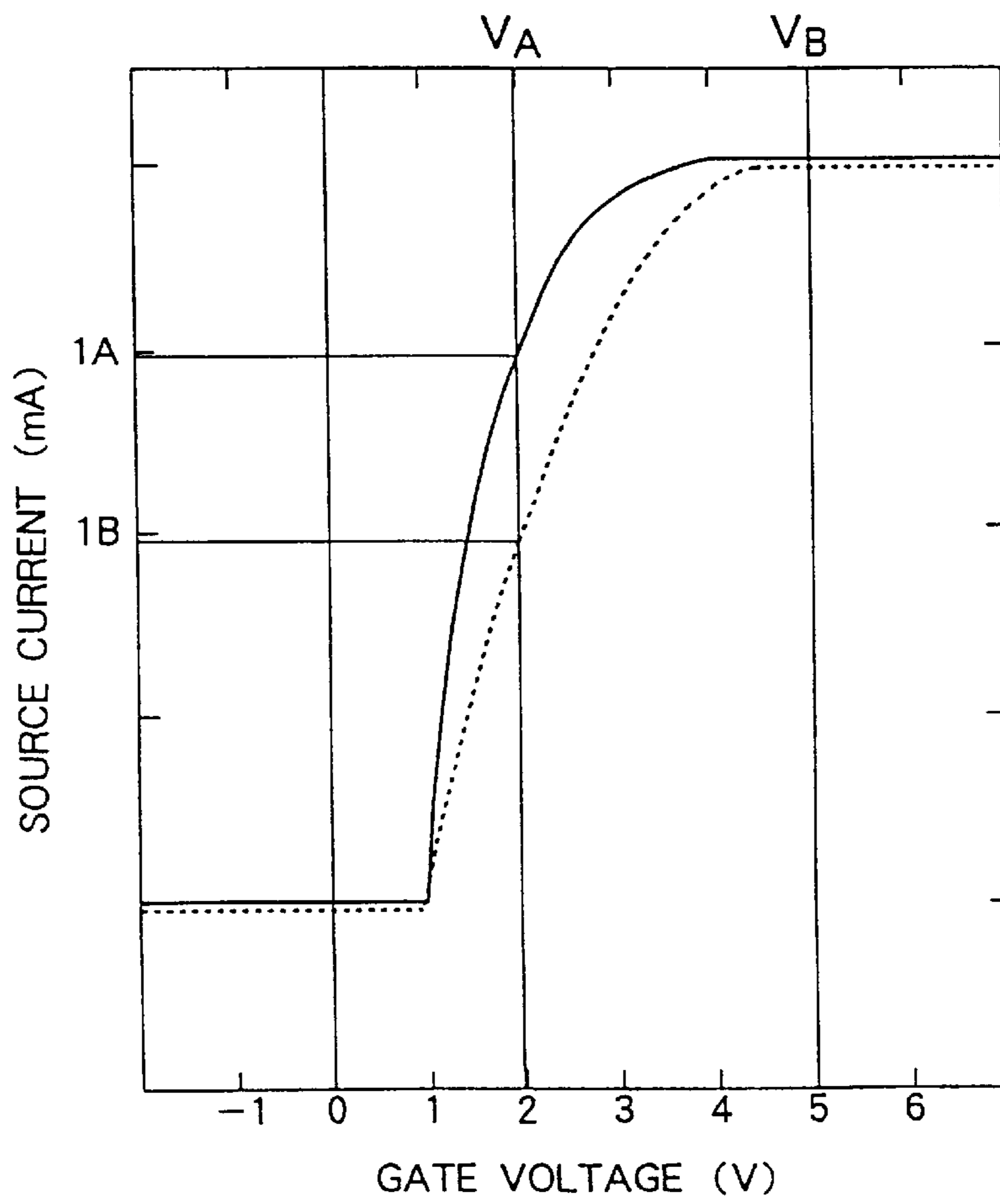
FIG. 3 PRIOR ART
