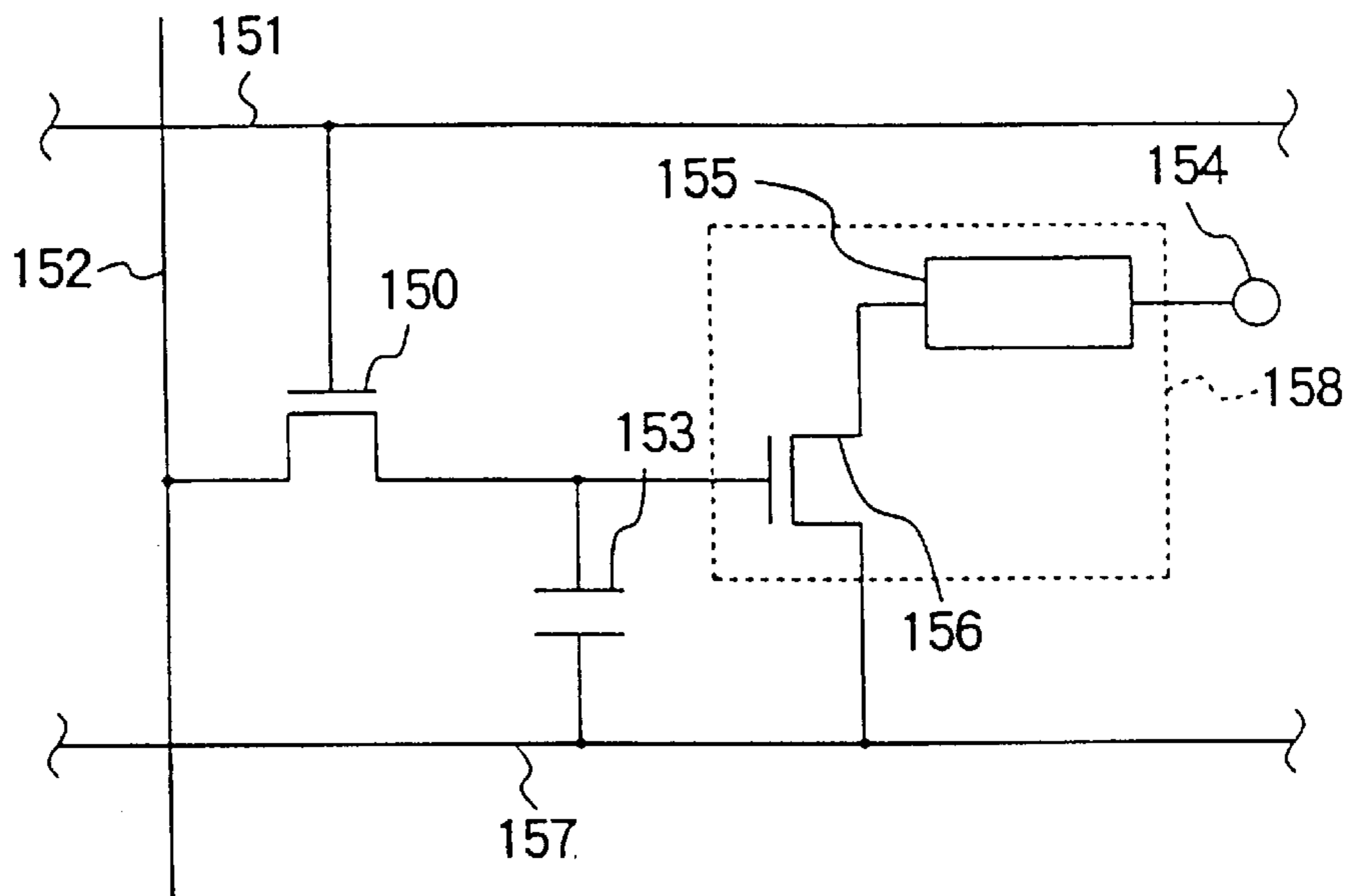
FIG. 2 PRIOR ART
