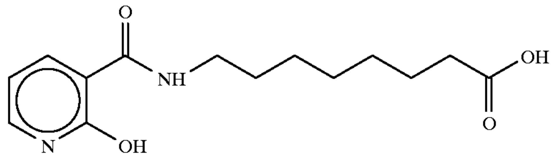
8-(2-Hydroxynicotinoyl)aminocaprylic acid
