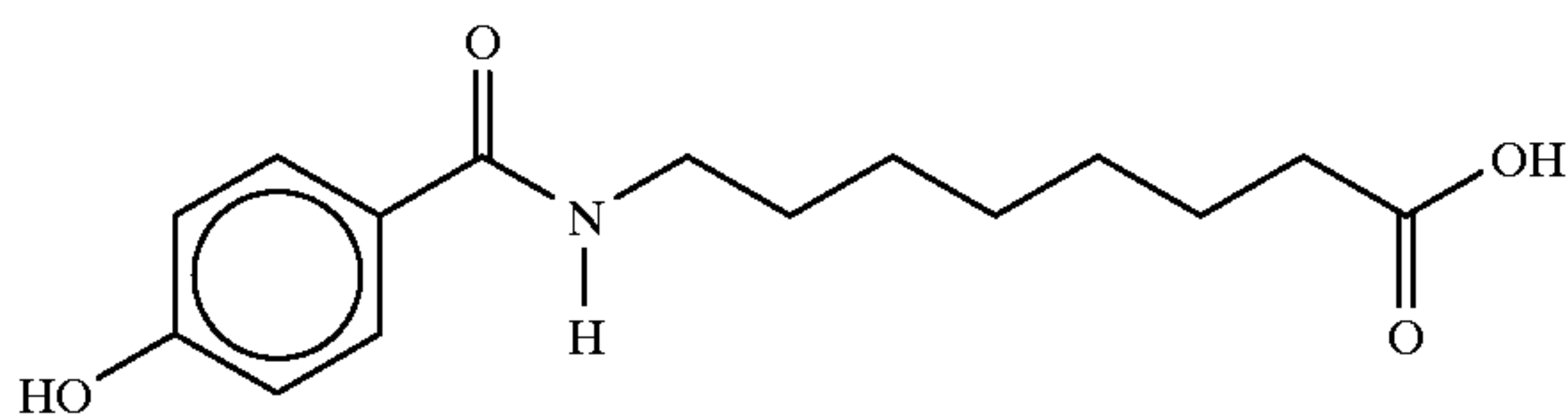
8-(N-2,4-Dihydroxybenzoyl)aminocaprylic acid
