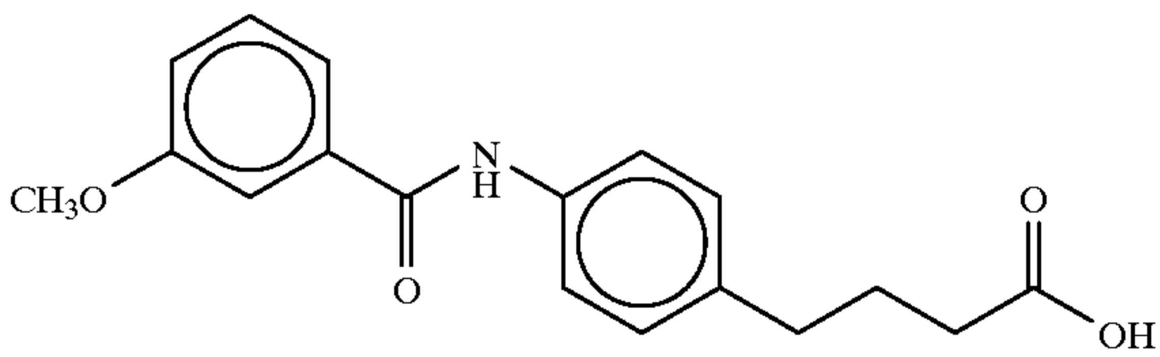
4-(4-(3-anisoyl)aminophenyl)butyric acid
