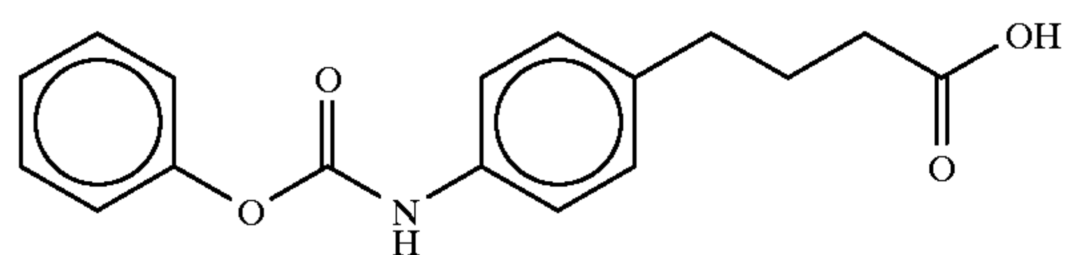
4-(4-phenyloxycarbonylamino)phenylbutyric acid
