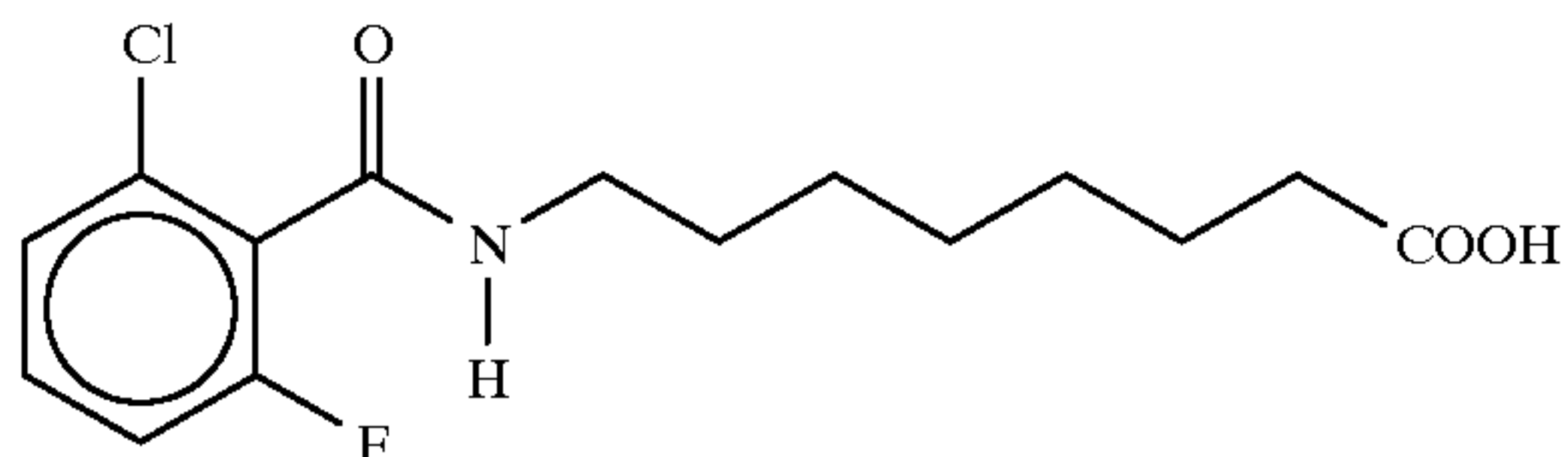
8-N-(2-chloro-6-fluorobenzoyl)aminocaprylic acid
