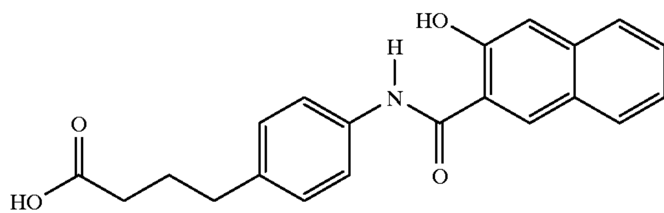
4-{4-[N-(3-hydroxy-2-naphthoyl)aminophenyl]}butanoic acid
