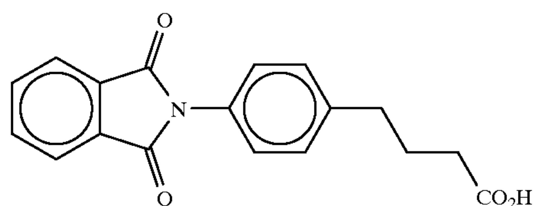
4-(4-phthalimidophenyl)butyric acid
