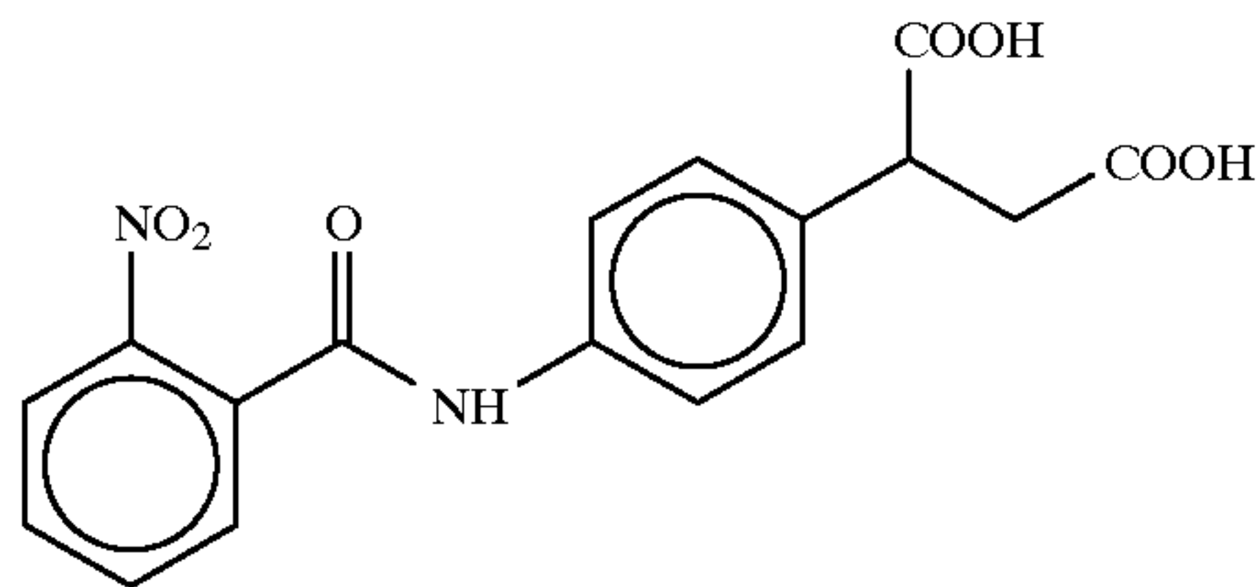
4-(2-Nitrobenzoyl)aminophenylsuccinic acid
