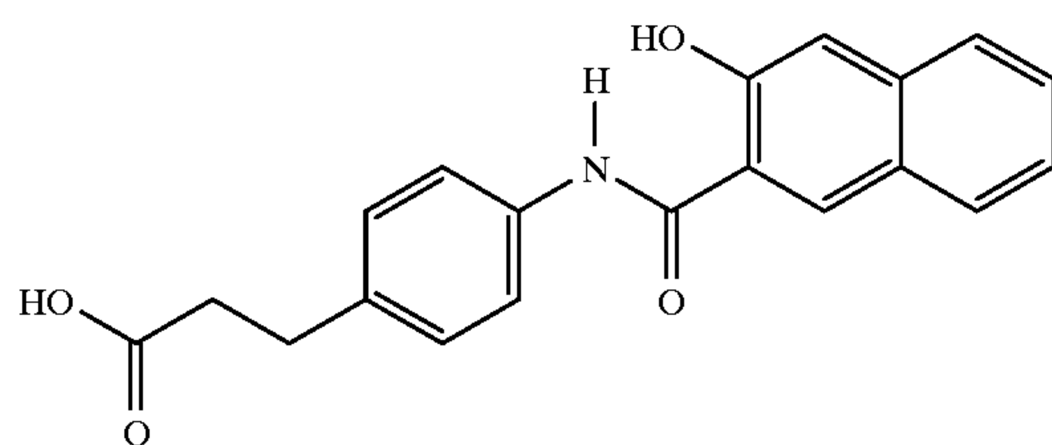
4-{4-[N-(3-hydroxy-2-naphthoyl)aminophenyl]}propanoic acid
