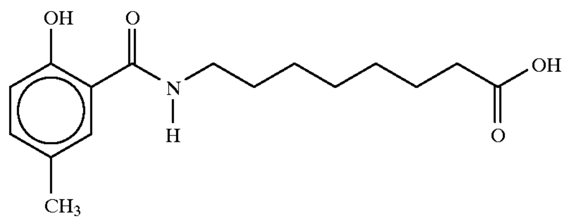
8-(N-5-methylsalicyloyl)aminocaprylic acid
