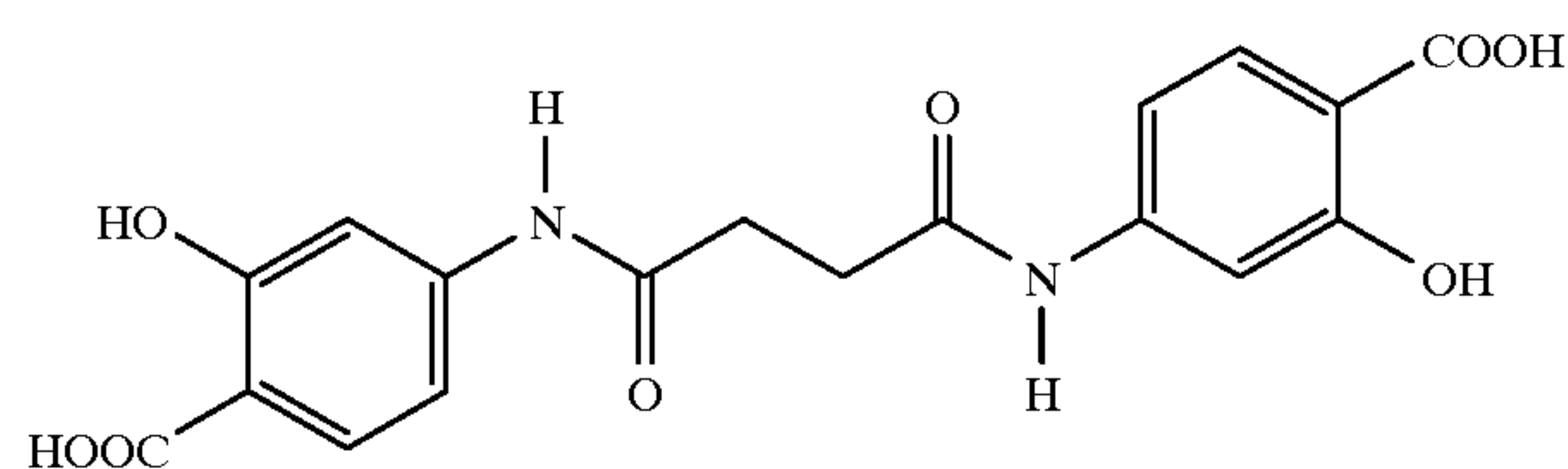
Succinyl-4-aminosalicylic acid
