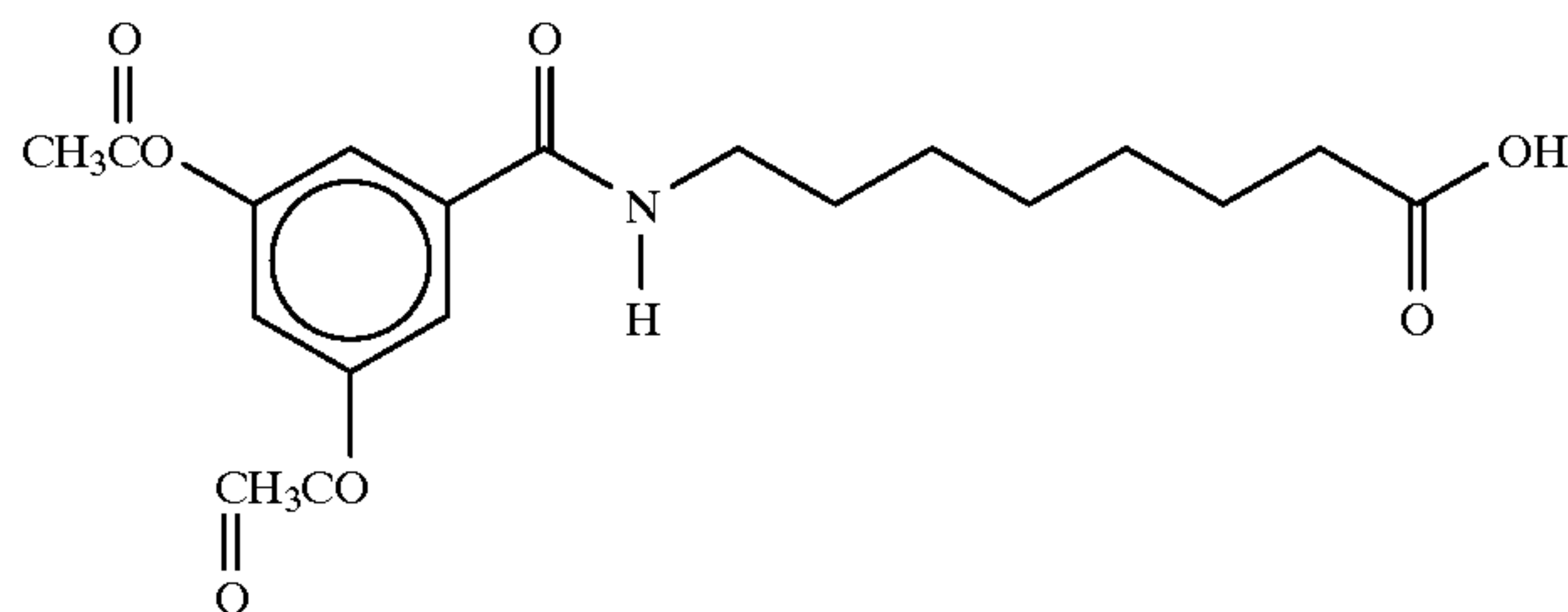
8-(N-3,5-Diacetyloxybenzoyl)aminocaprylic acid
