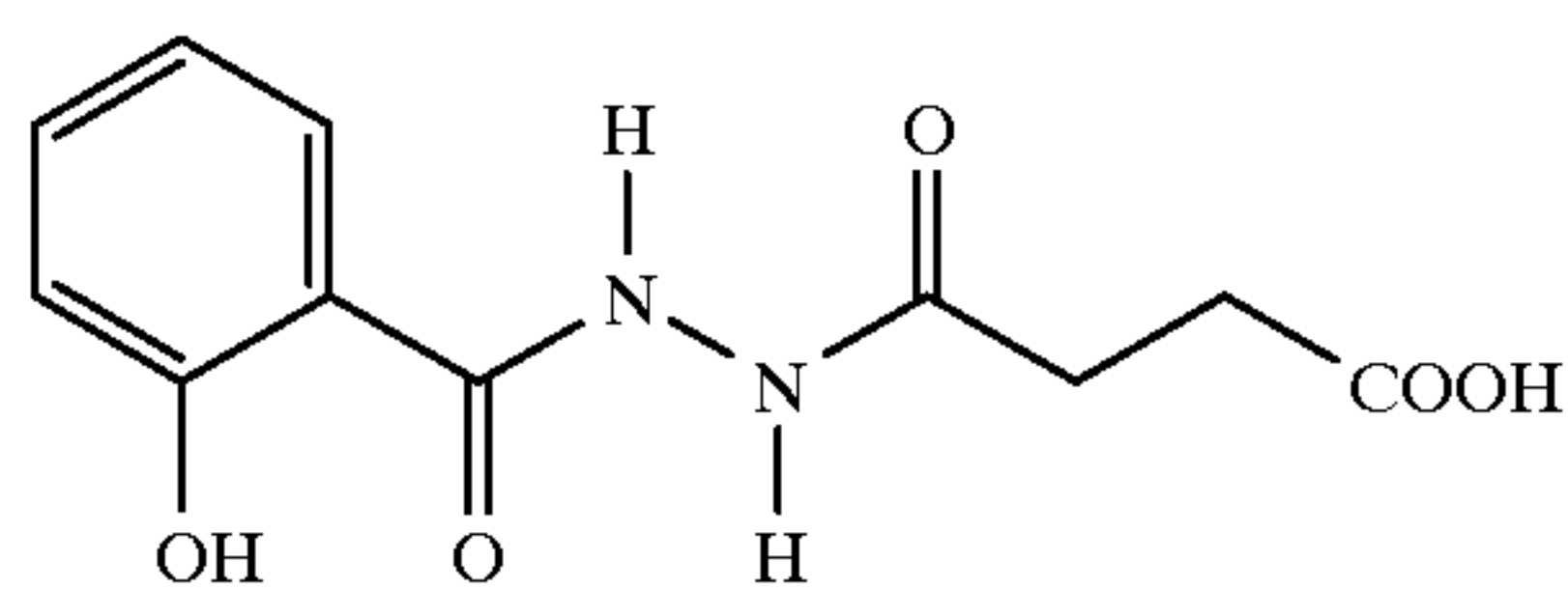
1-salicyloyl-2-succinyl hydrazide
