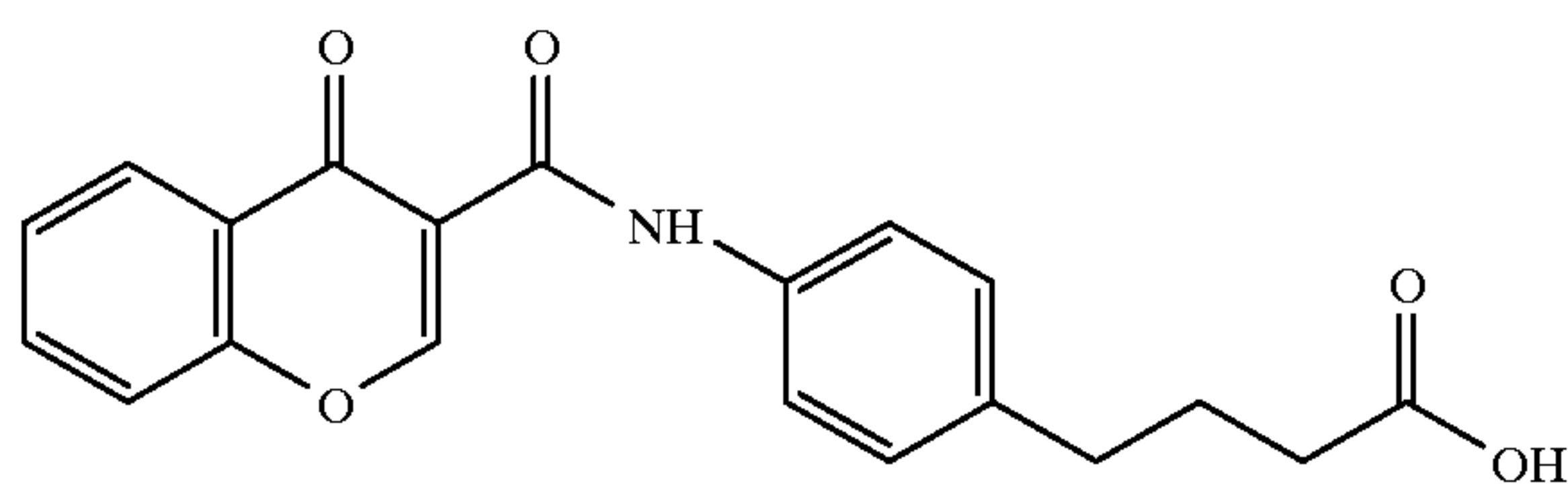
4-(4-(chromone-3-carbonyl)aminophenyl)butyric acid
