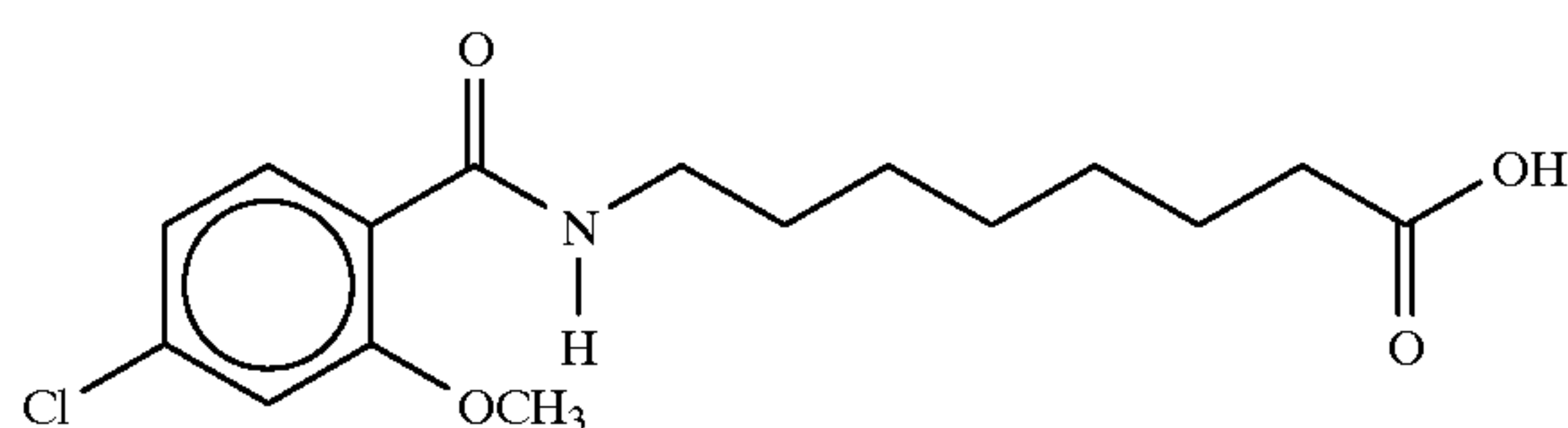
8-(4-chloro-o-anisoyl)aminocaprylic acid
