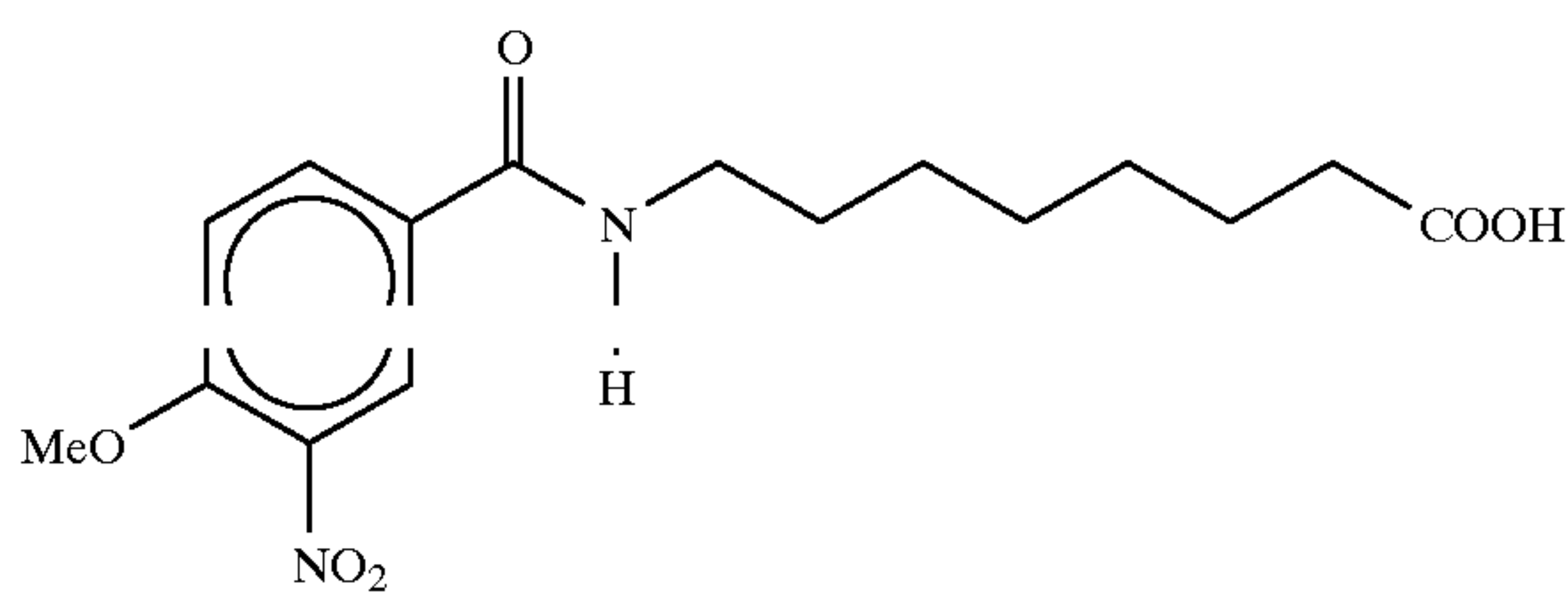
8-N-(4-methoxy-3-nitrobenzoyl)aminocaproic acid
