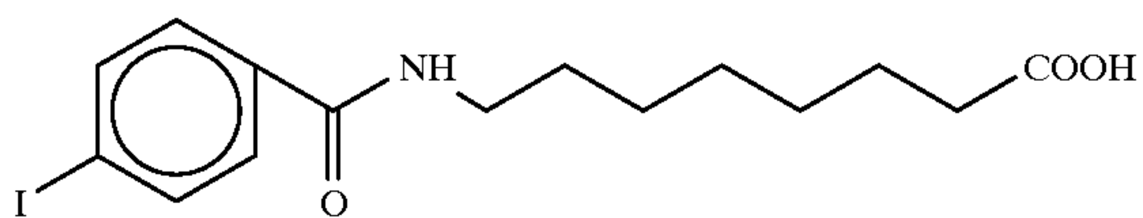
8-[N-(4-iodobenzoyl)]aminocaprylic acid
