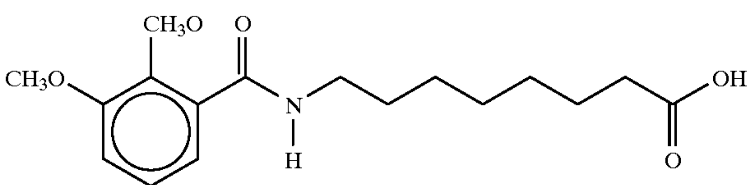
8-(N-2,3-Dimethoxybenzoyl)aminocaprylic acid
