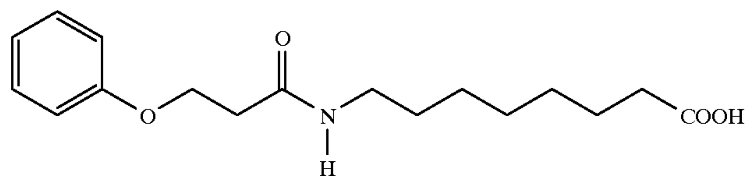
8-(3-Phenoxypropionylamino)caprylic acid
