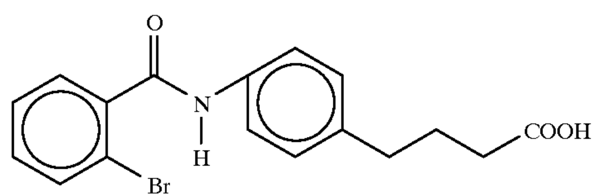
4{4-[N-2-bromobenzoyl]}aminophenyl}butyric acid
