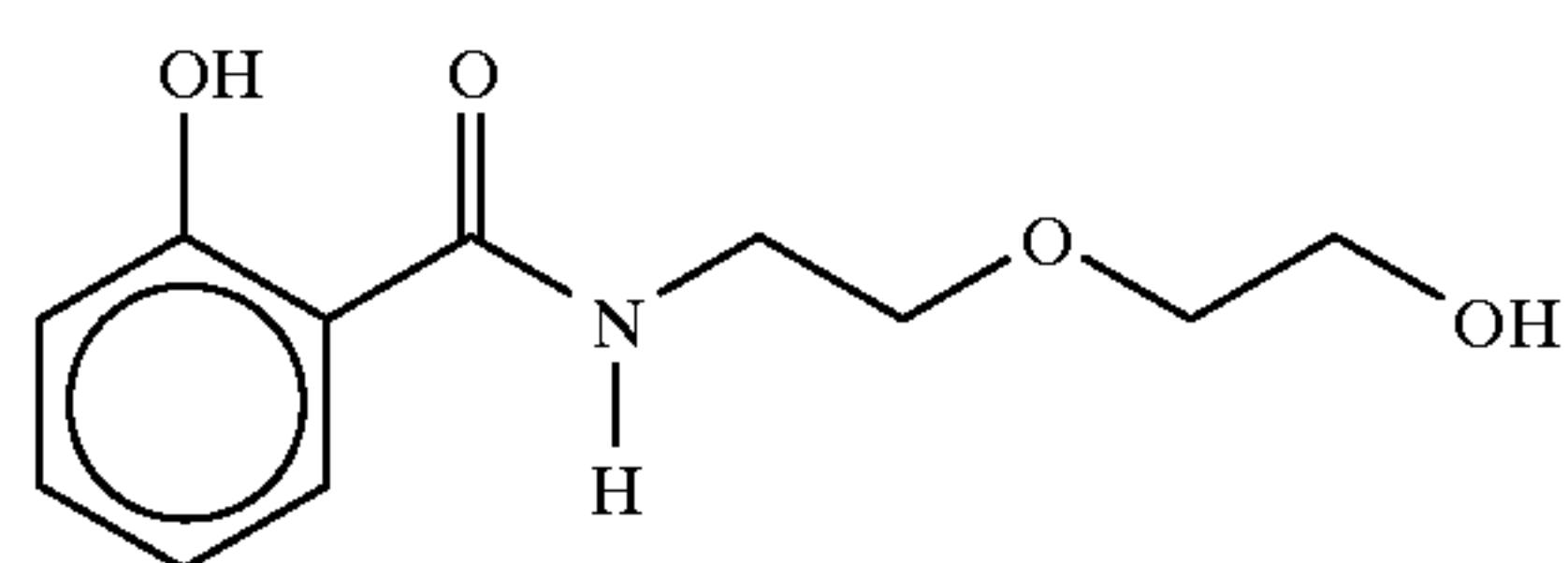
2-[N-(2-hydroxybenzoylamino)ethoxy]ethanol
