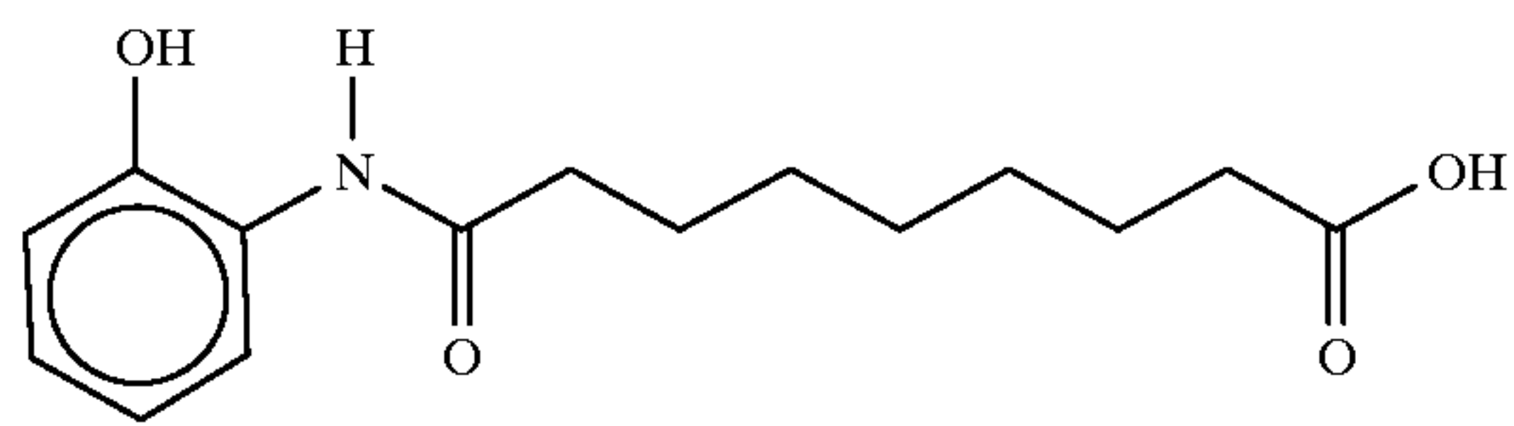
9-(2-hydroxybenzamido)nonanoic acid
