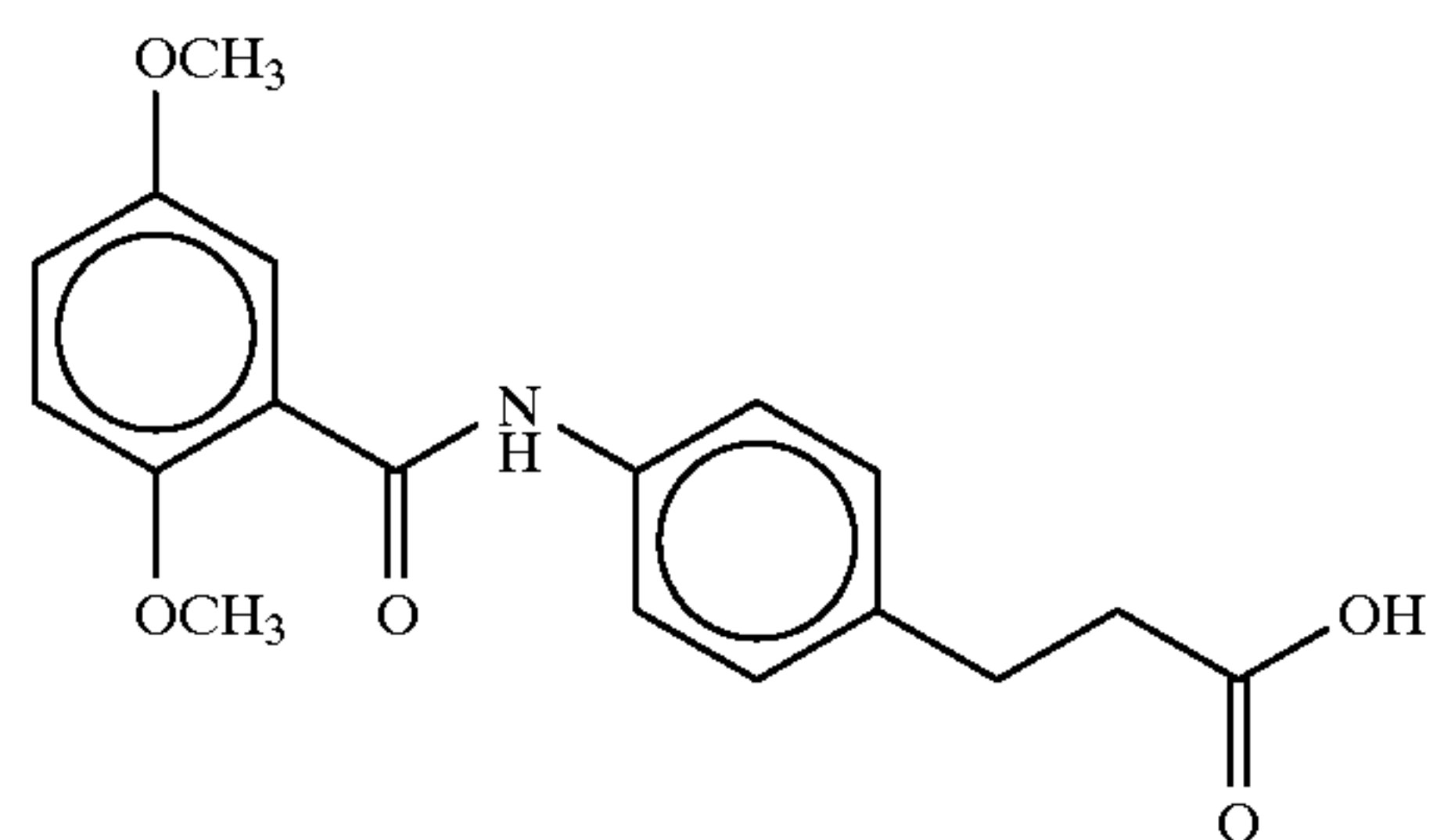
3-(4-(2,5-dimethoxybenzoyl)aminophenyl)propionic acid
