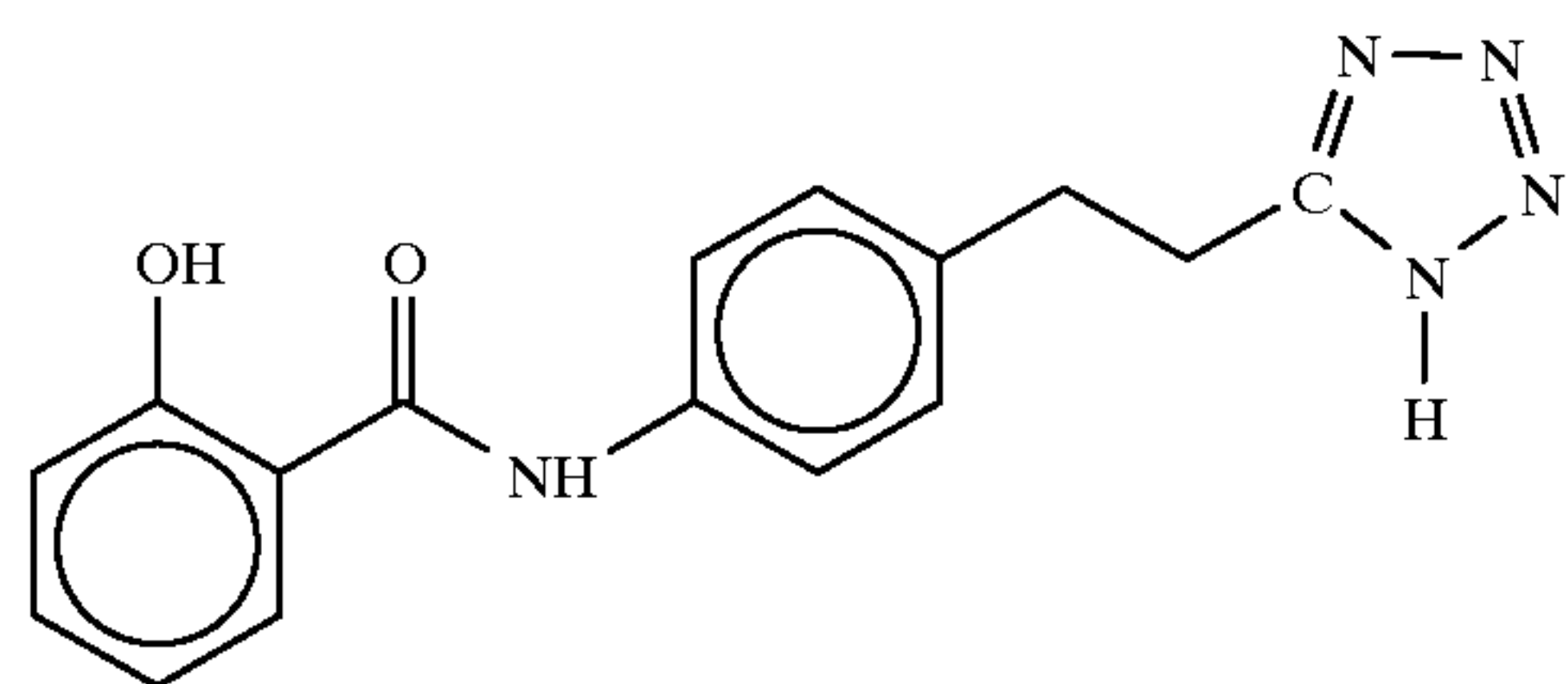
4-(Salicyloyl)aminophenylethyltetrazole
