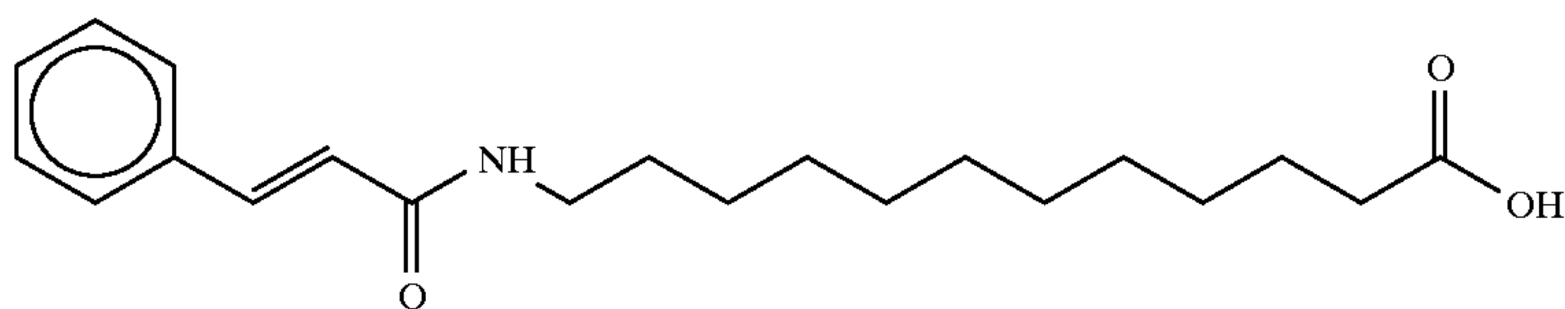
12-cinnamoyldodecanoic acid
