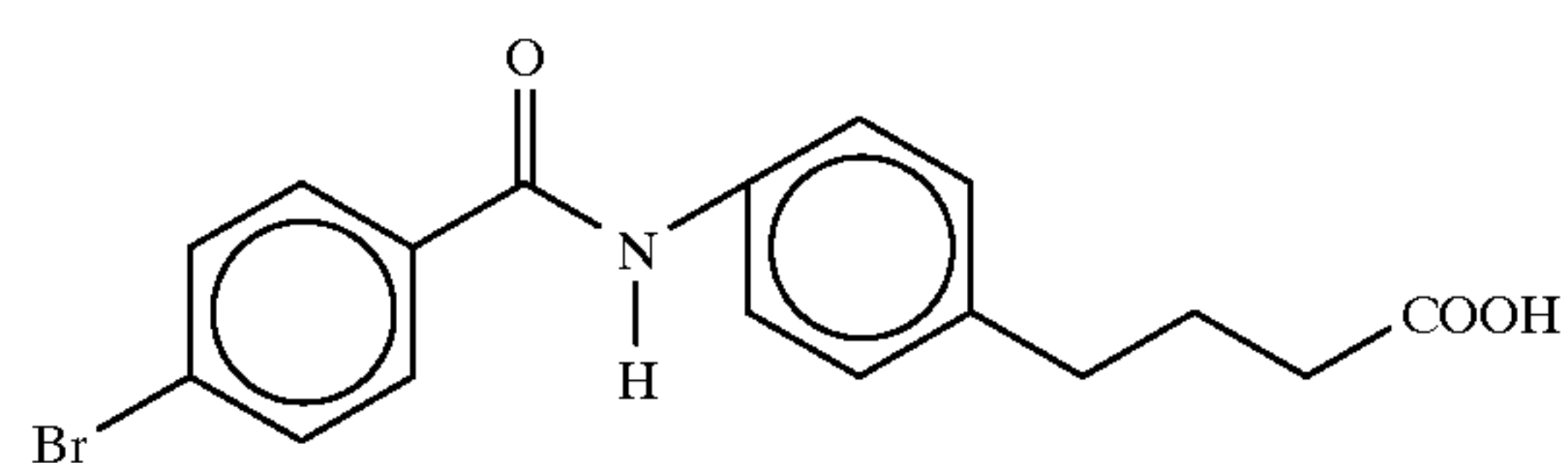
4{4-[N-(4-bromobenzoyl)aminophenyl]}butyric acid
