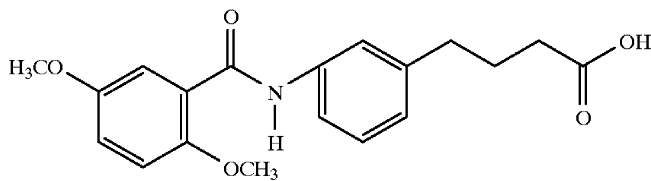
4-(4-(2,5-dimethoxybenzoyl)aminophenyl)butyric acid
