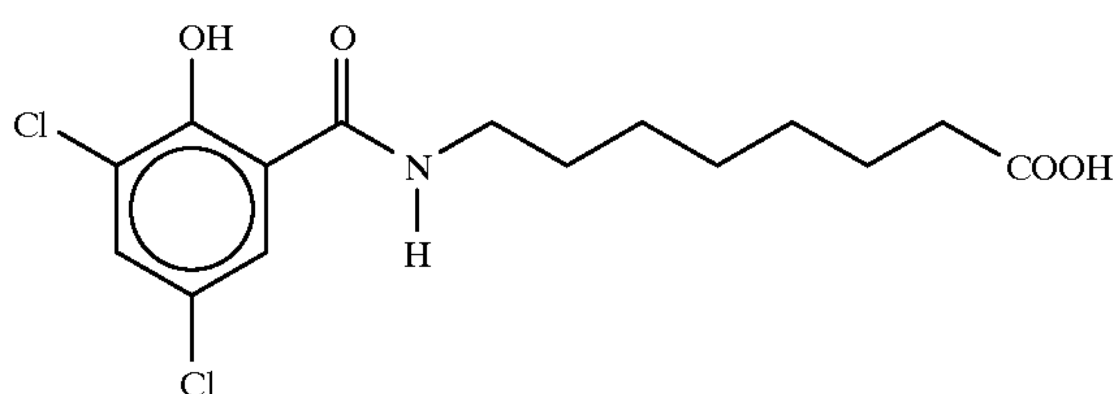
8-[N-(2-acetoxy-3,5-dichlorobenzoyl)]aminocaprylic acid
