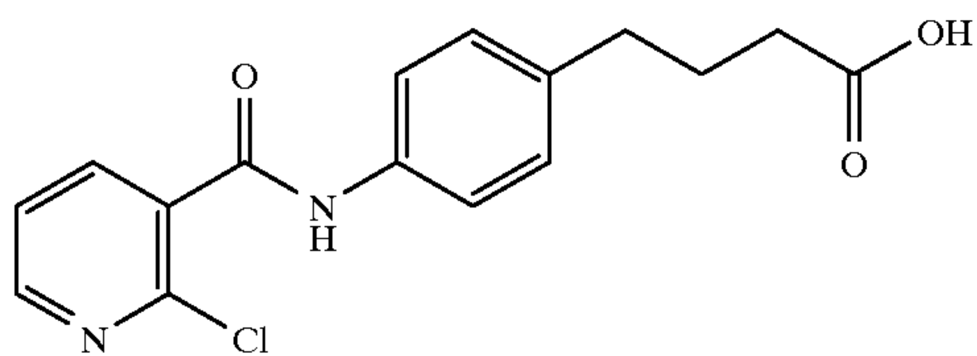
4-(4-(2-chloronicotinoyl)aminophenyl)butyric acid
