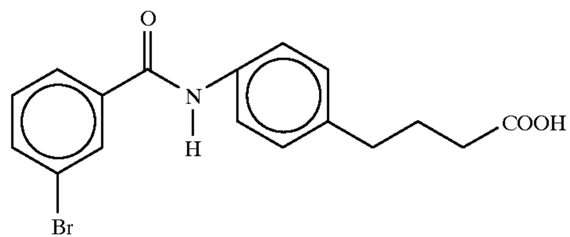
4{4-[N-3-bromobenzoyl]aminophenyl}butyric acid
