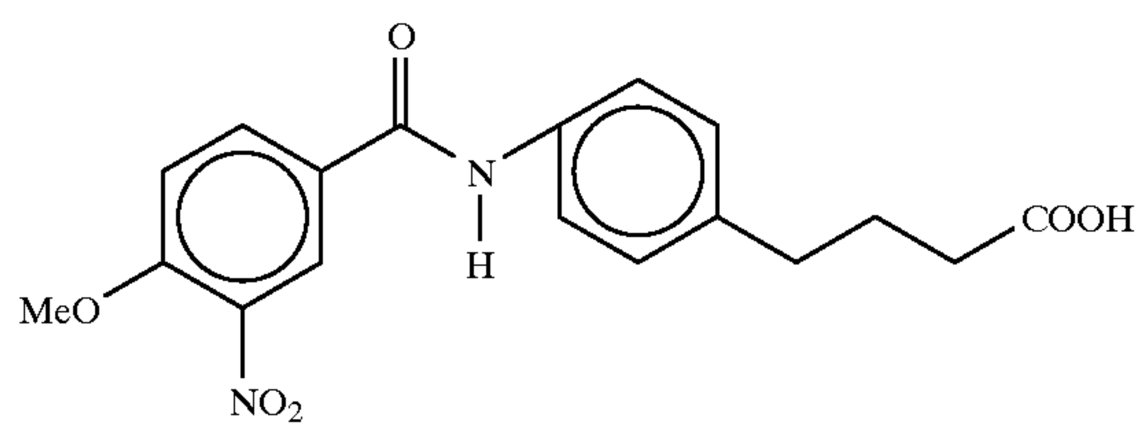
4-[4-N-(4-methoxy-3-nitrobenzoyl)aminophenyl]butyric acid
