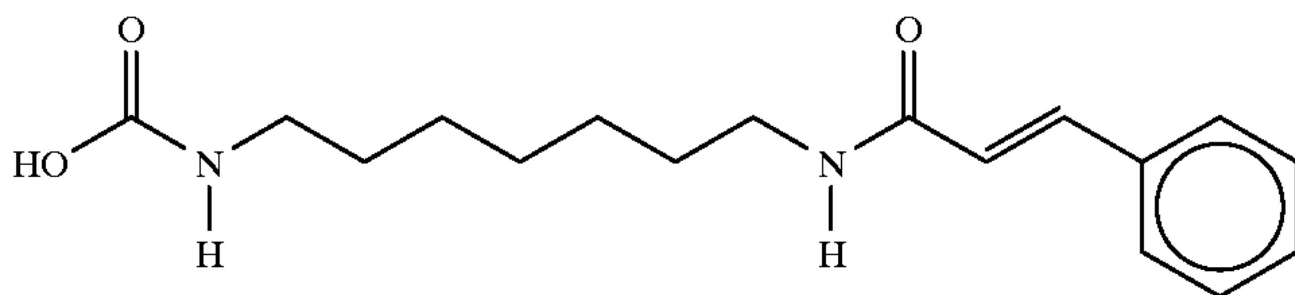
9-(cinnamoylamino)nonanoic acid
