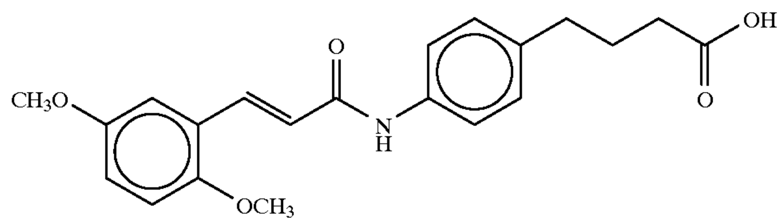
4-(4-(2,5-dimethoxycinnamoyl)aminophenyl)butyric acid
