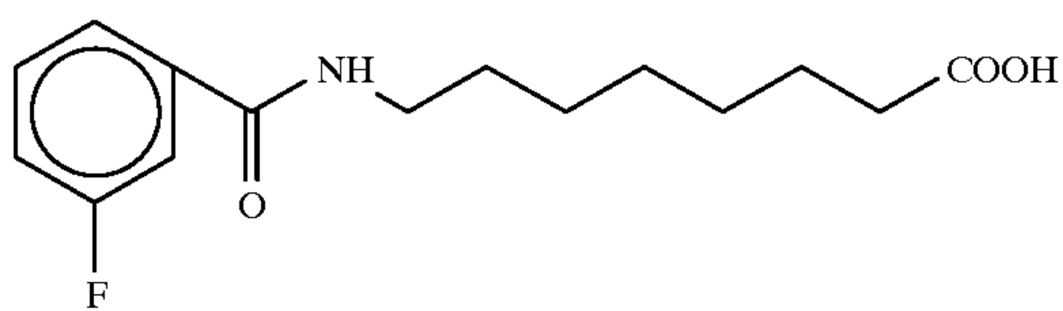
8-[N-(3-fluorobenzoyl)]aminocaprylic acid
