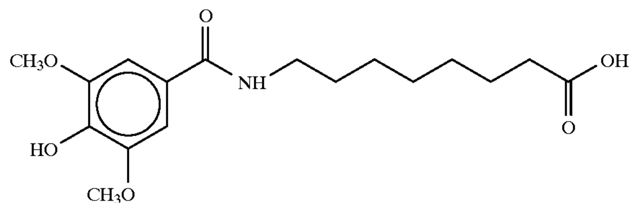
8-(N-3,5-Dimethoxy-4-hydroxybenzoyl)aminocaprylic acid
