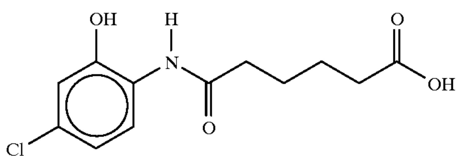
5-(4-chloro-2-hydroxyanilino)valeric acid
