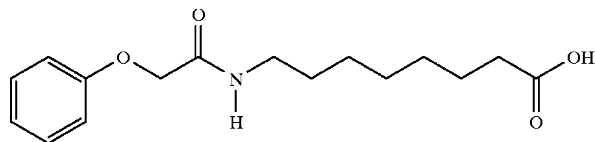
8-(Phenoxyacetyl)aminocaprylic acid
