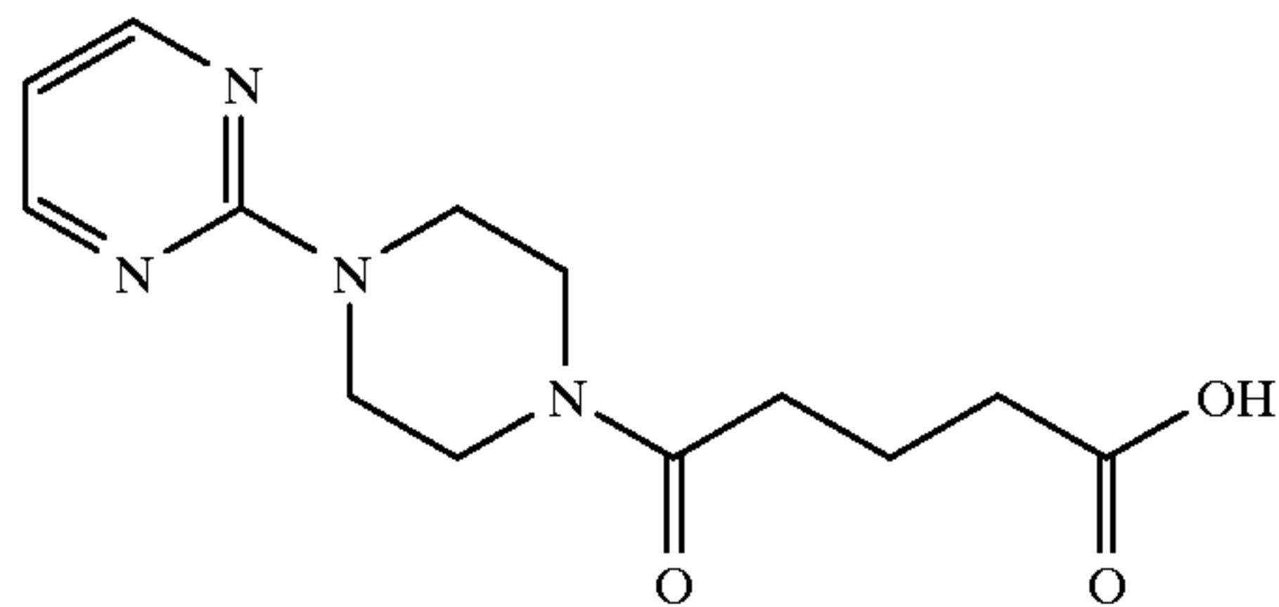
4-(1-(2-pyrimidyl)piperazinoyl)butyric acid
