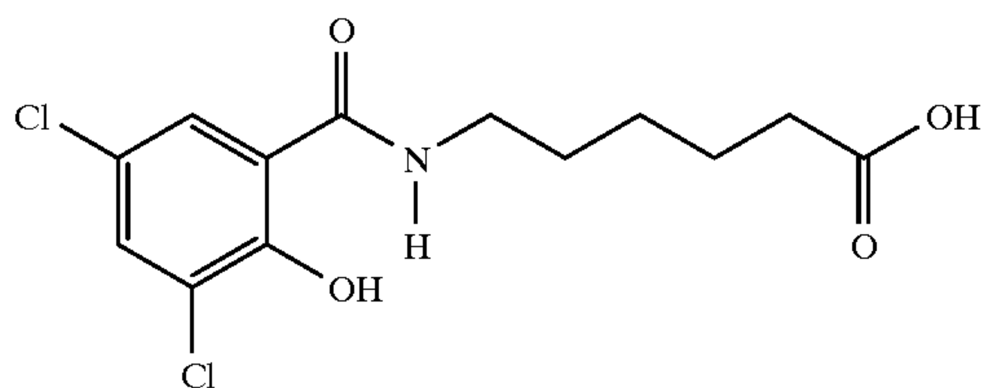
6-N-(3,5-dichloro-2-hydroxybenzoyl)aminocaproic acid
