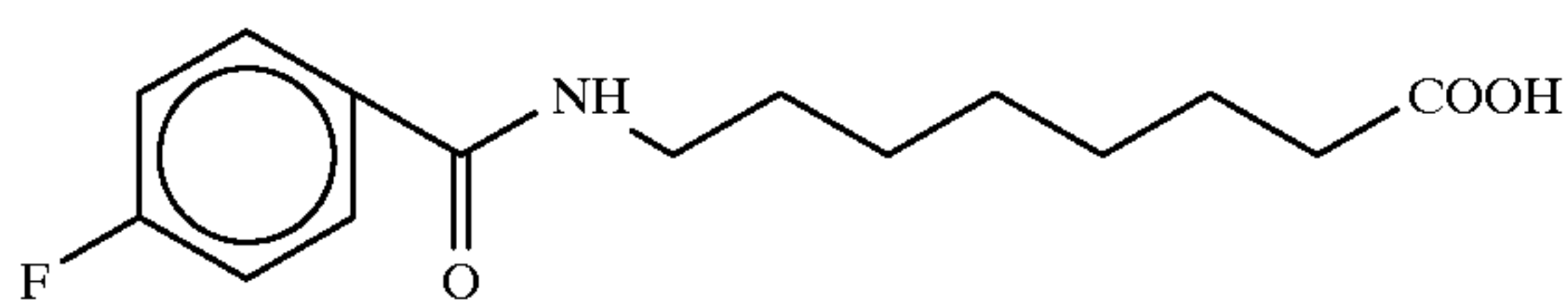
8-[N-(4-fluorobenzoyl)]aminocaprylic acid
