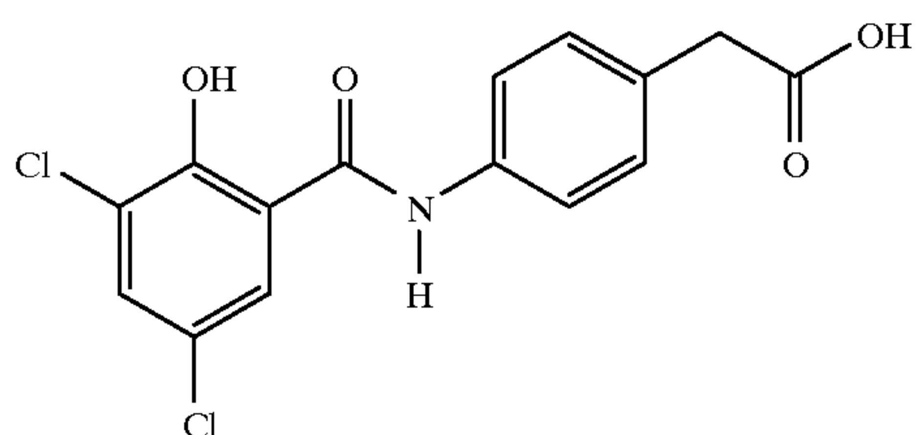
4-[N-(3,5-dichloro-2-hydroxybenzoyl)]aminophenylacetic acid
