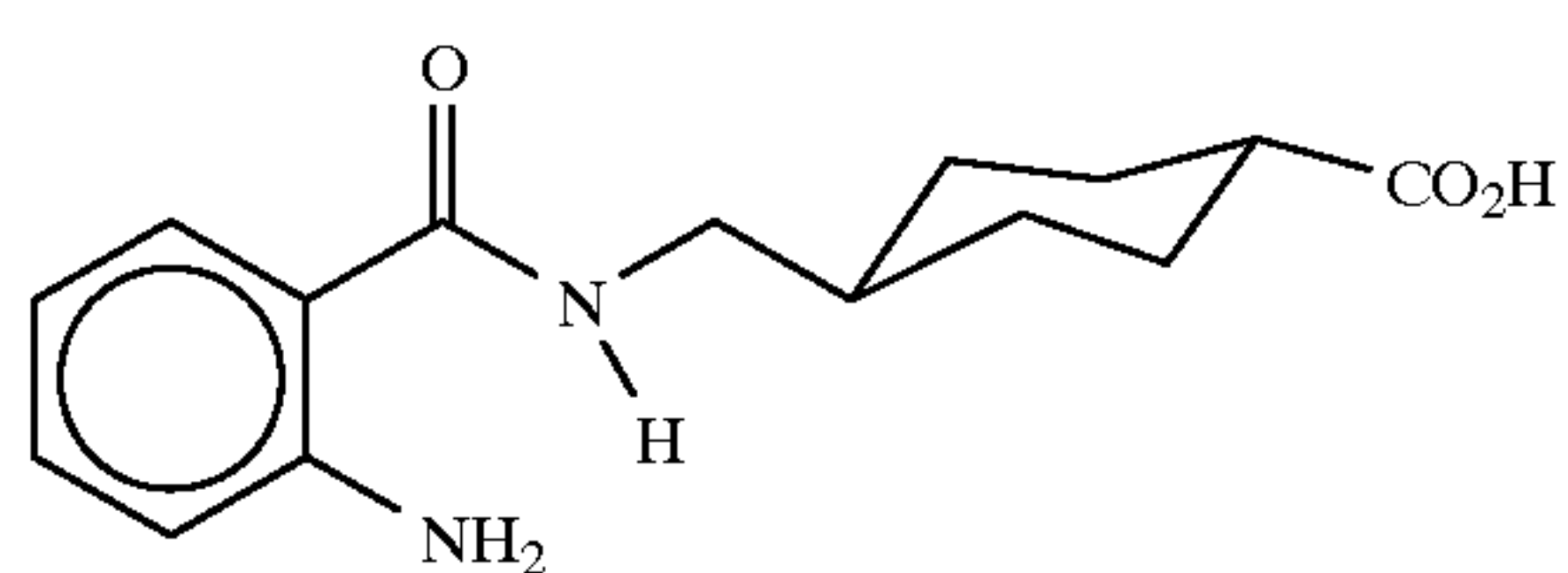
trans-4-(2-aminobenzamidomethyl)cyclohexanecarboxylic acid
