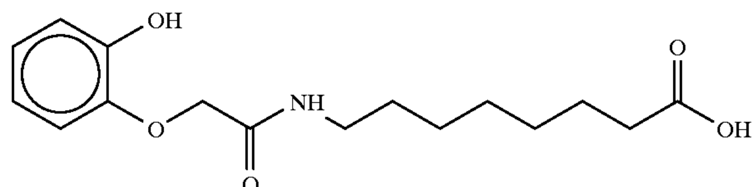
7-(2-hydroxyphenoxyacetyl)aminocaprylic acid
