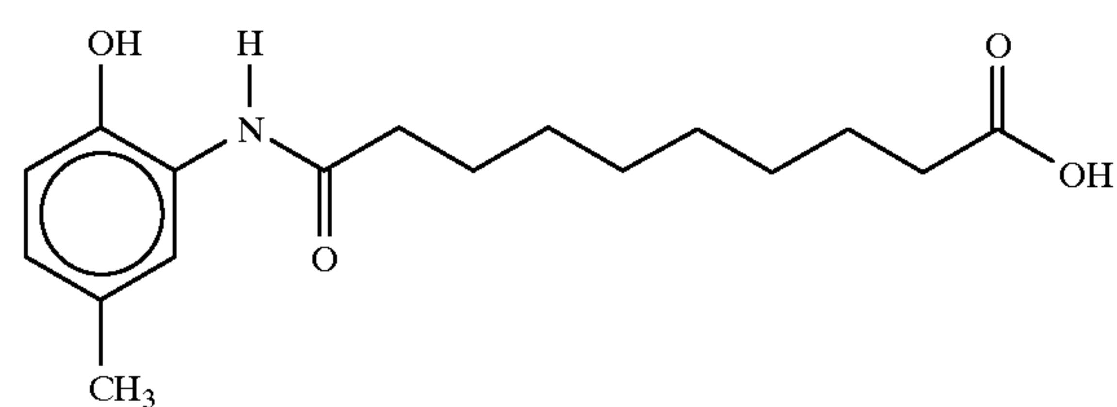
9-(2-hydroxy-5-methylanilino)nonanoic acid
