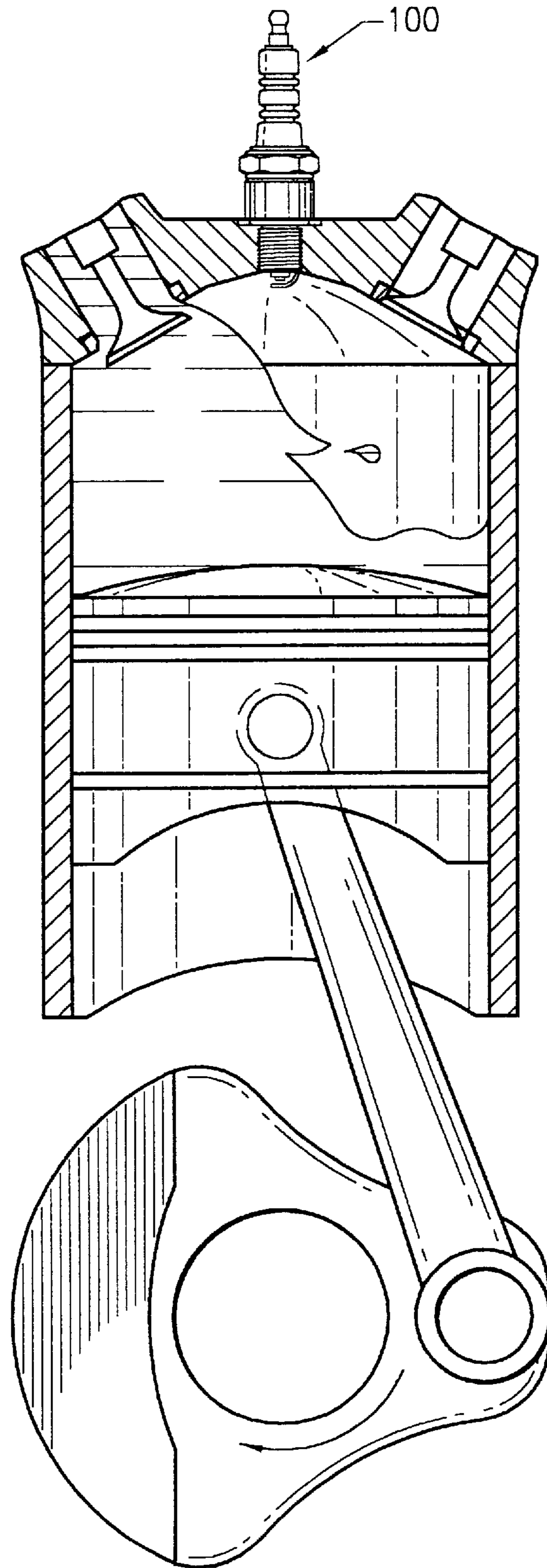
FIG. 2 (PRIOR ART)
