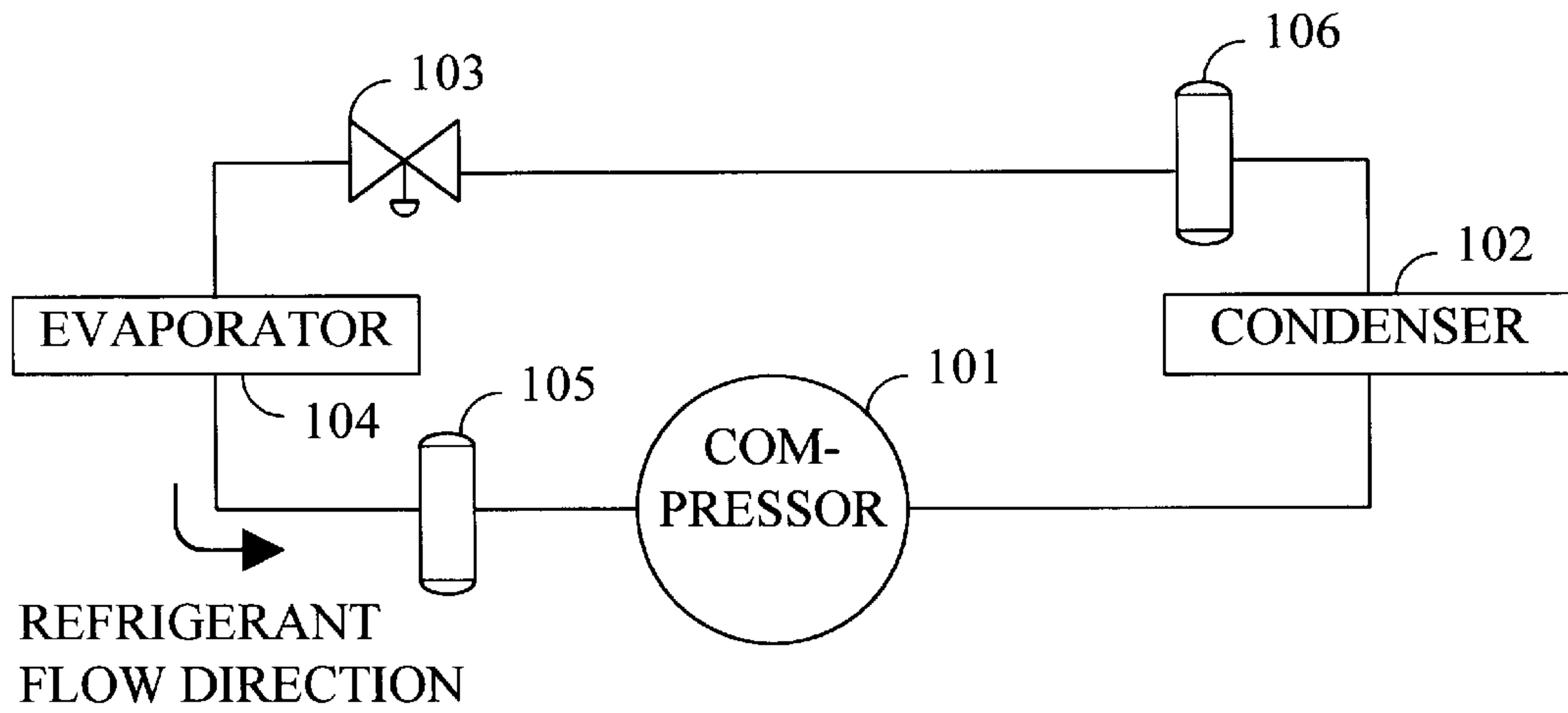
FIG. 1 (PRIOR ART)
