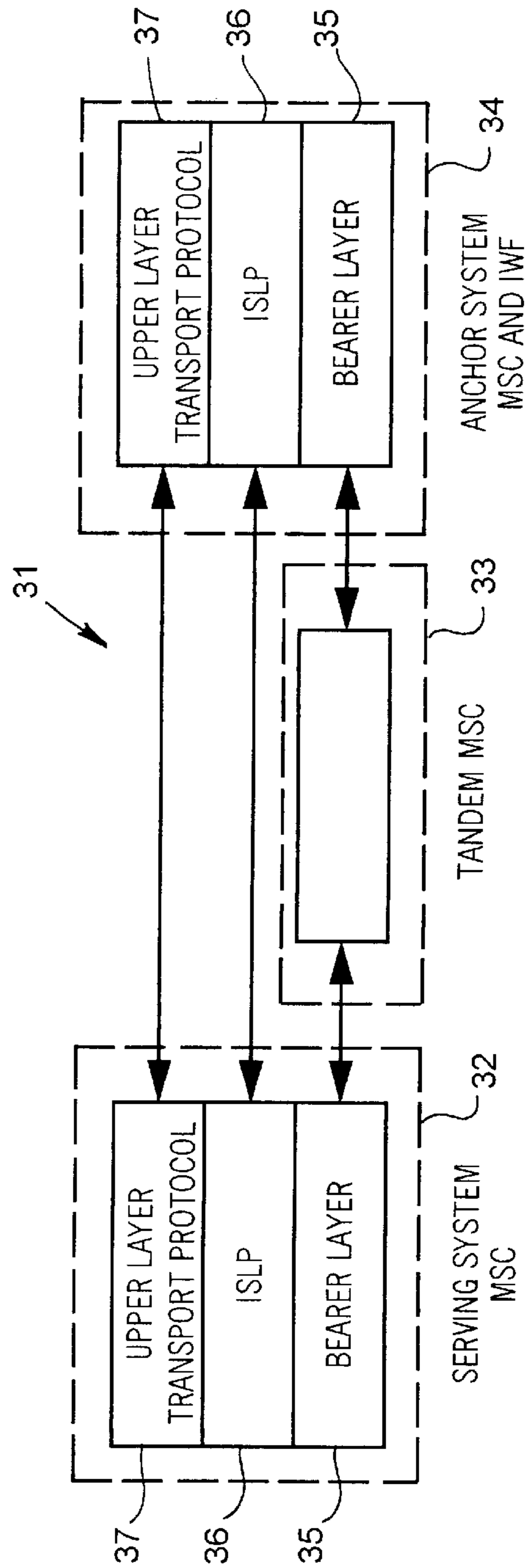
FIG. 2 (PRIOR ART)
