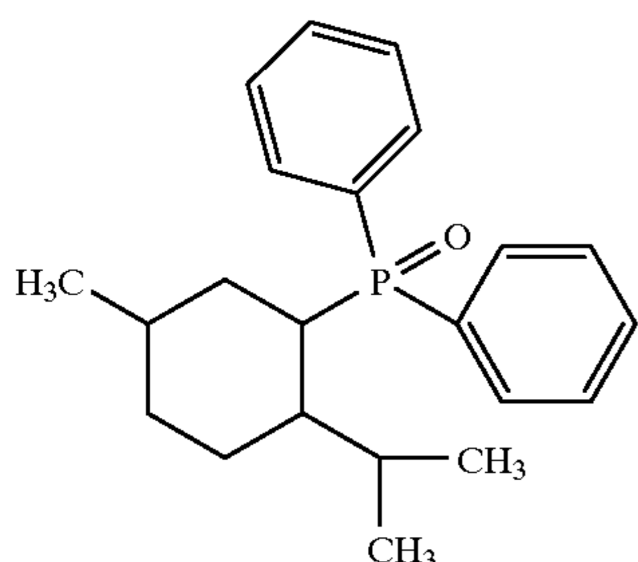
(2-Isopropyl-5-methylcyclohexyl)diphenylphosphine oxide, also referred to as Compound D; and
