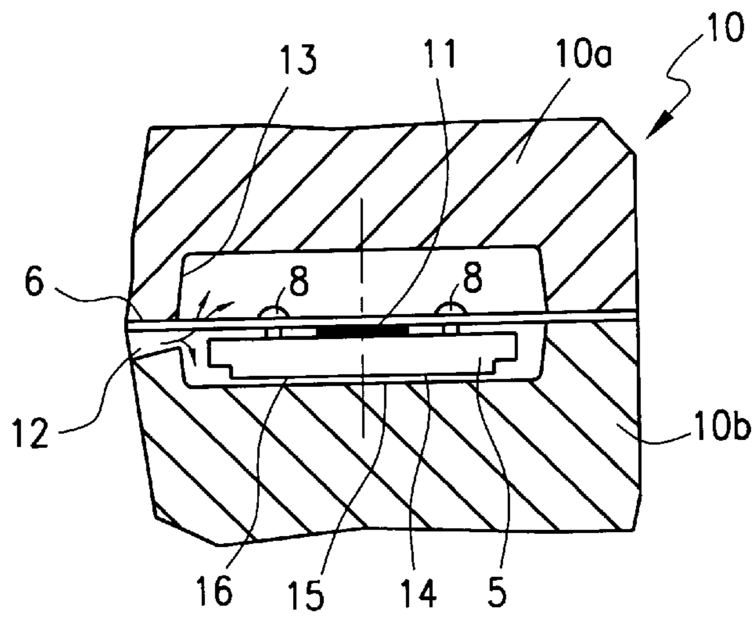
FIG. 3 (PRIOR ART)
