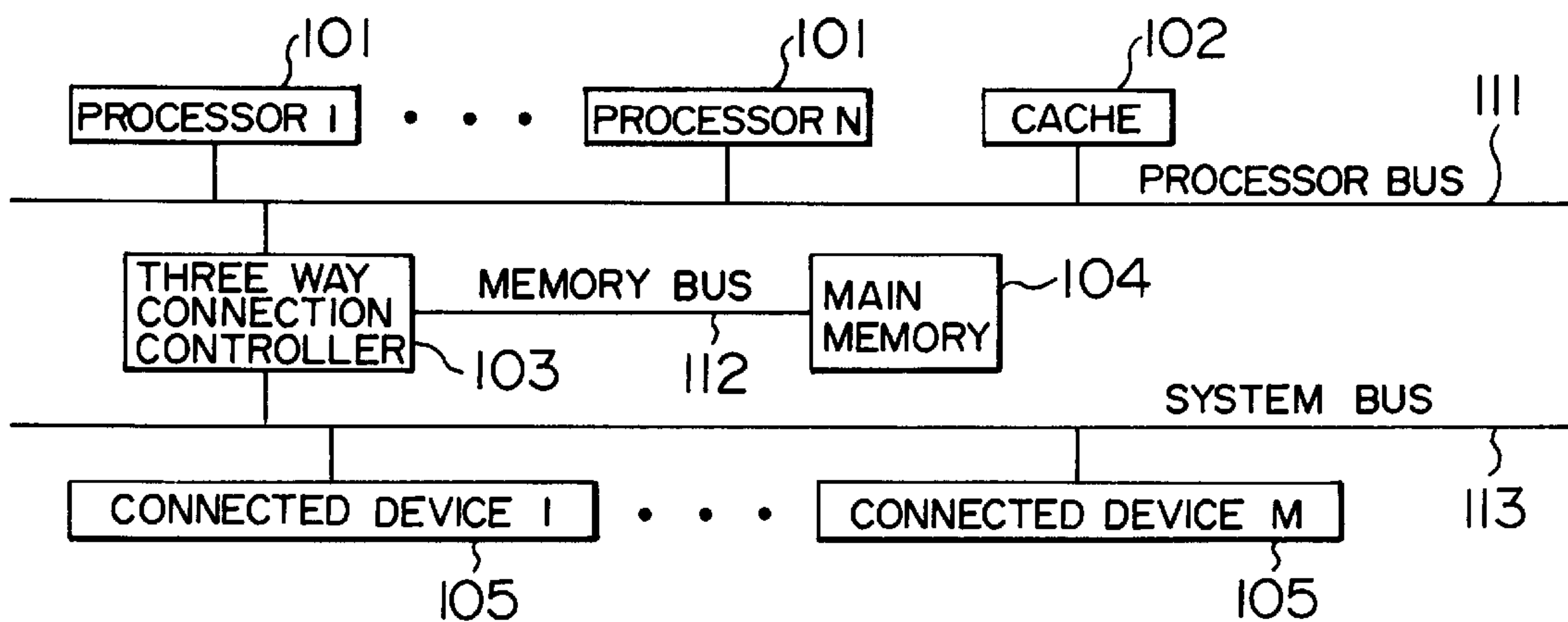
FIG. 2 PRIOR ART
