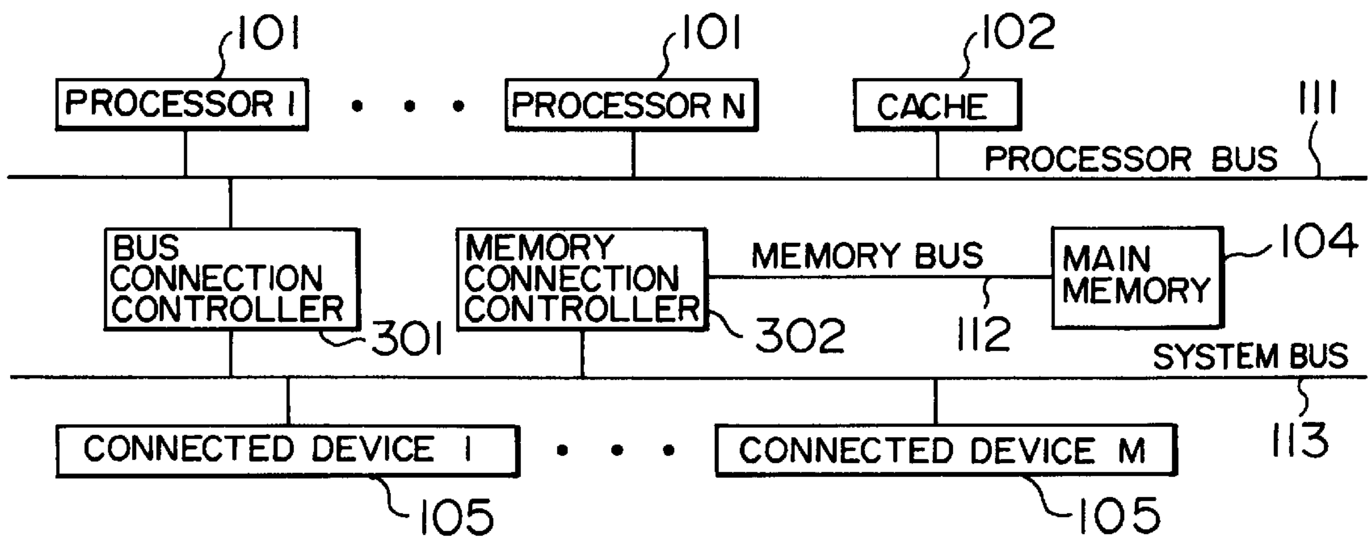
FIG. 3 PRIOR ART
