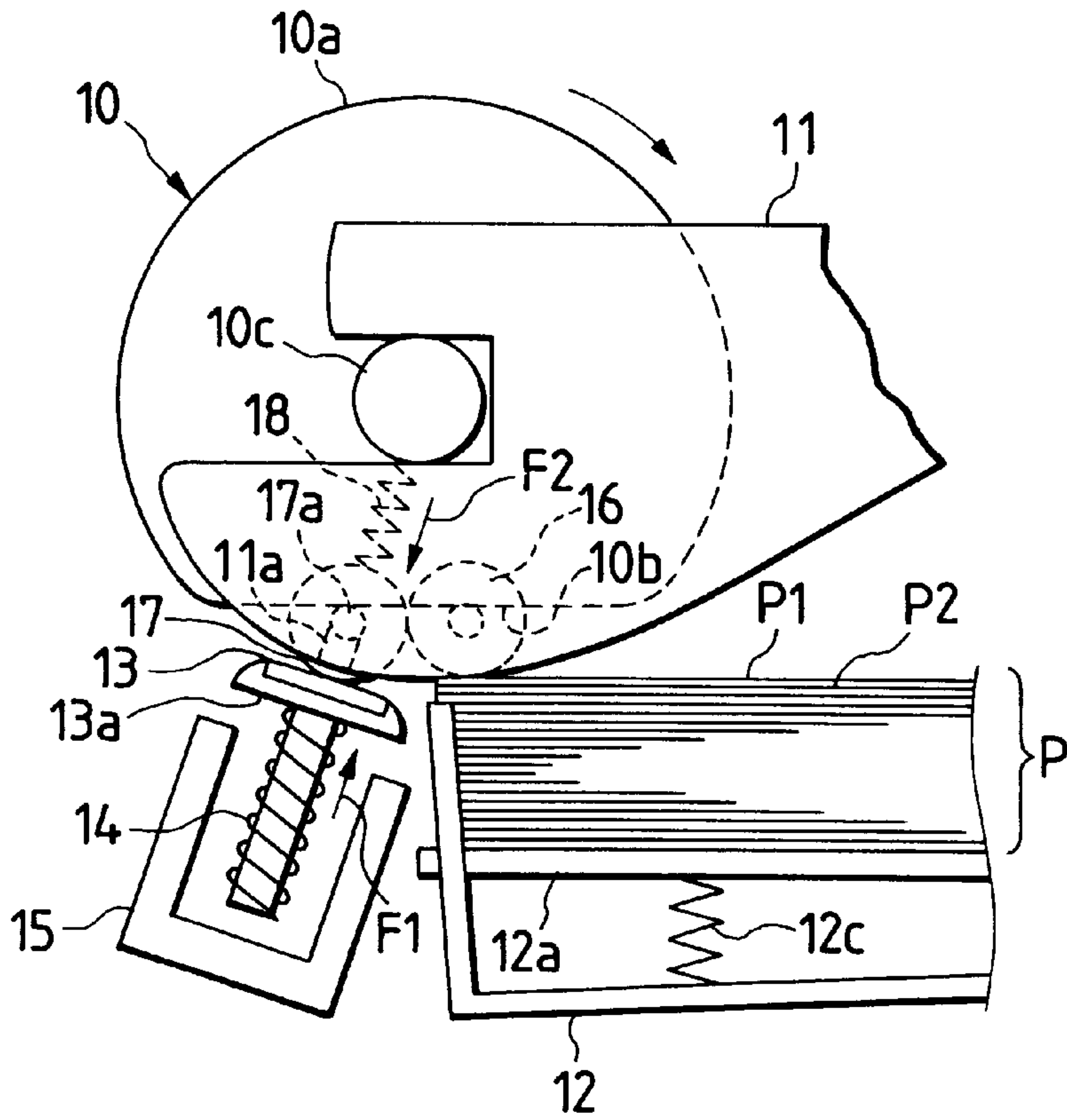
FIG. 14 RELATED ART
