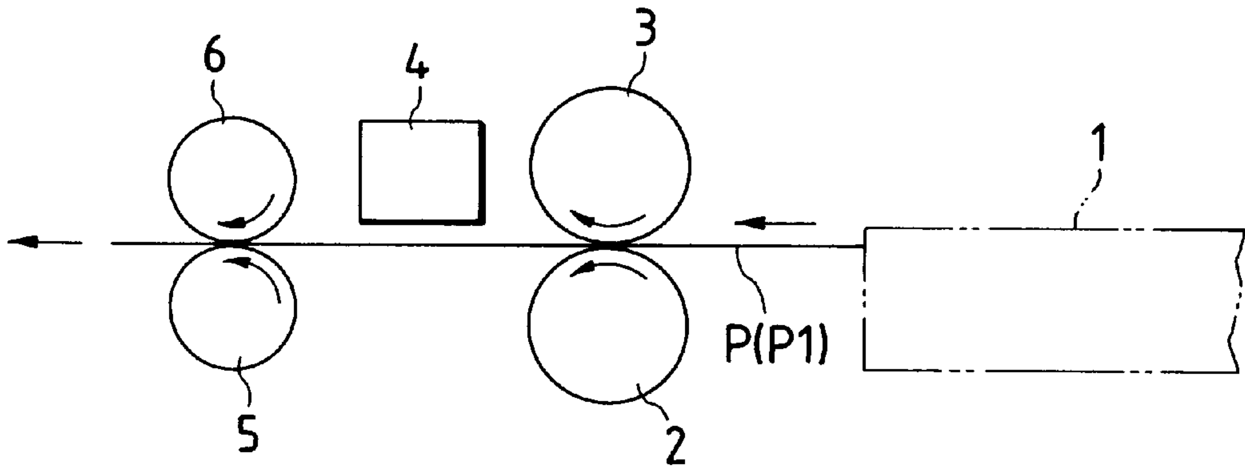
FIG. 13 RELATED ART
