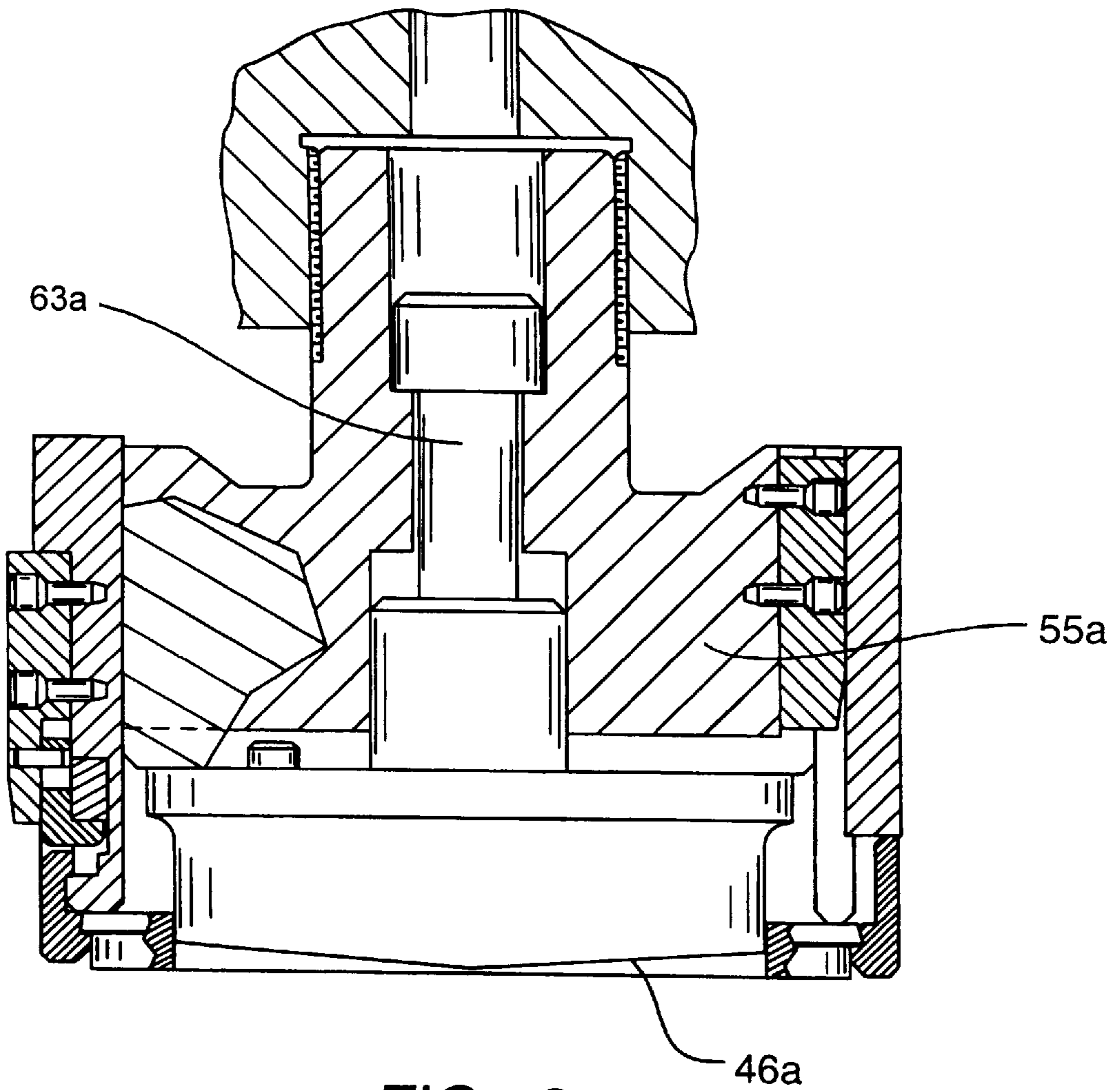
FIG. 8 (PRIOR ART)
