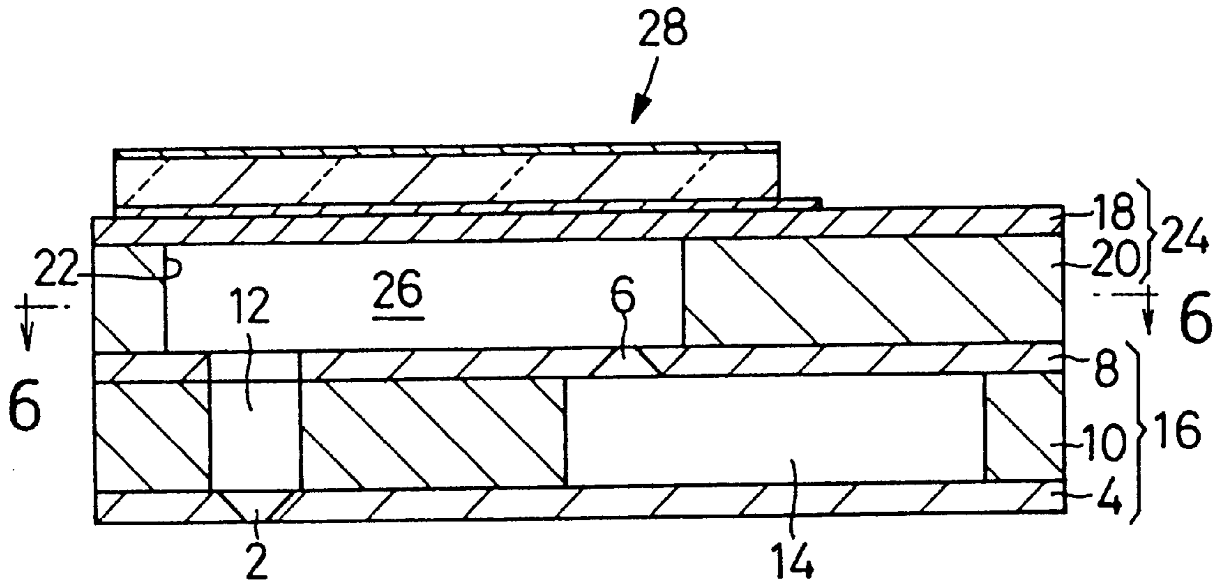
FIG. 5 PRIOR ART
