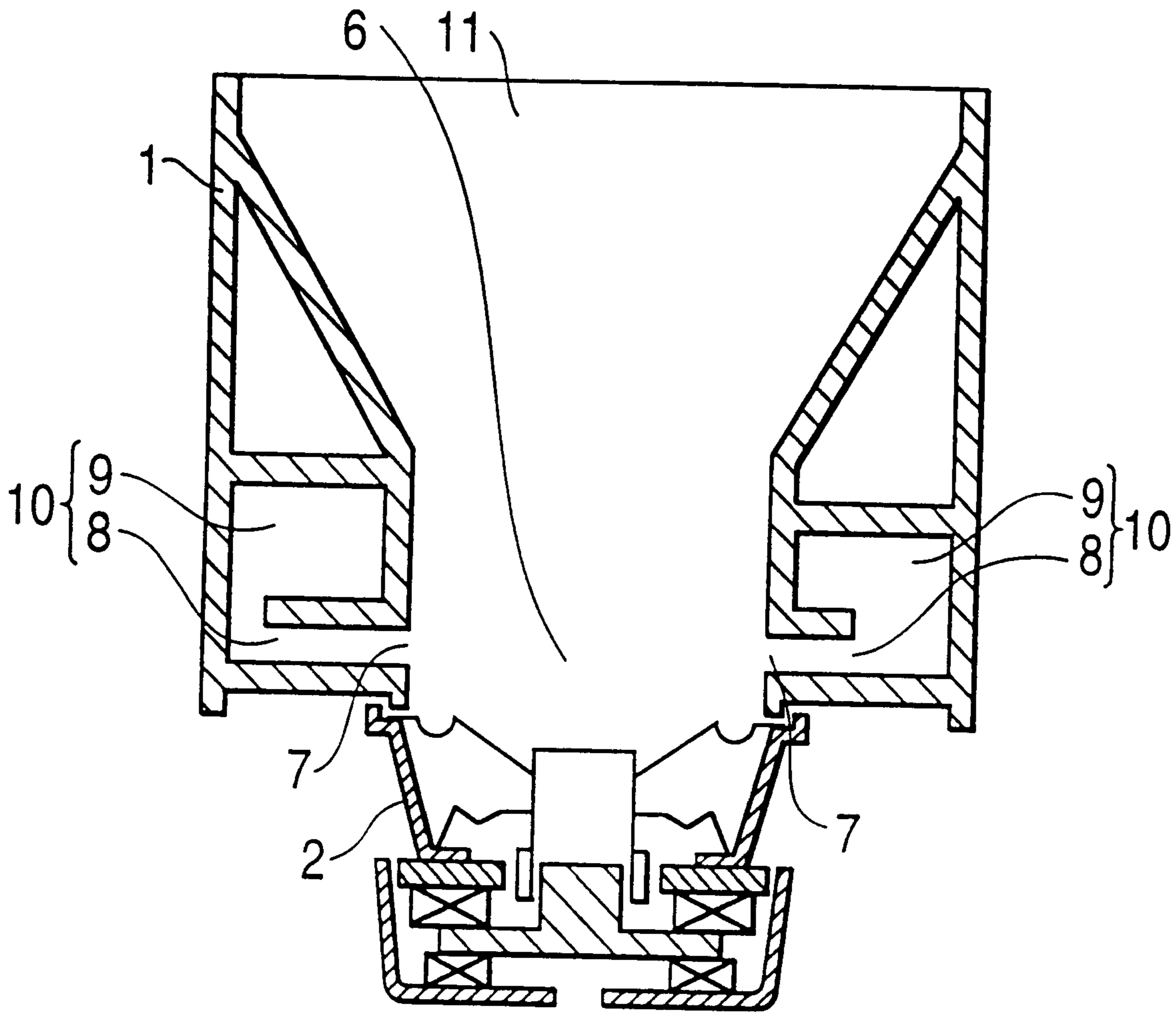
FIG. 12 (PRIOR ART)
