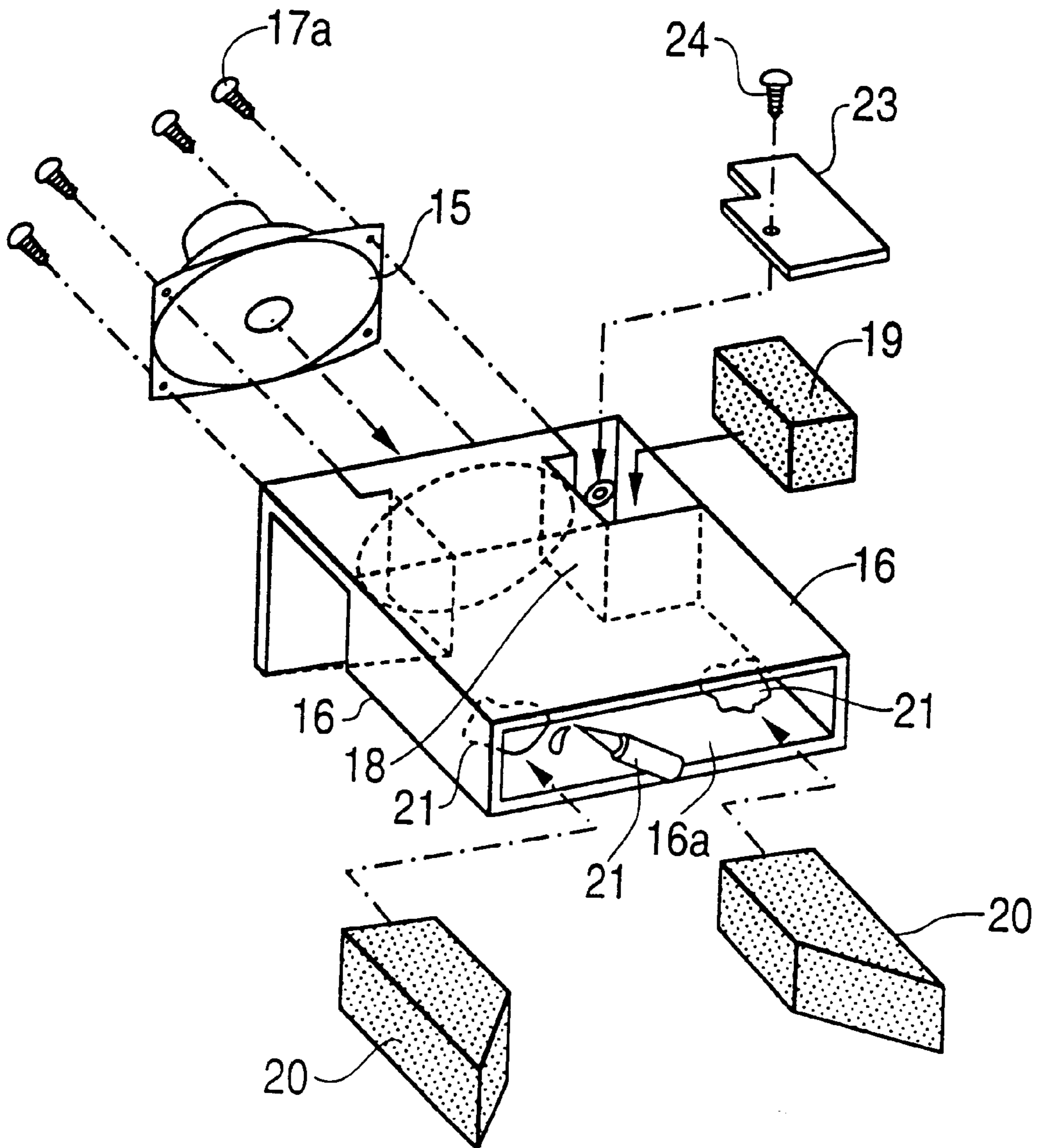
FIG. 14 (PRIOR ART)
