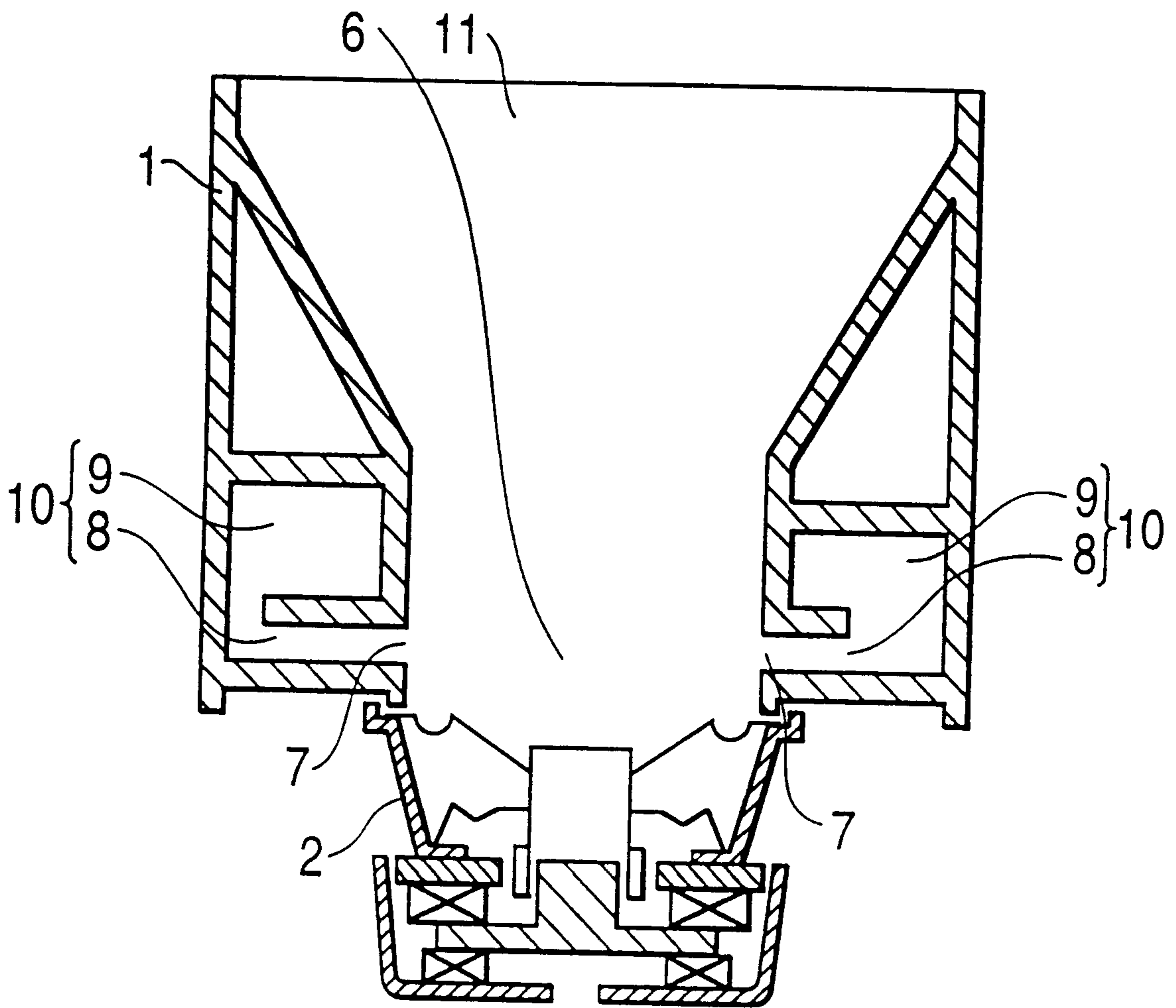
FIG. 12 (PRIOR ART)
