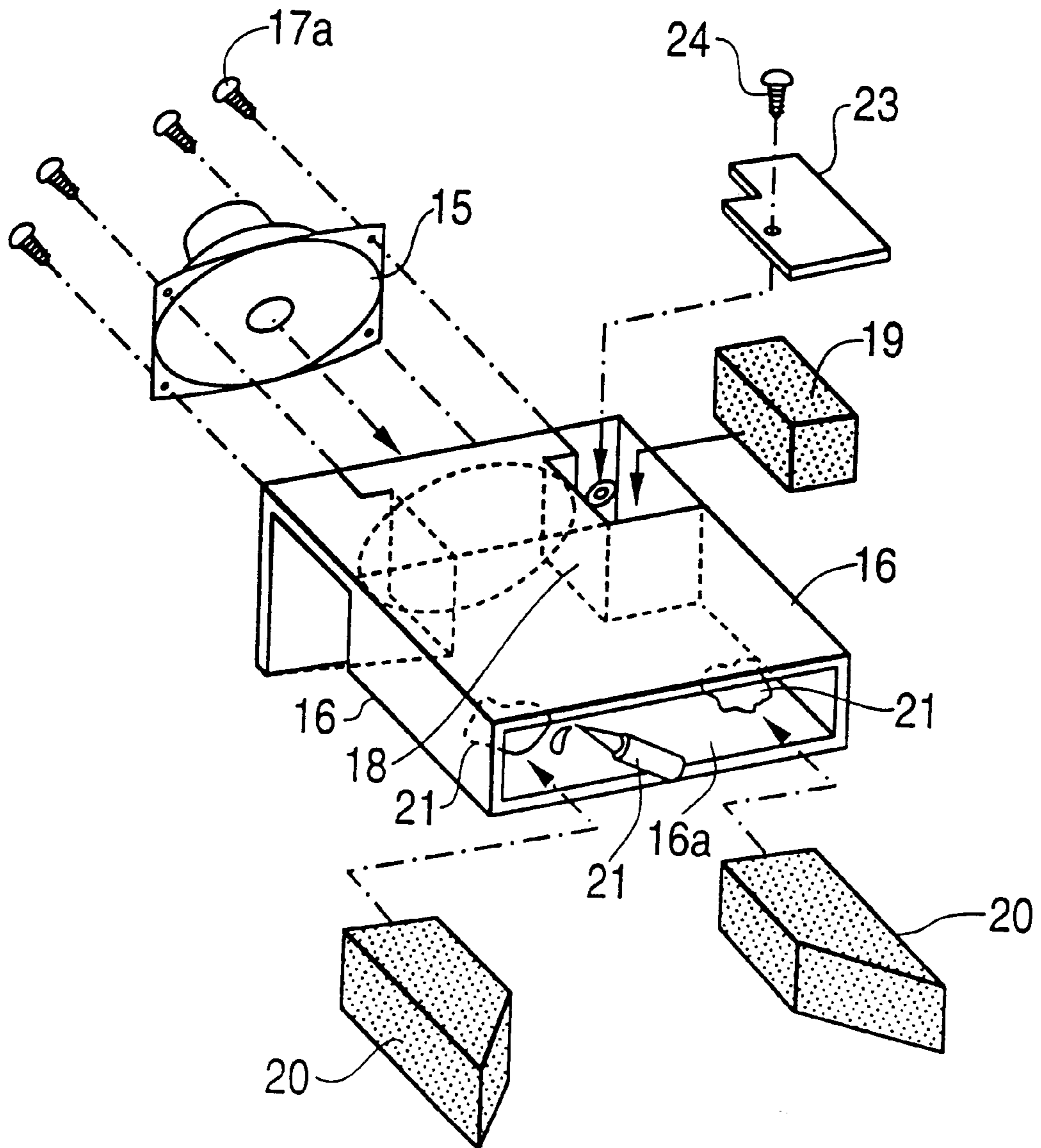
FIG. 14 (PRIOR ART)
