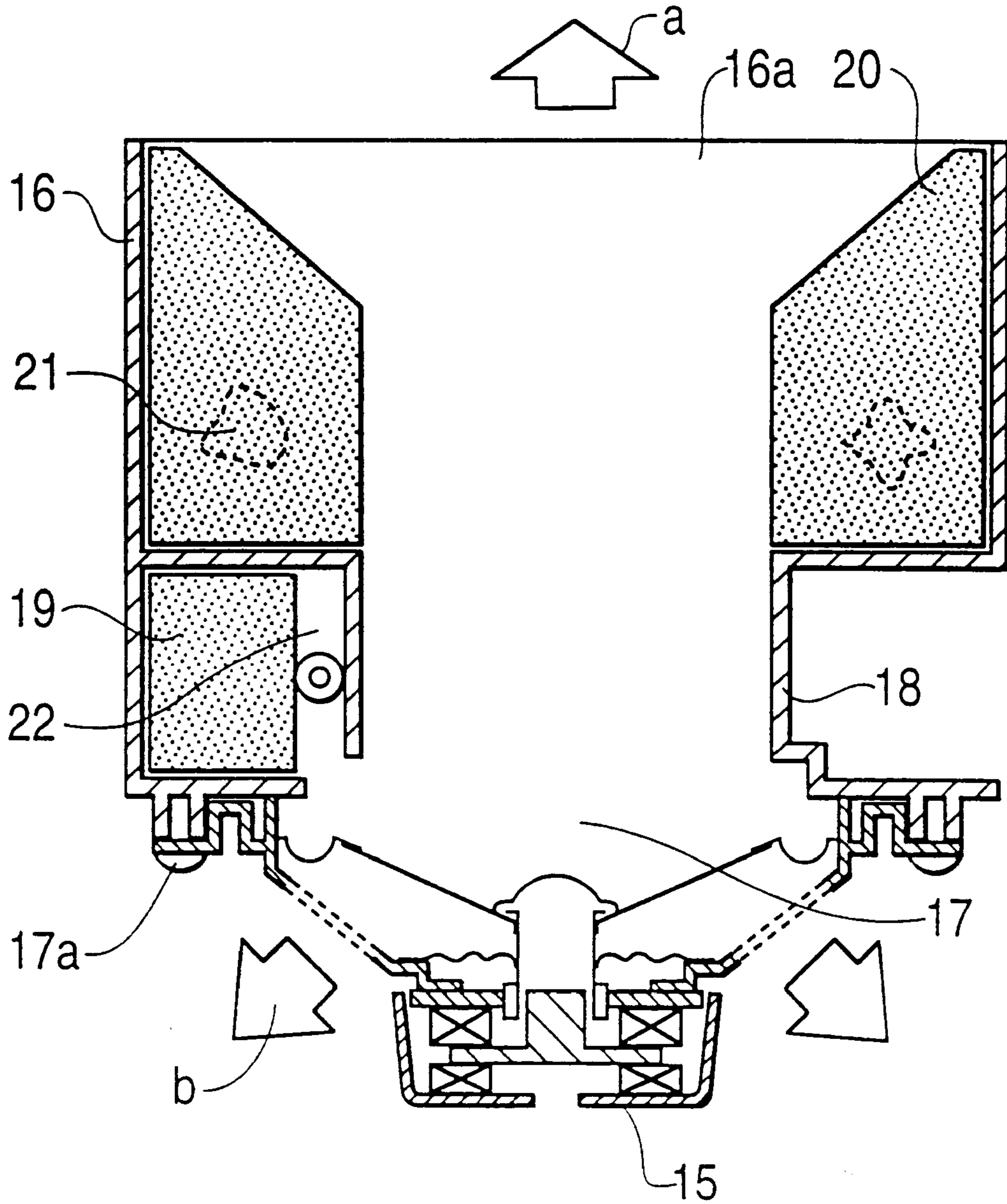
FIG. 13 (PRIOR ART)
