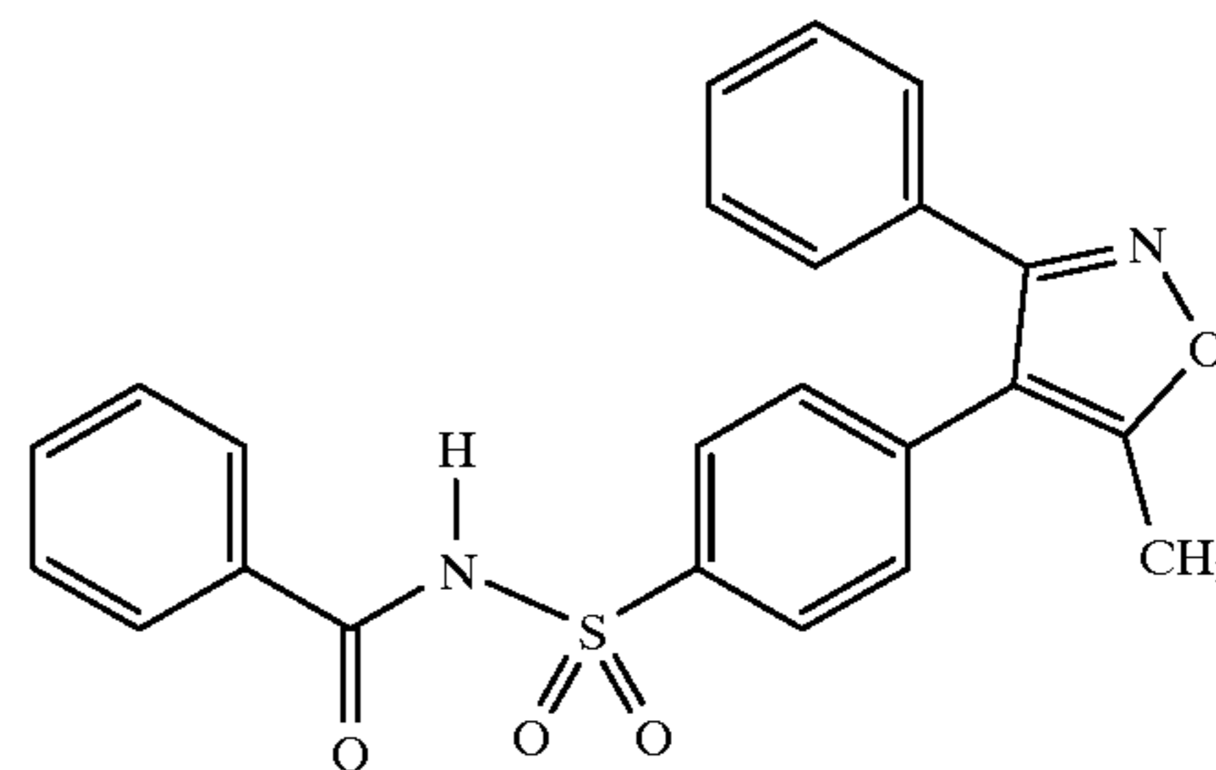
N-[[4-(5-Methyl-3-phenylisoxazol-4-yl)phenyl]sulfonyl]benzamide
