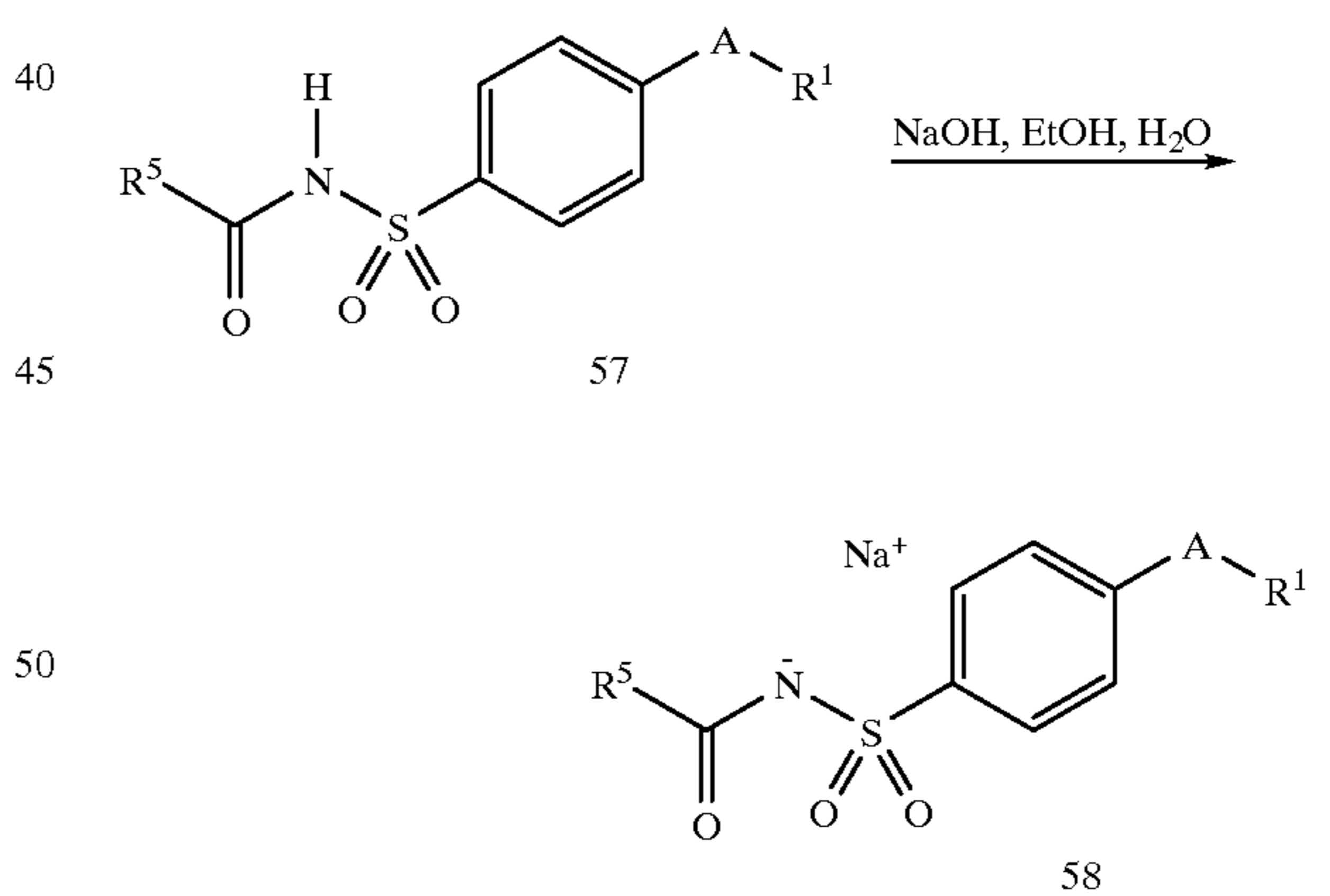
Scheme XII
