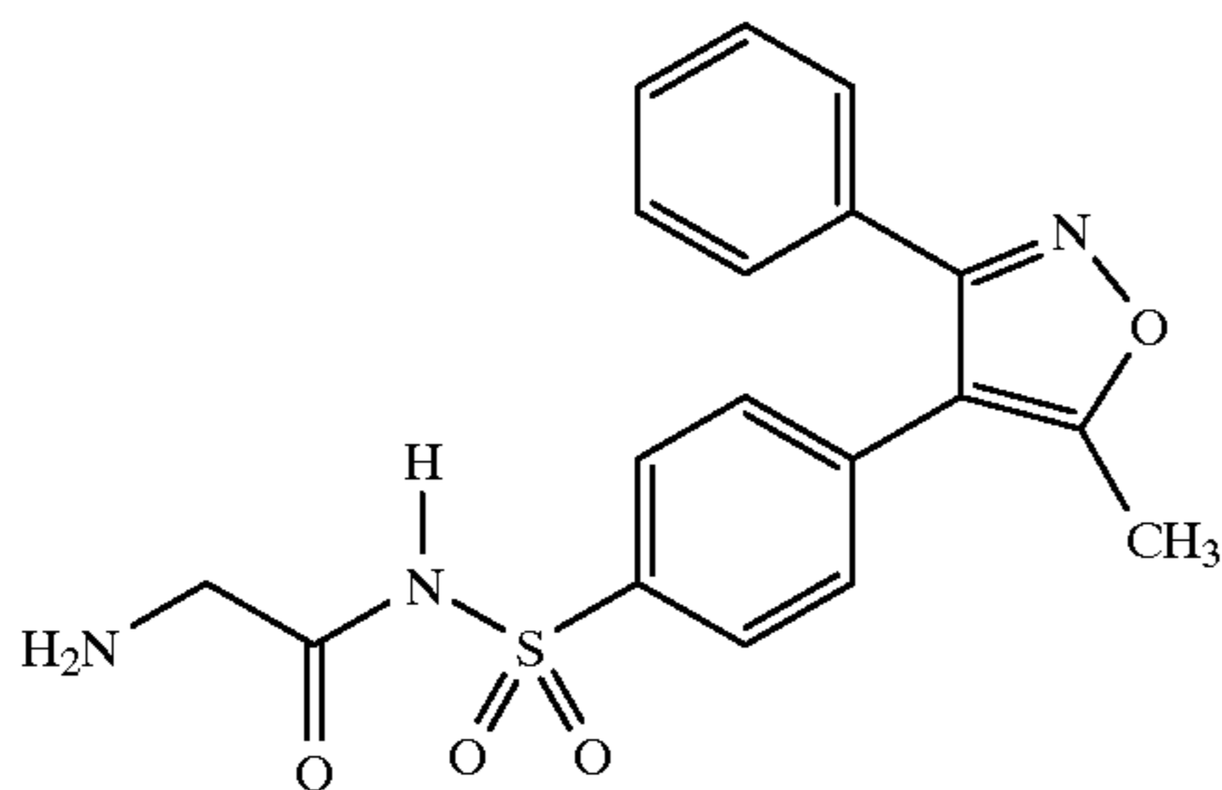
2-Amino-N-[[4-(5-methyl-3-phenylisoxazol-4-yl)phenyl]sulfonyl]acetamide
