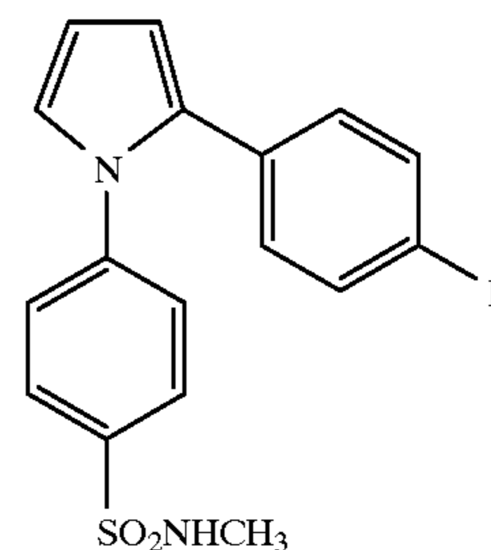
4-[2-(4-Fluorophenyl)-1H-pyrrol-1-yl]-N-methylbenzenesulfonamide
