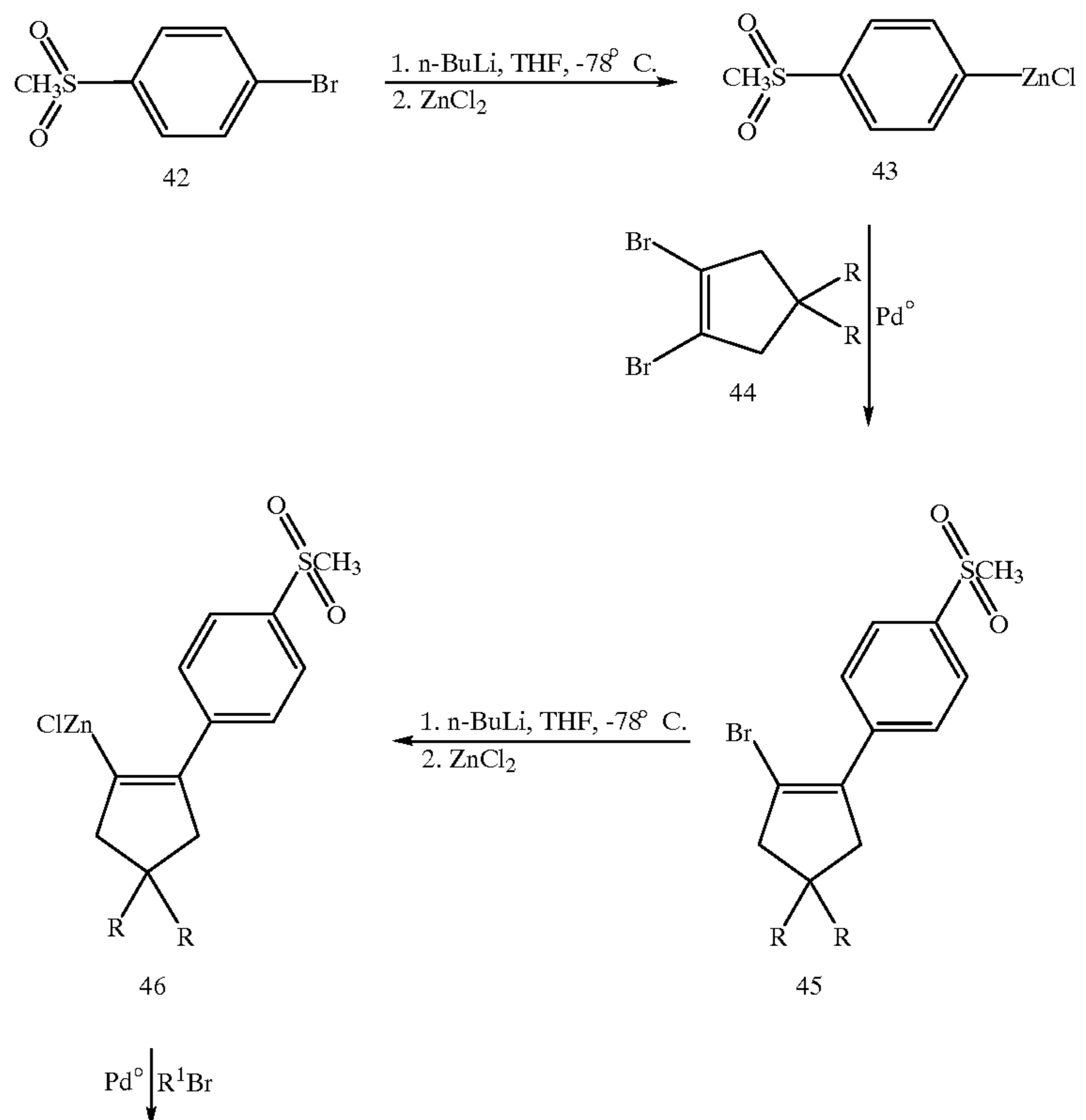
Scheme VIII
