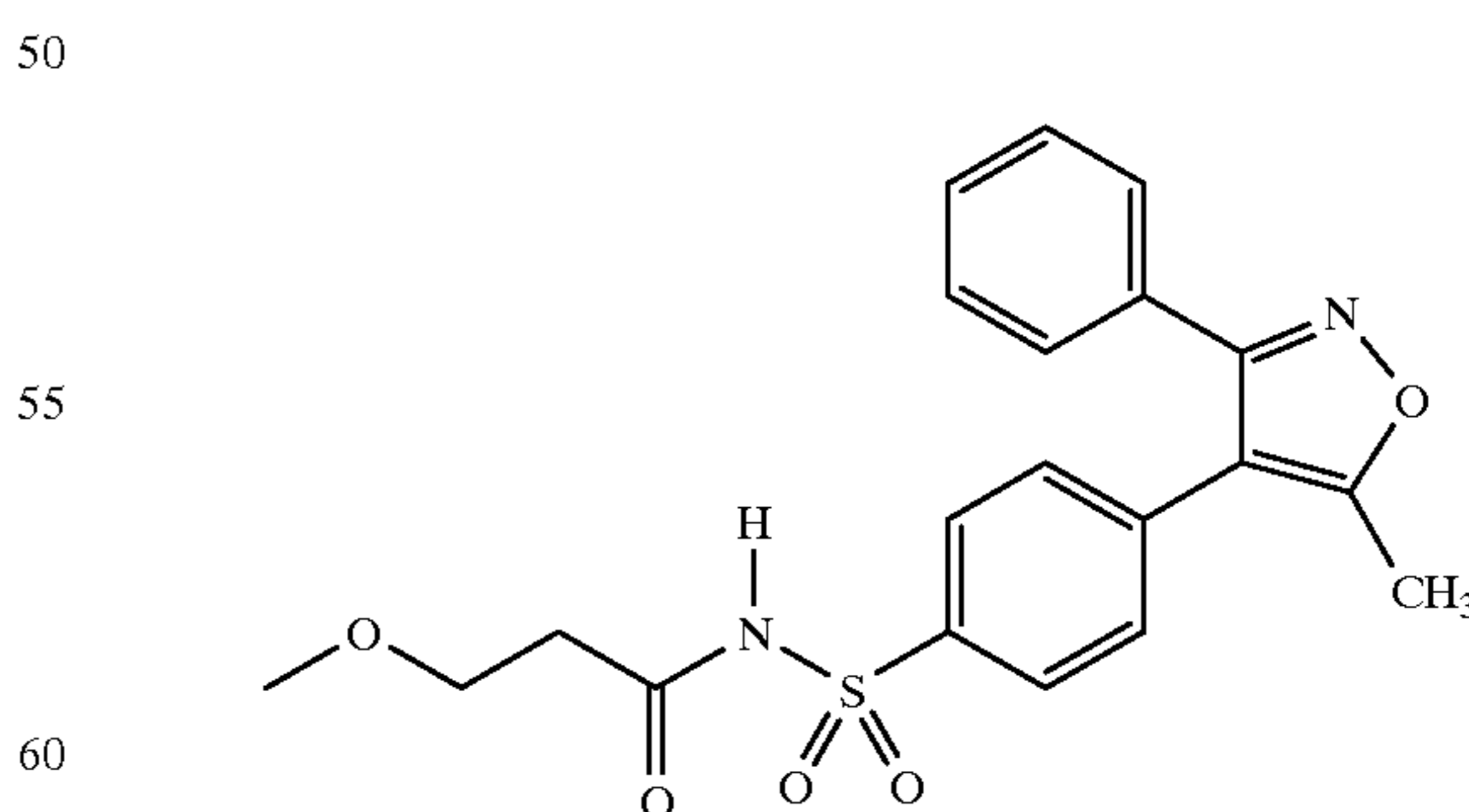
3-Methoxy-N-[[4-(5-methyl-3-phenylisoxazol-4-yl)phenyl]sulfonyl]propanamide
