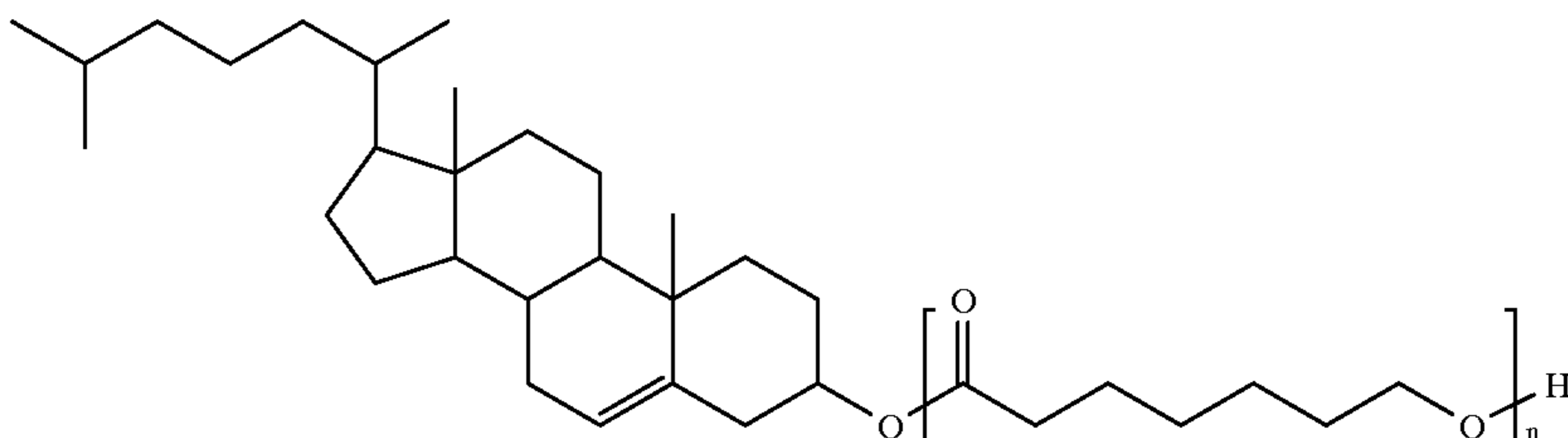
Cholesteroyl-(caprolactone) n
