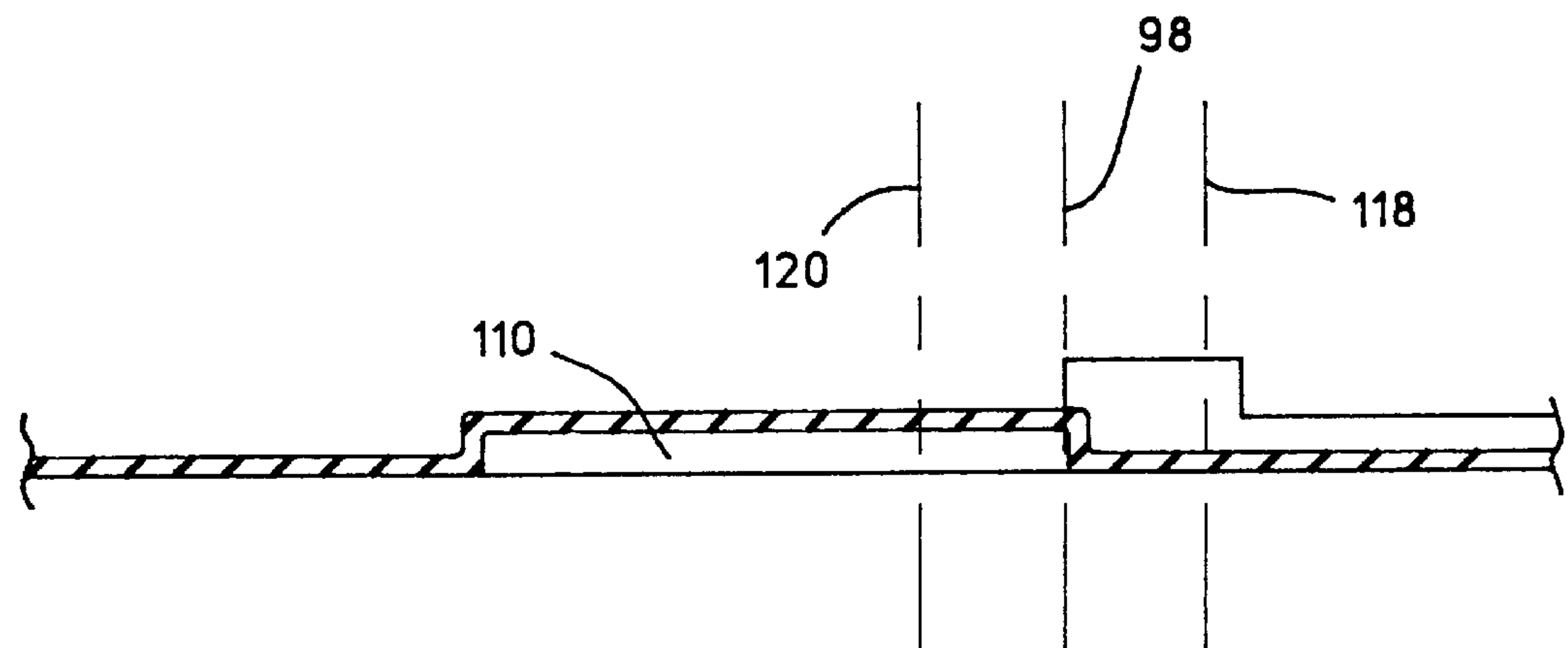
FIG. 7G (Prior Art)
