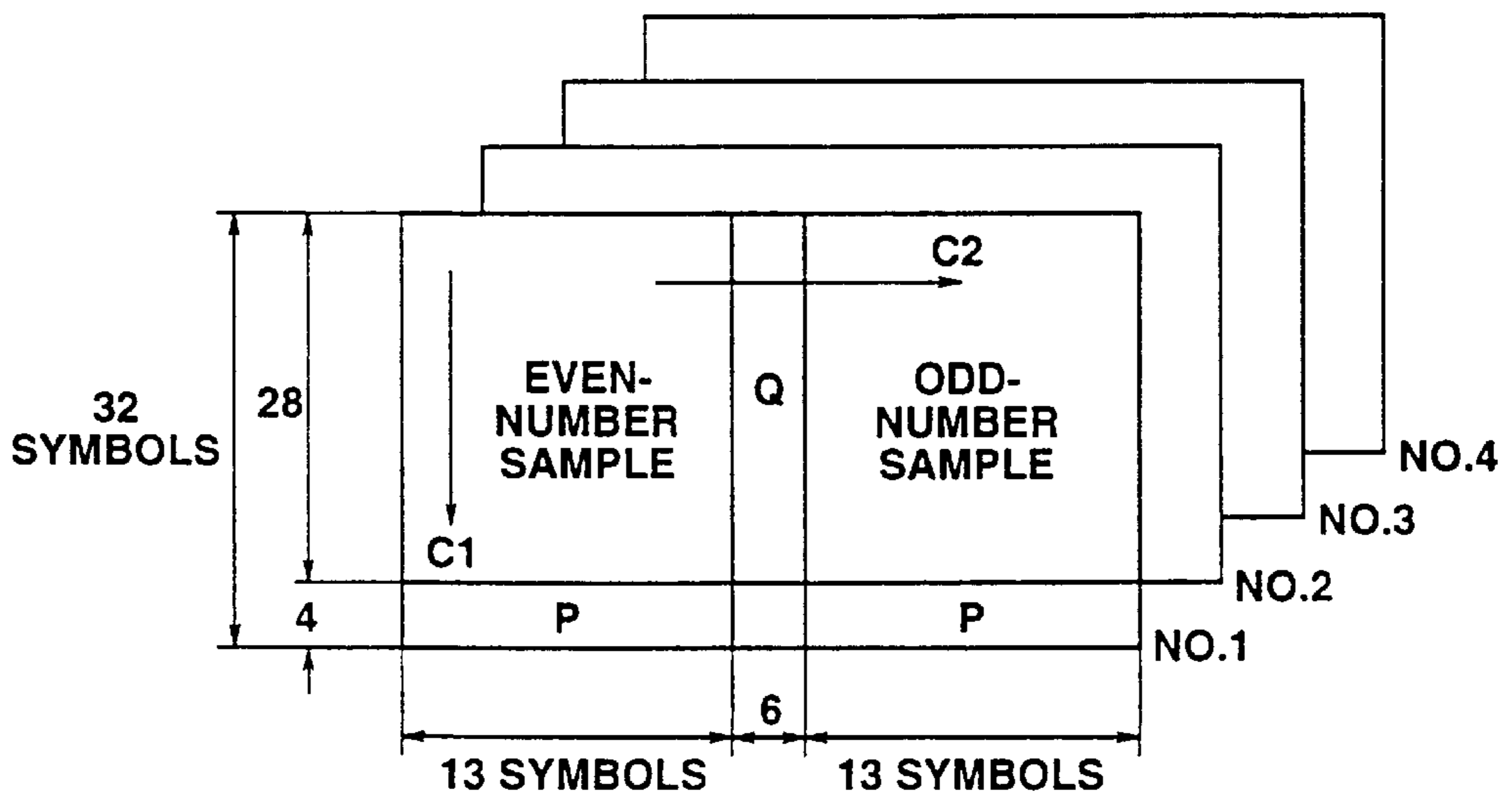
FIG.4 (PRIOR ART)
