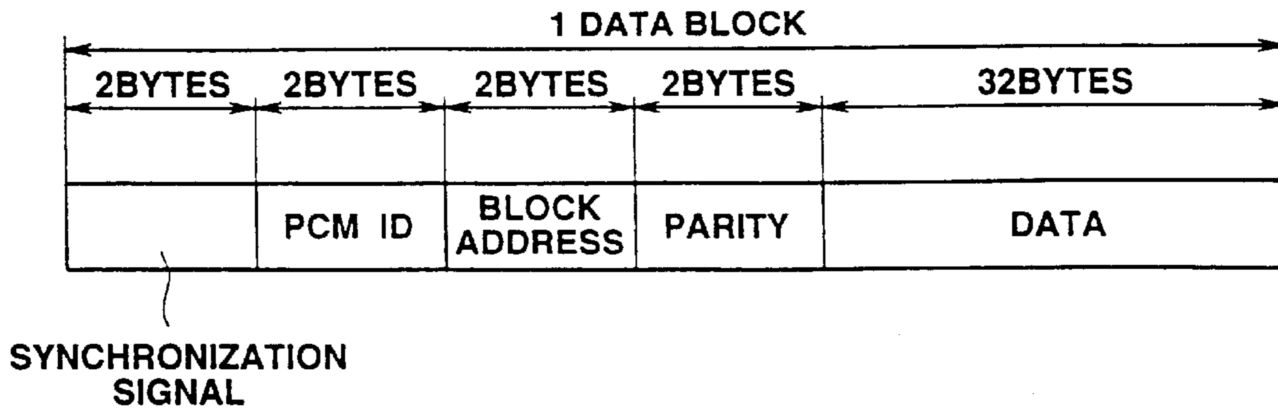
FIG.2 (PRIOR ART)
