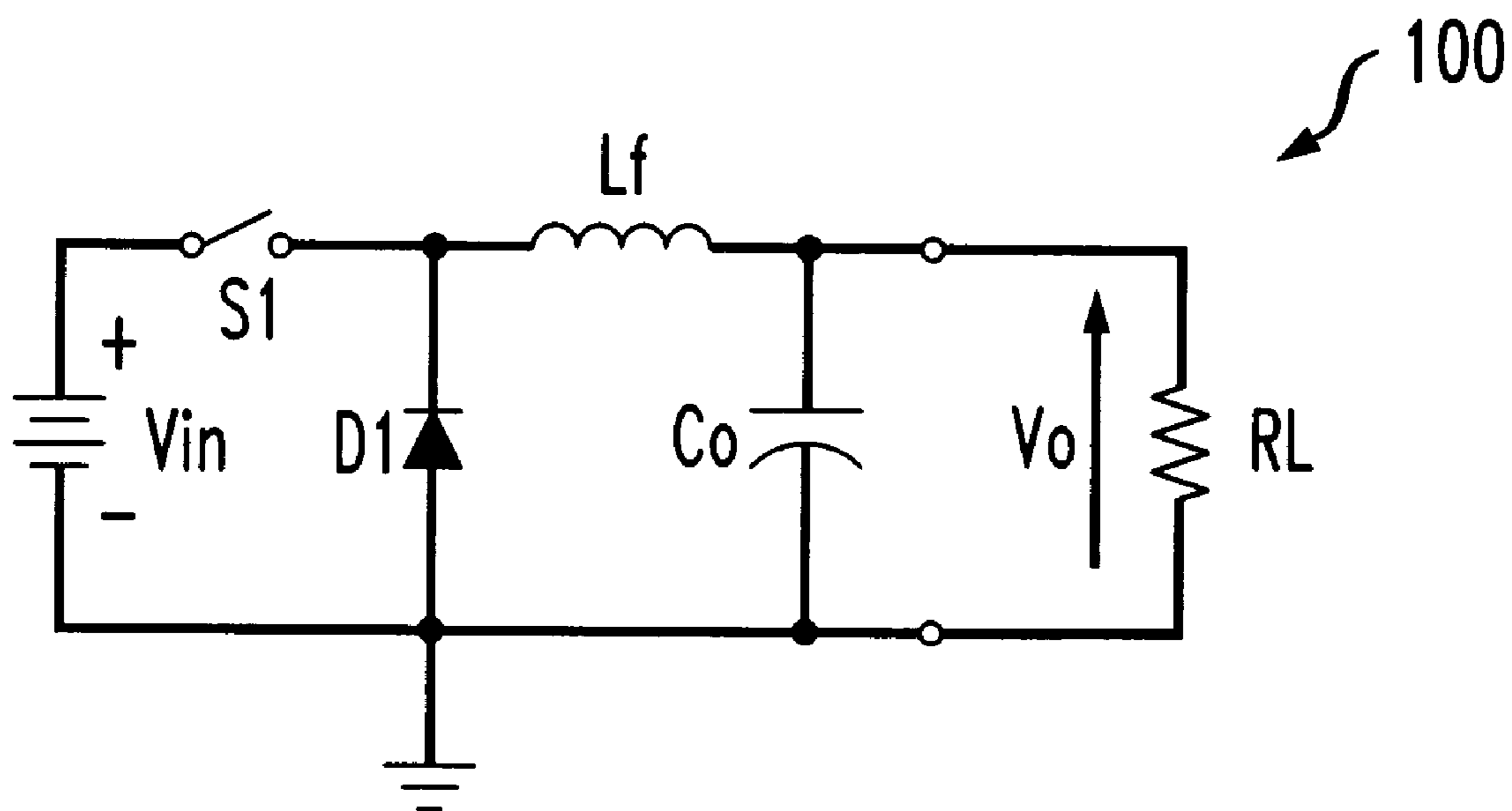
FIG. 1 (PRIOR ART)
