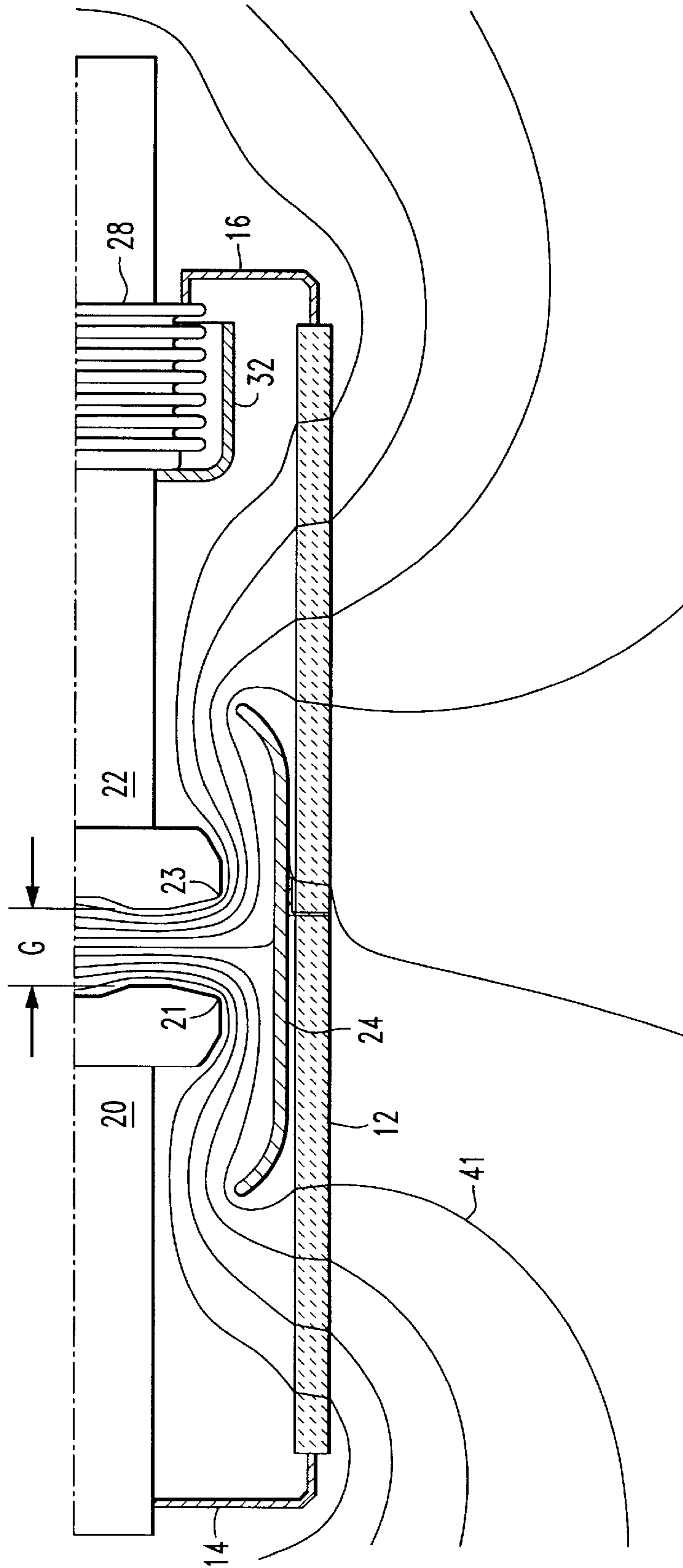
FIG. 2 PRIOR ART
