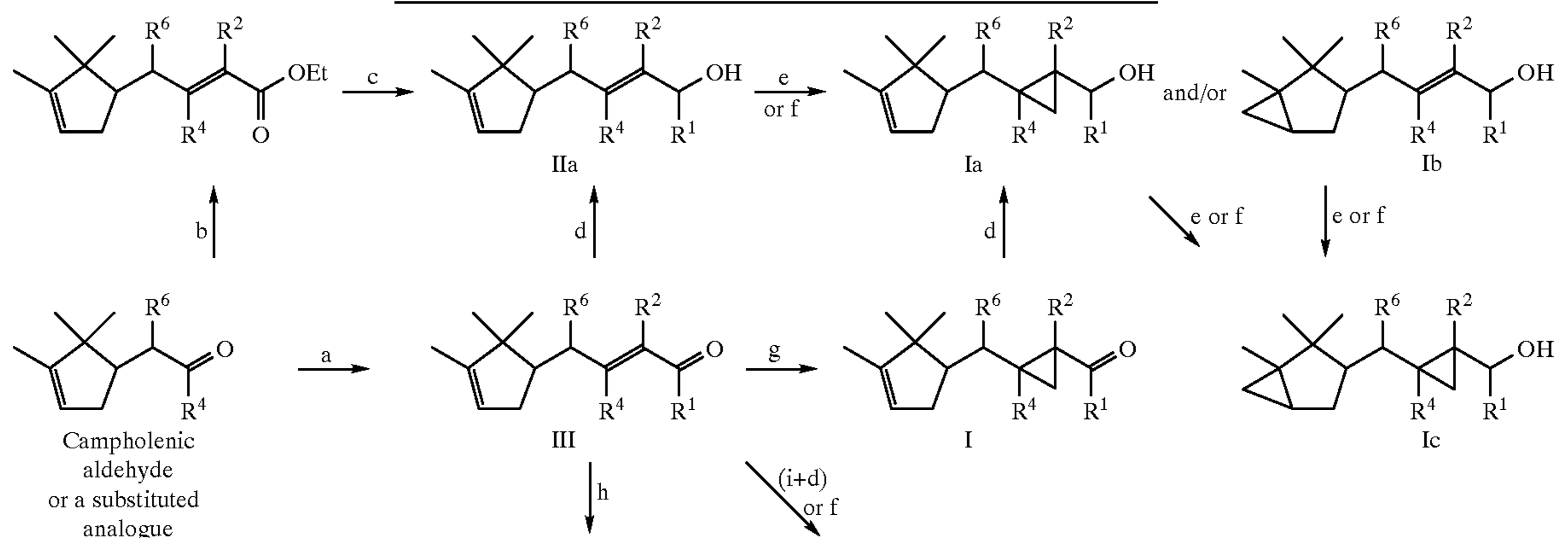
Scheme 1. Access to cyclopropanated campholenic aldehyde derivatives Ia-e
