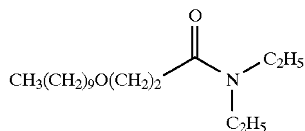
3-(Decyloxy)-N,N-diethylpropanamide
