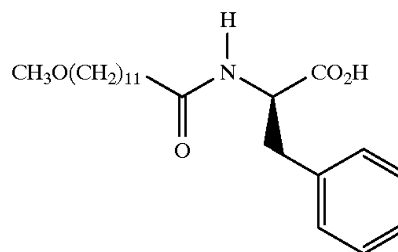
N-(12-Methoxy-1-oxododecyl)-D-phenylalanine
