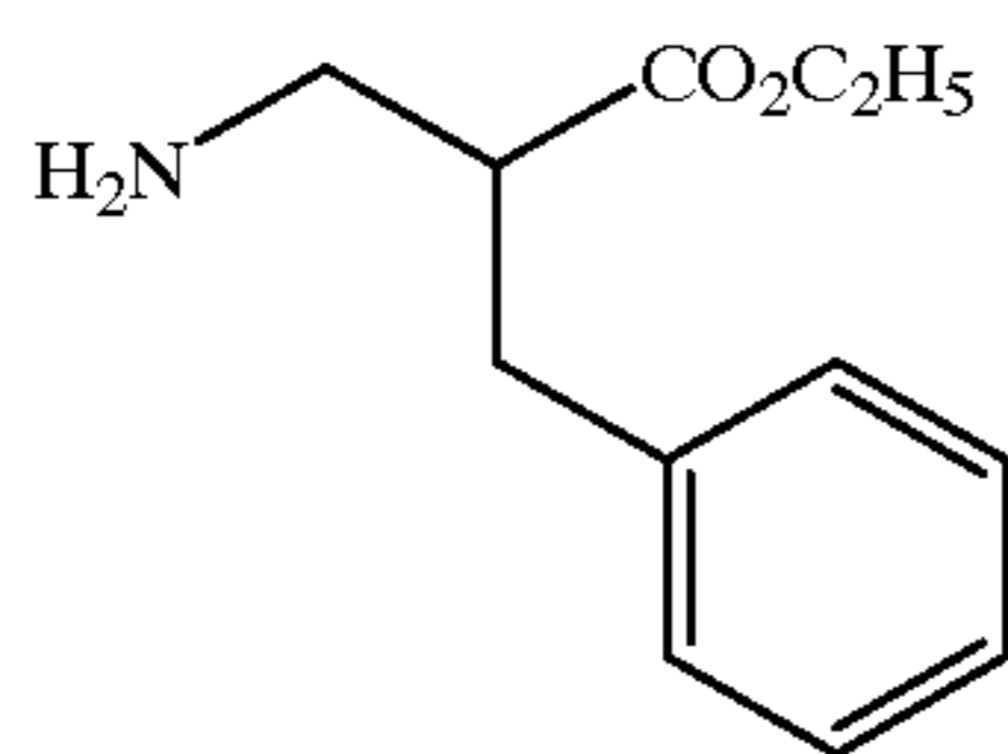
Ethyl 3-Amino-2R-(phenylmethyl)propanoate
