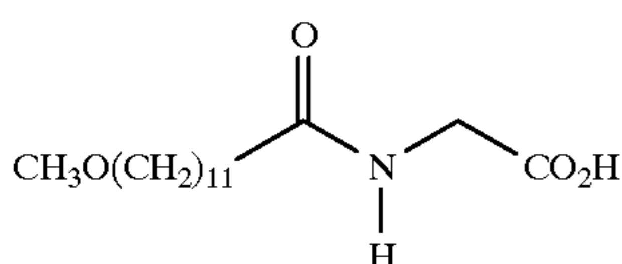
N-(12-Methoxy-1-oxododecyl)glycine
