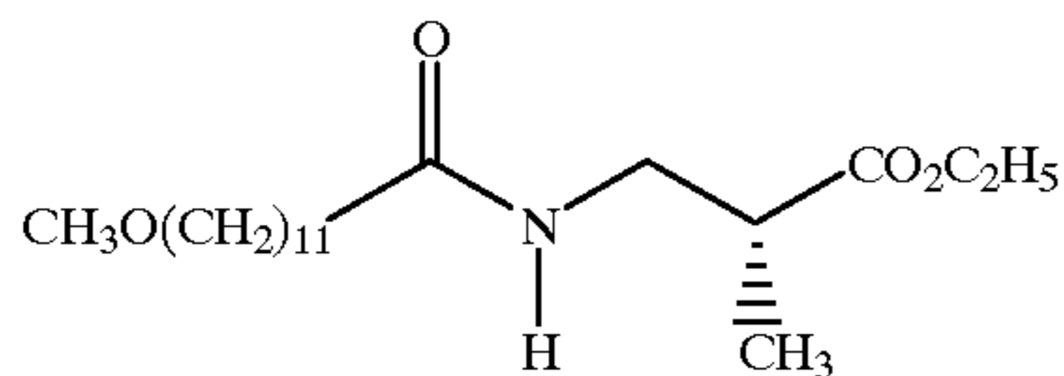
Ethyl 3-[[[(12-methoxy-1-oxododecyl)amino]-2R-methyl]propanoate
