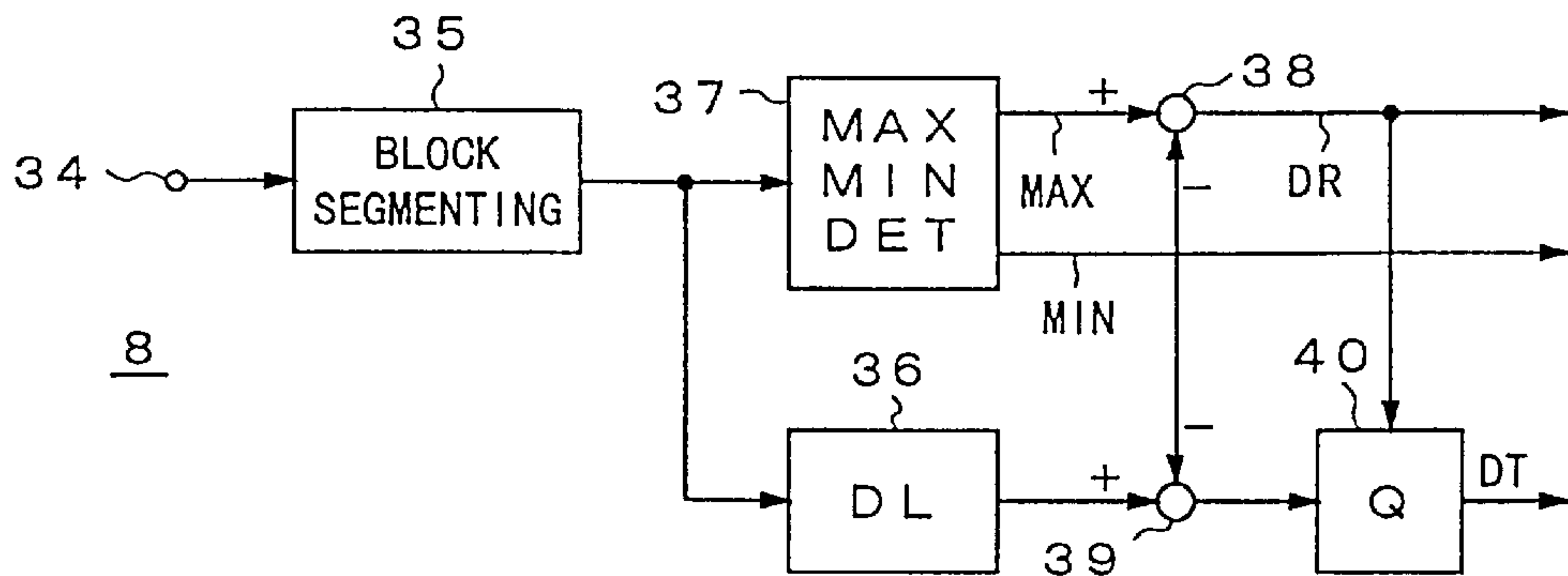
Fig. 5 PRIOR ART
