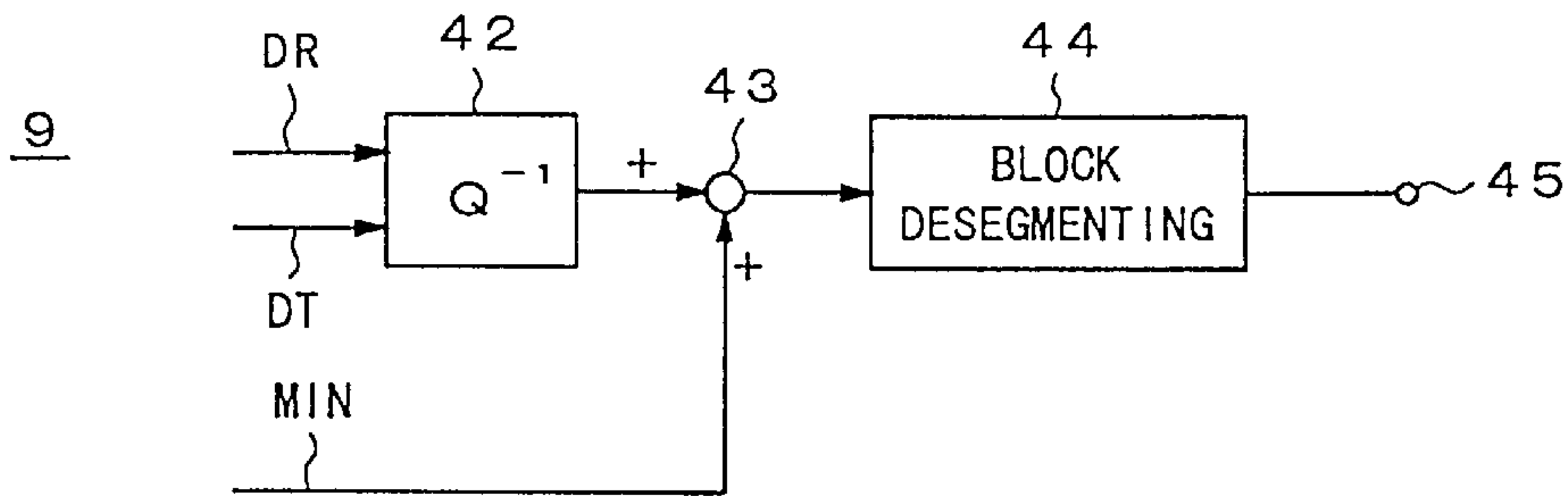
Fig. 6 PRIOR ART
