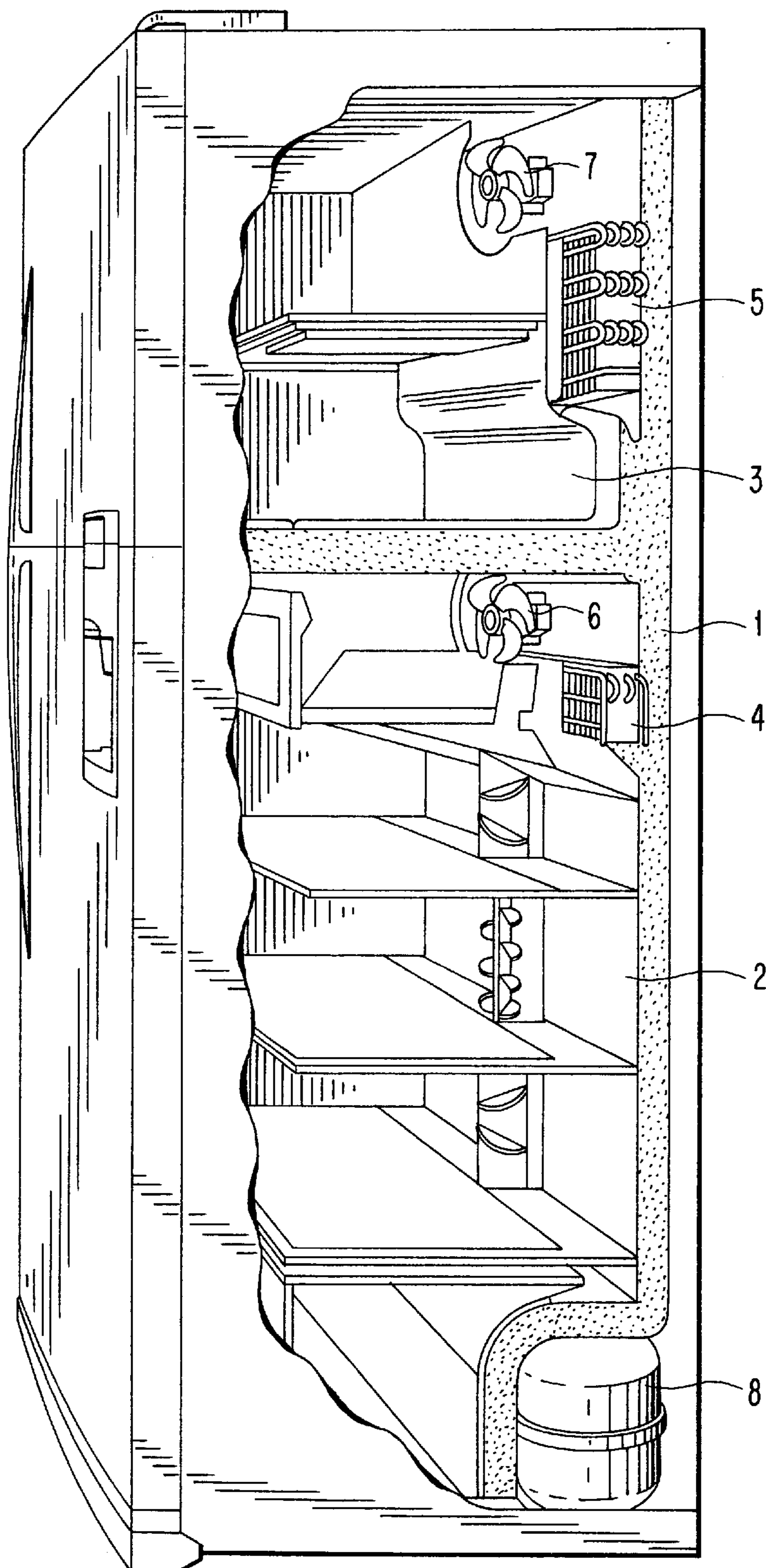
FIG. 1 (PRIOR ART)
