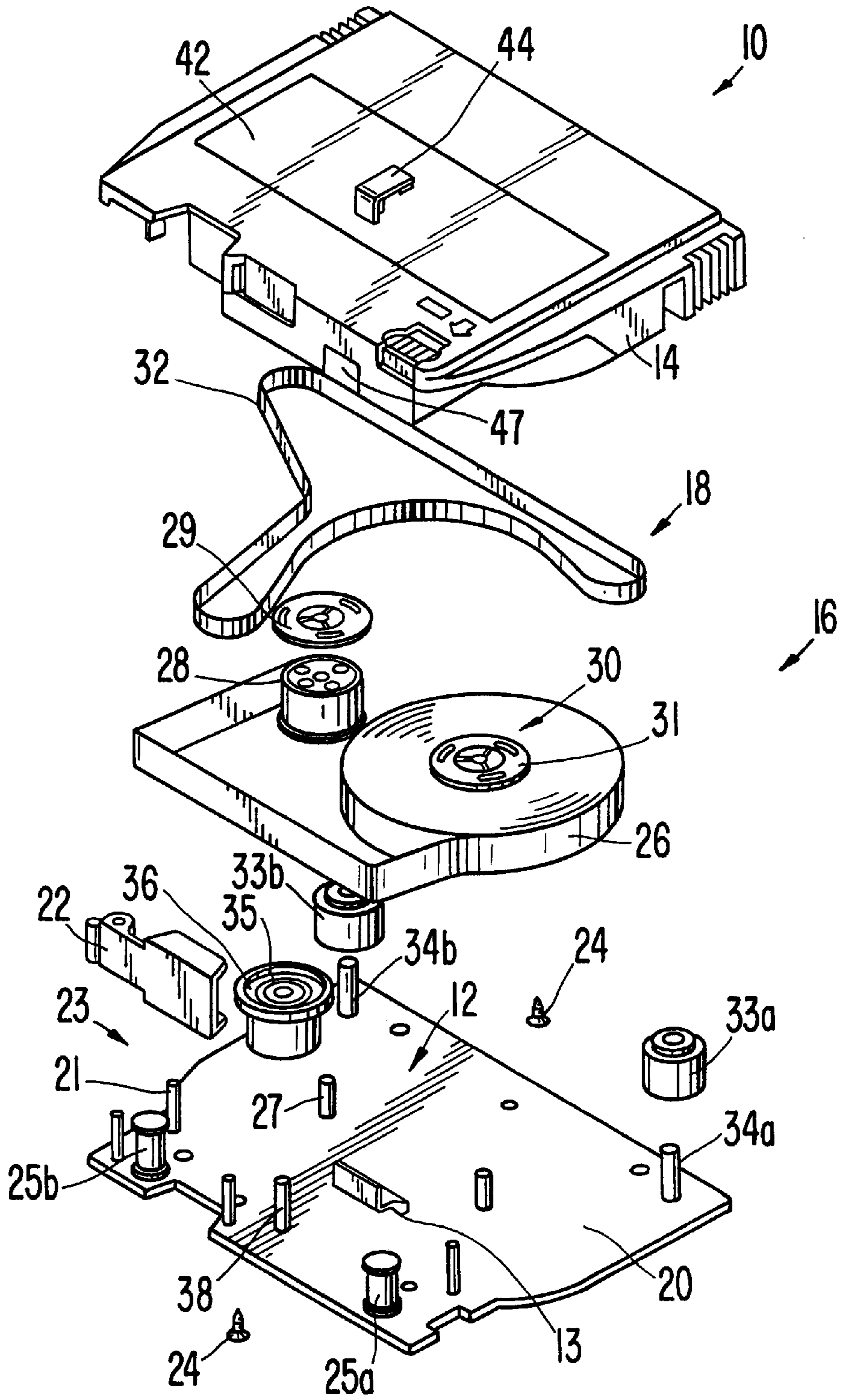
FIG. 1 (PRIOR ART)
