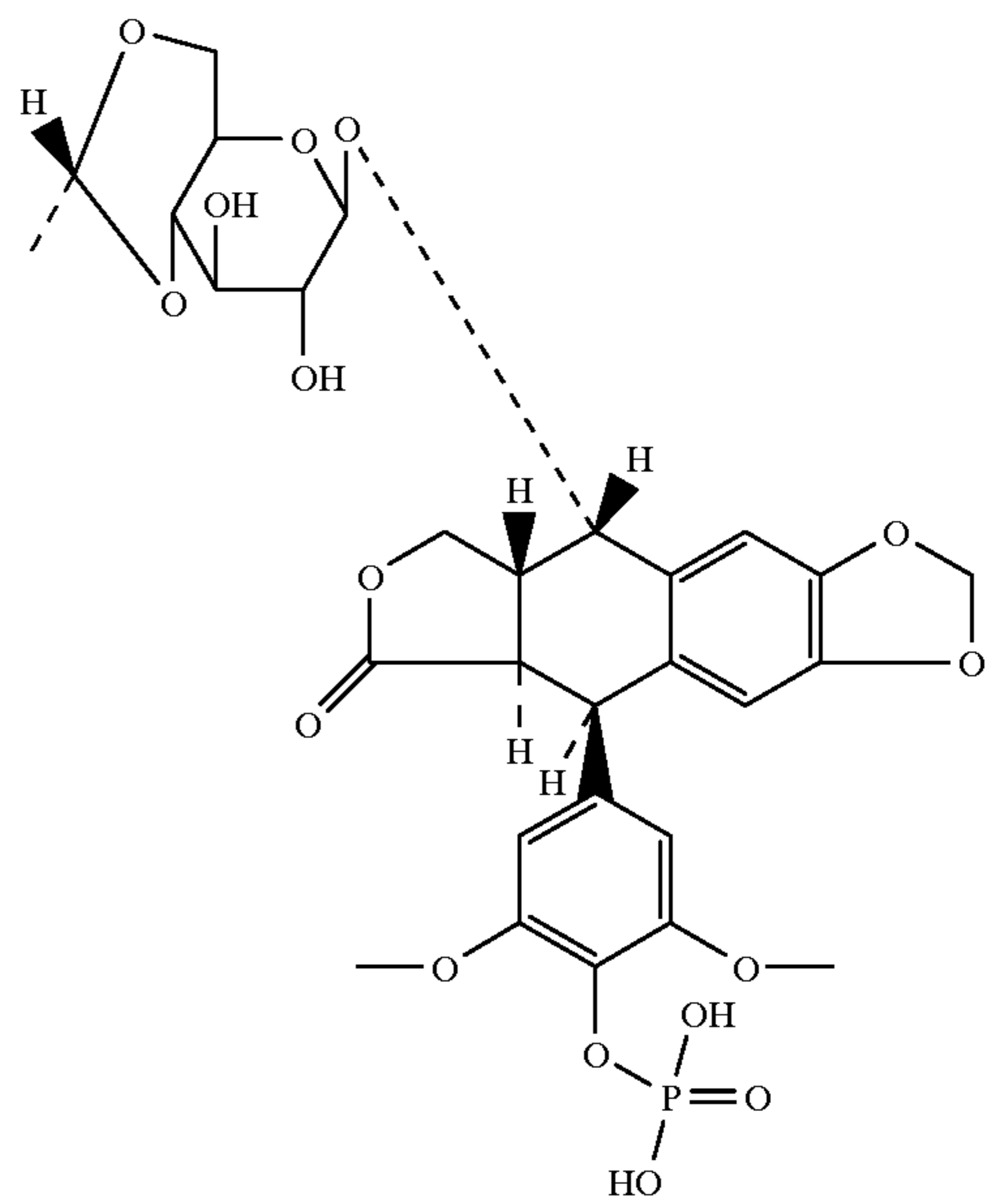
Etoposide Phosphate
