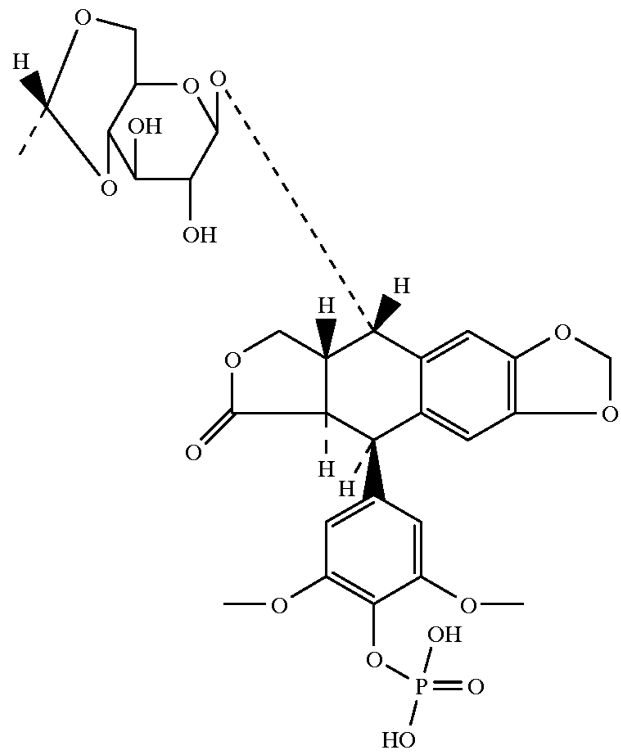
Etoposide Phosphate
