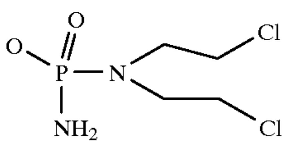
Phosphoramidate Mustard
