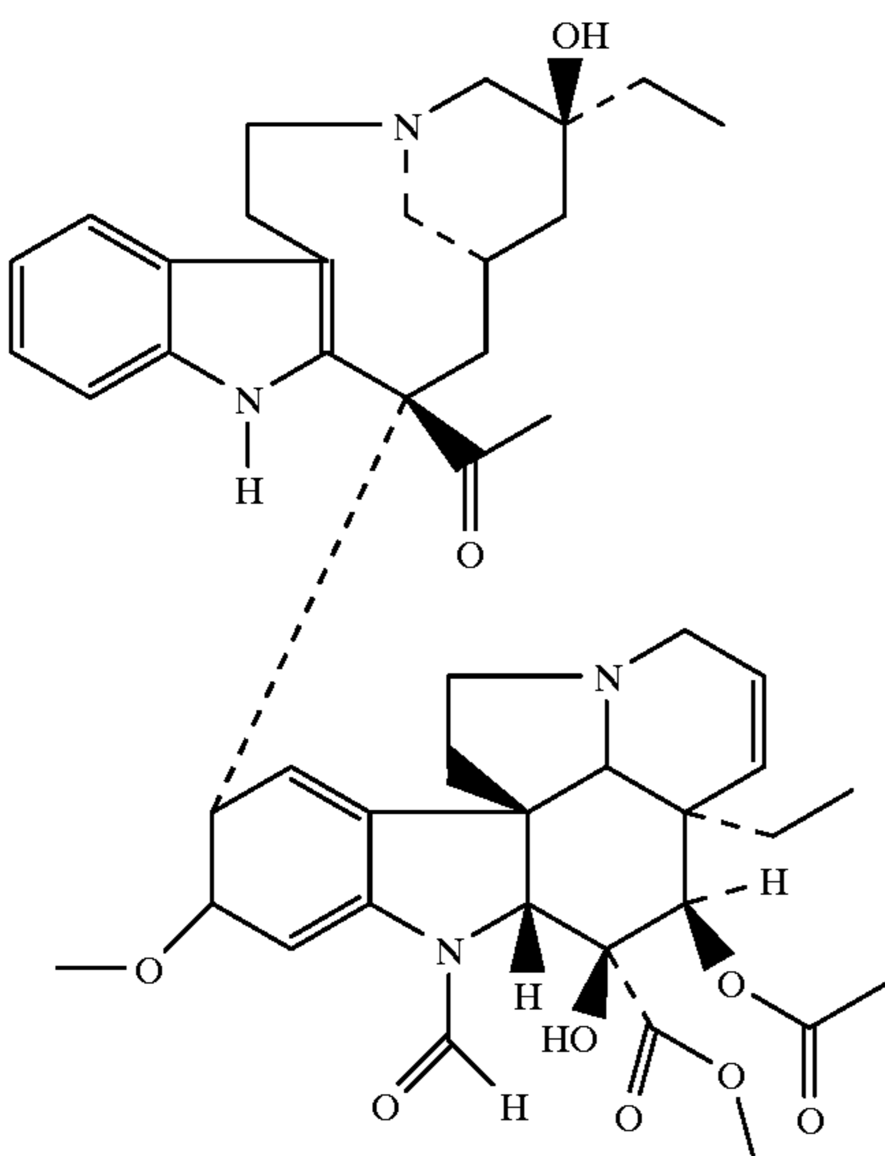
Vincristine
