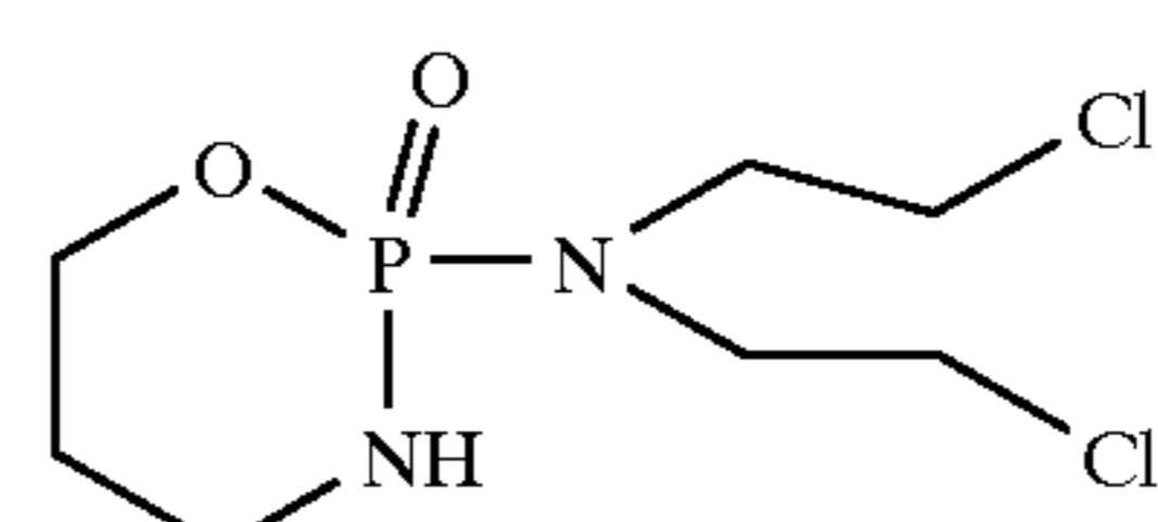
Cyclophosphamide
