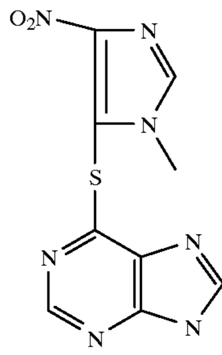
Azathioprine
