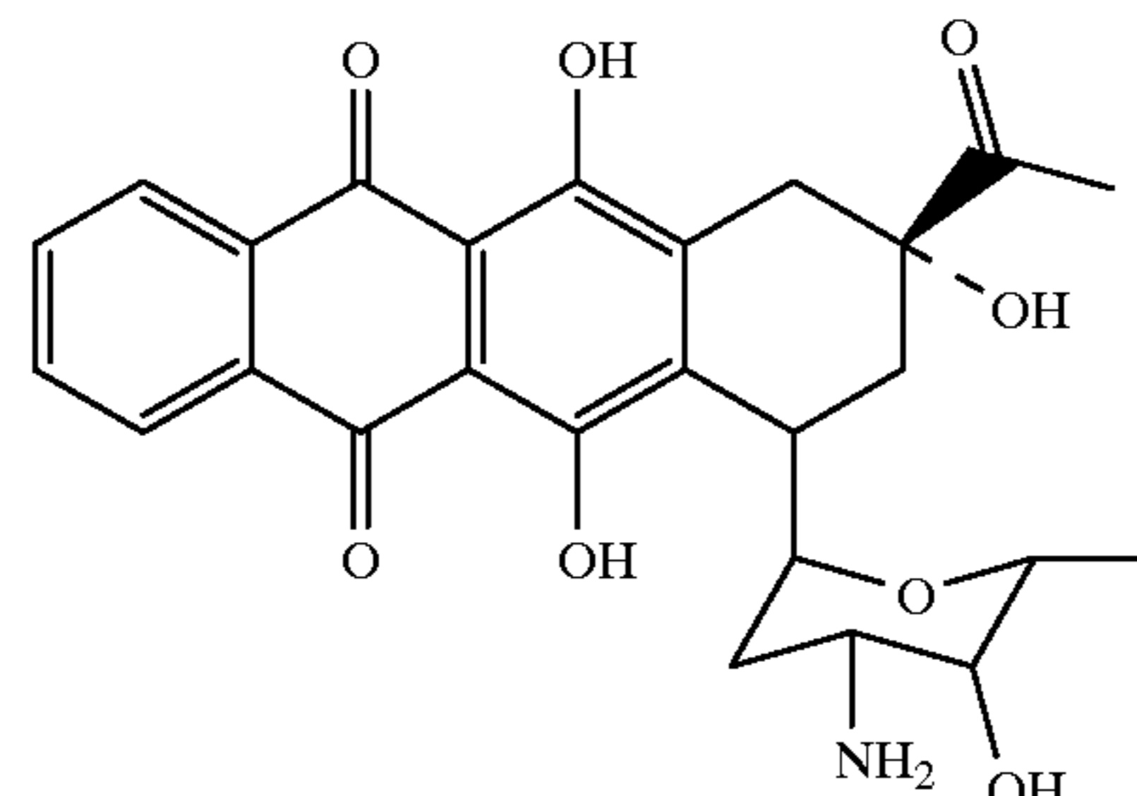
Idarubicin
