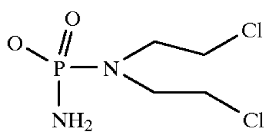
Phosphoramidate Mustard
