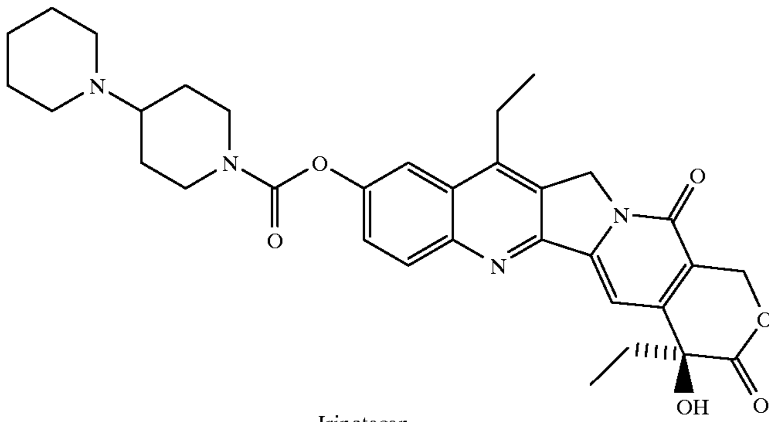
Irinotecan
