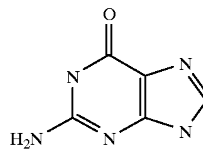
Guanine
