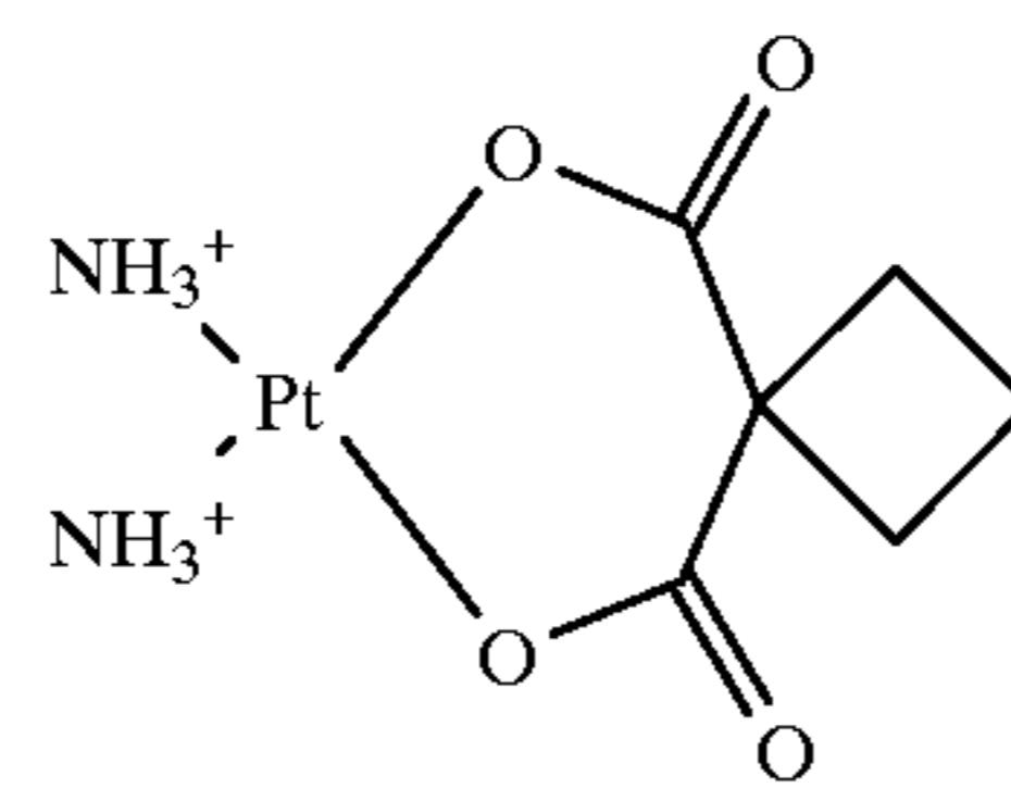
Carboplatin
