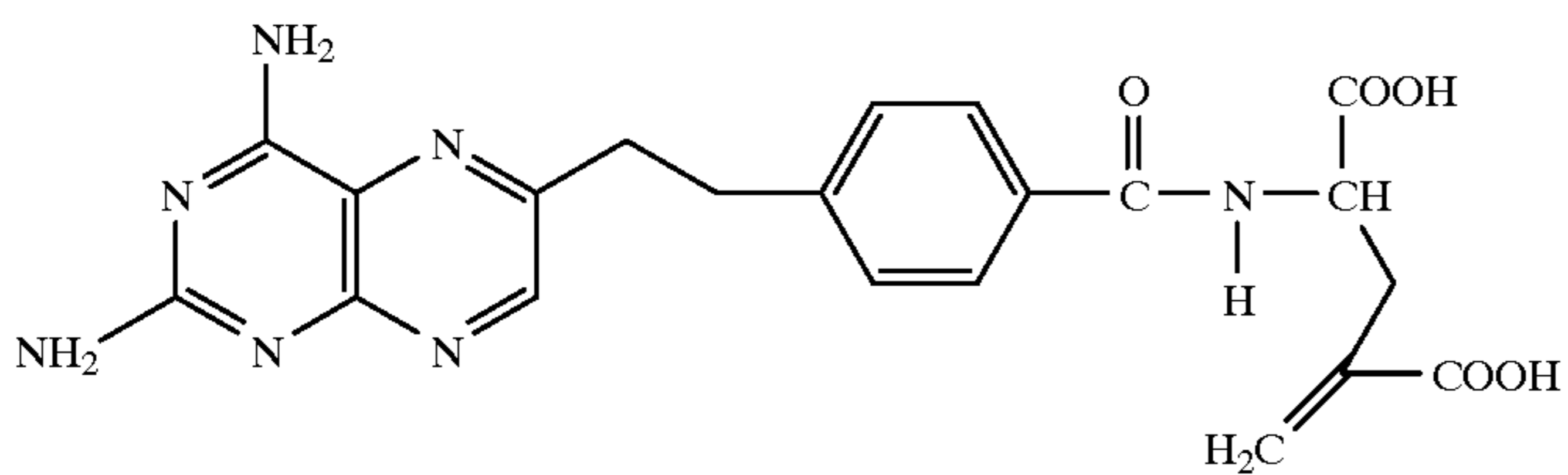
\gamma -methylene-10-deaza aminopterin (MDAM)
