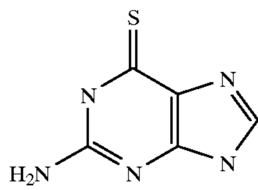
6-Thioguanine
