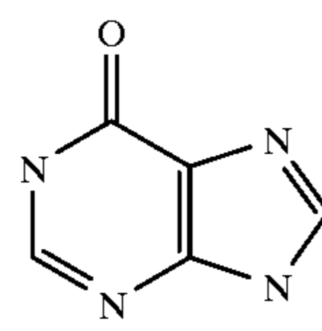
Hypoxanthine
