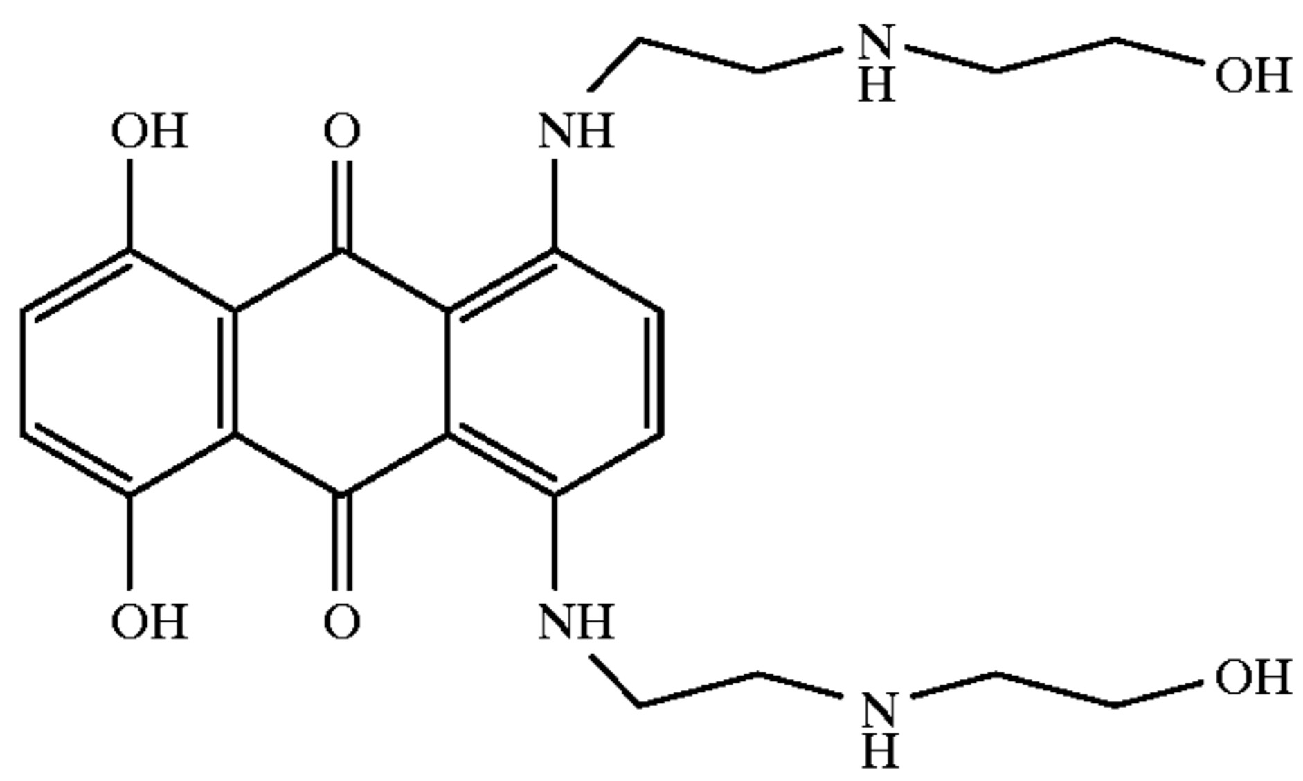
Mitoxantrone
