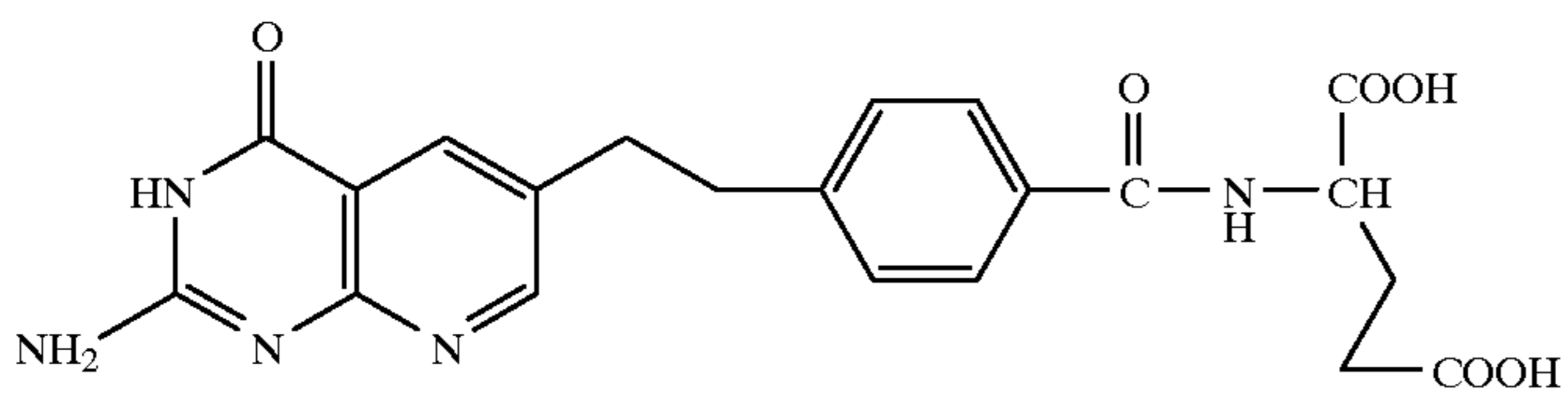
5, 10-dideaza tetrahydrofolate
