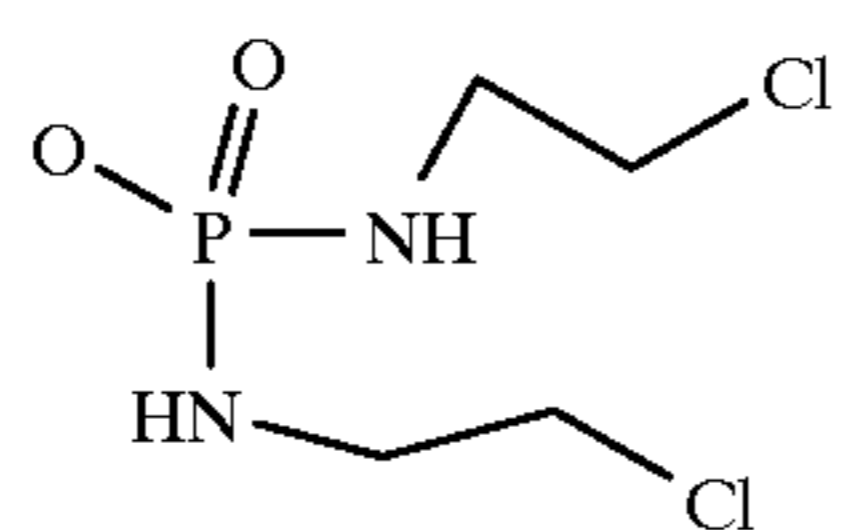
Isophosphoramidate Mustard
