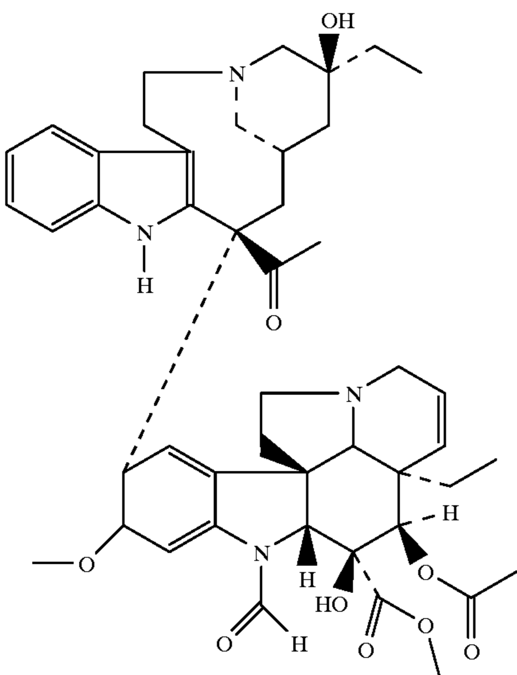
Vincristine
