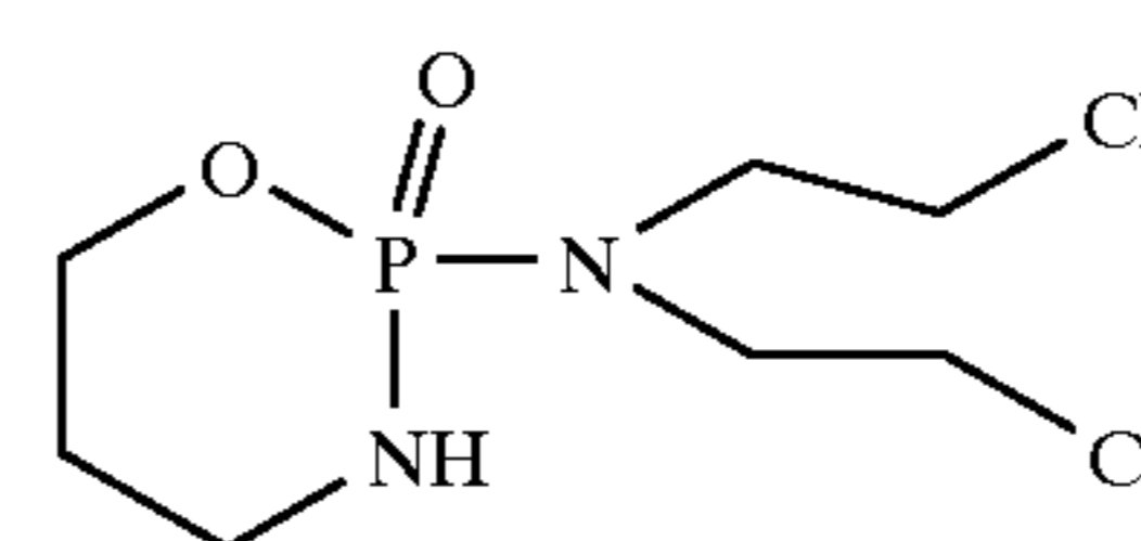
Cyclophosphamide
