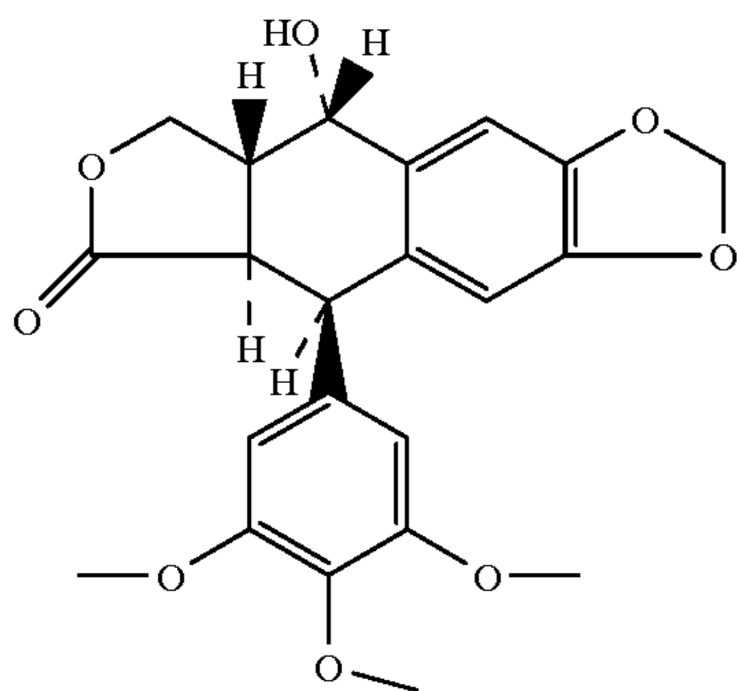
Podophyllotoxin
