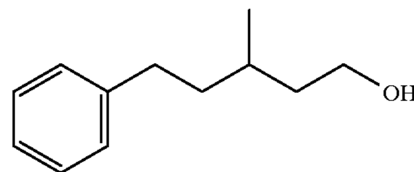
5-phenyl-3-methylpentanol
