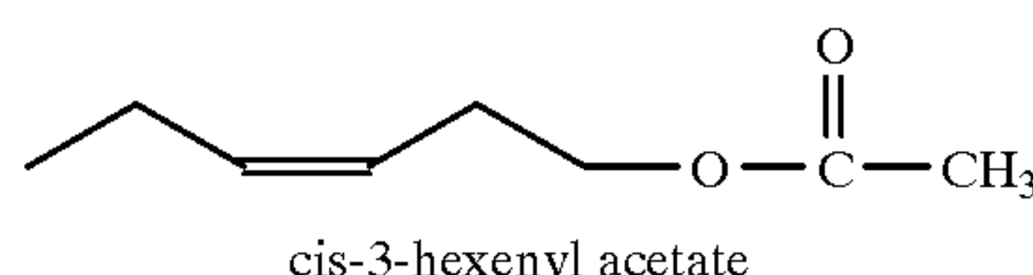
cis-3-hexenyl acetate
