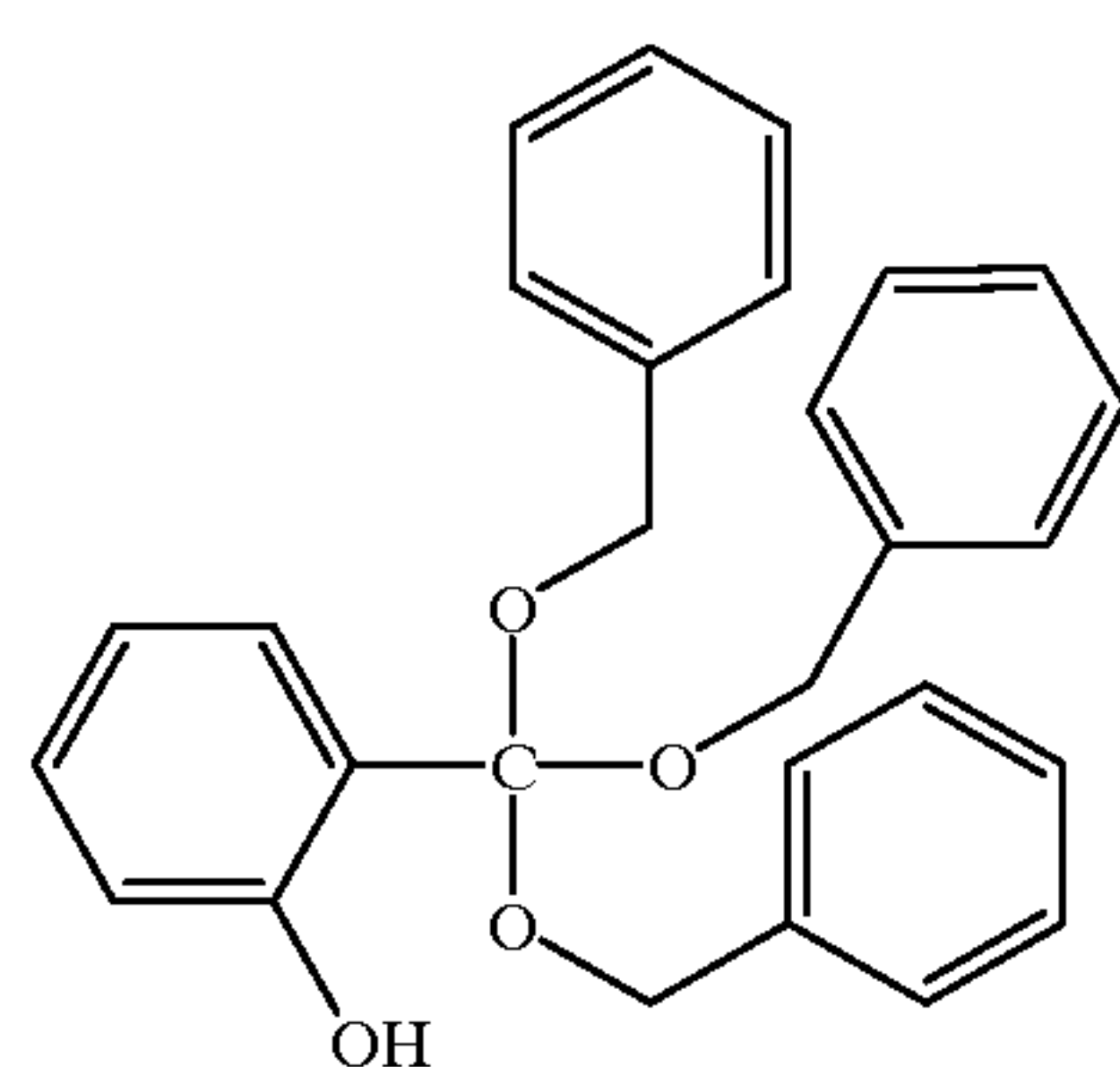
tris(benzyl) orthosalicylate
