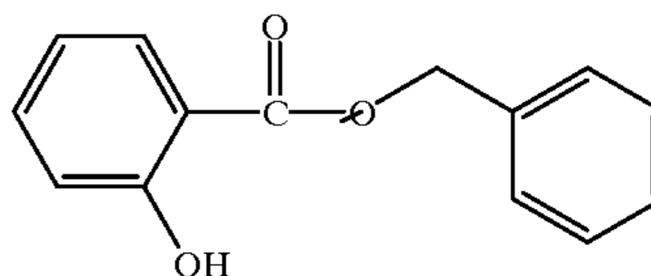
benzyl salicylate
