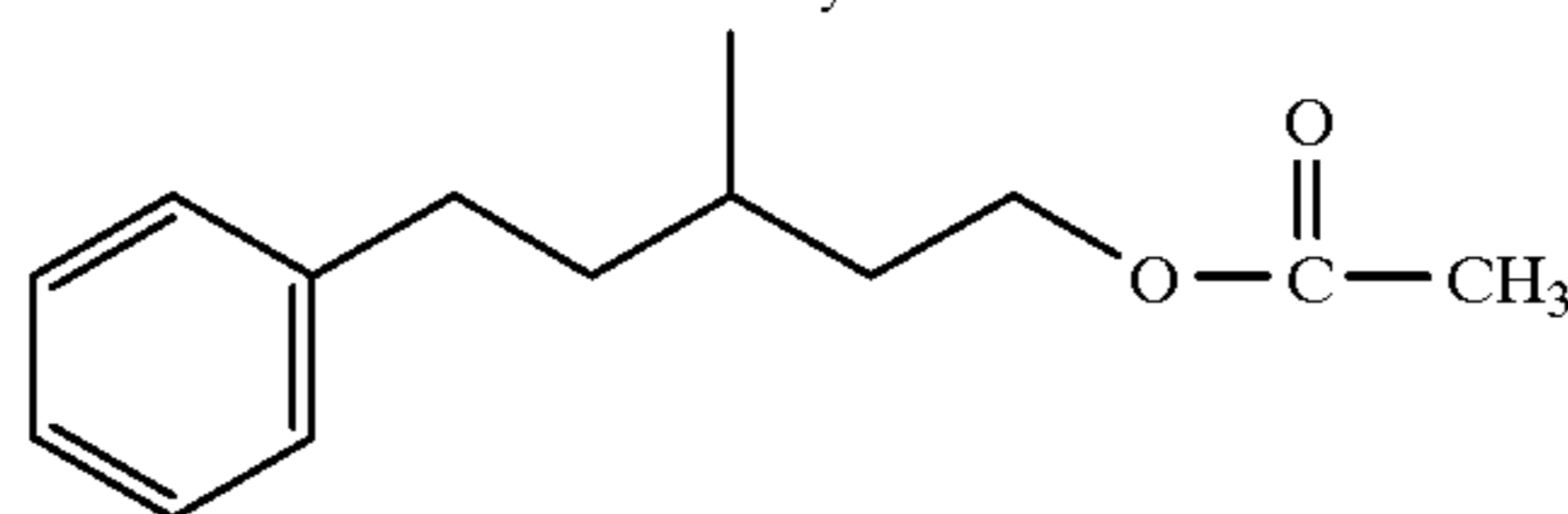
5-phenyl-3-methylpentyl acetate
