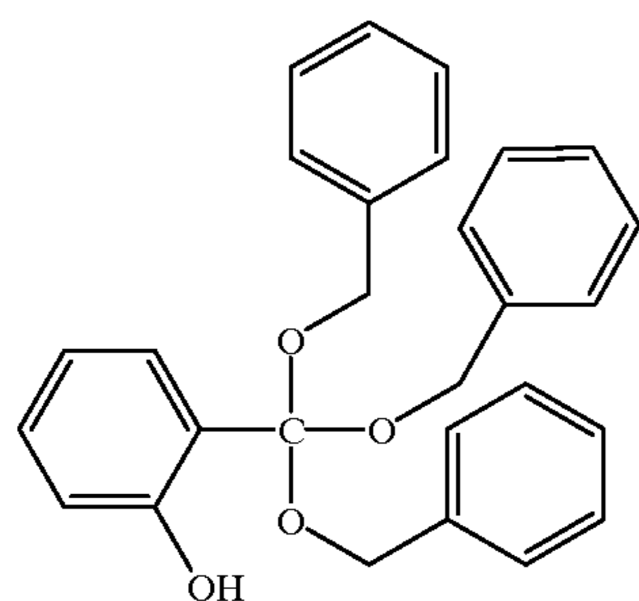
tris(benzyl) orthosalicylate
