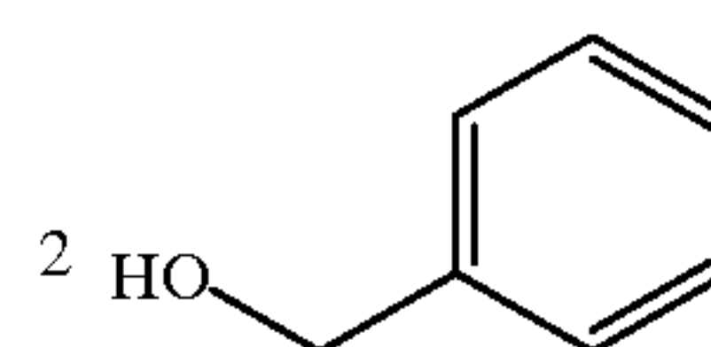
benzyl alcohol
