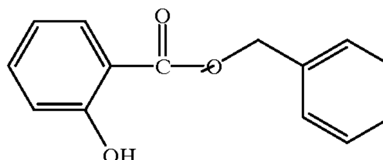
benzyl salicylate
