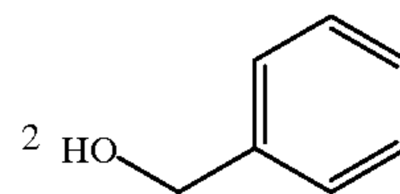
benzyl alcohol
