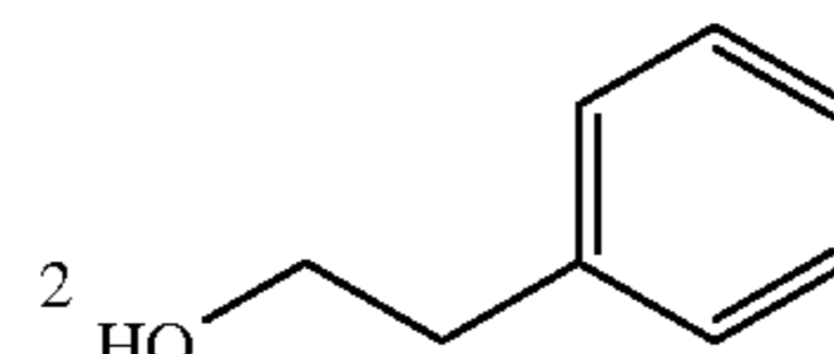
phenylethyl alcohol
