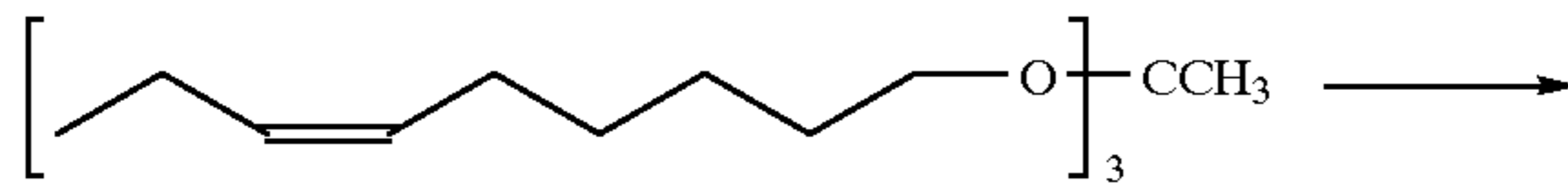
tris(cis-6-nonenyl) orthoacetate
