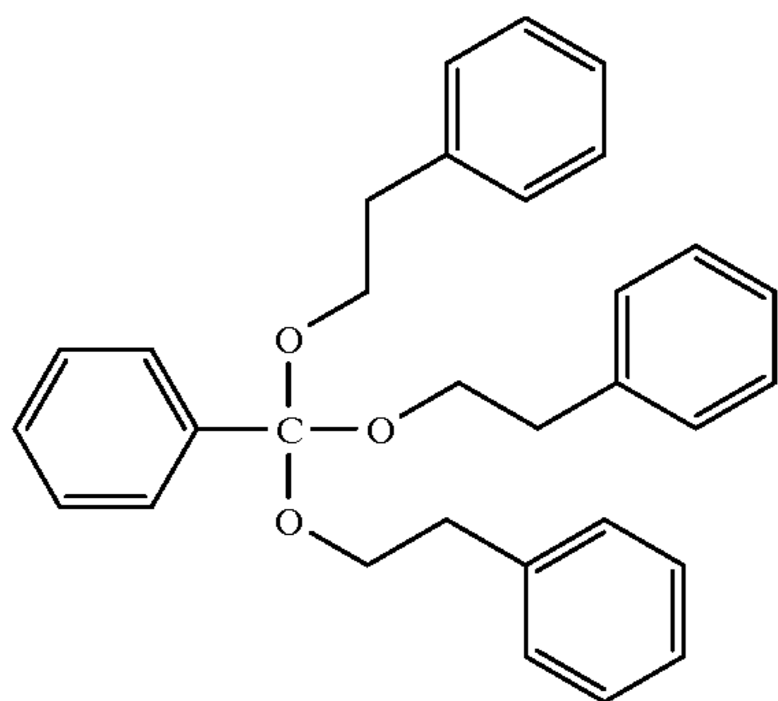
tris(phenylethyl) orthobenzoate
