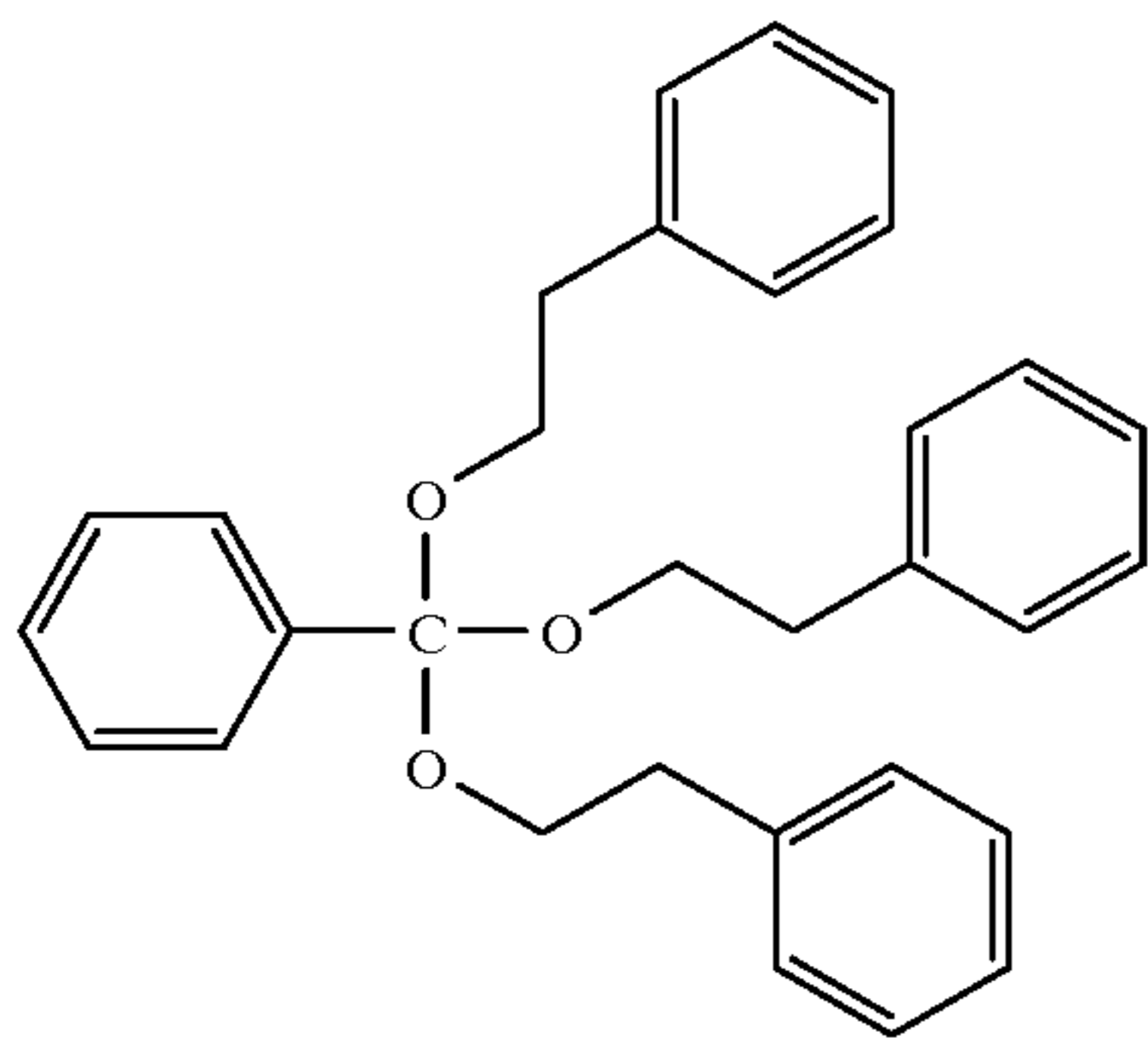
tris(phenylethyl) orthobenzoate
