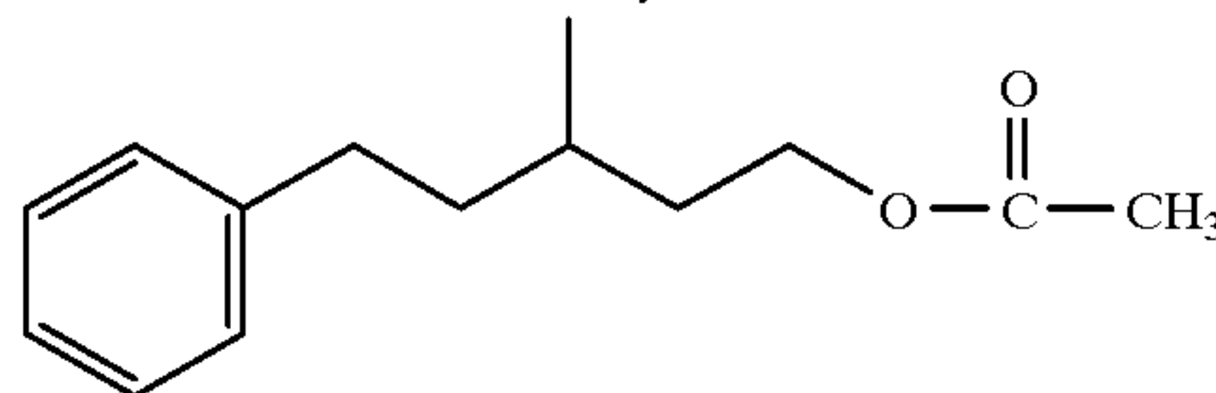
5-phenyl-3-methylpentyl acetate
