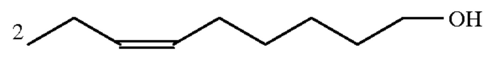
cis-6-nonenol
