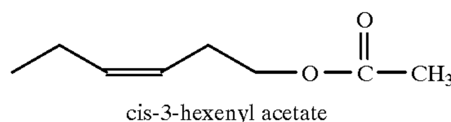
cis-3-hexenyl acetate
