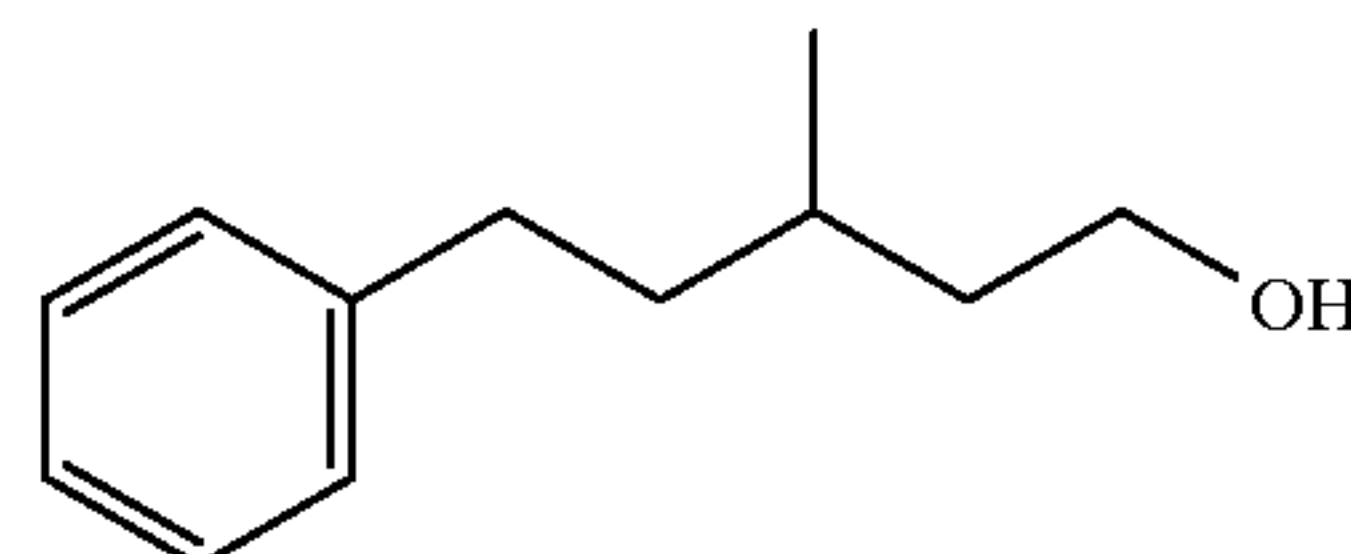
5-phenyl-3-methylpentanol
