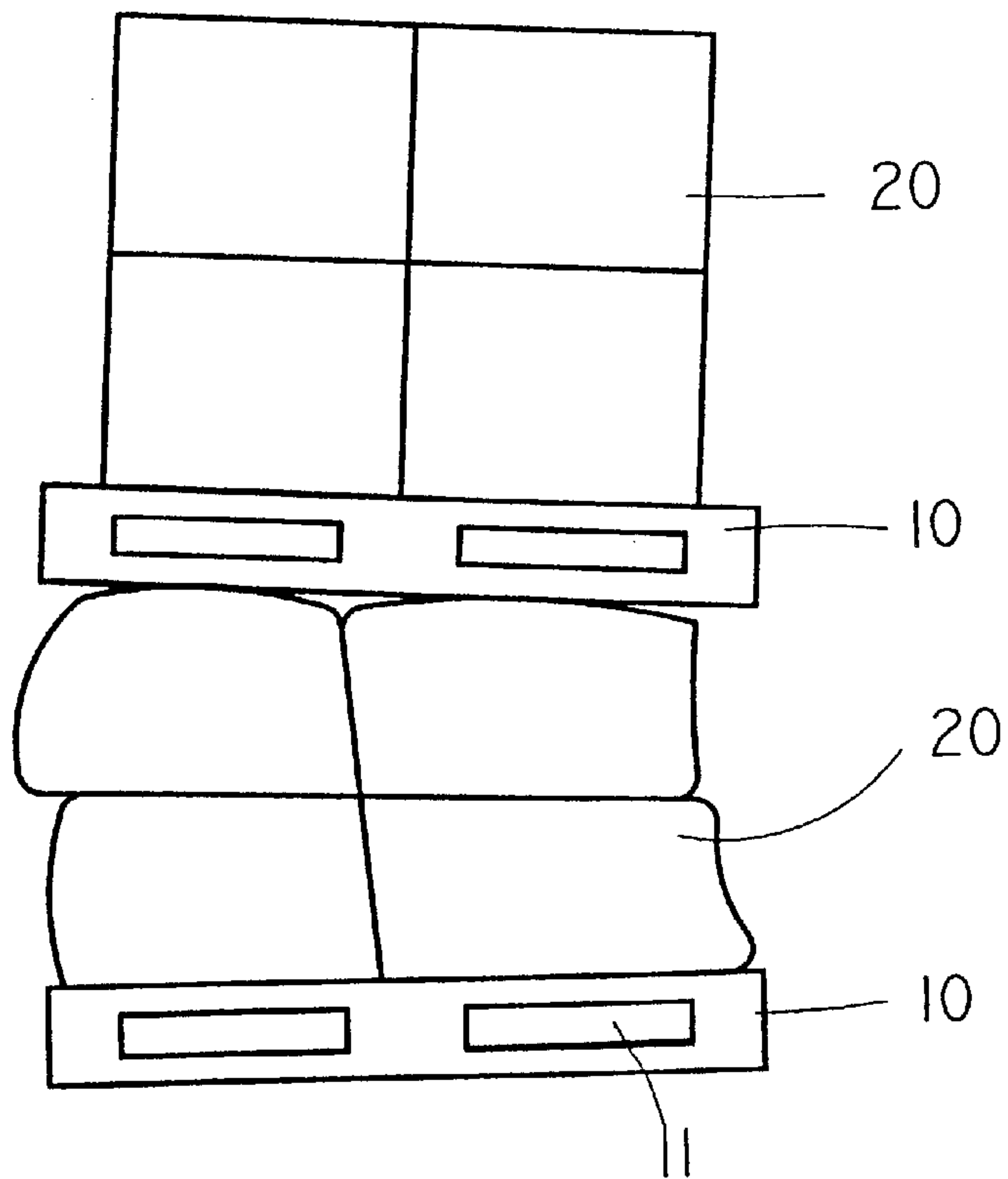
Fig. 2 PRIOR ART
