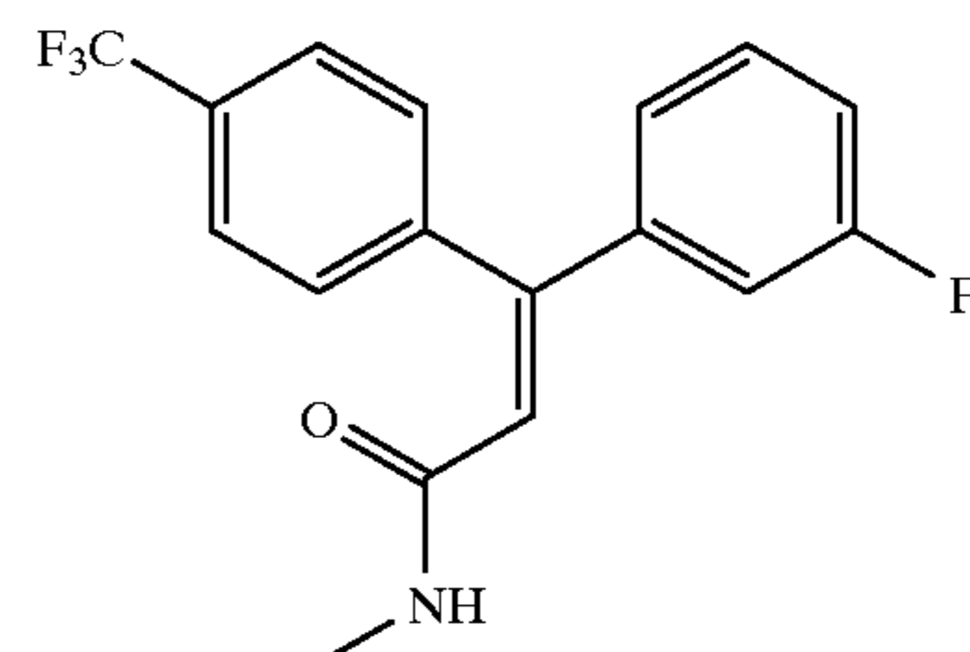
(E)-3-(4-α,α,α-trifluoromethylphenyl)-3-(3-fluorophenyl)-N-methyl-2-propenamide
