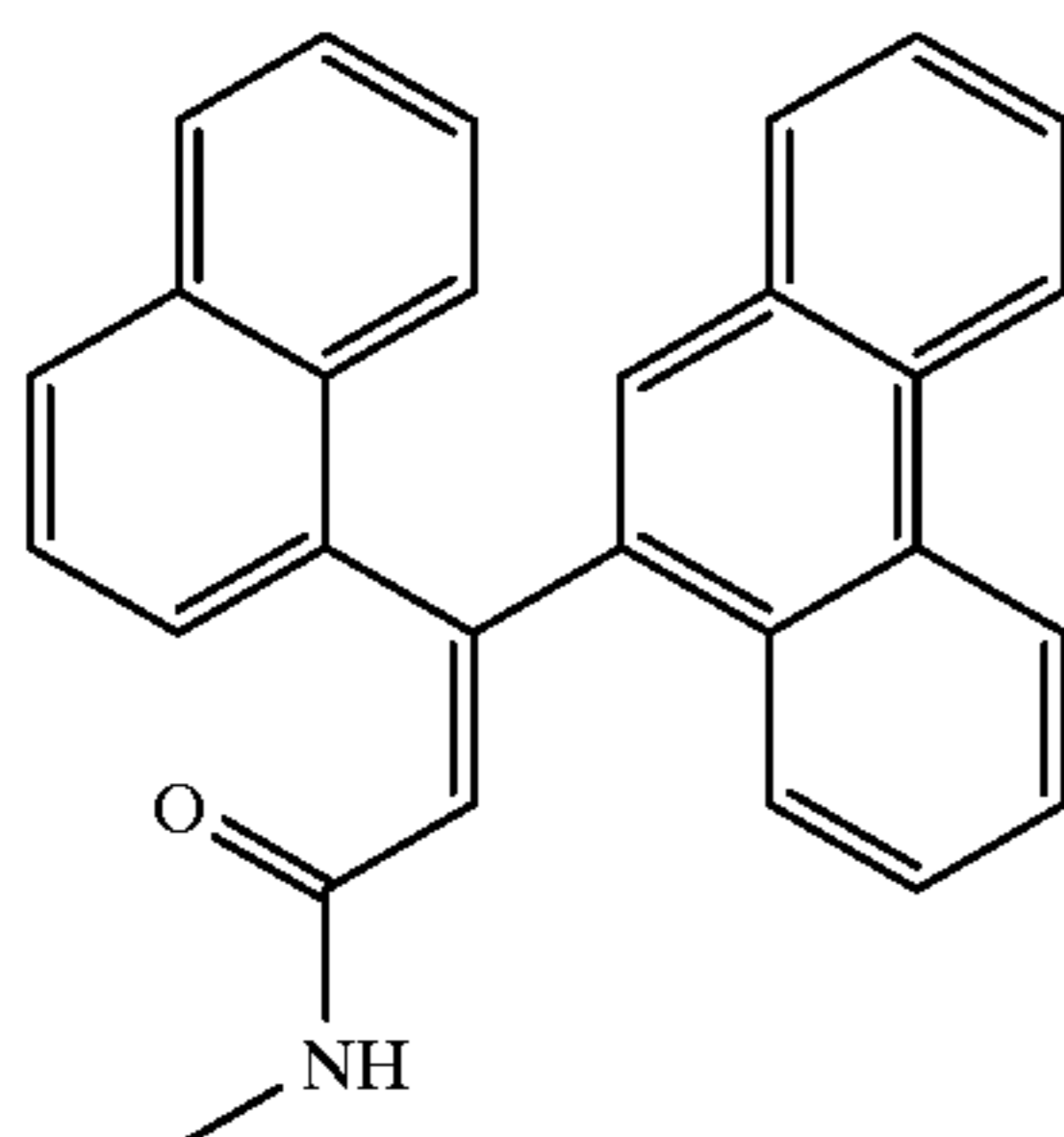
(E)-N-methyl-3-(1-naphthyl)-3-(9-phenanthryl)-2-propenamide
