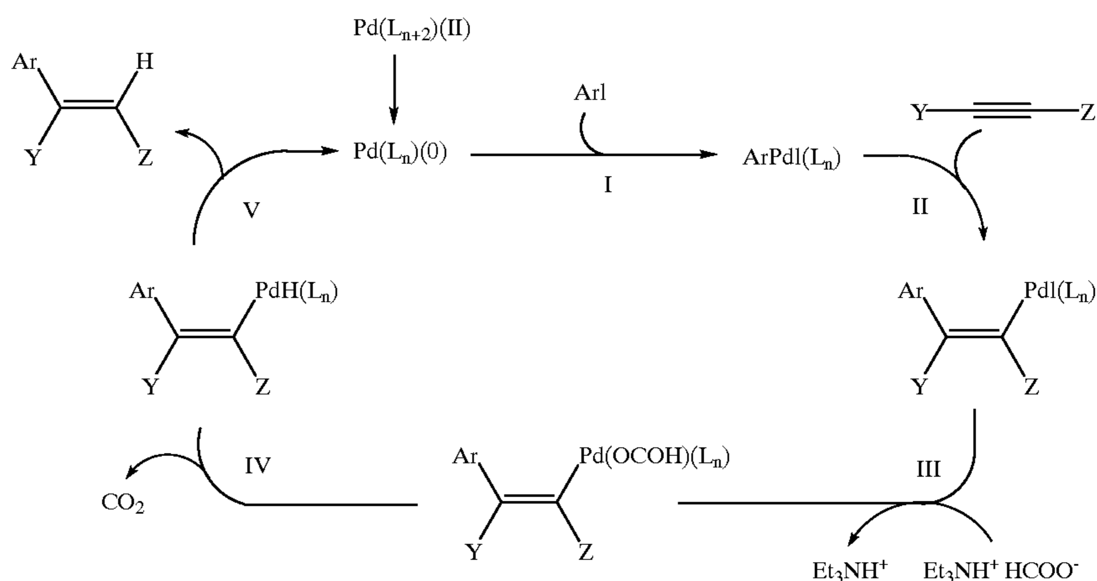
Scheme 2
