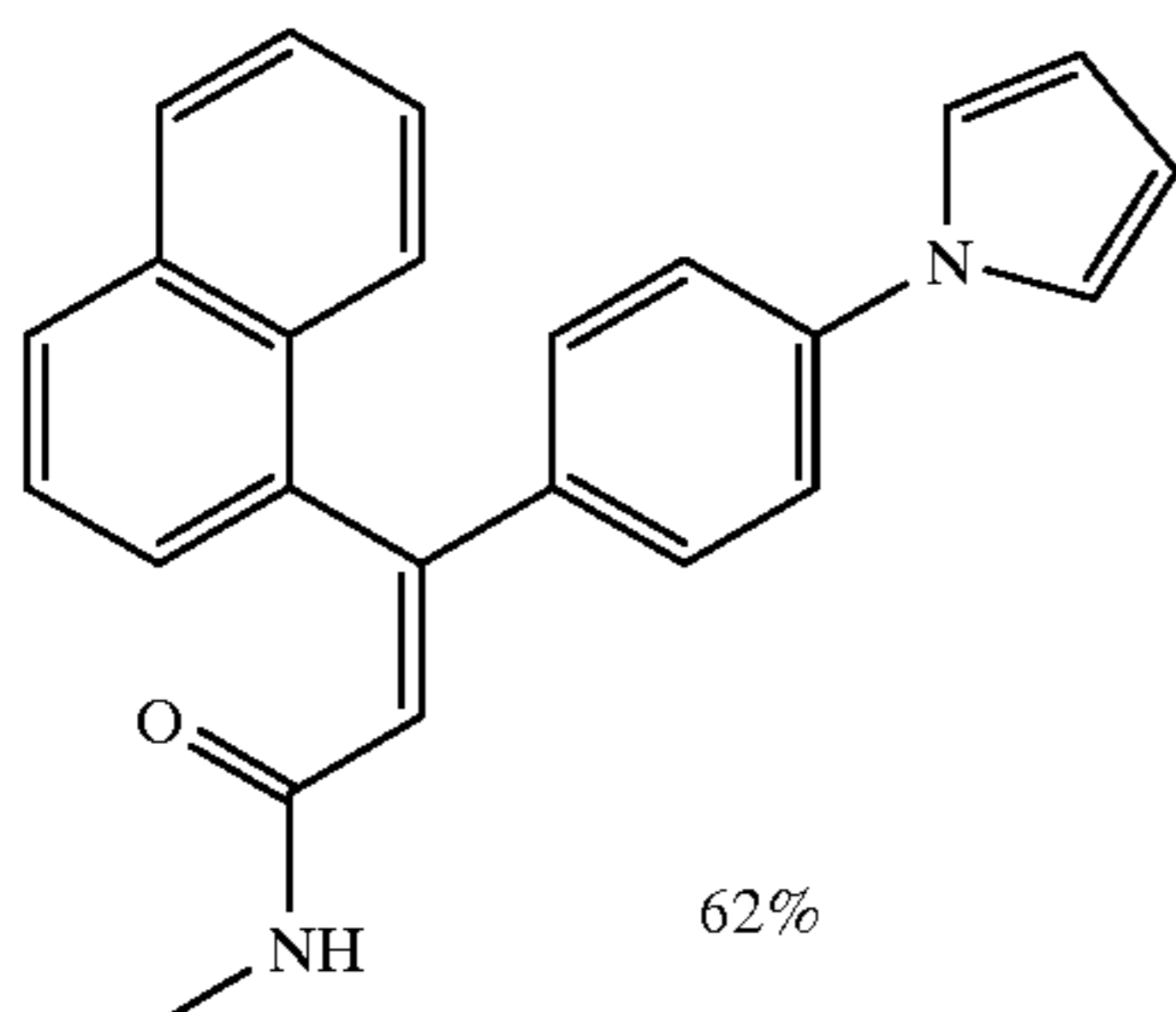
(Z)-N-methyl-3-(1-naphthyl)-3-[4-(1-pyrrolo)phenyl]-2-propenamide
