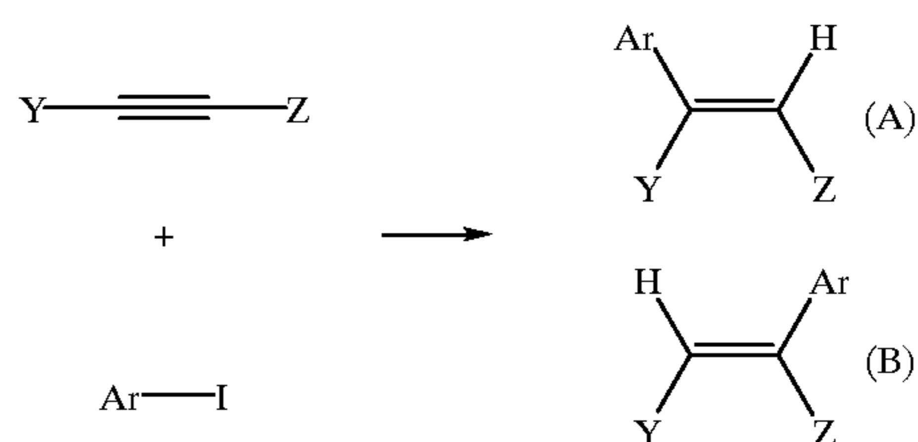
Scheme 1
