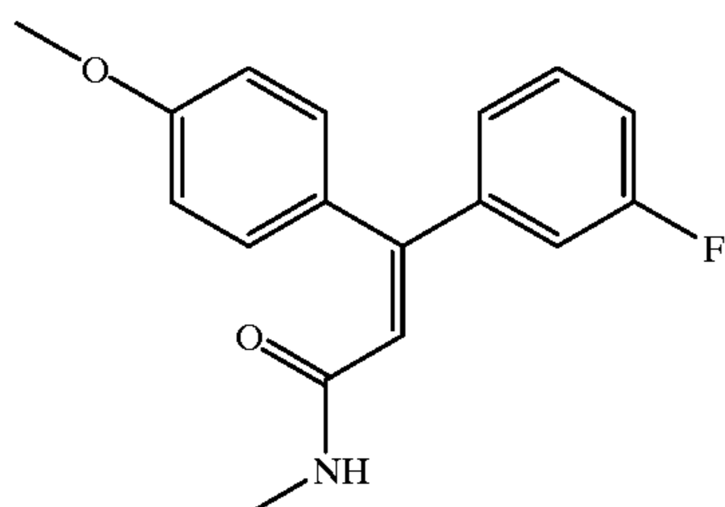
(E)-3-(4-anisyl)-3-(3-fluorophenyl)-N-methyl-2-propenamide
