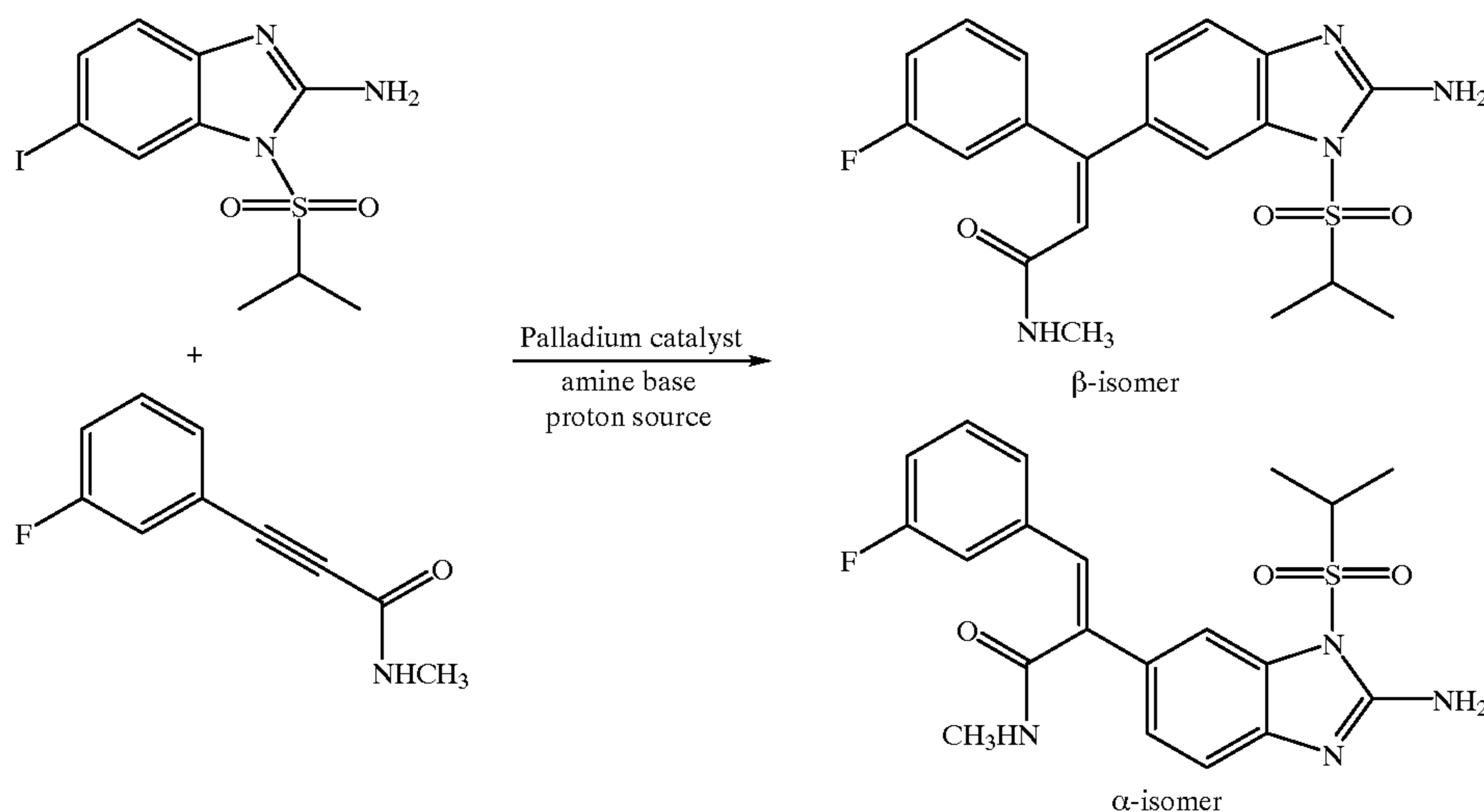
Scheme 4
