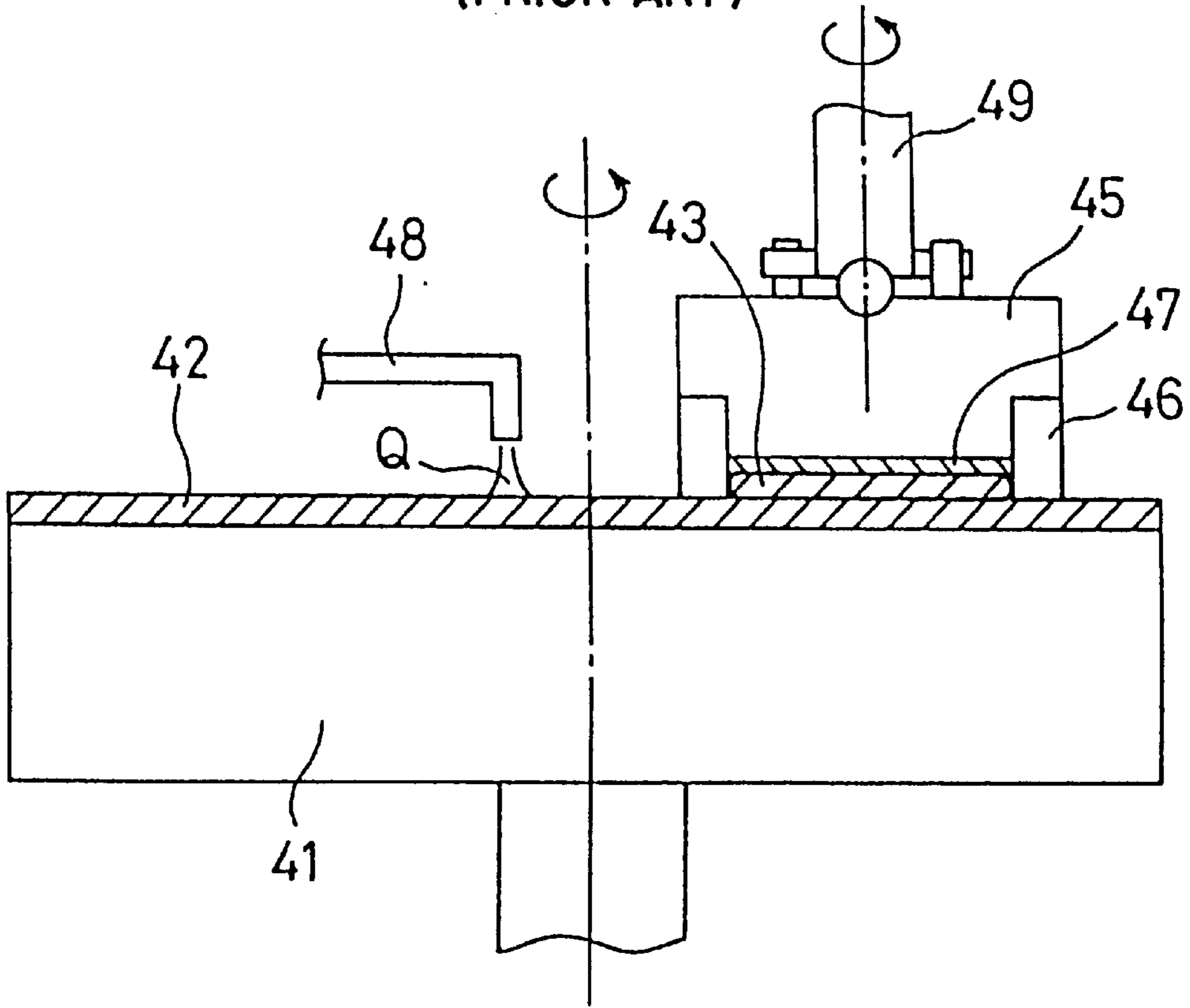
FIG. 15 (PRIOR ART)
