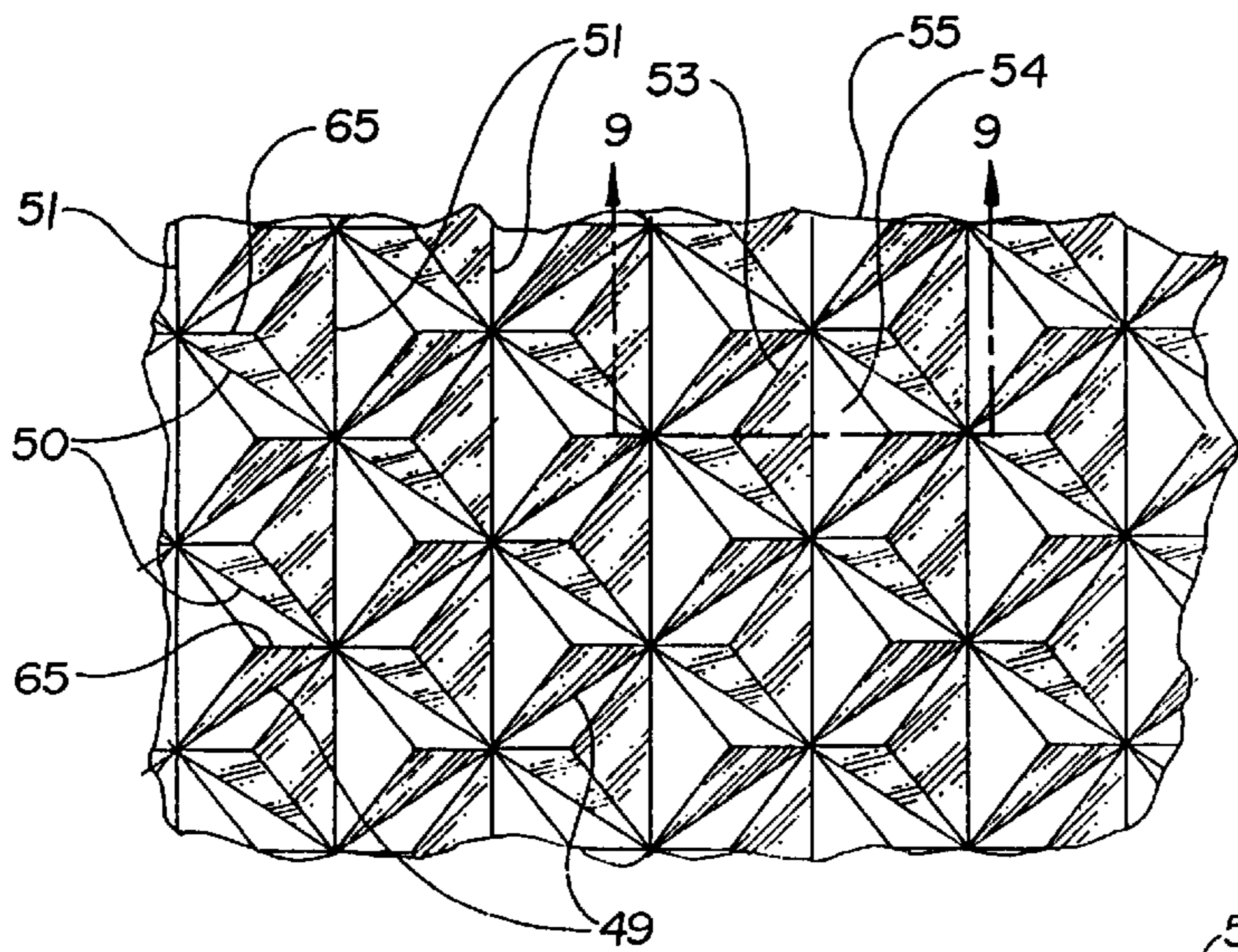
Fig. 8 PRIOR ART
